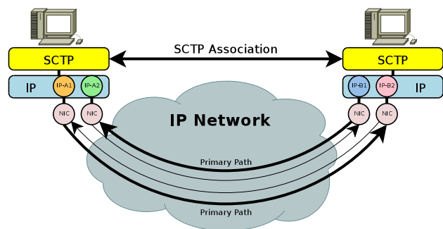
Figure 1. Multi-Homing with SCTP
