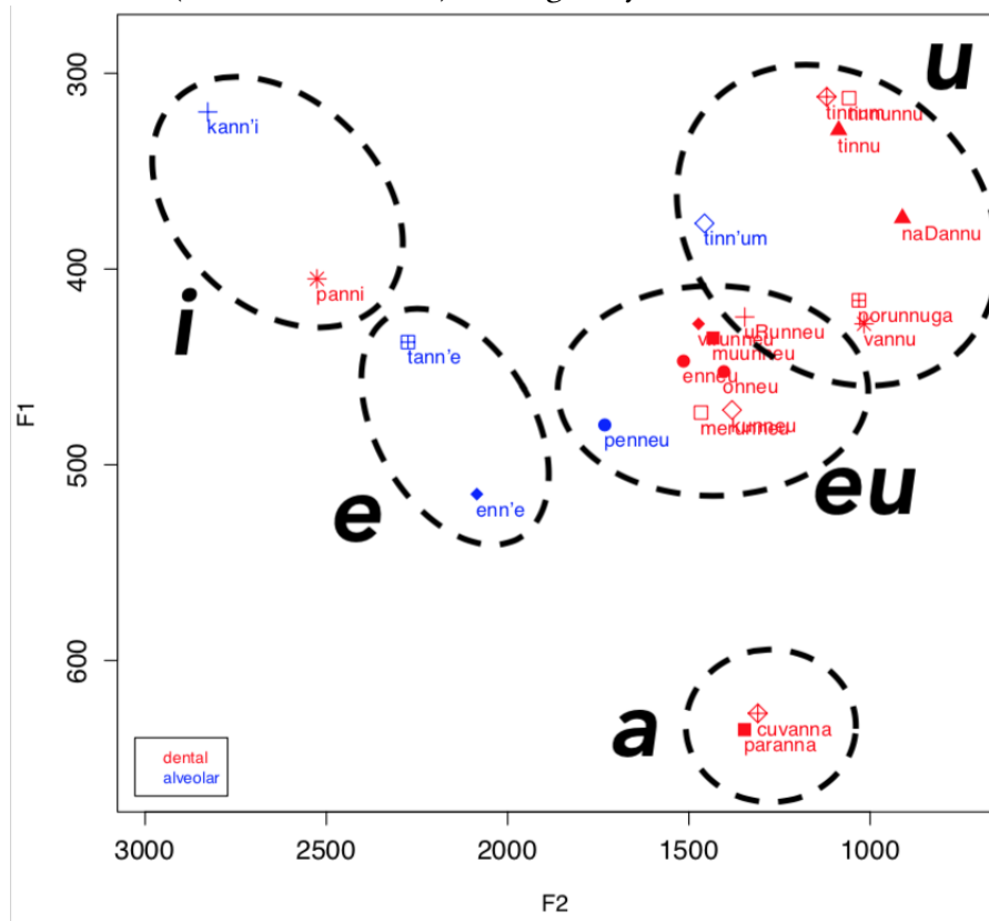
Figure 5: F1xF2 plots for the midpoint of the vowel following dental nn (in red) and alveolar nn' ( nn' below, in blue), averaged by word.
