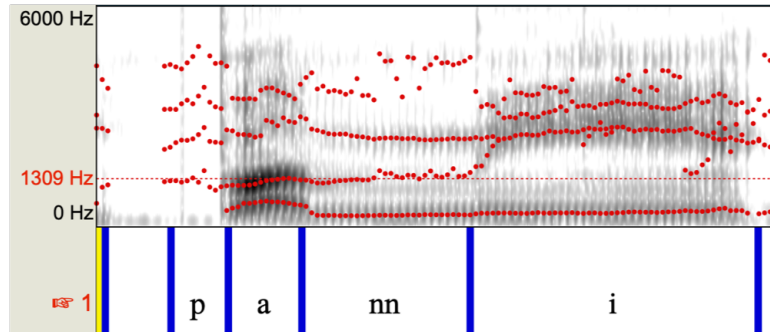
Figure 2: Spectrogram of panni ‘pig’, showing F2 lowered adjacent to the dental nasal nn .
