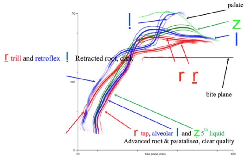
Figure 1: Ultrasound tracings from Scobbie et al. (2013). The tongue blade points to the right.
