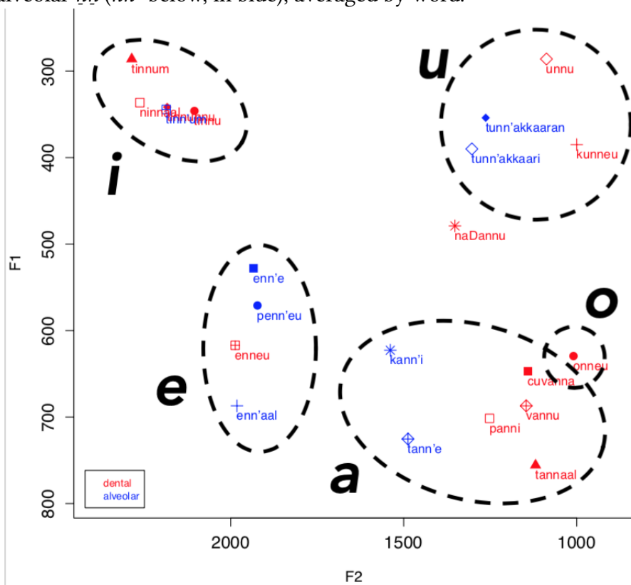
Figure 4: F1xF2 plots for the midpoint of the vowel preceding dental nn (in red) and alveolar nn' ( nn' below, in blue), averaged by word.
