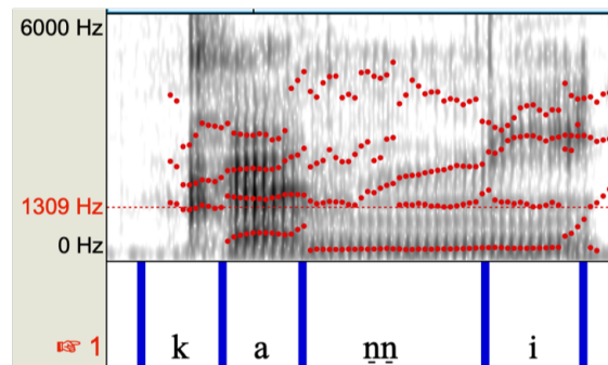
Figure 3: Spectrogram of kanni ‘(a month)’, showing F2 raised adjacent to the alveolar nasal nn̥ . (Note that the actual F2 is mistracked as F3 in the final vowel i .)
