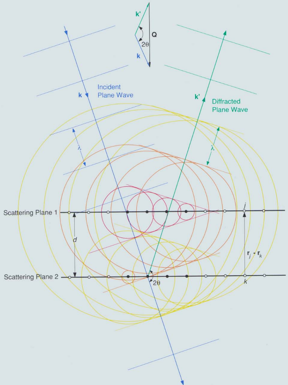
Fig. 6. As a neutron (represented in the figure by a plane wave) passes through a lattice of regularly spaced scattering centers (rather than the single scattering center of Fig. 4), the spherical wavefronts that represent scattered neutrons will overlap and interfere with each other. In those directions in which the interference is constructive, scattered neutrons may be measured. The figure depicts such constructive interference in two dimensions with planar wavefronts represented as lines, spherical wavefronts as colored circles, and the scattering centers as small circles. To simplify the diagram, the scattering is shown only for four centers (solid black) in each of the two rows of scattering planes. Also, color is used to relate each incident wavefront to the scattered wavefronts that have so far been generated by it. Thus, the incident red wavefront has passed over and scattered from four scattering centers in Scattering Plane 1; the orange wavefront has passed over and scattered from these scattering centers plus the leftmost scattering center in Scattering Plane 2; the yellow wavefront has passed over all eight scattering centers in both planes. For constructive interference to take place, Q \cdot (r_j - r_k) = Qd = 2\pi n must be satisfied, where |r_j - r_k| = d is the distance between the two scattering planes and n is an integer. Combining this condition with Q = 4\pi \sin \theta / \lambda (from Fig. 5a) yields Bragg's law: n\lambda = 2d \sin \theta .
