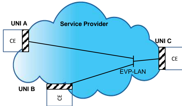
Figure 2: Subscriber’s view of EVP-LAN Service
