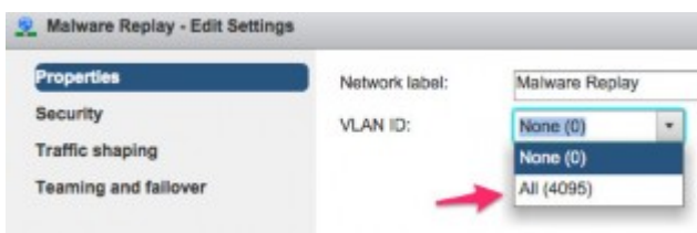
Figure 2: vSwitch VLAN Troubleshooting Config in port-groups
