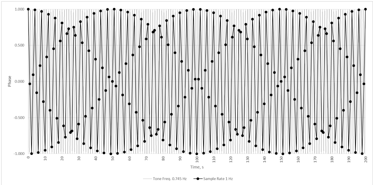
Figure VI.3 – Sub-Nyquist artefact for m = 3 , n = 4 , \epsilon = -0.005 Hz
