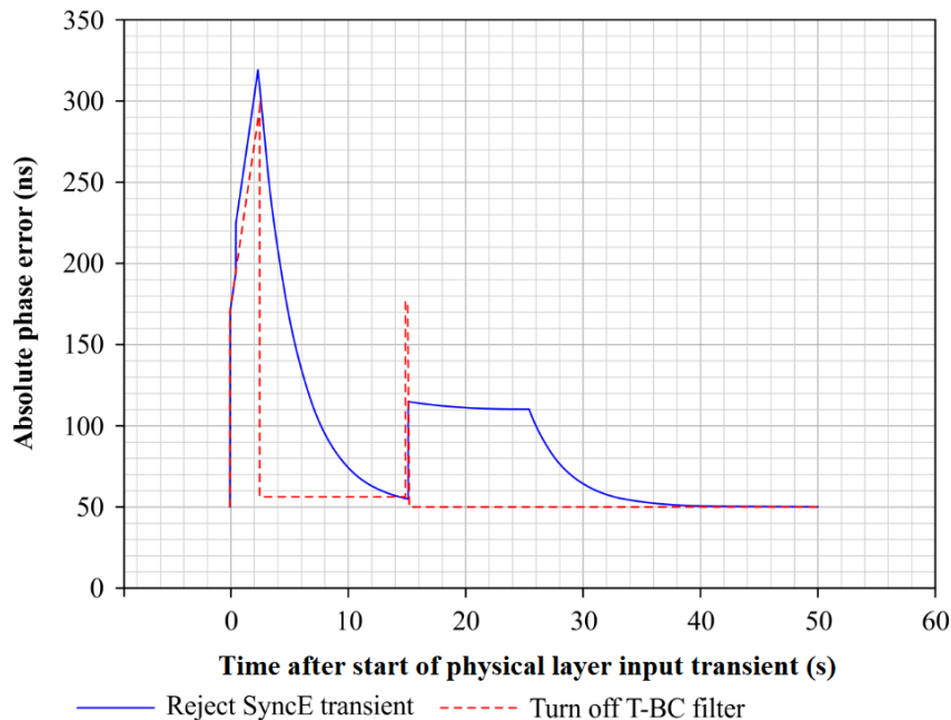
Figure II.1 – T-BC output phase error histories for each of the two techniques, assuming physical layer frequency input transient starts at time zero
