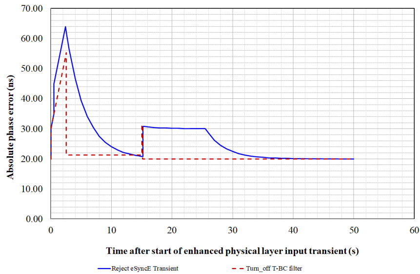
Figure II.6 – T-BC output phase error histories for each of the two techniques, assuming enhanced physical layer frequency input transient starts at time zero
