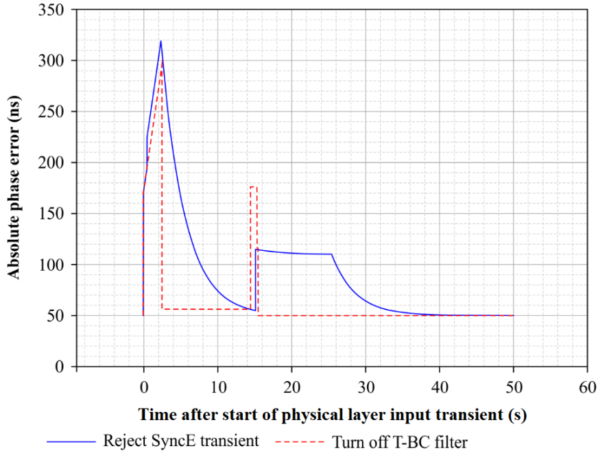
Figure II.2 – T-BC output phase error histories for each of the two techniques, assuming physical layer frequency input transient starts at time zero, and allowing 1 s of margin for the time of second 120 ns phase jump for scheme (b)
