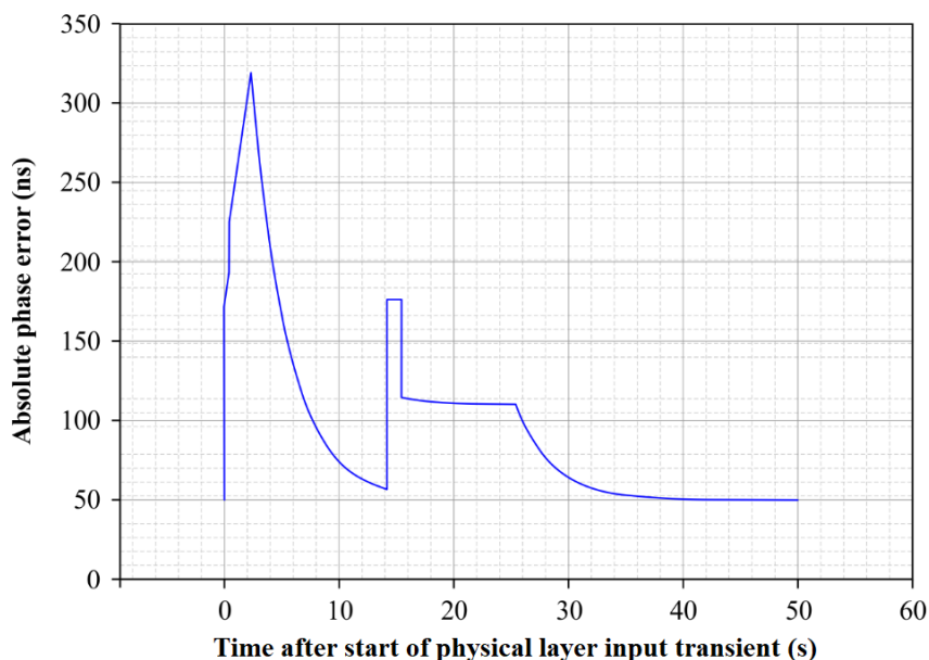
Figure II.5 – Upper envelope of masks of Figure II.3 and Table II.4 after applying simplifications in the range 14.25-14.5 s
