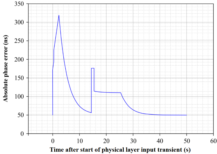
Figure II.4 – Upper envelope of masks of Figure II.3 and Table II.4
