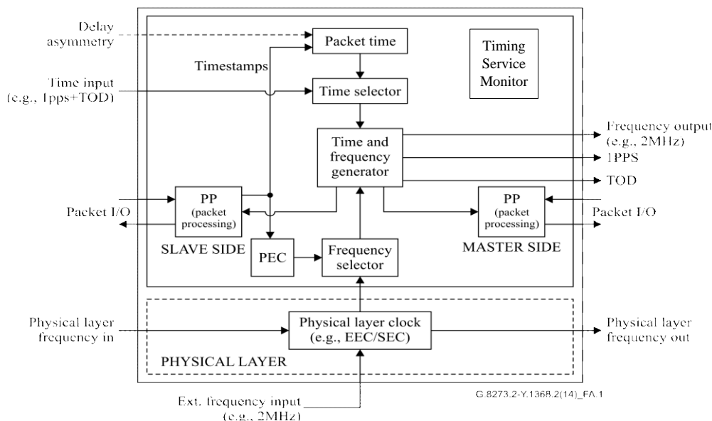
Figure A.1 – Telecom boundary clock and telecom synchronous clock models
