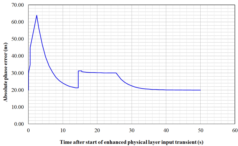
Figure II.8 – Upper envelope of masks of Figure II.7
