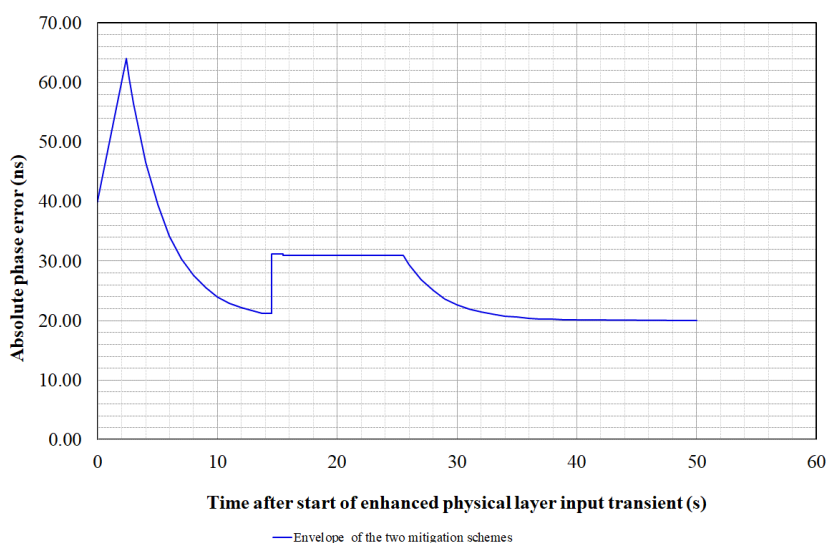
Figure C.1 – Phase error limit for PTP and 1 PPS output phase error transient after the start of the enhanced physical layer frequency input transient
