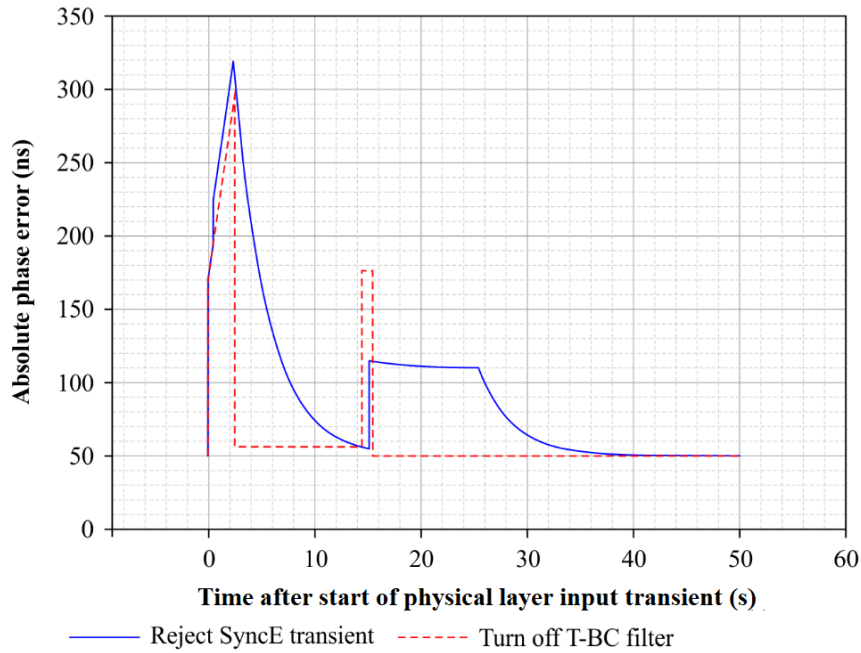
Figure II.3 – T-BC output phase error histories for each of the two techniques, assuming physical layer frequency input transient starts at time zero, and allowing 1 s of margin for the time of second 120 ns phase jump for scheme (b)
