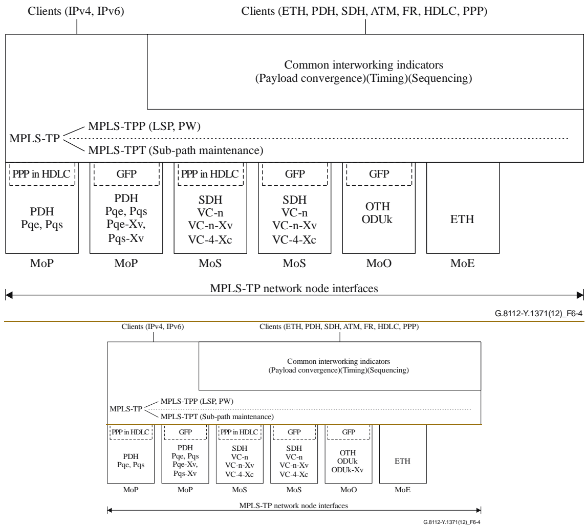
Figure 6-4 – Structure of the MPLS-TP network-to-node interfaces
