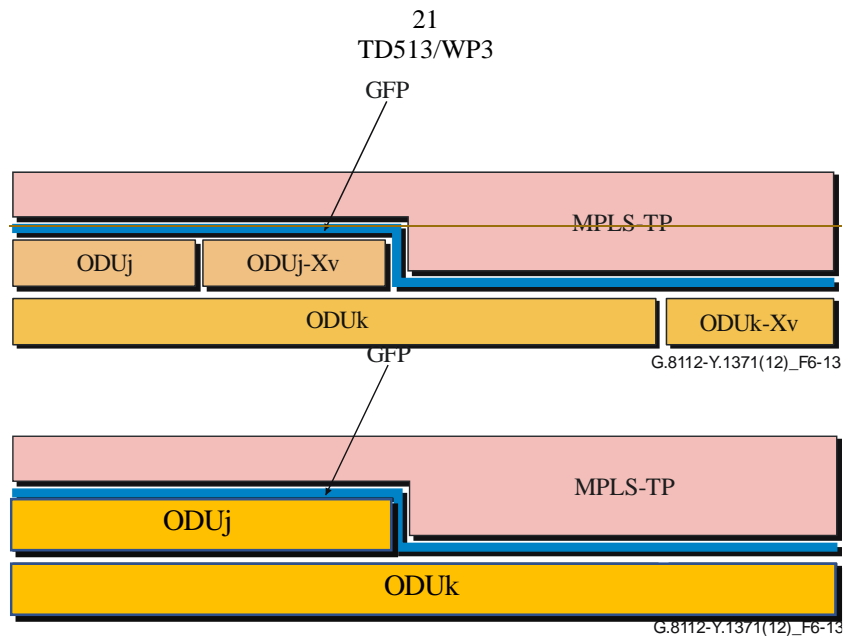
Figure 6-13 – Components of the MPLS-TP over OTH NNI
