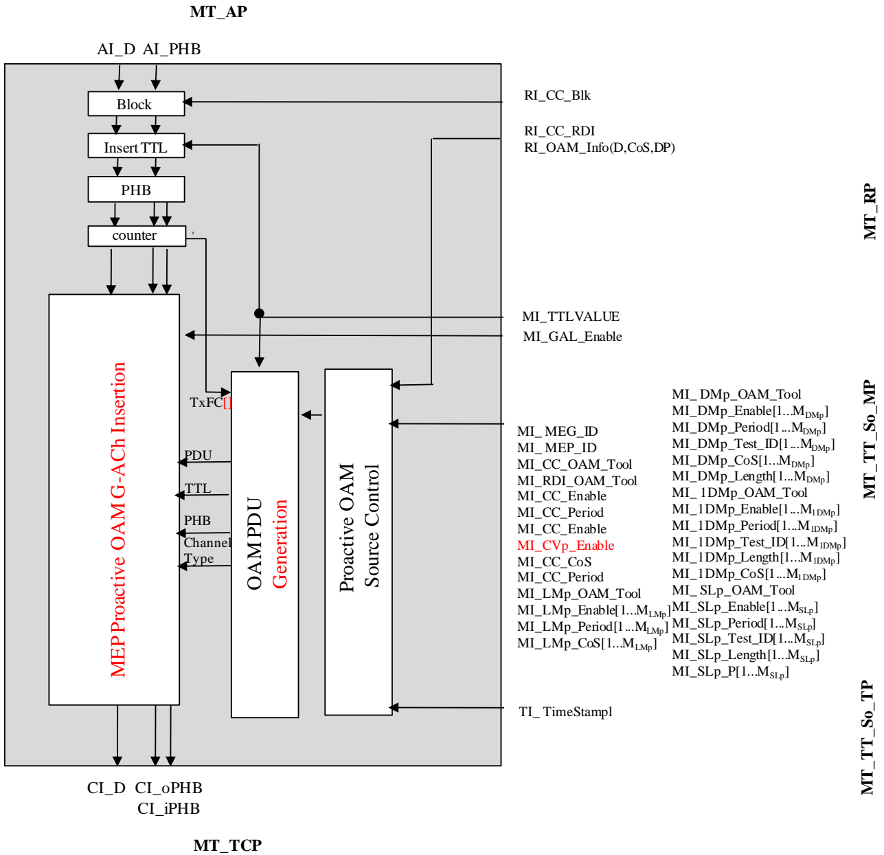
Figure 9-5/G.8121/Y.1381 –MT_TT_So process diagram
