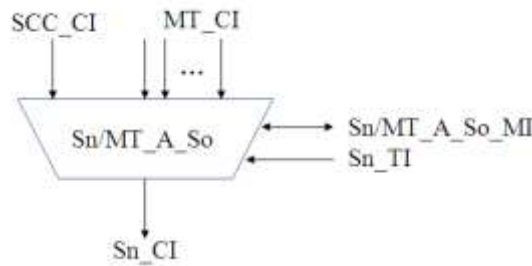
Figure 11-1/G.8121/Y.1381 – Sn/MT_A_So symbol
