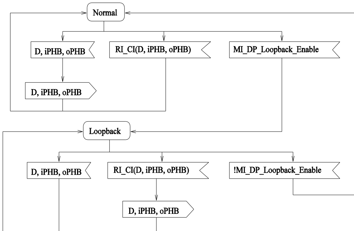
Figure 8-31/G.8121/Y.1381 – Dataplane Loopback Source process
