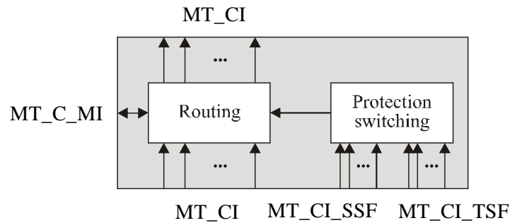
Figure 9-2/G.8121/Y.1381 – MT_C process diagram
