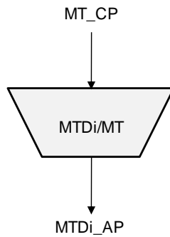
Figure 9-21/G.8121/Y.1381 – MTDi/MT_A_So symbol
