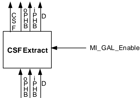
Figure 8-24/G.8121/Y.1381 – CSF Extract process
