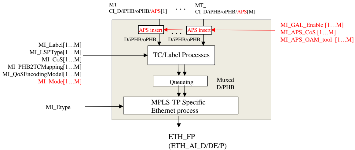
Figure11-38 – ETH/MT_A_So process
