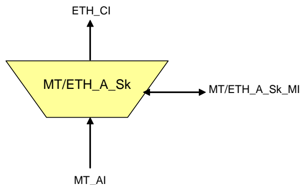
Figure 10-3/G.8121/Y.1381 – MT/ETH_A_Sk function
