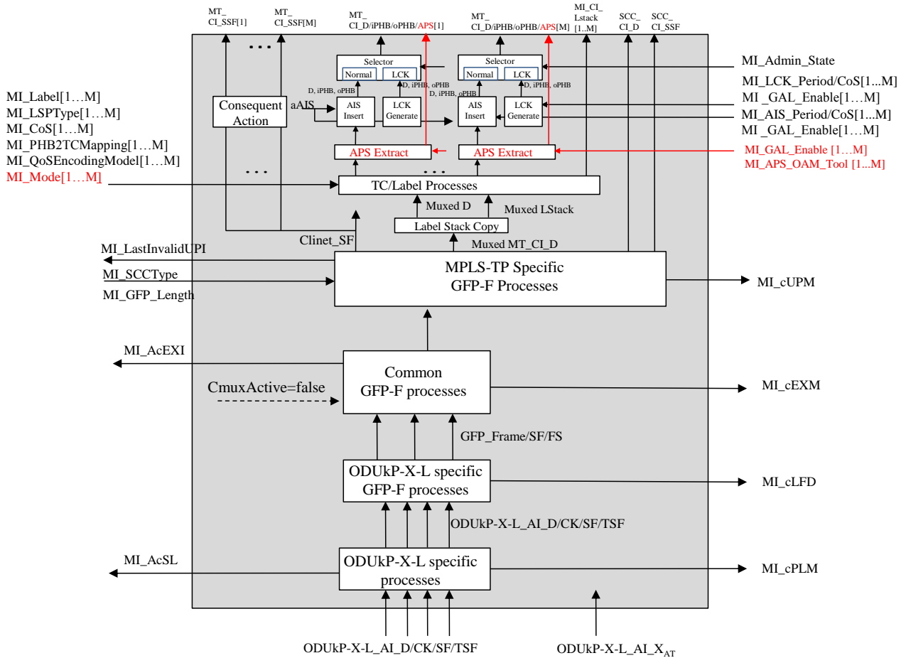
Figure 11-27/G.8121/Y.1381 – ODUkP-X-L/MT_A_Sk process diagram
