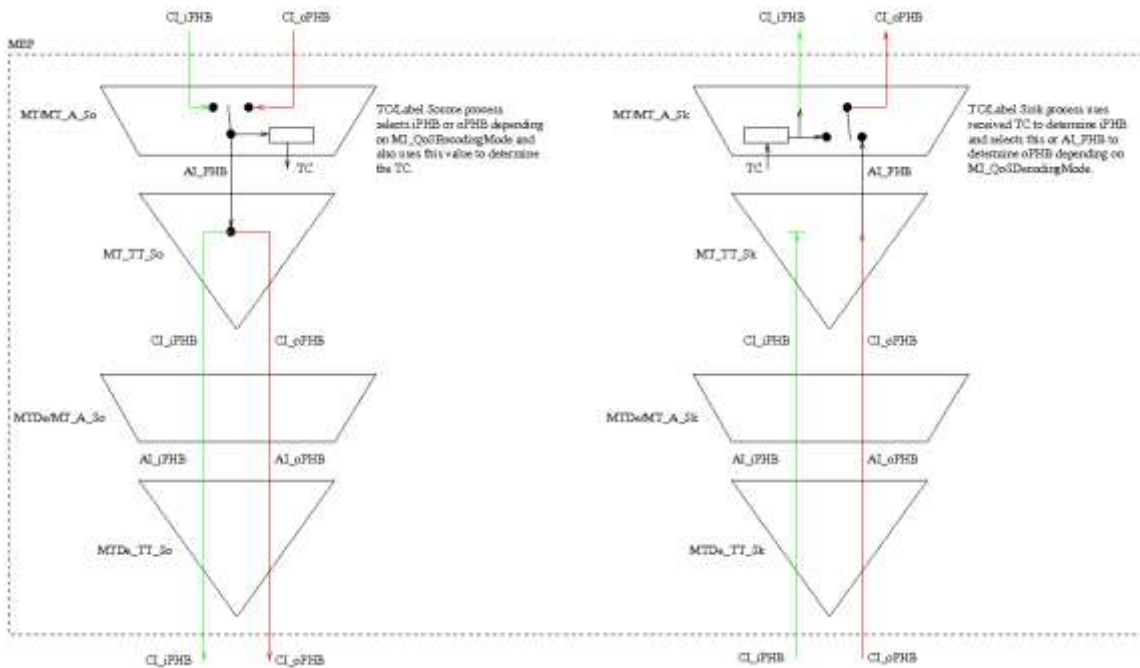
Figure II.1 – Flow of PHB information through a MEP
