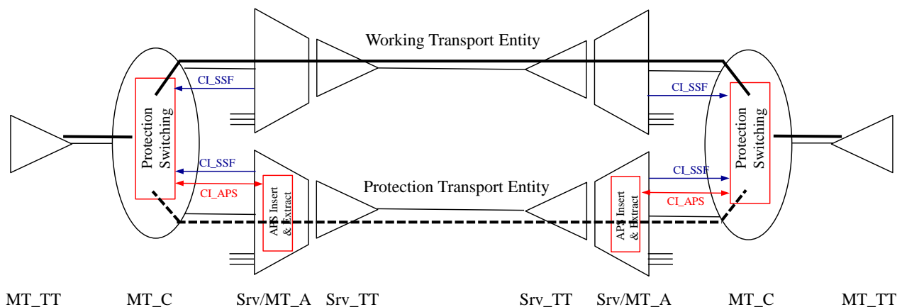
Figure III-1/G.8121/Y.1381 – MPLS-TP SNC/I protection switching architecture
