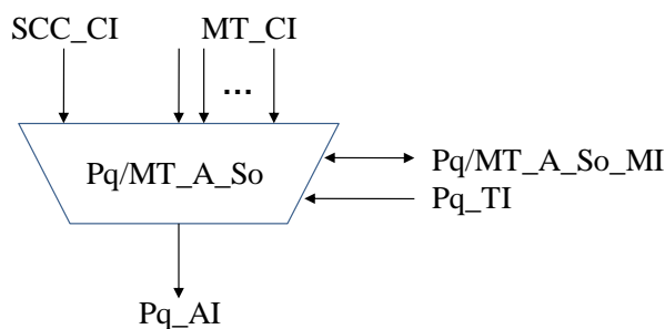
Figure 11-29/G.8121/Y.1381 – P q /MT_A_So symbol
