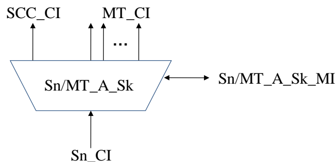
Figure 11-3/G.8121/Y.1381 – Sn/MT_A_Sk symbol
