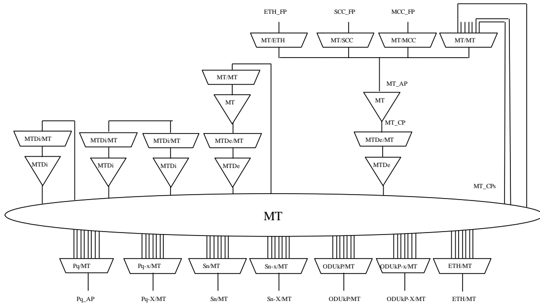
Figure 1/G.8121/Y.1381 – MPLS-TP atomic functions
