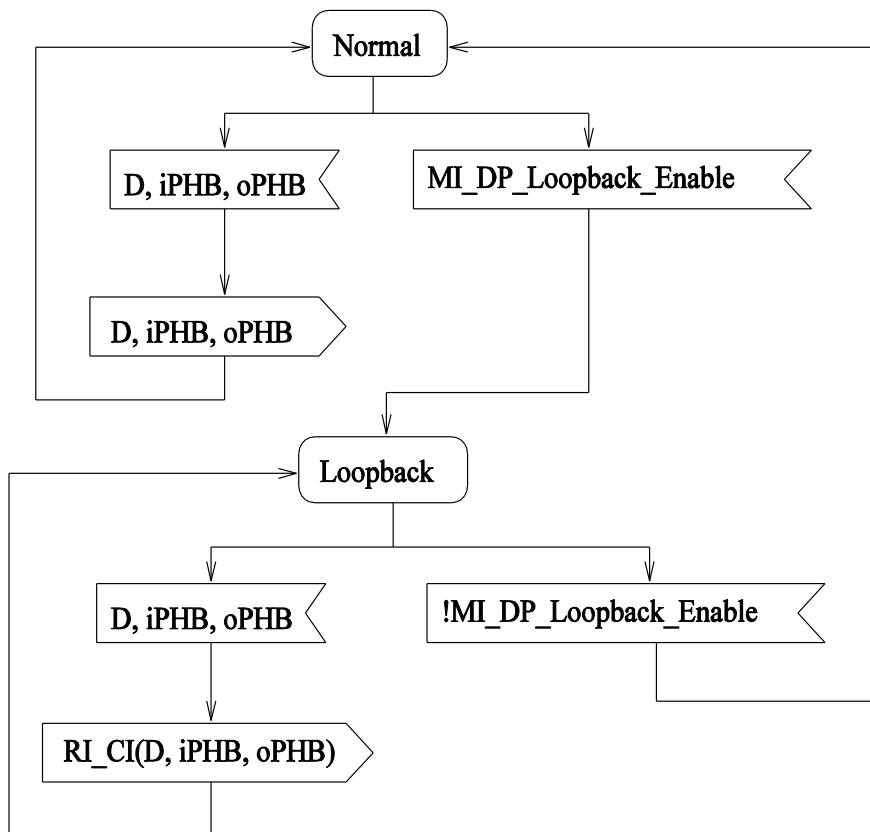
Figure 8-30/G.8121/Y.1381 – Dataplane Loopback Sink process
