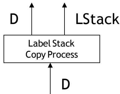
Figure 8-5/G.8121/Y.1381 – Label Stack Copy Process
