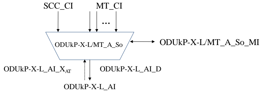
Figure 11-26/G.8121/Y.1381 – ODUkP-X-L/MT_A_Sk symbol
