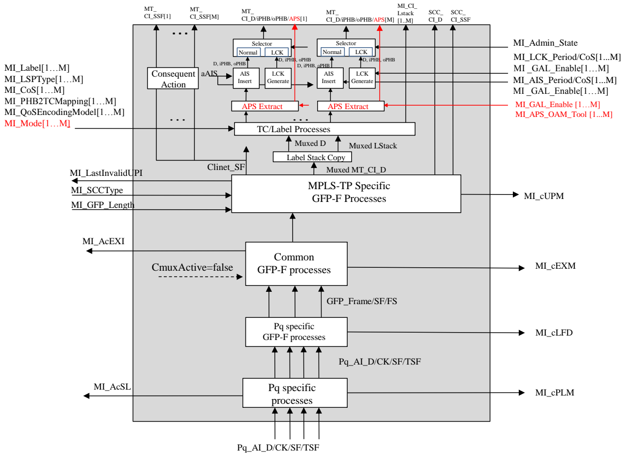
Figure 11-32/G.8121/Y.1381 – Pq/MT_A_Sk process diagram
