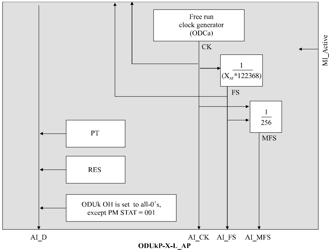
Figure 11-25/G.8121/Y.1381 – ODUkP-X-L specific source processes
