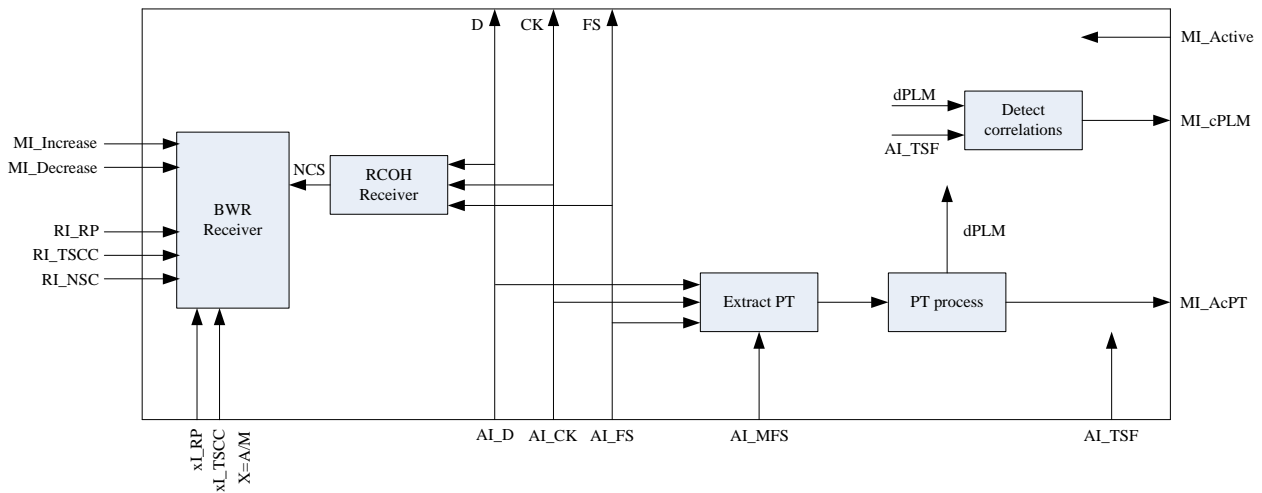
Figure 11-28e/G.8121/Y.1381 – ODUkP (k=flex) specific sink processes
