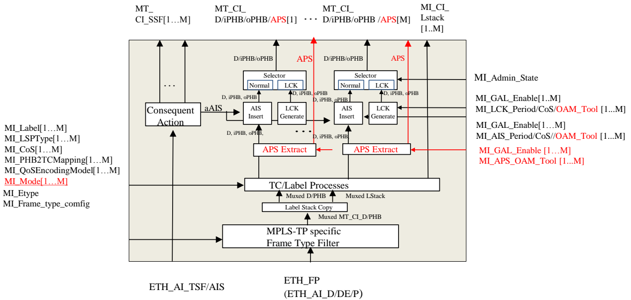
Figure 11-40 – ETYn/ETH_A_Sk process
