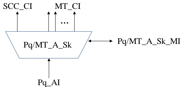
Figure 11-31/G.8121/Y.1381 – Pq/MT_A_Sk symbol
