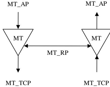
Figure 9-3/G.8121/Y.1381 – MT_TT
