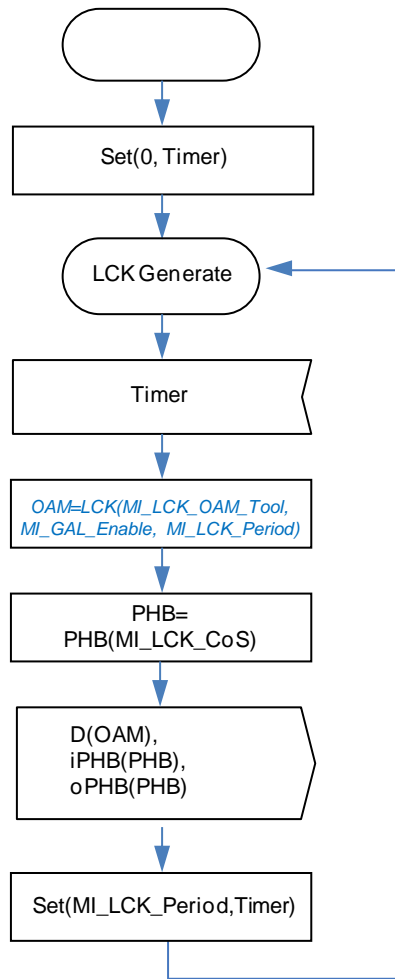
Figure 8-15/G.8121/Y.1381 – LCK Generation behaviour
