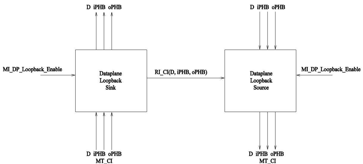
Figure 8-29/G.8121/Y.1381 – Overview of the processes involved with Dataplane Loopback
