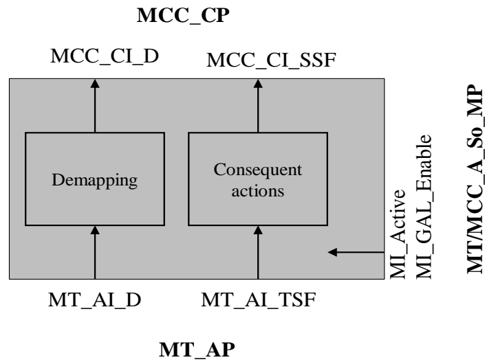
Figure 10-13/G.8121/Y.1382 – MT/MCC_A_Sk processes
