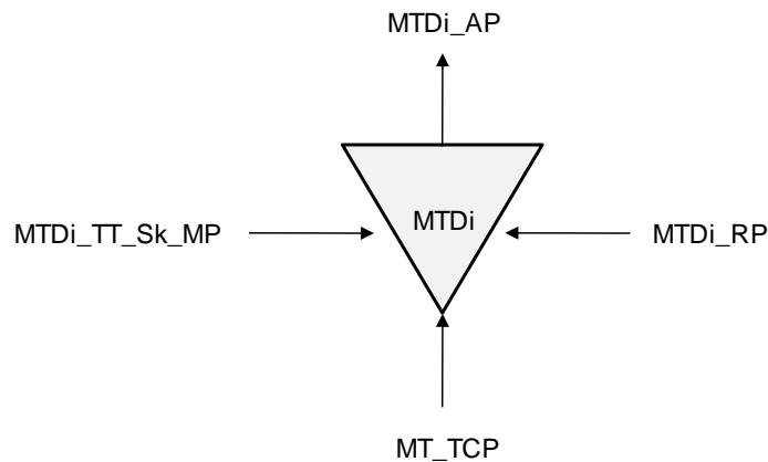
Figure 9-19/G.8121/Y.1381 – MTDi_TT_Sk symbol
