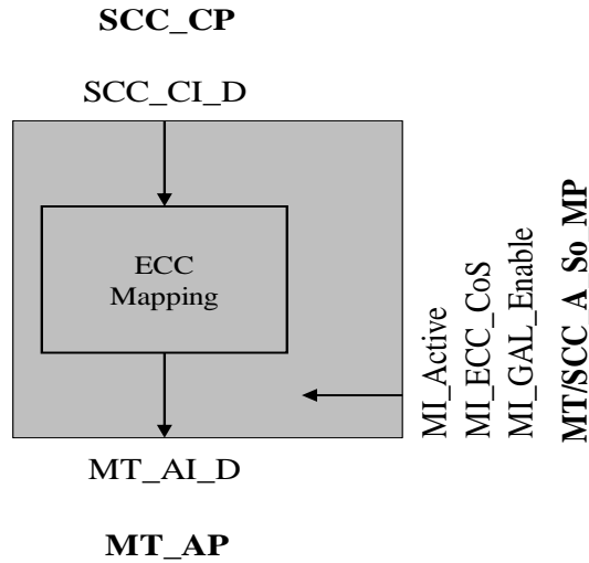
Figure 10-7/G.8121/Y.1382 – MT/SCC_A_So processes
