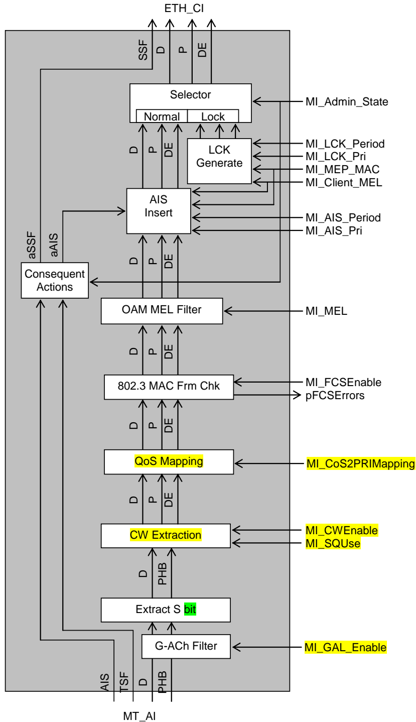
Figure 10-4/G.8121/Y.1381 – MT/ETH_A_Sk process diagram
