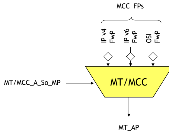
Figure 10-10/G.8121/Y.1382 – MT/MCC_A_So function
