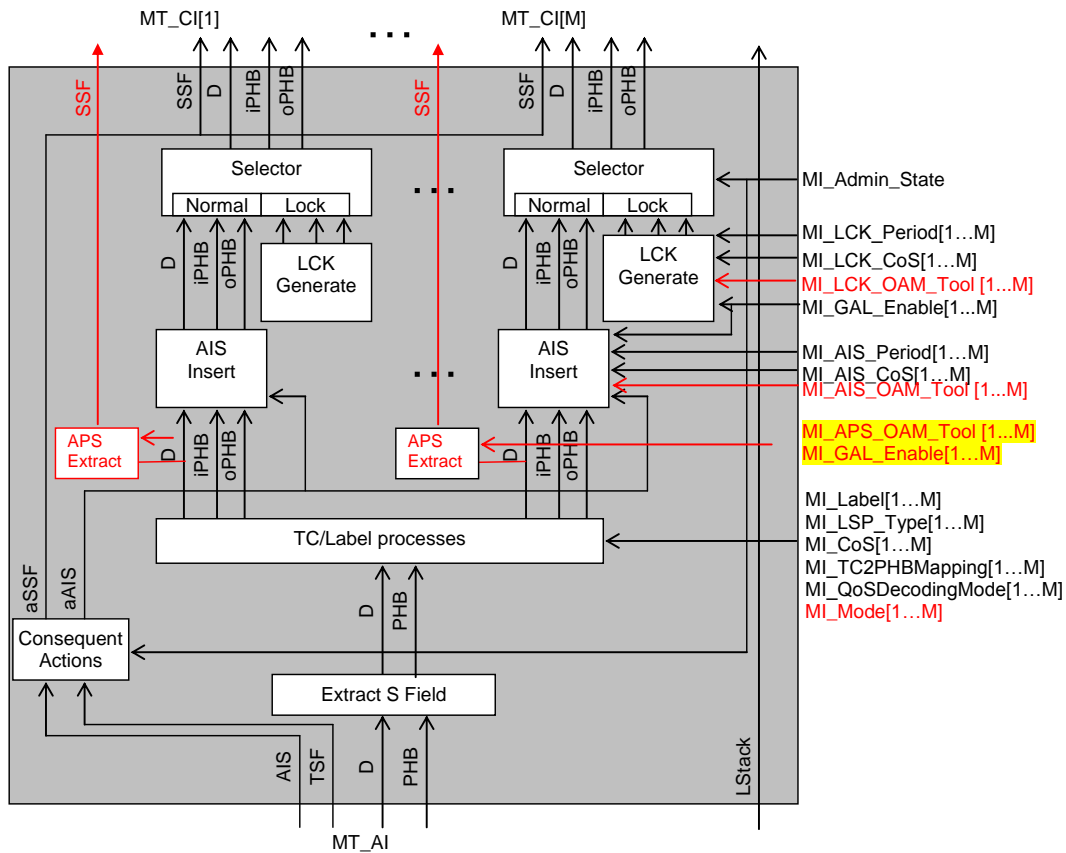
Figure 9-11/G.8121/Y.1381 – MT/MT_A_Sk process diagram
