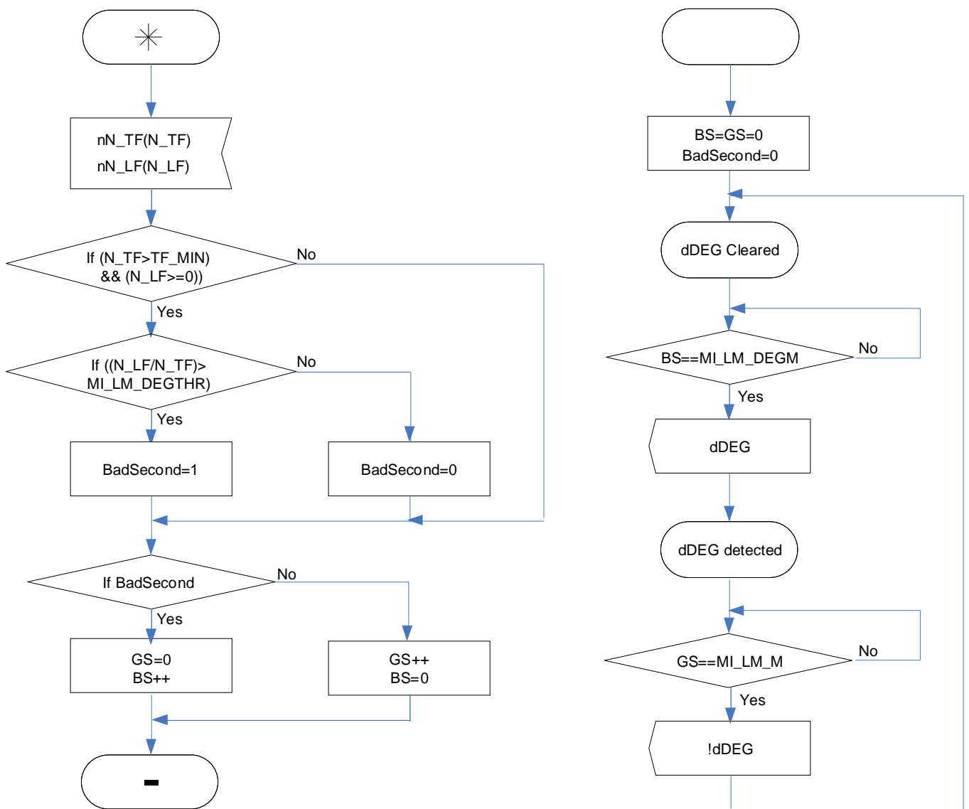
Figure 6-3/G.8121 – dDEG detection and clearance process
