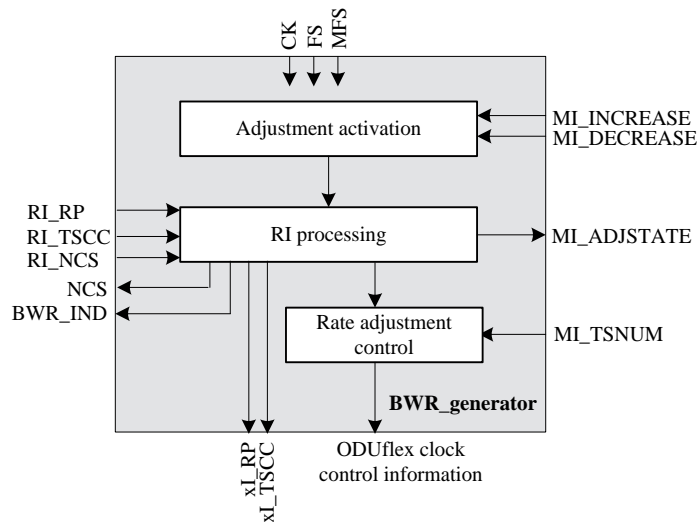
Figure 11-28c – BWR_Generator process
