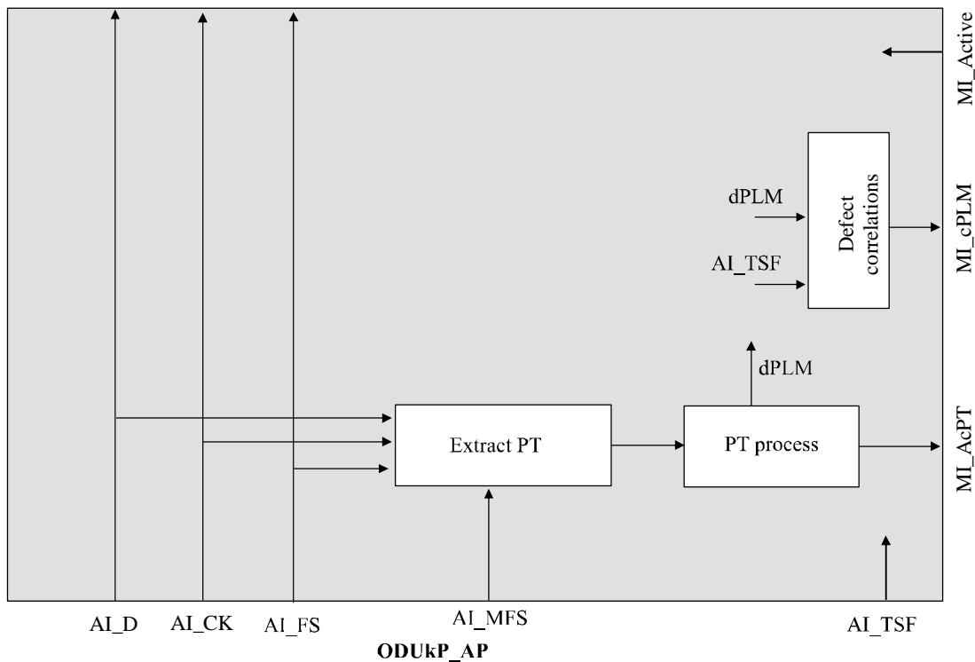
Figure 11-22/G.8121/Y.1381 – ODUkP specific sink processes
