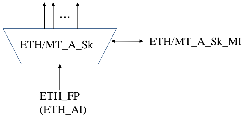
Figure 11-39 – ETH/ETH_A_Sk symbol
