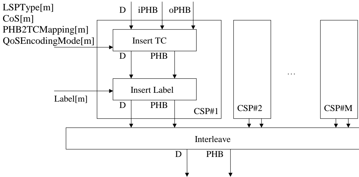
Figure 8-3/G.8121/Y.1381 – TC/Label source processes in Mode 1
