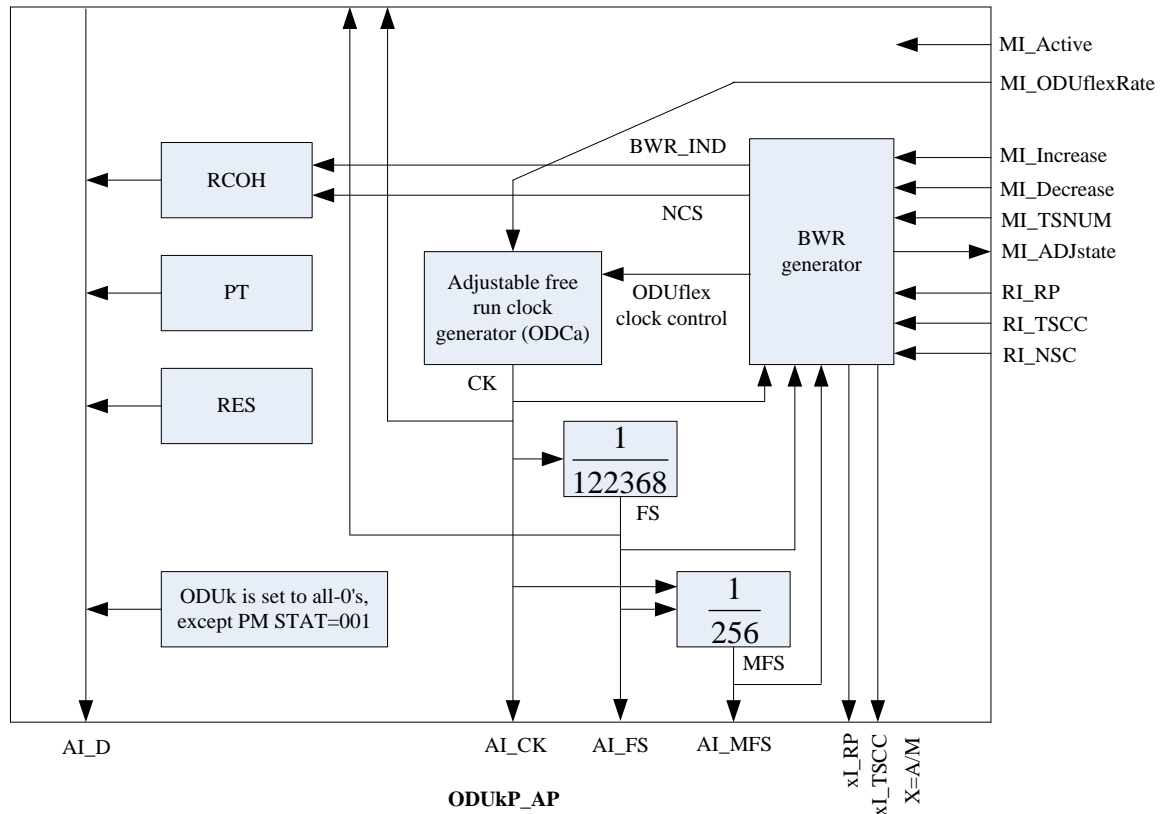
Figure 11-28b/G.8121/Y.1381 – ODUkP (k=flex) specific source processes
