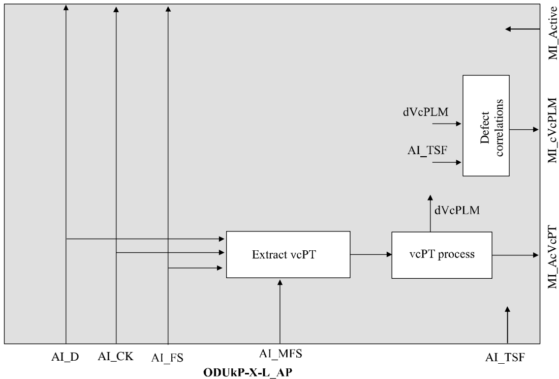
Figure 11-28/G.8121/Y.1341 – ODUkP-X-L specific sink processes
