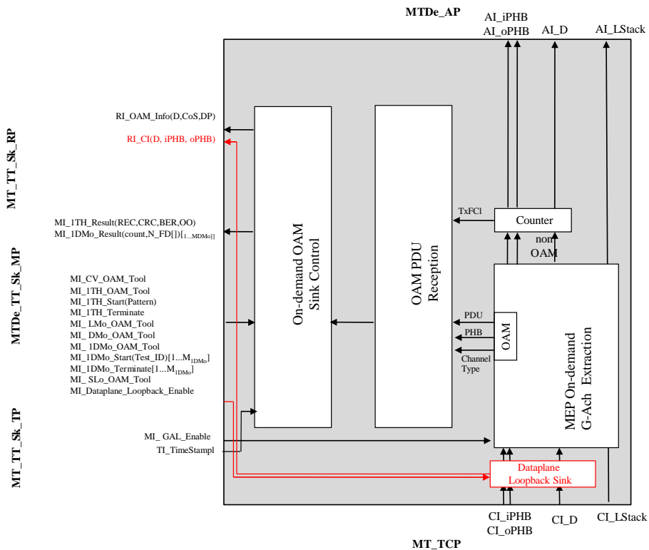
Figure 9-16/G.8121/Y.1381 – MTDe_TT_Sk Process
