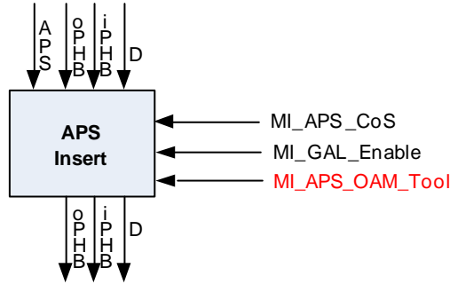
Figure 8-17/G.8121/Y.1381 – APS Insert process
