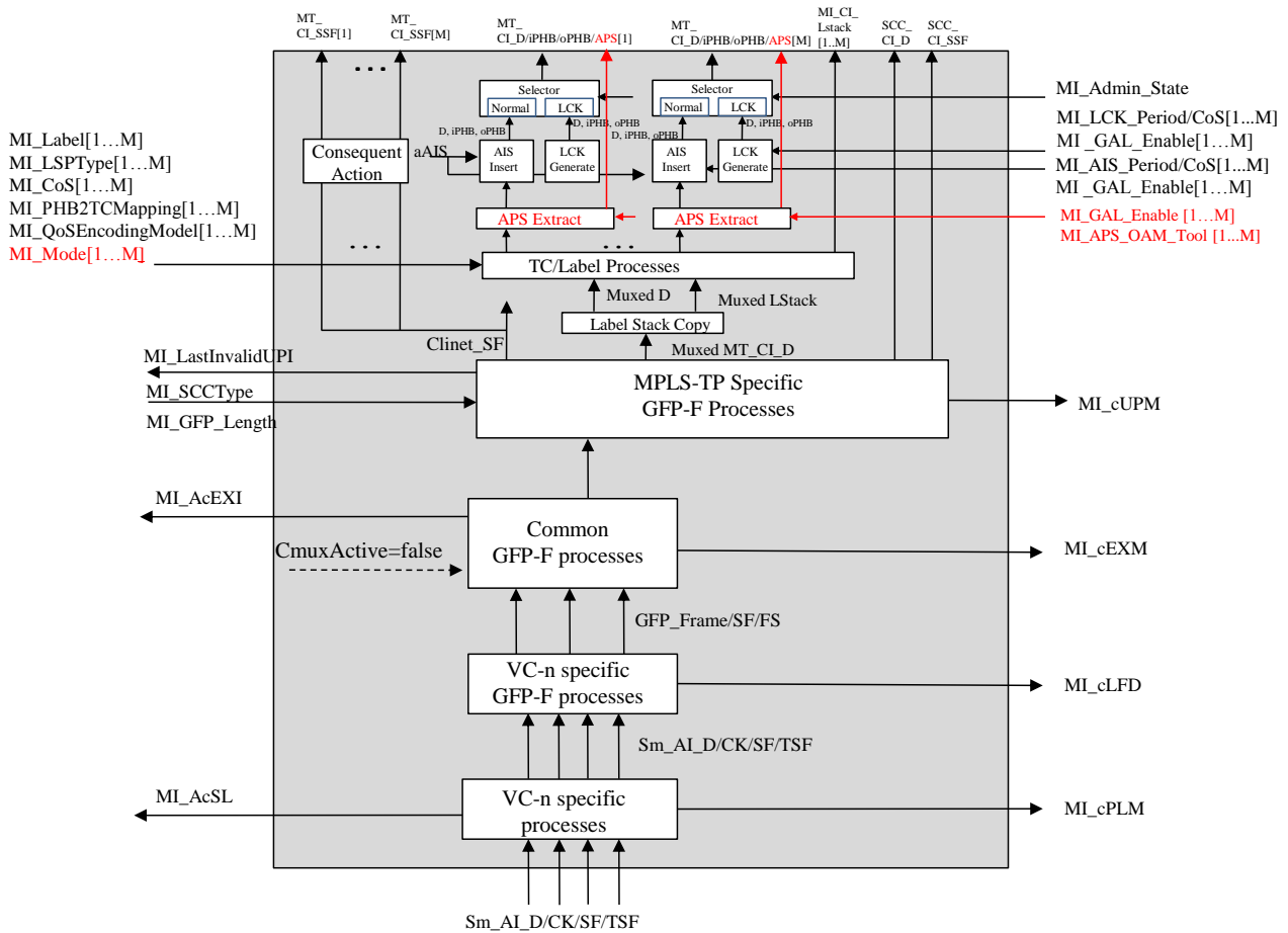
Figure 11-12/G.8121/Y.1381 – Sm/MT_A_Sk process diagram
