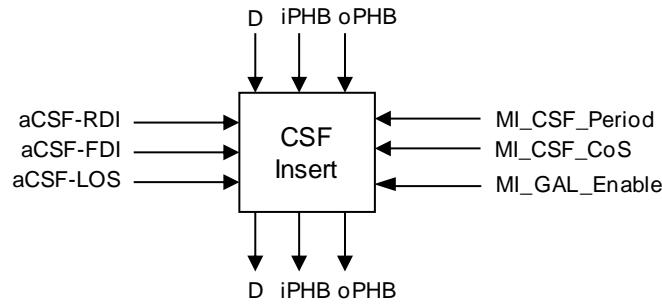
Figure 8-22/G.8121/Y.1381 – CSF Insert process
