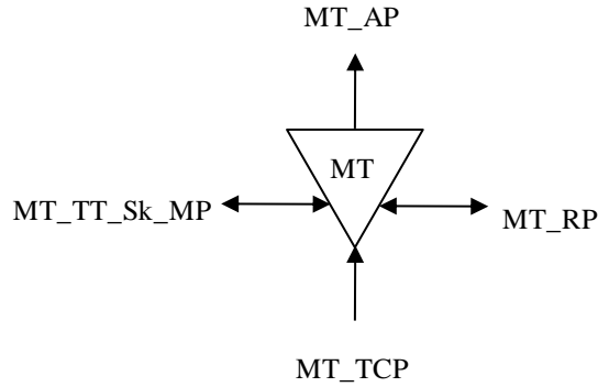
Figure 9-6/G.8121/Y.1381 – MT_TT_Sk function
