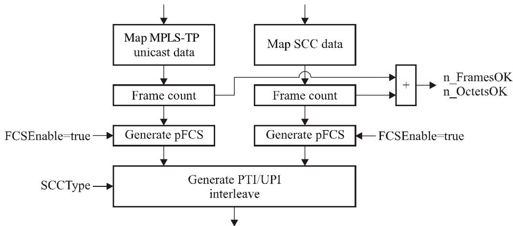
Figure 8-7/G.8121/Y.1381 – MPLS-TP-specific GFP-F source process
