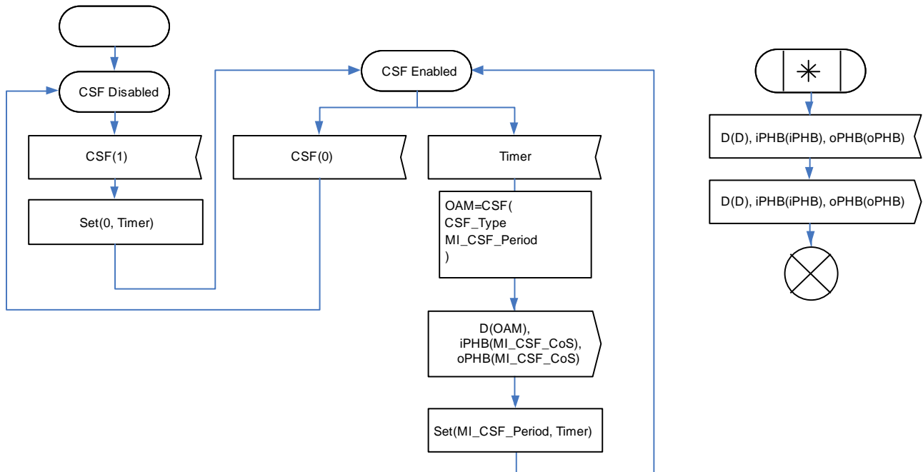
Figure 8-23/G.8121/Y.1381 – CSF Insert behaviour
