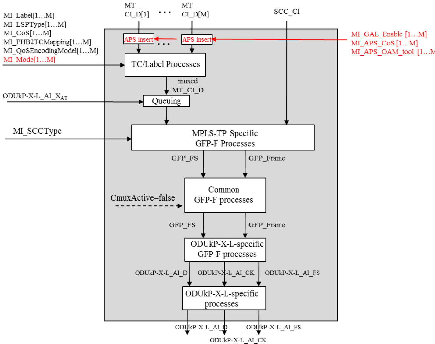
Figure 11-24/G.8121/Y.1381 – ODUkP-X-L/MT_A_So process diagram
