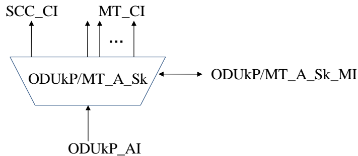
Figure 11-20/G.8121/Y.1381 – ODUkP/MT_A_Sk symbol
