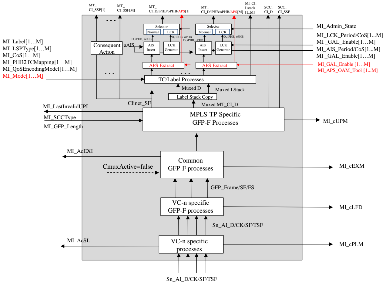
Figure 11-4/G.8121/Y.1381 – Sn/MT_A_Sk process diagram
