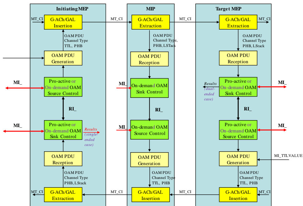
Figure 8-26/G.8121/Y.1381 – Overview of the processes involved with proactive or on-demand OAM functions
