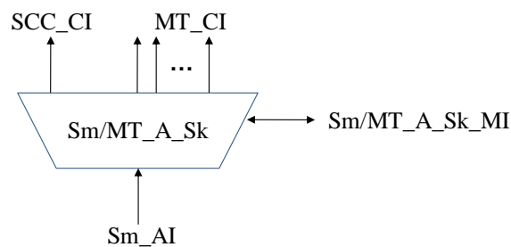
Figure 11-11/G.8121/Y.1381 – Sm/MT_A_Sk symbol
