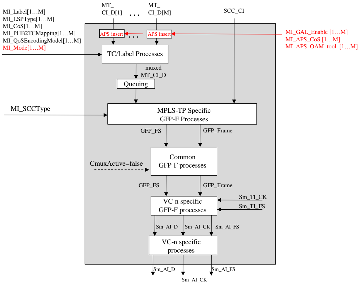
Figure 11-10/G.8121/Y.1381 – Sm/MT_A_So process diagram
