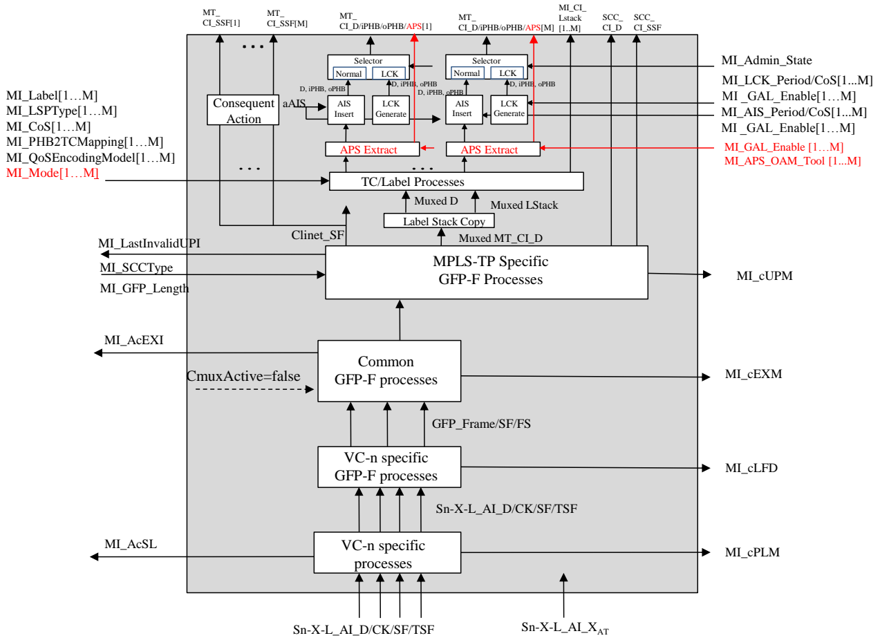
Figure 11-8/G.8121/Y.1381 – Sn-X-L/MT_A_Sk process diagram
