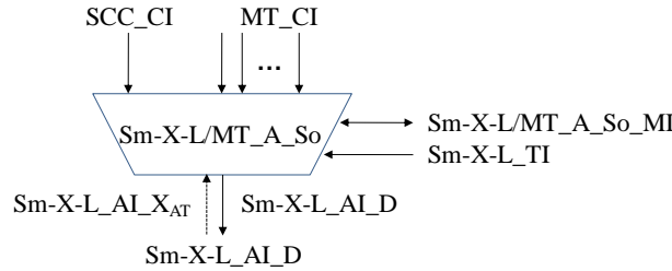
Figure 11-13/G.8121/Y.1381 – Sm-X-L/MT_A_So symbol
