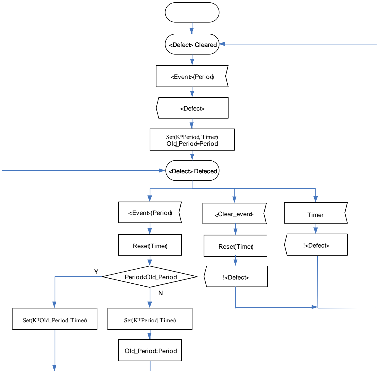
Figure 6-2/G.8021/Y.1341 – Defect detection and clearance process for dMMG, dUNM, dUNP, dUNC, dAIS, dLCK and dCSF
