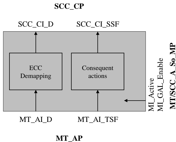
Figure 10-9/G.8121/Y.1382 – MT/SCC_A_Sk processes
