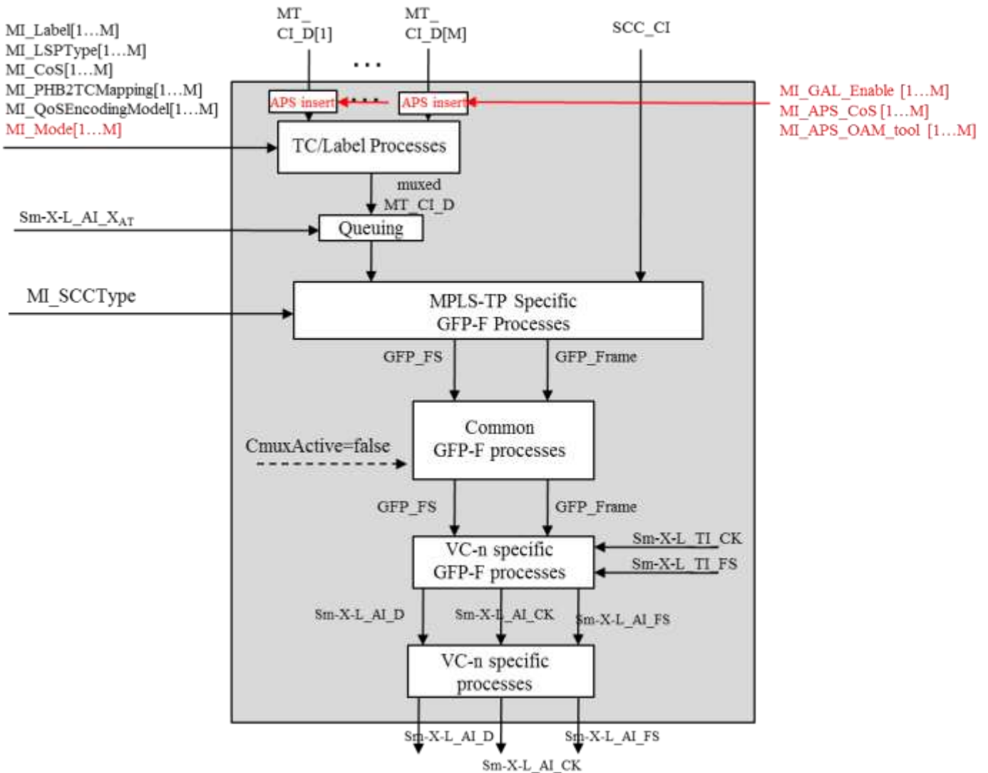
Figure 11-14/G.8121/Y.1381 – Sm-X-L/MT_A_So process diagram
