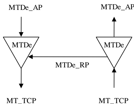
Figure 9-12/G.8121/Y.1381 – MTDe_TT
