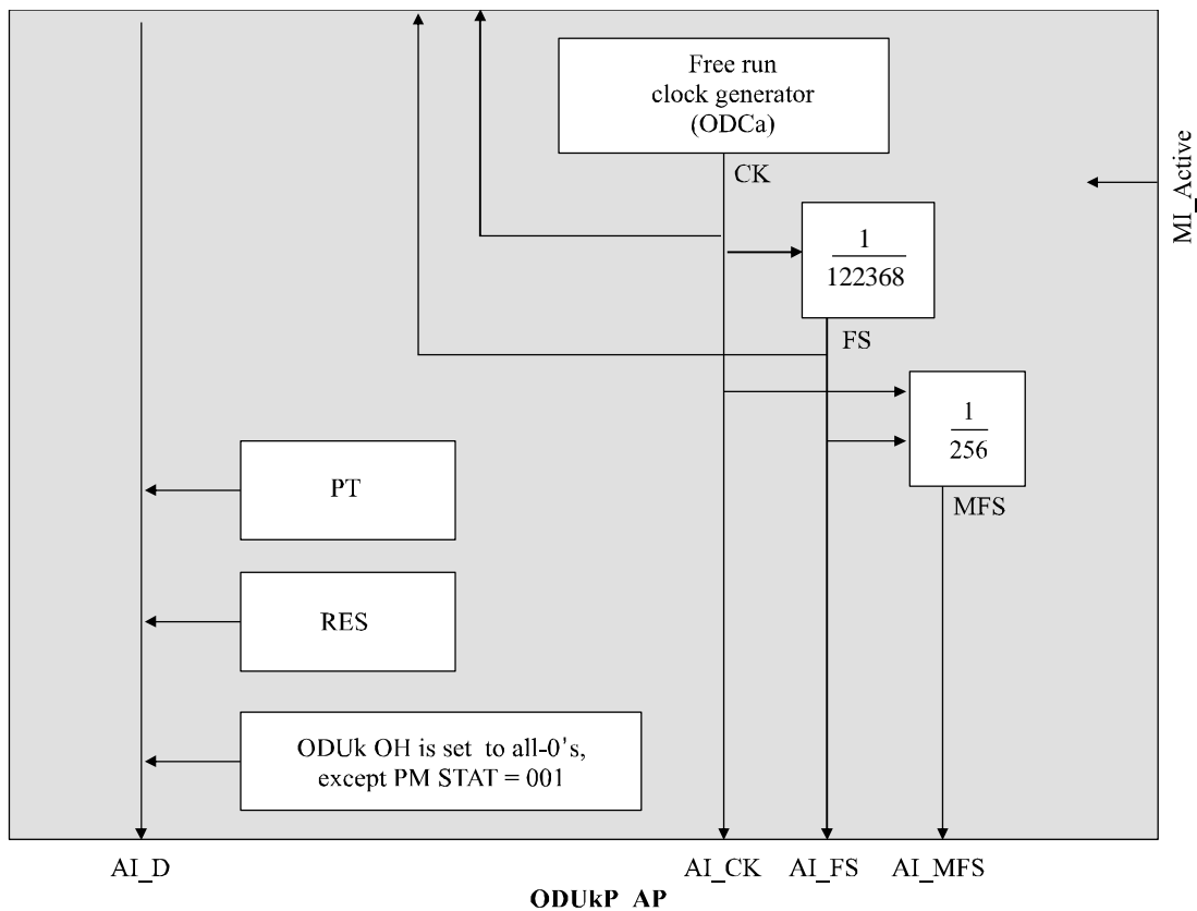
Figure 11-19/G.8121/Y.1381 – ODUkP specific source processes
