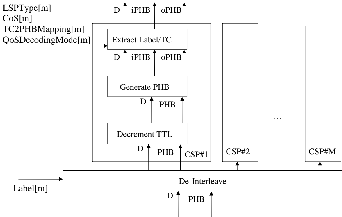
Figure 8-4/G.8121/Y.1381 – TC/Label sink processes in Mode 1
