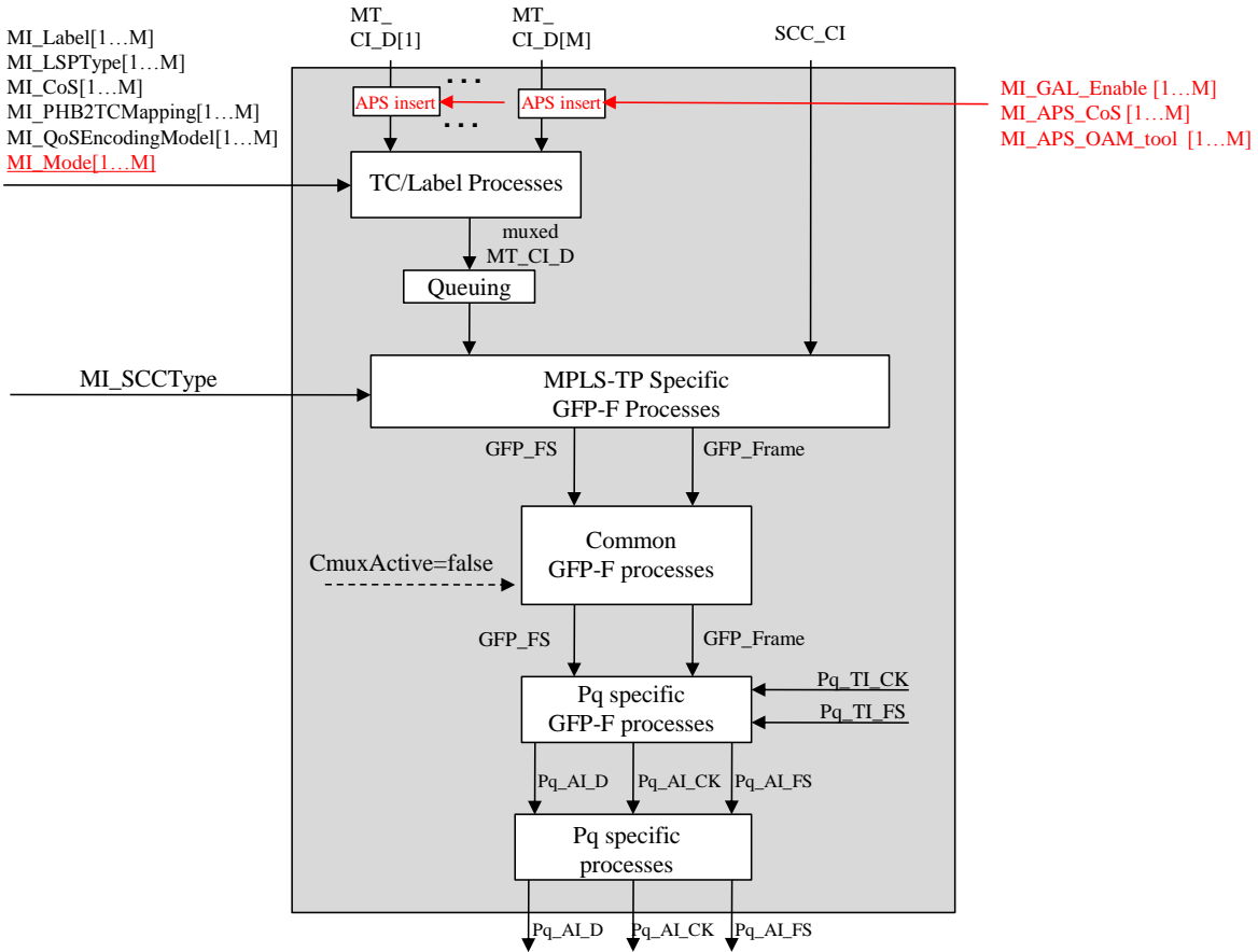
Figure 11-30/G.8121/Y.1381 – Pq/MT_A_So process diagram
