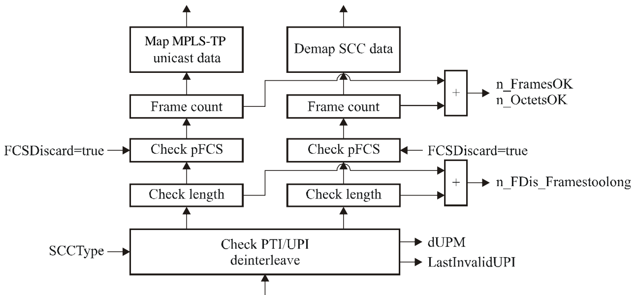
Figure8-8/G.8121/Y.1381 – MPLS-TP-specific GFP-F sink process
