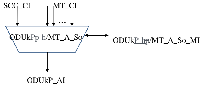
Figure 11-28a/G.8121/Y.1381 – ODUkP-h/MT_A_So symbol
