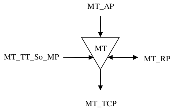
Figure 9-4/G.8121/Y.1381 –MT_TT_So function
