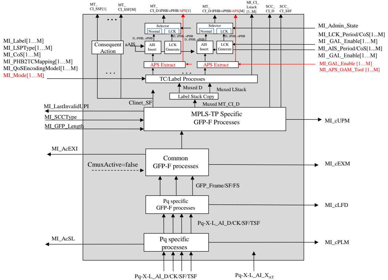
Figure 11-36/G.8121/Y.1381 – Pq-X-L/MT_A_Sk process diagram
