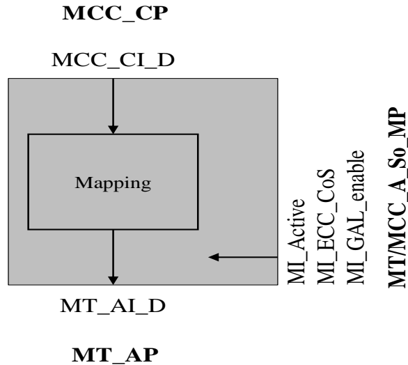
Figure 10-11/G.8121/Y.1382 – MT/MCC_A_So processes
