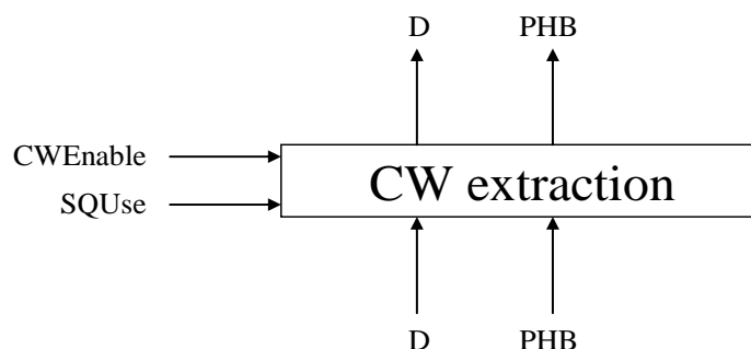
Figure 8-10/G.8121/Y.1381 – CW extraction process
