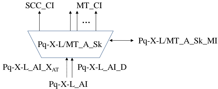
Figure 11-35/G.8121/Y.1381 – Pq-X-L/MT_A_Sk symbol
