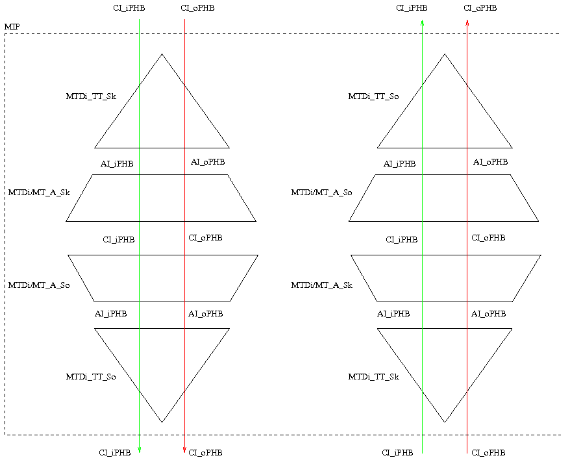
Figure I.2 – Flow of PHB information through a MIP
