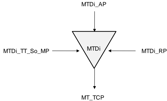
Figure 9-17/G.8121/Y.1381 – MTDi_TT_So symbol
