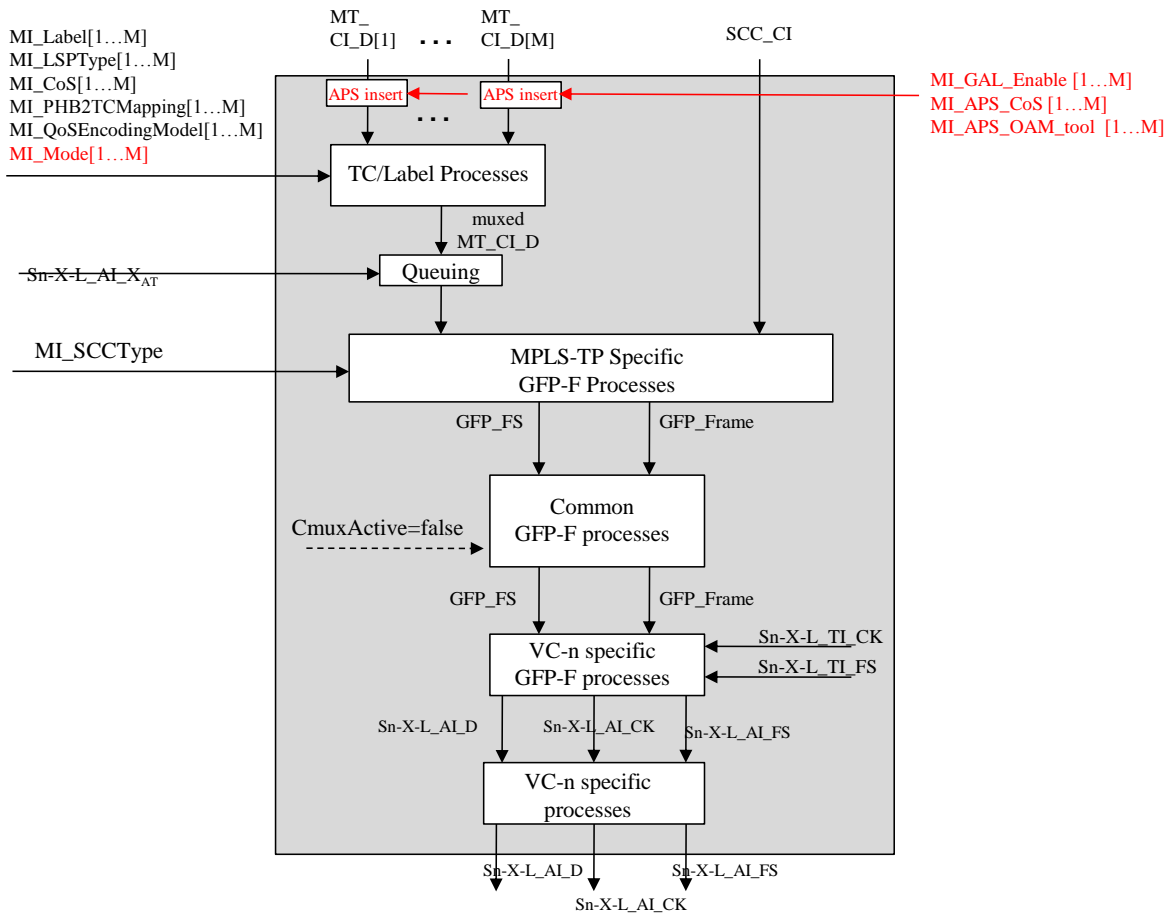
Figure 11-6/G.8121/Y.1381 – Sn-X-L/MT_A_So process diagram
