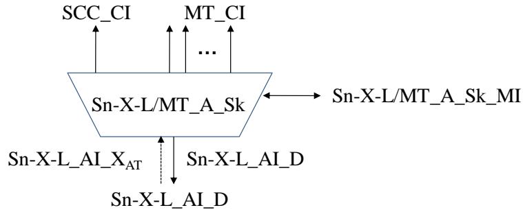
Figure 11-7/G.8121/Y.1381 – Sn-X-L/MT_A_Sk symbol
