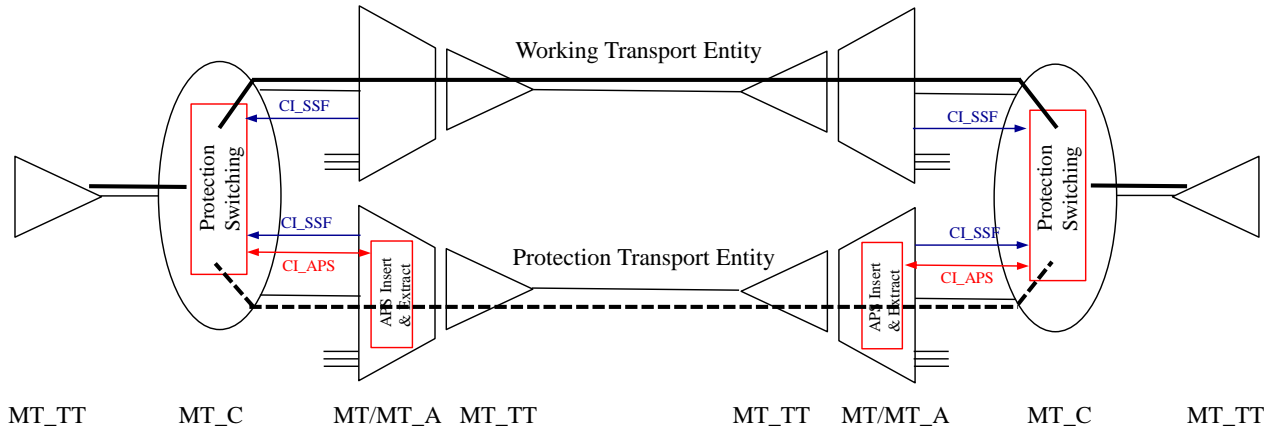
Figure III-2/G.8121/Y.1381 – MPLS-TP SNC/S protection switching architecture
