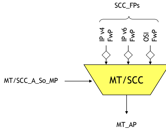
Figure 10-6/G.8121/Y.1382 – MT/SCC_A_So function
