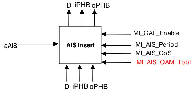
Figure 8-13/G.8121/Y.1381 – AIS Insert process
