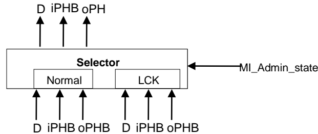
Figure 8-11/G.8121/Y.1381 – Selector process
