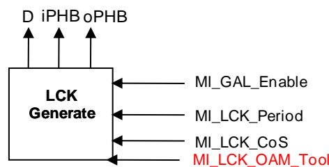
Figure 8-14/G.8121/Y.1381 – LCK Generation process
