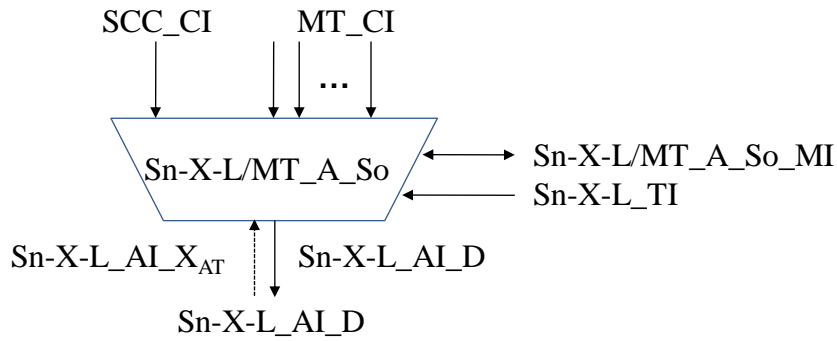
Figure 11-5/G.8121/Y.1381 – Sn-X-L/MT_A_So symbol
