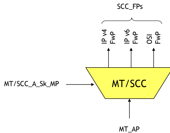
Figure 10-8/G.8121/Y.1382 – MT/SCC_A_Sk function
