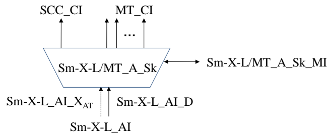
Figure 11-15/G.8121/Y.1381 – Sm-X-L/MT_A_Sk symbol
