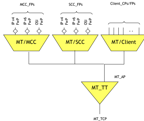
Figure 10-5/G.8121/Y.1382 – MT/SCC_A function, MT/MCC_A function, and MT/client_A function
