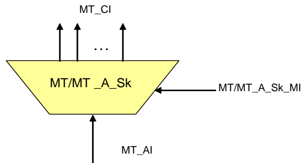
Figure 9-10/G.8121/Y.1381 – MT/MT_A_Sk function
