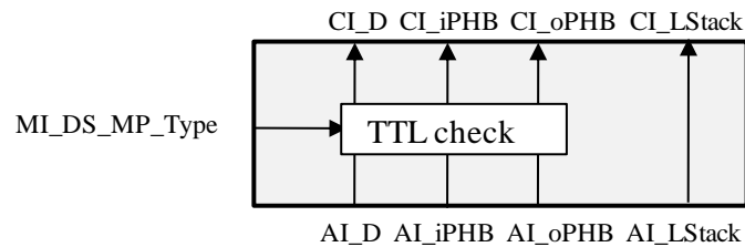
Figure 9-24/G.8121/Y.1381 – MTDi/MT_A_Sk Process
