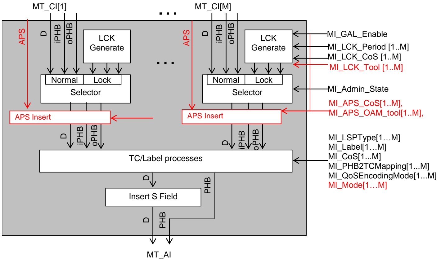
Figure 9-9/G.8121/Y.1381 – MT/MT_A_So process diagram
