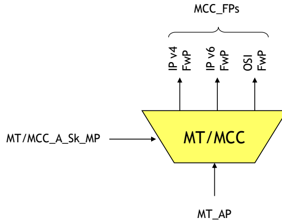
Figure 10-12/G.8121/Y.1382 – MT/MCC_A_Sk function
