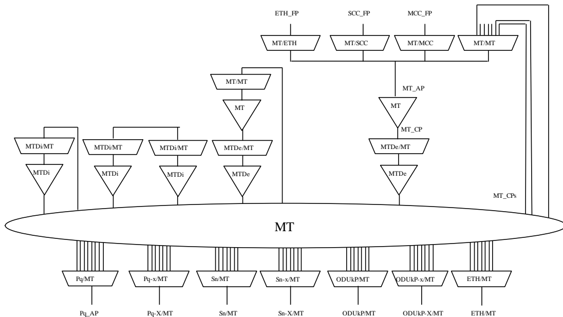
Figure 9-0/G.8121/Y.1381 – MPLS-TP atomic functions
