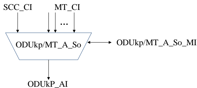
Figure 11-17/G.8121/Y.1381 – ODU k P/MT_A_So symbol
