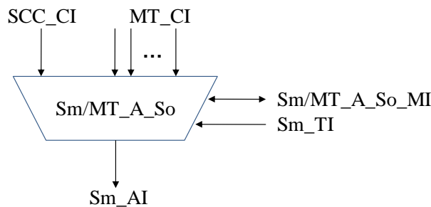
Figure 11-9/G.8121/Y.1381 – Sm/MT_A_So symbol
