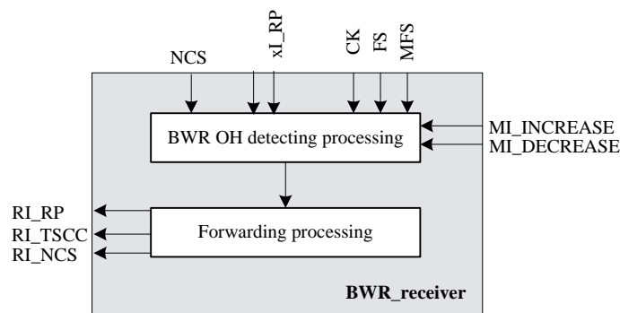
Figure 11-28f – BWR_Receiver process
