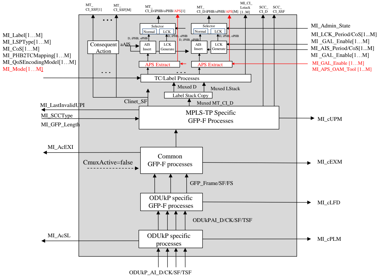
Figure 11-21/G.8121/Y.1381 – ODUkP/MT_A_Sk process diagram
