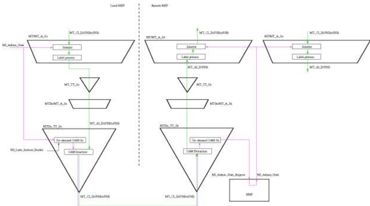
Figure 8-27/G.8121/Y.1381 – Overview of the processes involved with Lock Instruct
