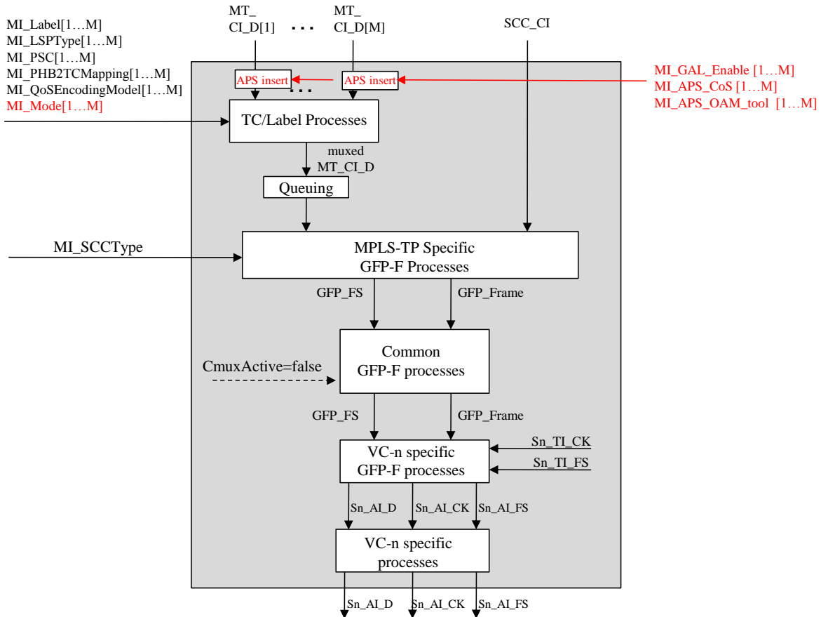
Figure 11-2/G.8121/Y.1381 – Sn/MT_A_So process diagram
