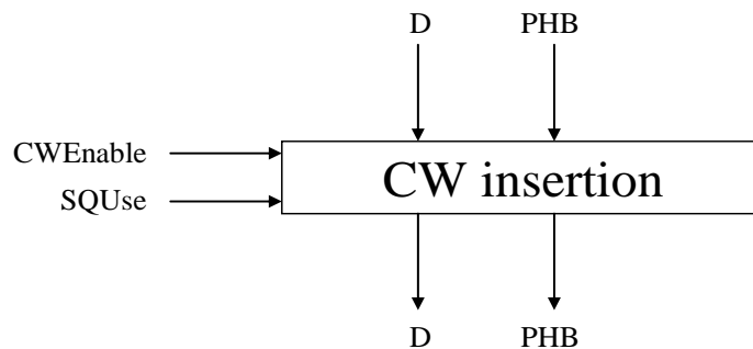
Figure 8-9/G.8121/Y.1381 – CW insertion process
