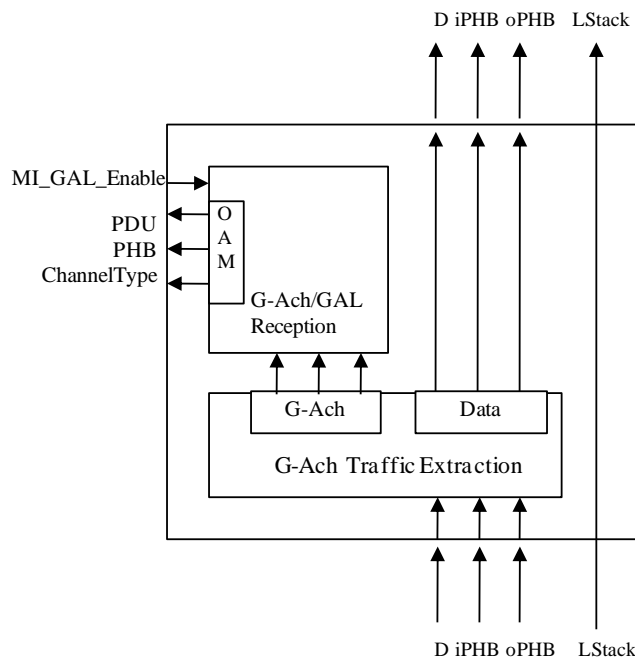
Figure 8-2/G.8121/Y.1381 – G-ACh Reception Process
