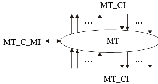
Figure 9-1/G.8121/Y.1381 – MT_C symbol
