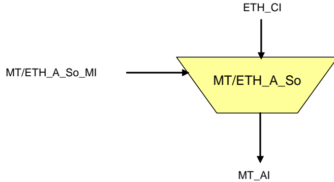
Figure 10-1/G.8121/Y.1381 – MT/ETH_A_So function
