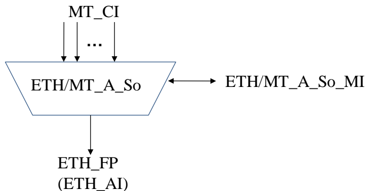
Figure 11-37 – ETH/MT_A_So symbol
