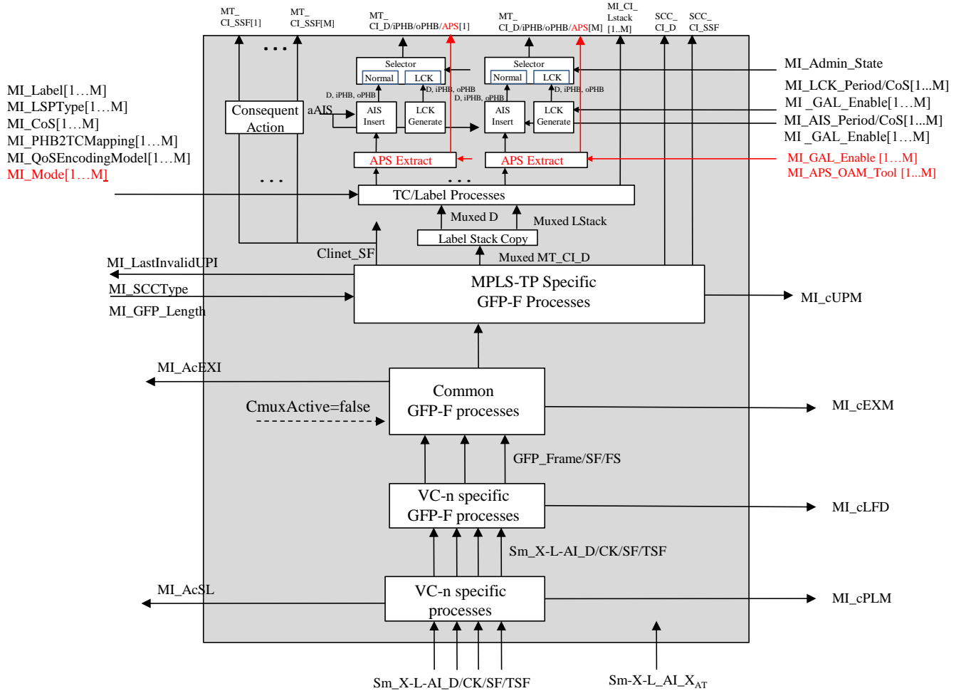
Figure 11-16/G.8121/Y.1381 – Sm-X-L/MT_A_Sk process diagram
