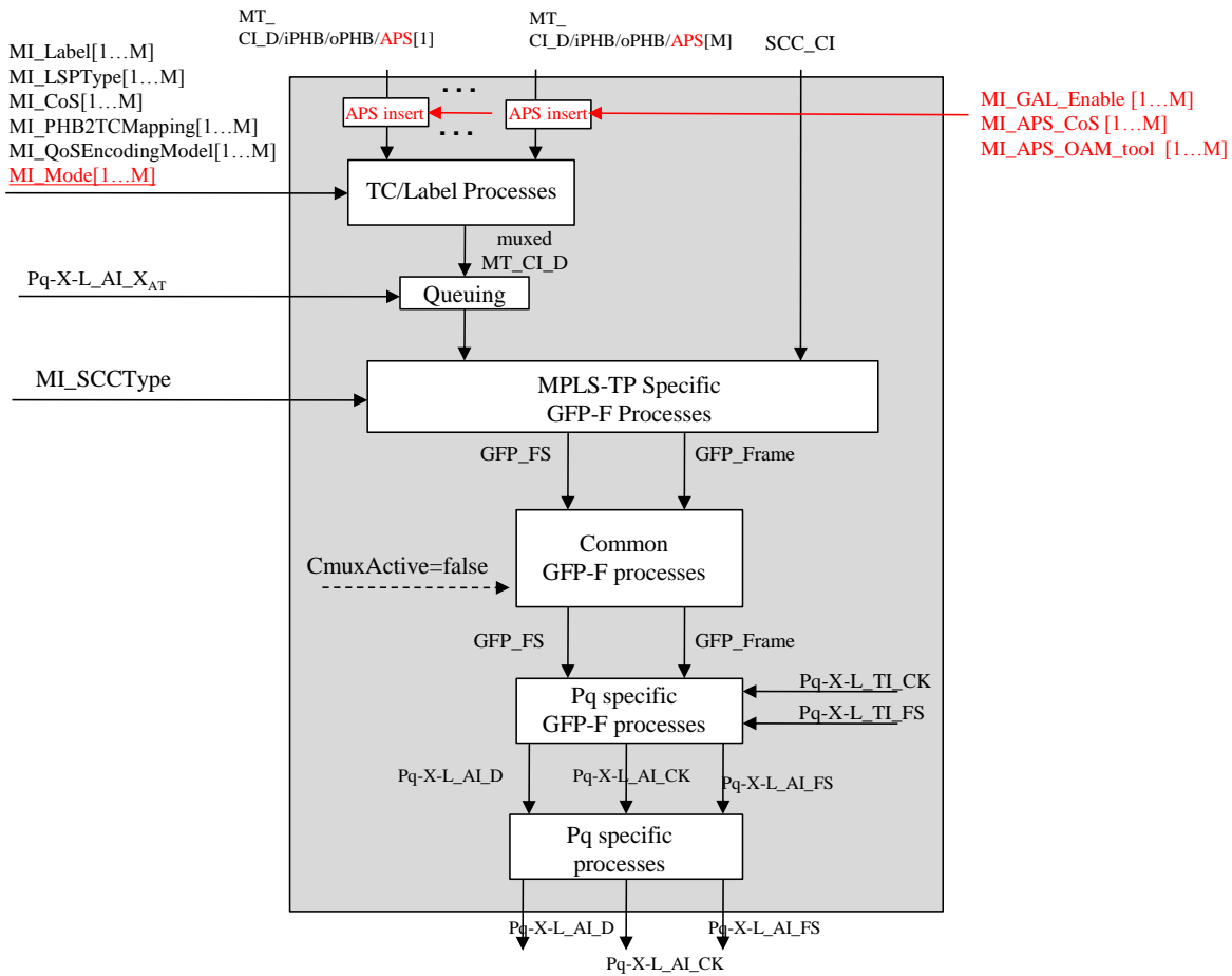
Figure 11-34/G.8121/Y.1381 – Pq-X-L/MT_A_So process diagram
