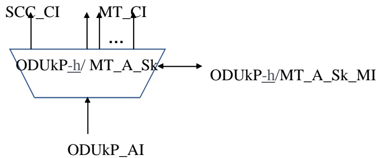
Figure 11-28d/G.8121/Y.1381 – ODUkP-h/MT_A_Sk symbol
