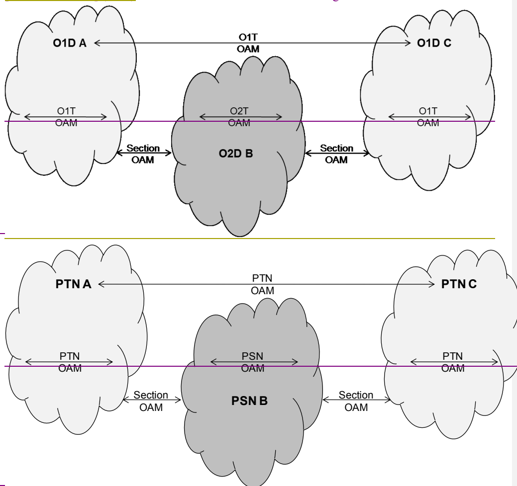
Figure B.1 Interconnection case 1) PTN O1T client over a PSN O2T server
