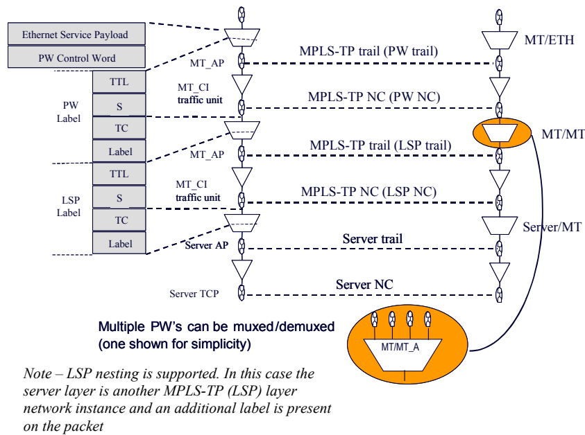
Figure 6-5 – MPLS-TP layer network structure example
