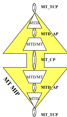
Figure 8-4 – MPLS-TP MIP compound function
