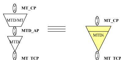
Figure 8-5 – MPLS-TP half MIP compound function
