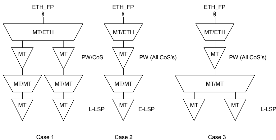
Figure 6-6 – Examples of QoS processing in MT/Client_A function
