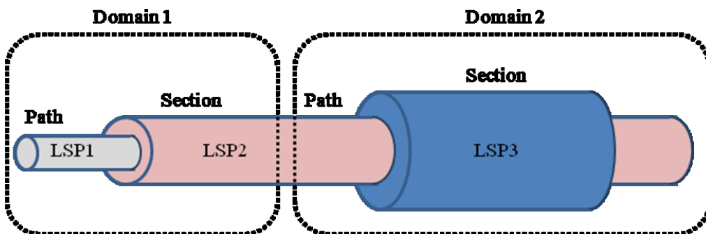
Figure 6-1 – MPLS-TP roles and layers
