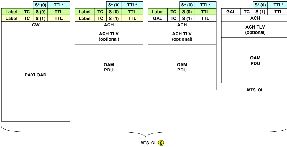
Figure I-6 – MPLS-TP network adapted and characteristic information traffic units (Reference point 6)
