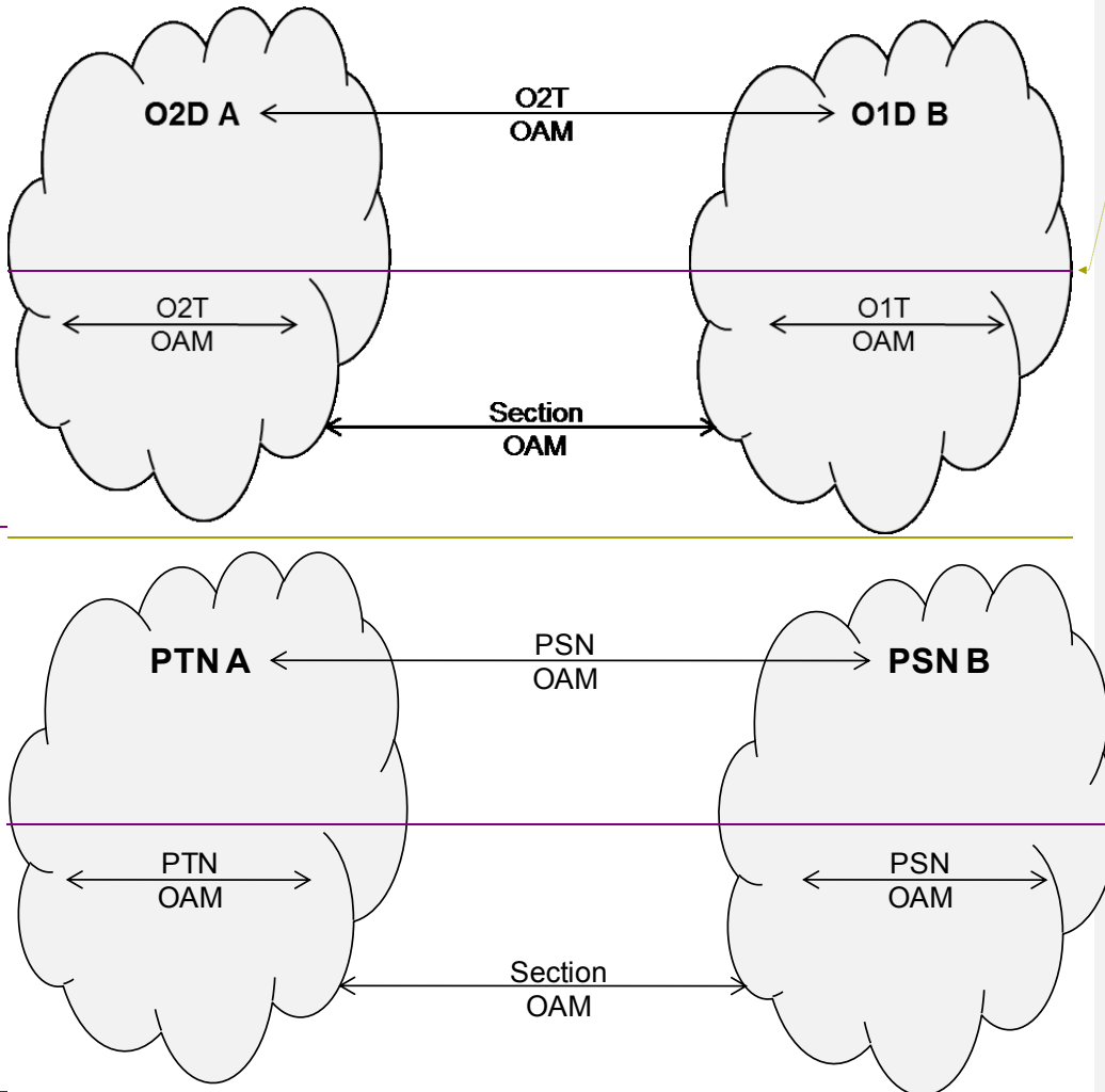
Figure B.5 Interconnection case 3) PTN O2D to PSN O1D
