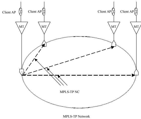
Figure 6-7 – Point-to-multipoint MPLS-TP connection
