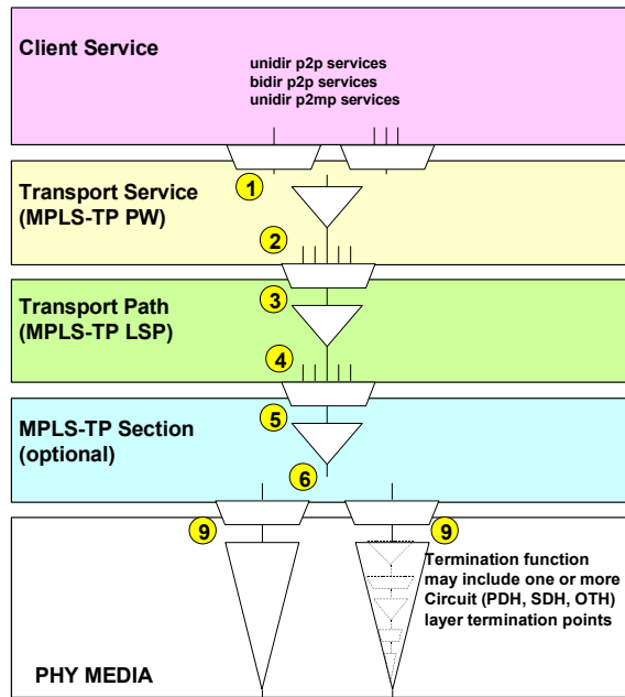
Figure I-1 – MPLS-TP network architecture (layer view) example
