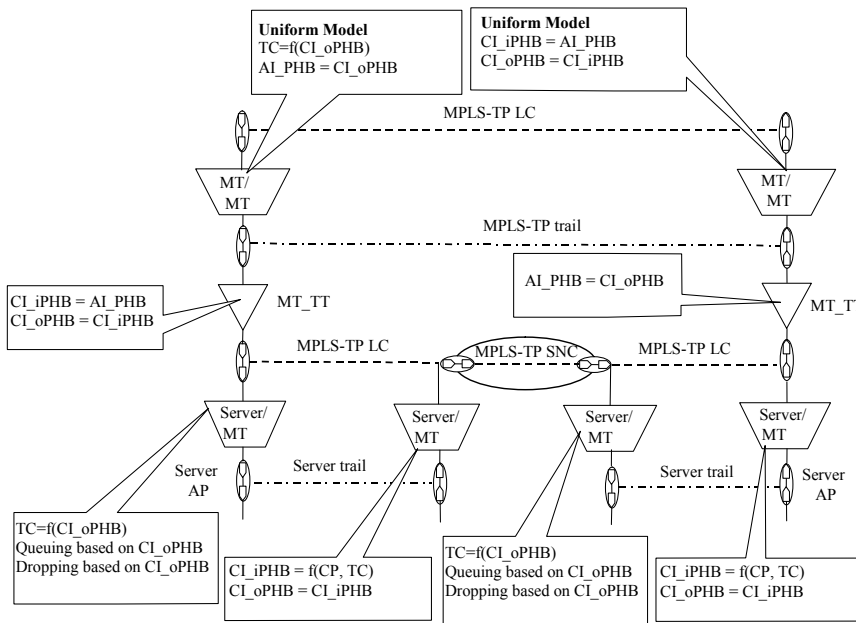
Figure 10-2 – Reference diagram for the uniform model
