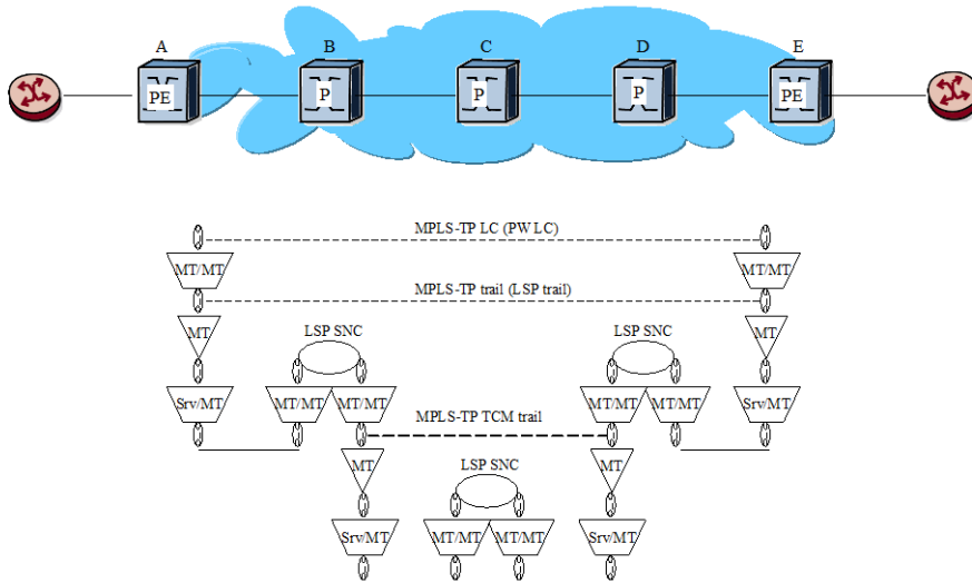
Figure 8-3 – MPLS-TP TCM Example
