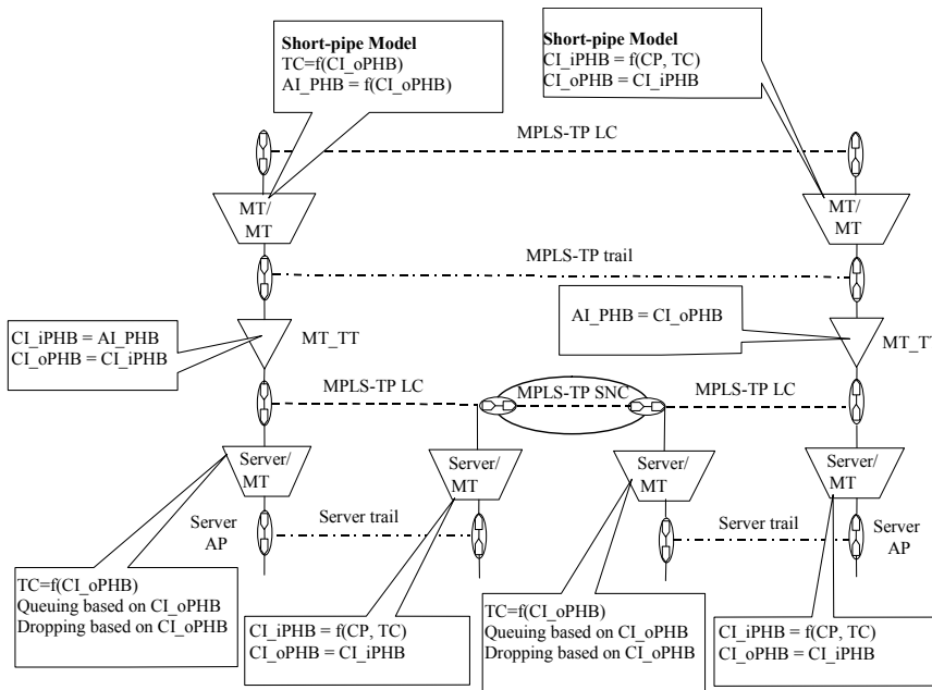
Figure 10-1 – Reference diagram for the short-pipe model
