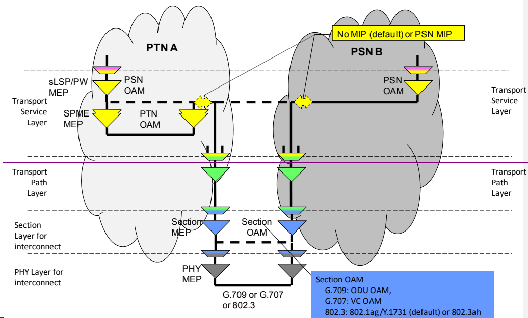
Figure B.6 Interconnection case 3) PTN O2D to PSN O1D
