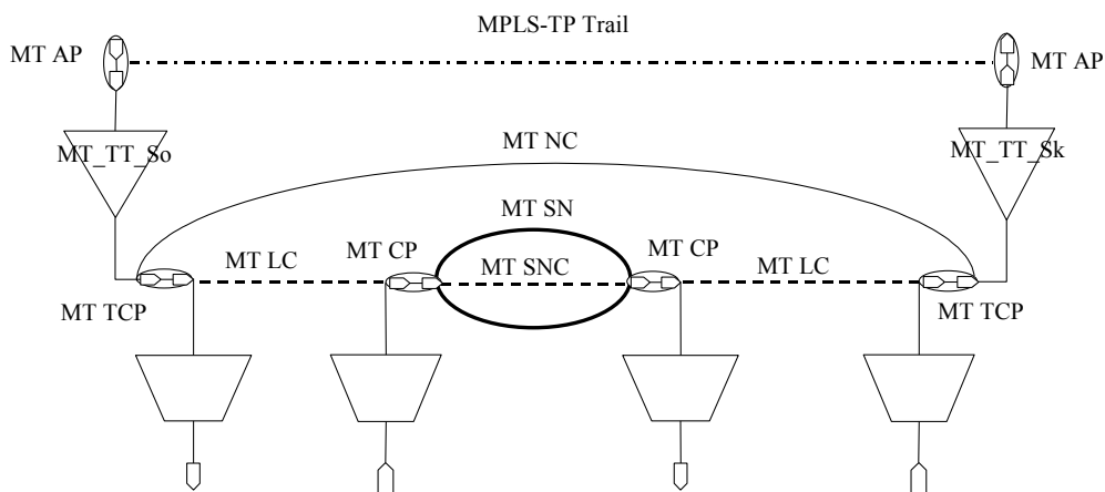
Figure 6-4 – MPLS-TP layer network example
