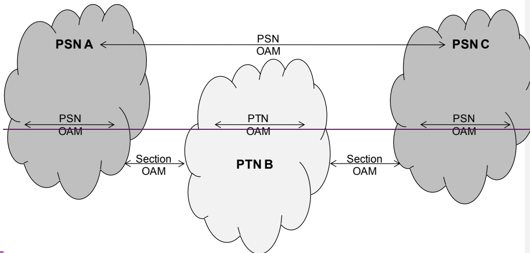
Figure B.3 Interconnection case 2) PSN O2T client over an PTN O1T server
