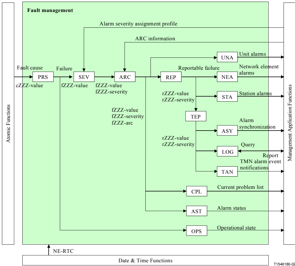
Figure 7-1/G.8151/Y.1374– Fault management within the T-MPLS-TP NEF
