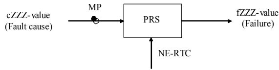
Figure 7-2/G.8151/Y.1374– Fault Cause Persistency function
