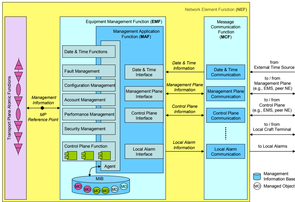
Figure 6.4/G.8151/Y.1374 – T-MPLS-TP Equipment Management Function
