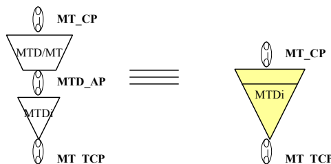
Figure 8-5 – MPLS-TP half MIP compound function
