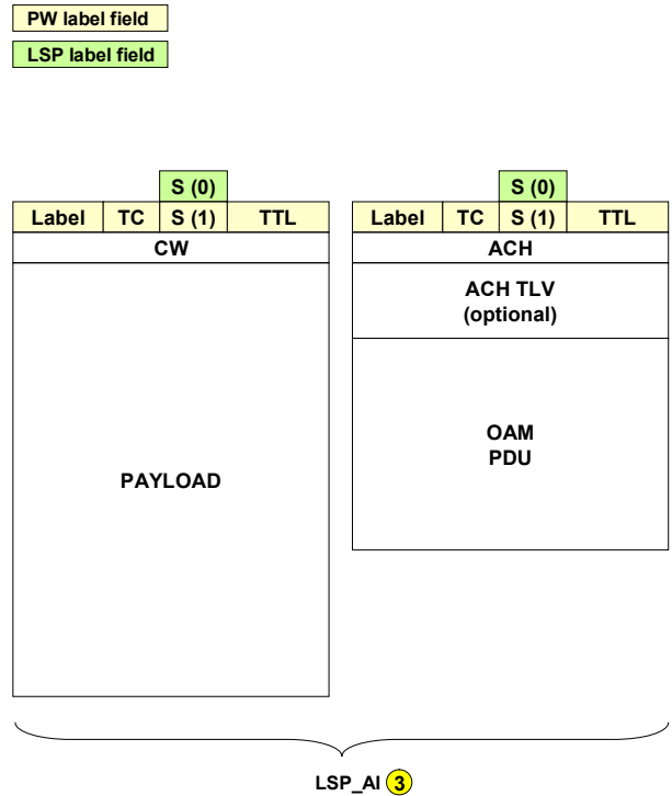
Figure I-3 – MPLS-TP network adapted and characteristic information traffic units (Reference point 3)
