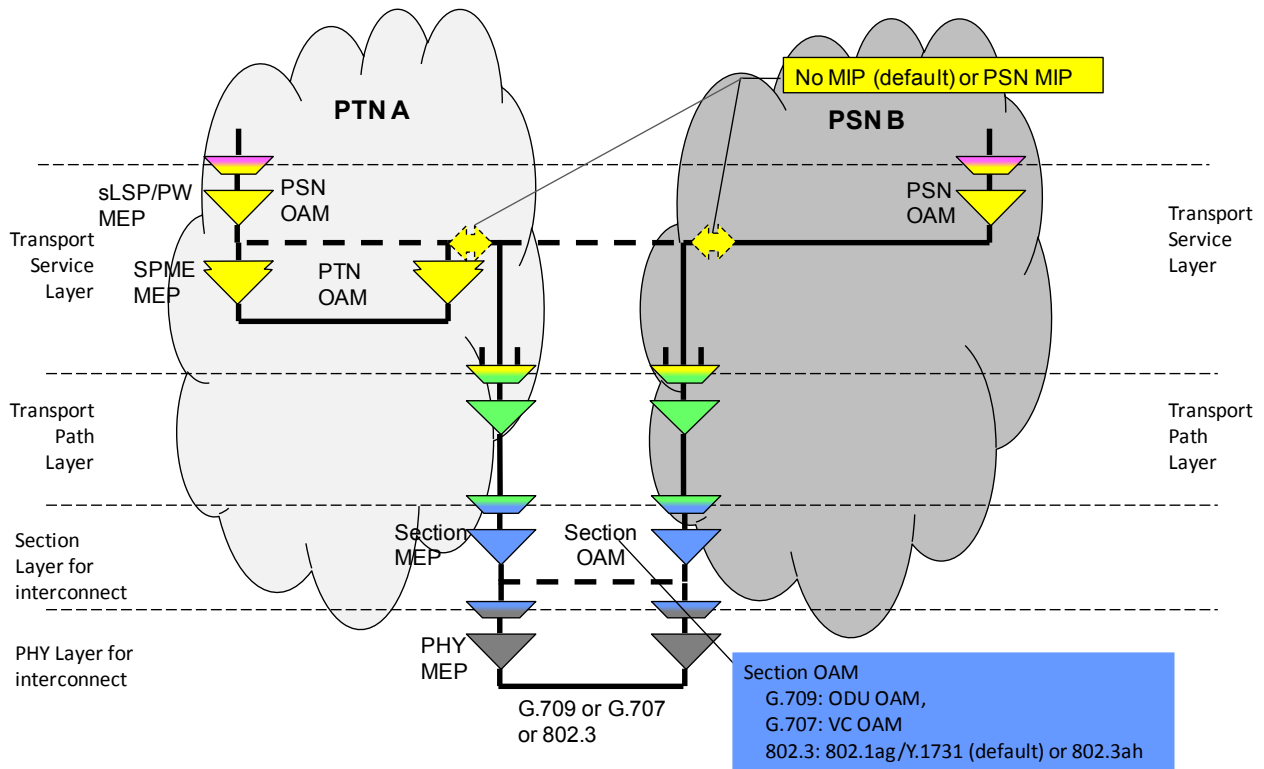
Figure B.6 Interconnection case 3) PTN to PSN
