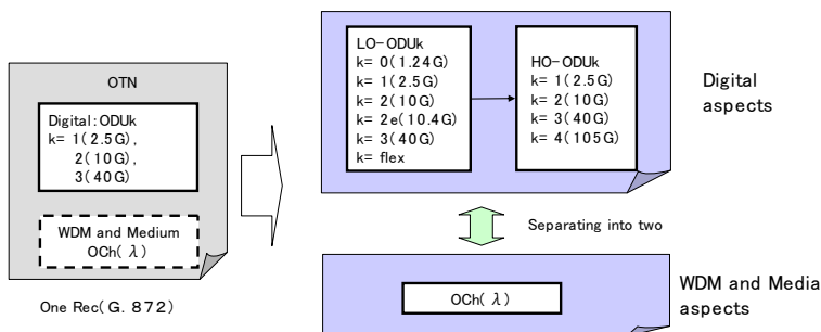
Figure 5-2: Direction of OTN evolution
