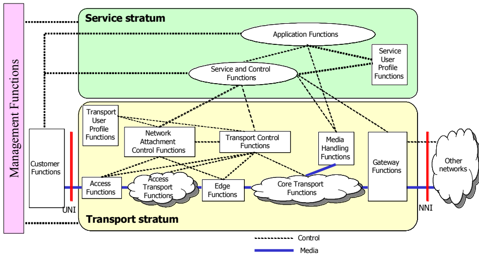
Figure 5-3 NGN architecture overview
