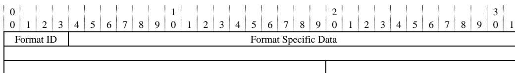
Figure 3/G.7714.1/Y.1705.1 – General Discovery Message format
