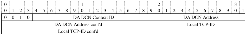
Figure 5/G.7714.1/Y.1705.1 – DA DCN Address Message format
