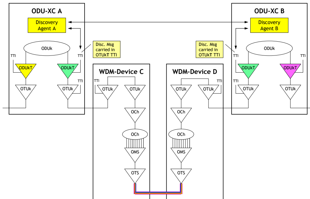
Figure VI.7/G.7714.1/Y.1705.1- Example of ODUkT TTI (SAPI sub-field)-based LAD for OTN with WDM equipment
