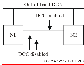
Figure VI.6/G.7714.1/Y.1705.1 – Central Office with DCC enabled on only one link or using an out-of-band DCN
