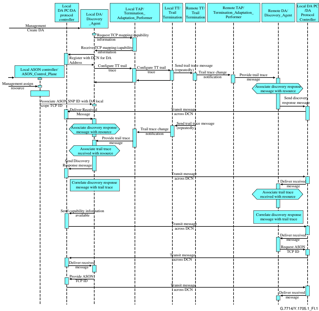
Figure I.1/G.7714.1/Y.1705.1 – Sequence diagram
