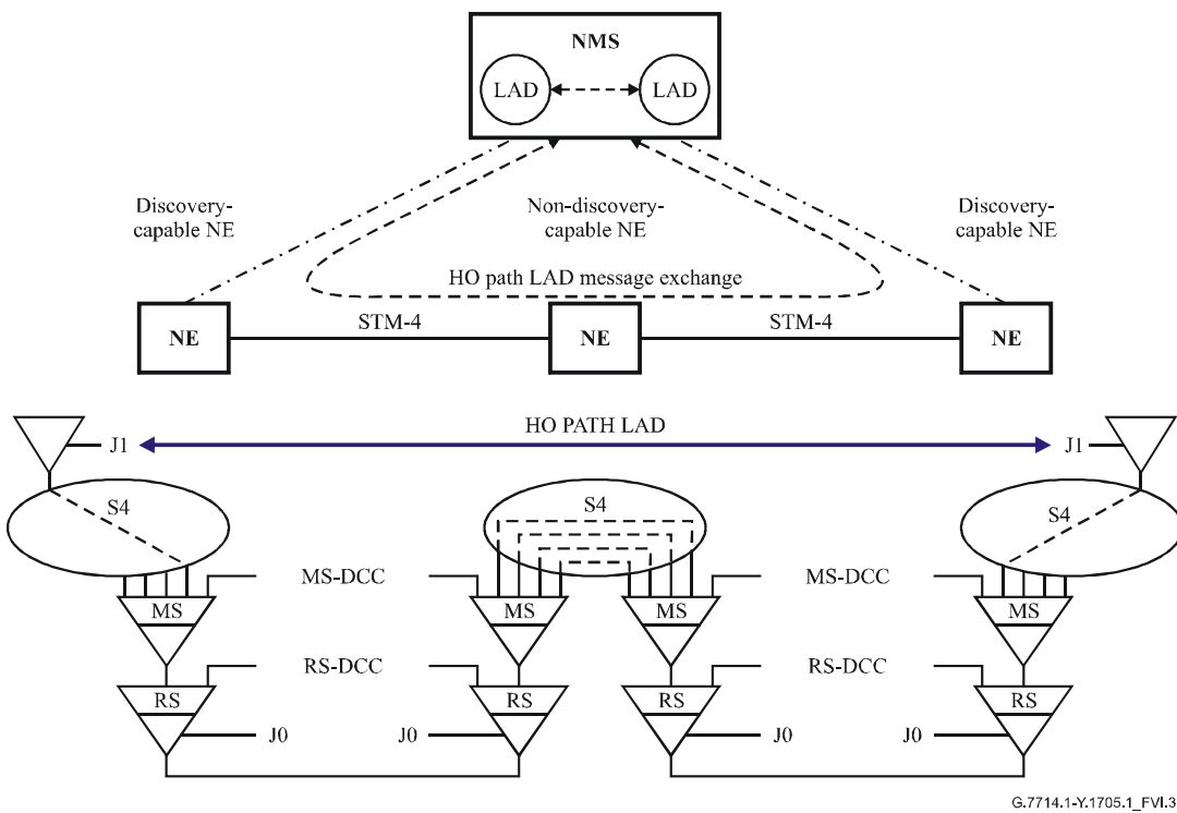
Figure VI.3/G.7714.1/Y.1705.1 – Immediate discovery-capable neighbours at HO path layer – LAD done by NMS
