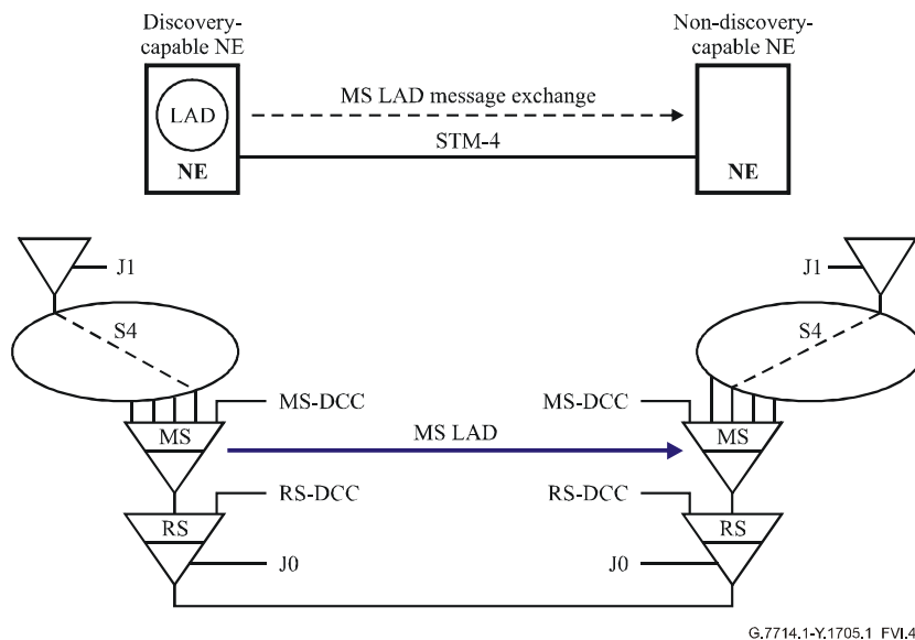
Figure VI.4/G.7714.1/Y.1705.1 – Discovery-capable NE trying to discover a non-discovery-capable NE
