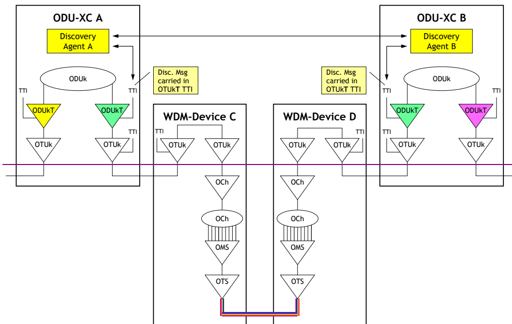
Figure 2/G.7714.1/Y.1705.1 Example of ODUkT TTI (SAPI sub-field) based LAD for OTN with WDM equipment
