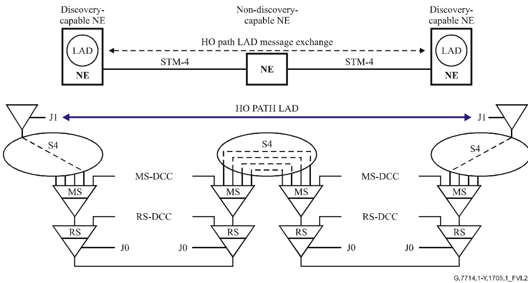
Figure VI.2/G.7714.1/Y.1705.1 – Immediate discovery-capable neighbours at HO path layer – LAD done by NEs
