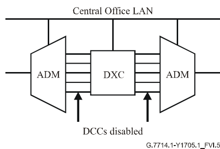
Figure VI.5/G.7714.1/Y.1705.1 – Central Office with disabled DCC connectivity
