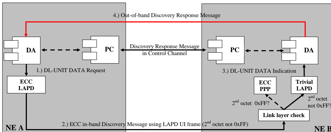
Figure 98/G.7714.1/Y.1705.1 – ECC-based Layer adjacency discovery using LAPD.
