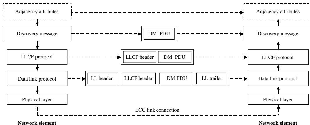
Figure 7/G.7714.1/Y.1705.1 – Layer Adjacency Discovery functions of importance for ECC messages
