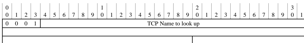
Figure 4/G.7714.1/Y.1705.1 – TCP-ID Name Message format
