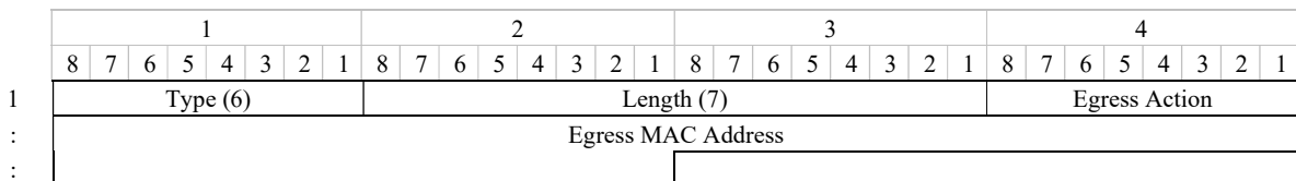
Figure 9.6-5 – Reply eEgress TLV format
