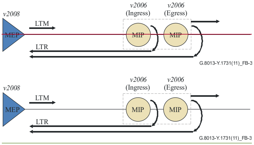
Figure B.3 – Interoperability case 3
