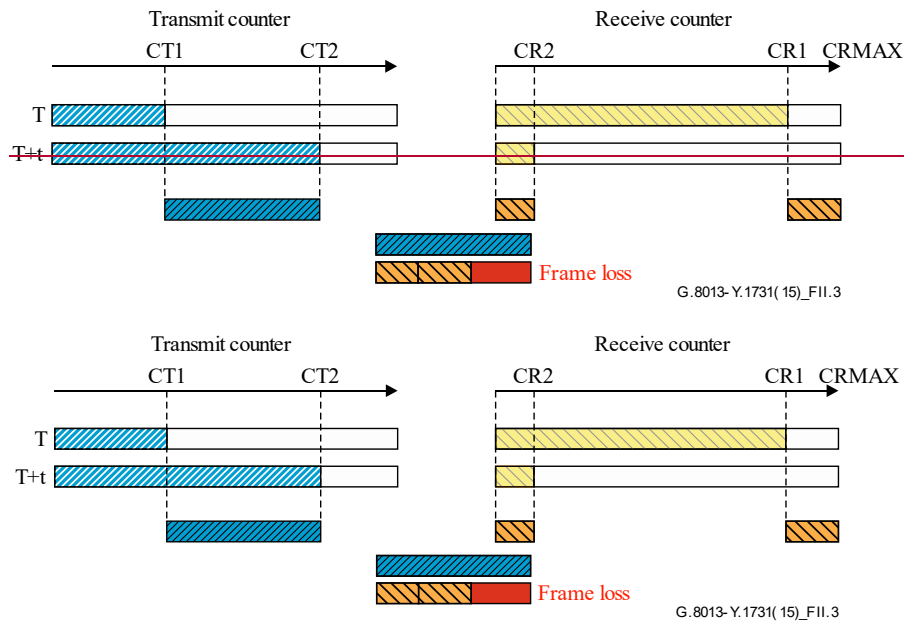
Figure II.3 – Receive counter wraps around
