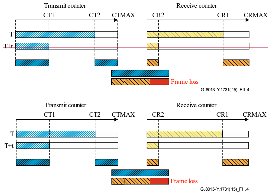
Figure II.4 – Both counters wrap around
