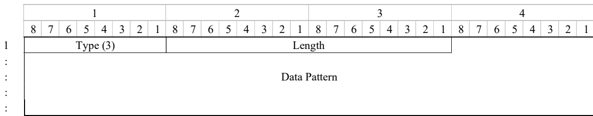
Figure 9.3-3 – Data TLV format
