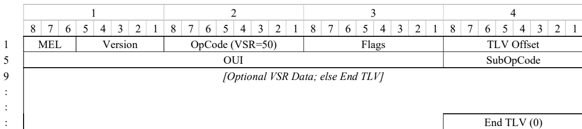
Figure 9.20-1 – VSR PDU format
