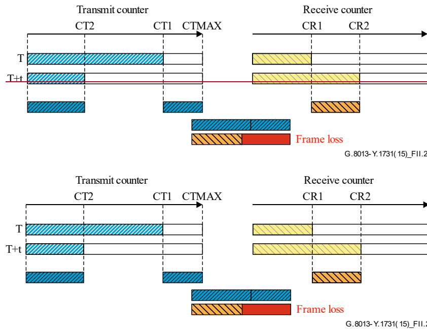
Figure II.2 – Transmit counter wraps around
