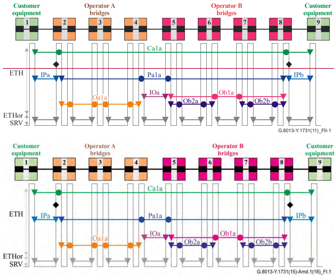
Figure I.1 – Example MEG level assignment for shared MEG levels
