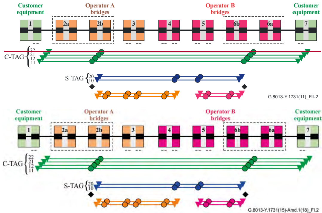
Figure I.2 – Example MEG level assignment for independent MEG levels
