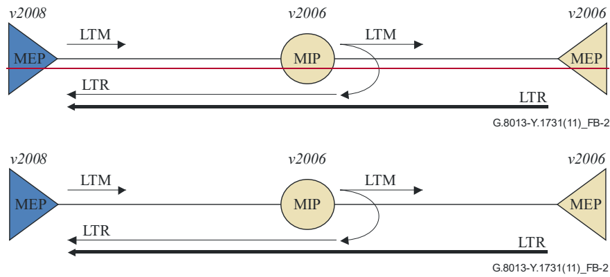
Figure B.2 – Interoperability case 2
