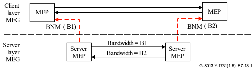
Figure 7.13-1 – Example of ETH-BN BNM transmission
