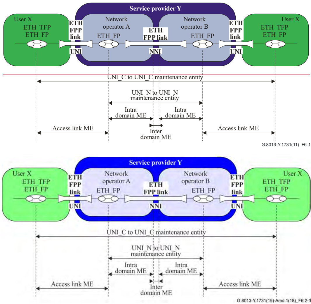
Figure 6.2-1 – Example of MEs associated with a point-to-point connection administrative domain shown in Figure 237-1 of [ITU-T G.8010]
