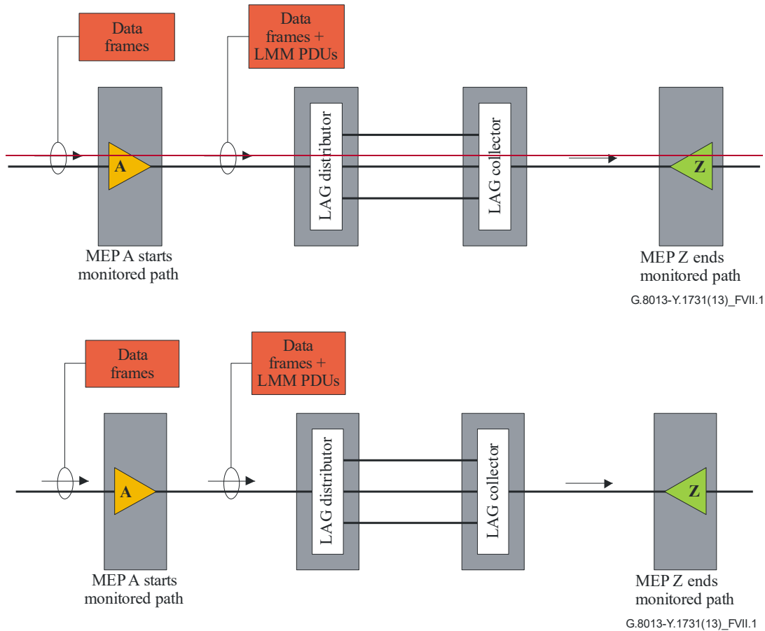
Figure VII.1 – Path monitored for frame loss between two terminating MEPs
