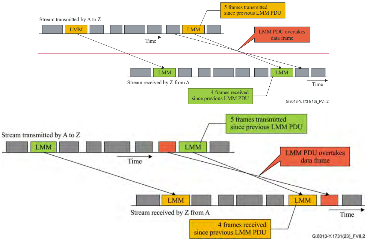
Figure VII.2 – LMM PDU overtakes data frame causing artificial frame loss (or gain)
