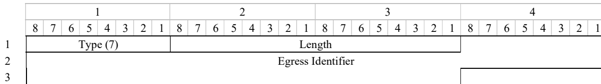
Figure 9.5-3 – LTM egress-identifier Egress Identifier TLV format
