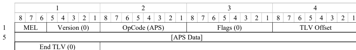
Figure 9.10-1 – APS PDU format
