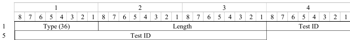
Figure 9.14-3 – Test ID TLV format
