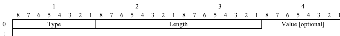
Figure 9.1-2 – Generic TLV format
