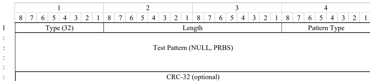
Figure 9.3-4 – Test TLV format
