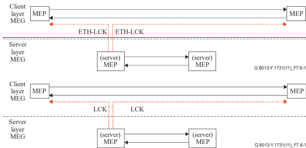
Figure 7.6-1 – Example of ETH-LCK transmission
