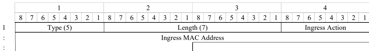
Figure 9.6-4 – Reply ingress TLV format
