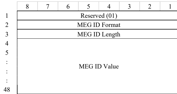
Figure A.1 – Generic MEG ID format
