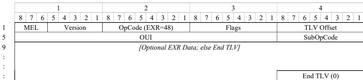
Figure 9.18-1 – EXR PDU format
