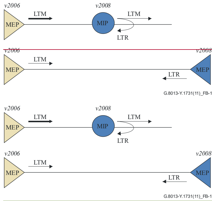
Figure B.1 – Interoperability case 1
