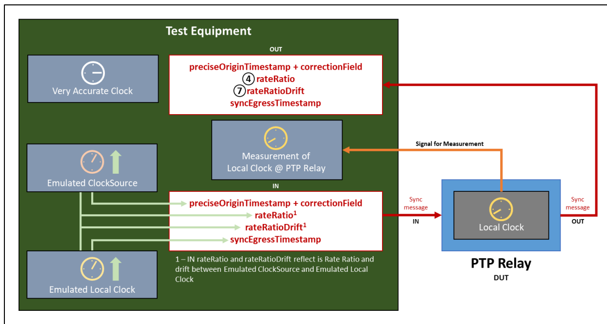
Figure 103: Approach to Testing Normative Requirements for PTP Relay Instance - 3
