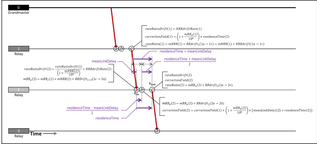
Figure 105: RR Drift Tracking and Error Compensation Calculations – PTP Relay Instance
