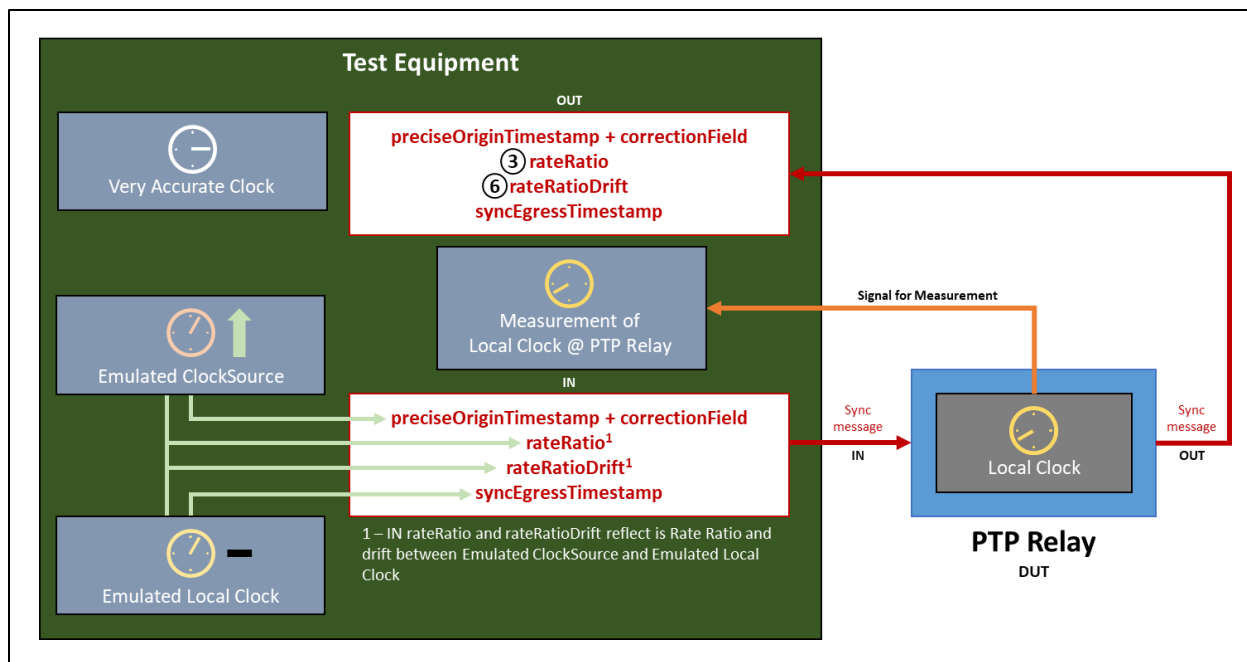
Figure 102: Approach to Testing Normative Requirements for PTP Relay Instance - 2
