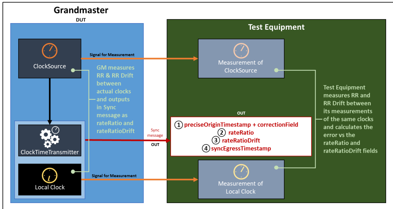
Figure 100: Approach to Testing Normative Requirements for Grandmaster PTP Instance
