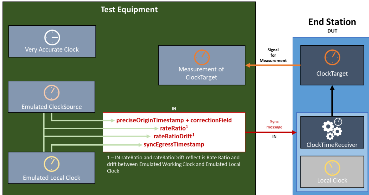
Figure 104: Approach to Testing Normative Requirements for PTP End Instance
