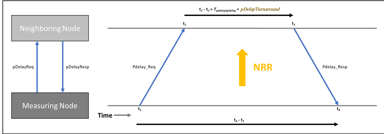
Figure 107: Signals and timestamps to measure path delay
