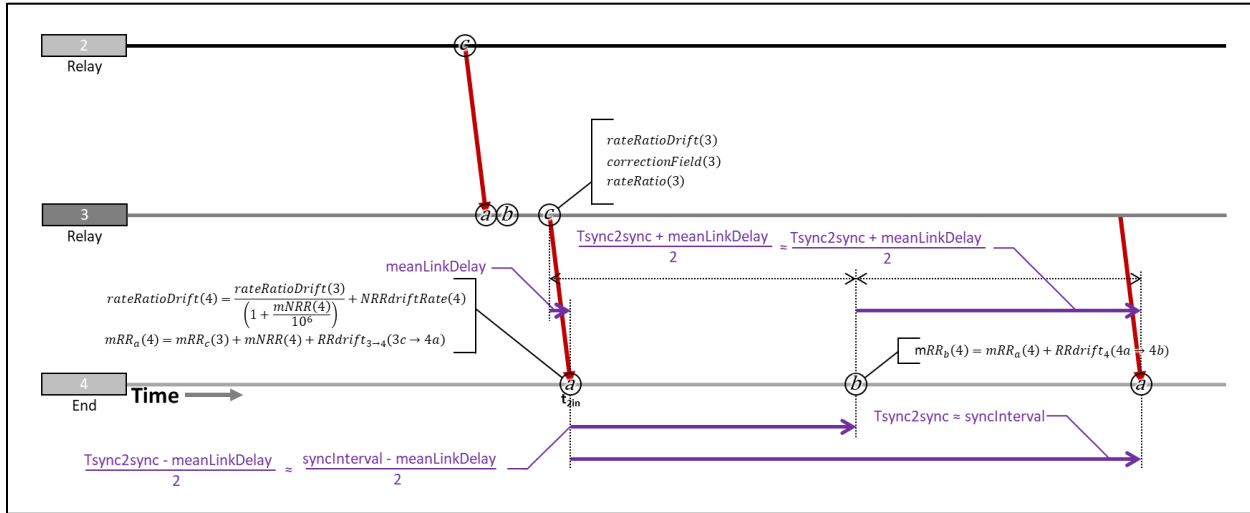
Figure 106: RR Drift Tracking and Error Compensation Calculations – PTP End Instance
