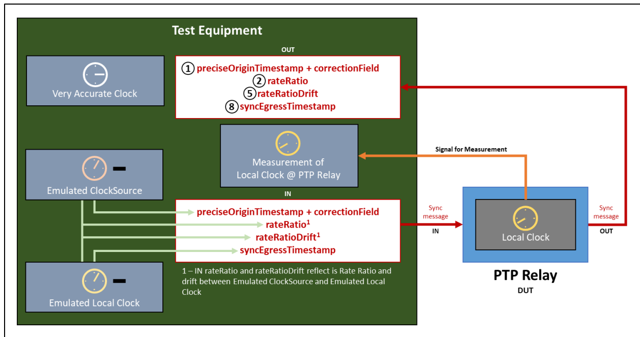
Figure 101: Approach to Testing Normative Requirements for PTP Relay Instance - 1
