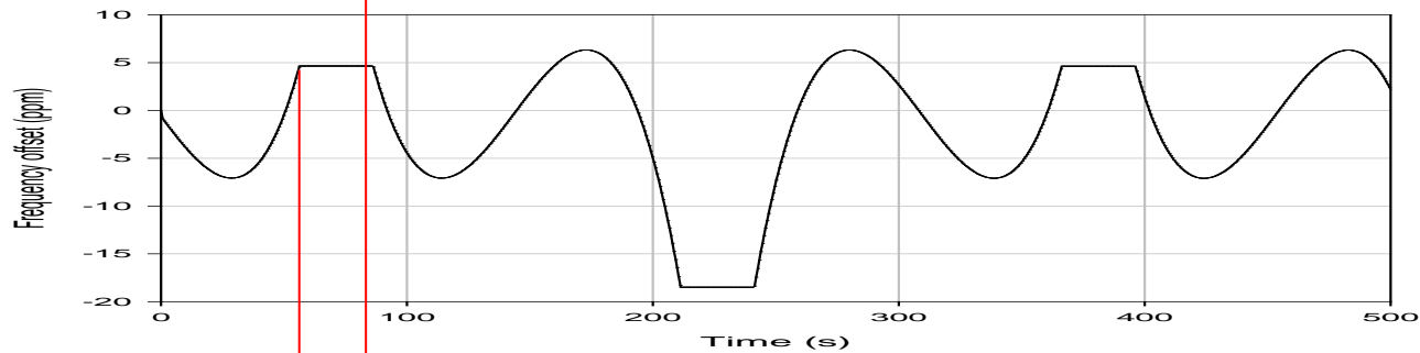
Node 2 error in measured cumulative fractional frequency offset (RR) relative to GM Case H (correction to nRR; no correction to RR or measured prop delay)
