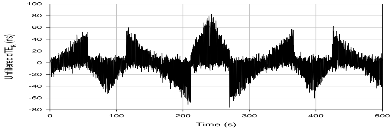
Node 2 dTE_R (relative to GM), before PLL filtering Case H (correction to nRR; no correction to RR or measured prop delay)
