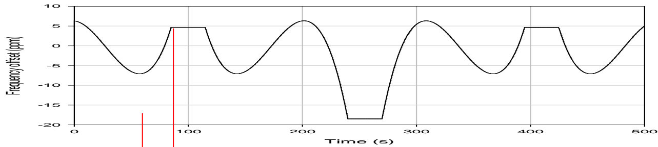
Node 2 local clock fractional frequency offset (relative to TAI frequency) Case G (no corrections to nRR, RR, or measured prop delay)
