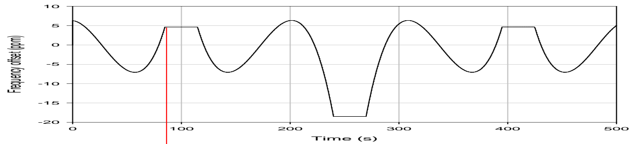
Node 2 local clock fractional frequency offset (relative to TAI frequency) Case H (no corrections to nRR, RR, or measured prop delay)
