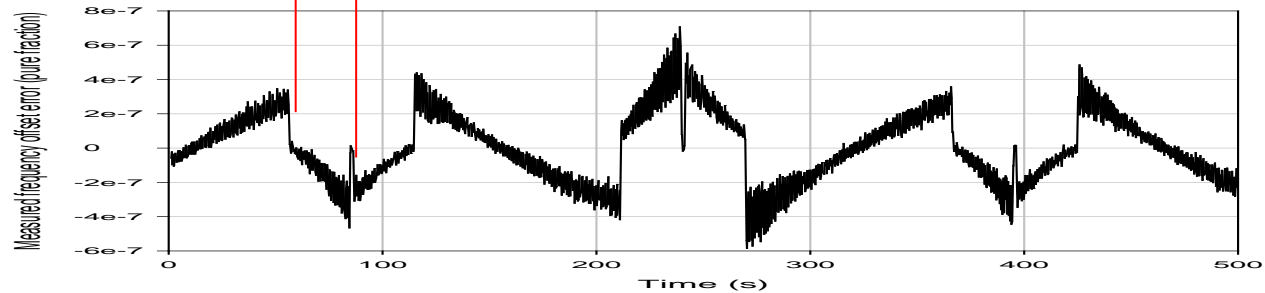
Node 2 error in measured cumulative fractional frequency offset (RR) relative to GM Case H (correction to nRR; no correction to RR or measured prop delay)
