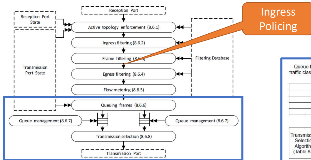
Figure 8-12—Forwarding process functions
