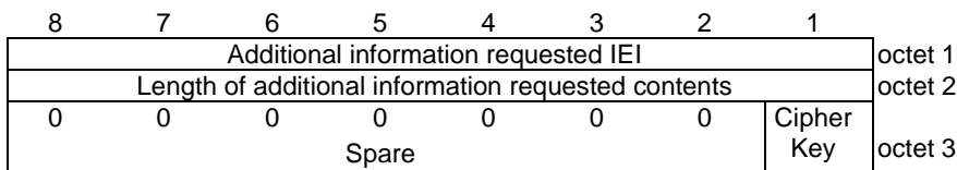
Figure 9.11.3.12A.1: Additional information requested information element
