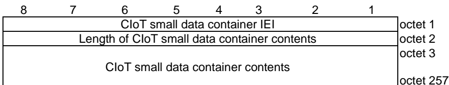
Figure 9.11.3.18B.1: CloT small data container information element
