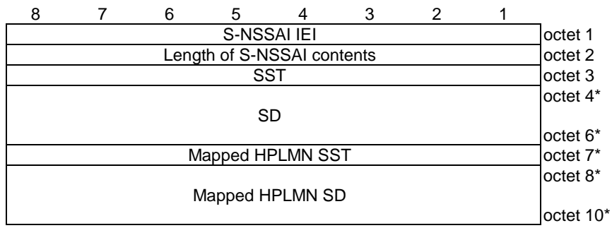
Figure 9.11.2.8.1: S-NSSAI information element
