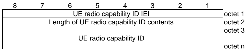
Figure 9.11.3.68.1: UE radio capability ID information element
