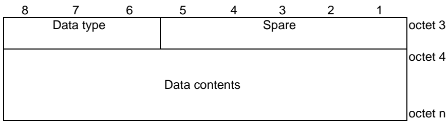
Figure 9.11.3.18B.4: CloT small data container contents for Data type "SMS"
