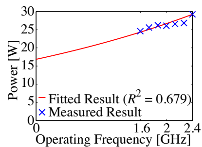
Fig. 4: Maximum Power Consumed by one CPU Core (E5620) in Each P-state
