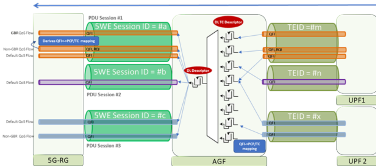
Figure 11: Example of downstream packet forwarding.
