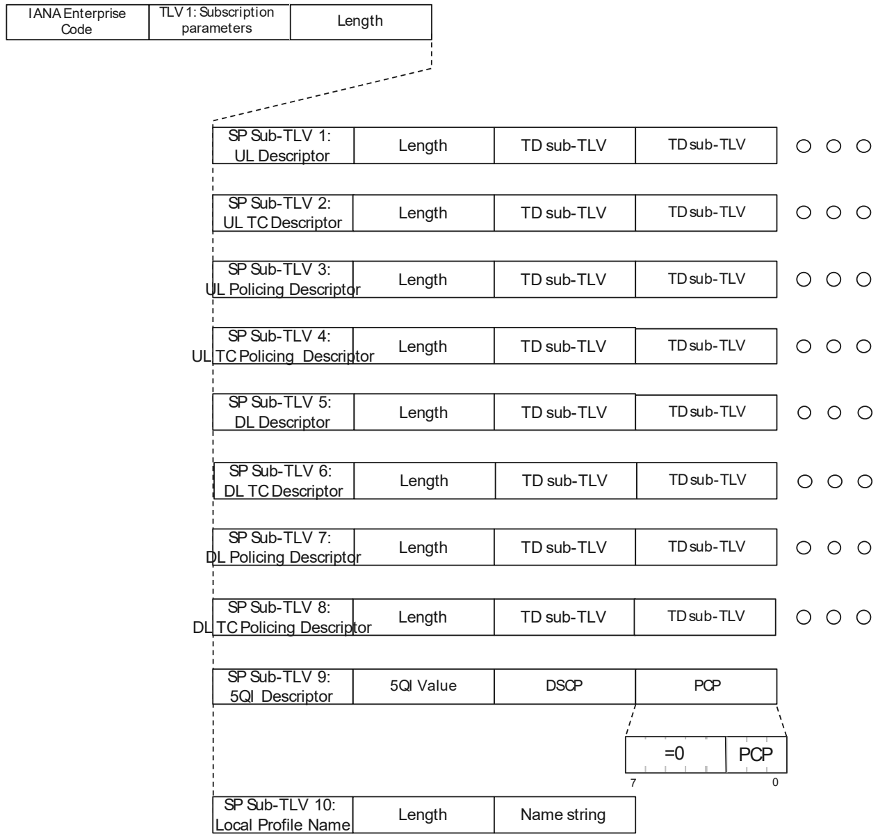
Figure 20: generalized structure of RG-LWAC.
