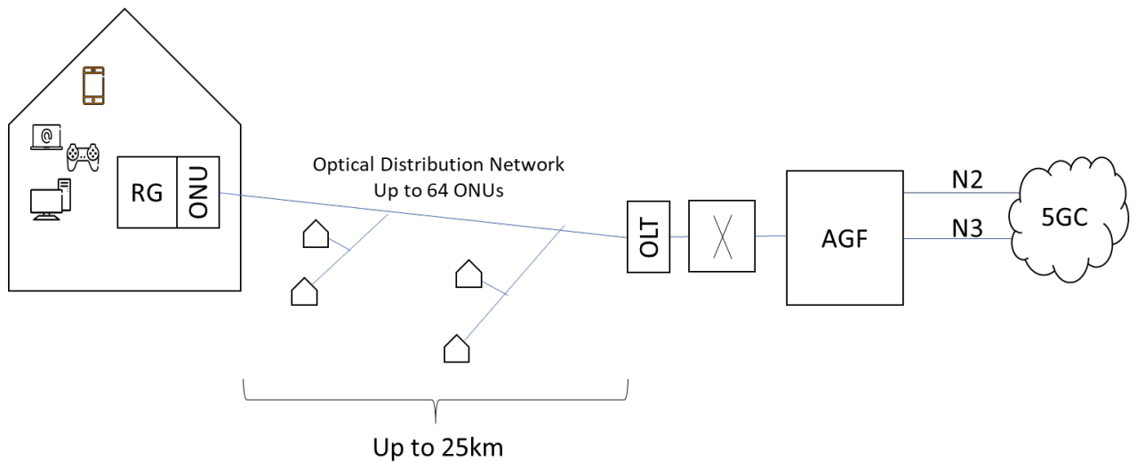
Figure 24: PON access to 5GC Example.
