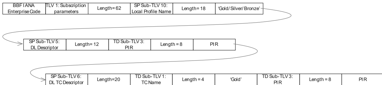
Figure 22: Example of a combination of local profile and selective overriding of parameters.
