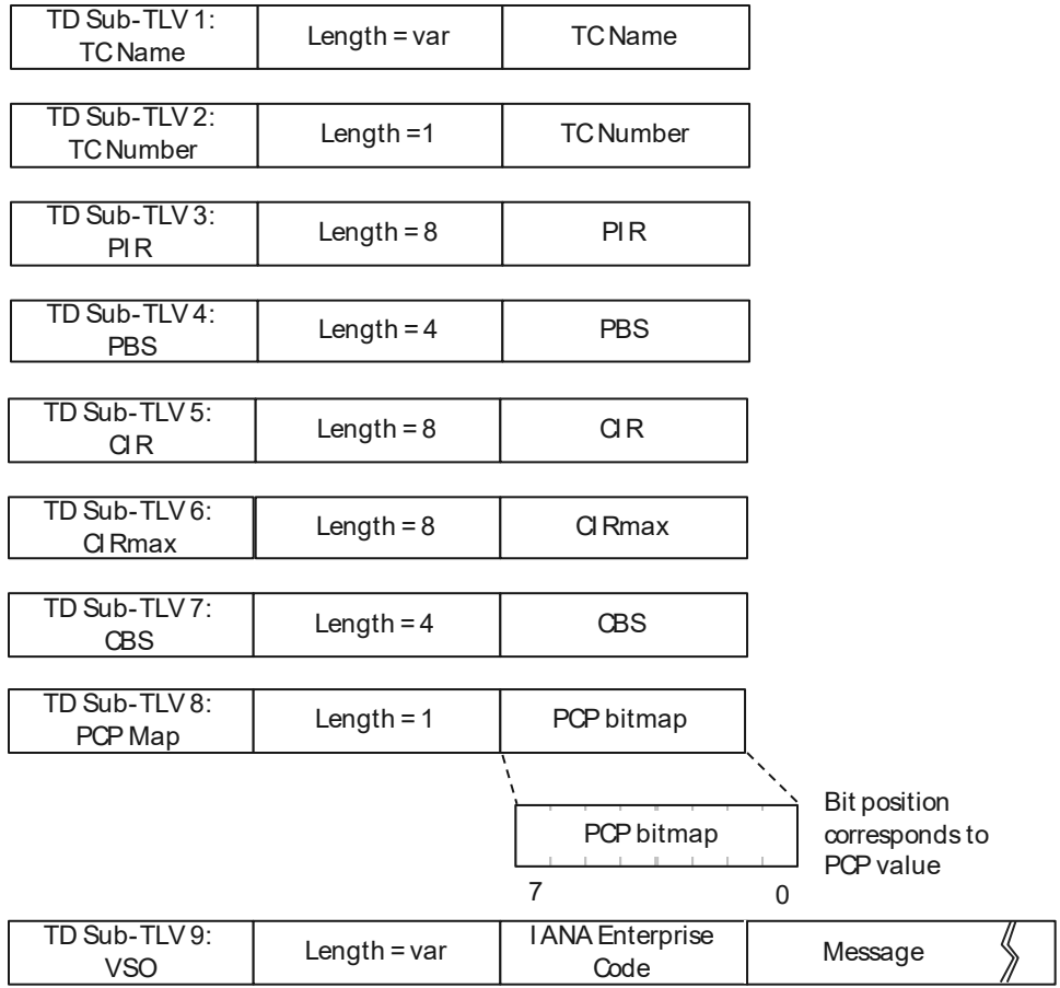
Figure 21: sub TLV family for RG-LWAC Subscription Parameters.
