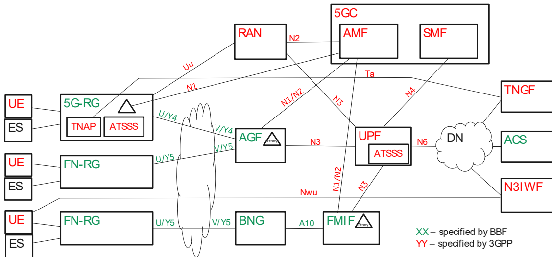
Figure 1: Architectural overview of WWC showing different functions.
