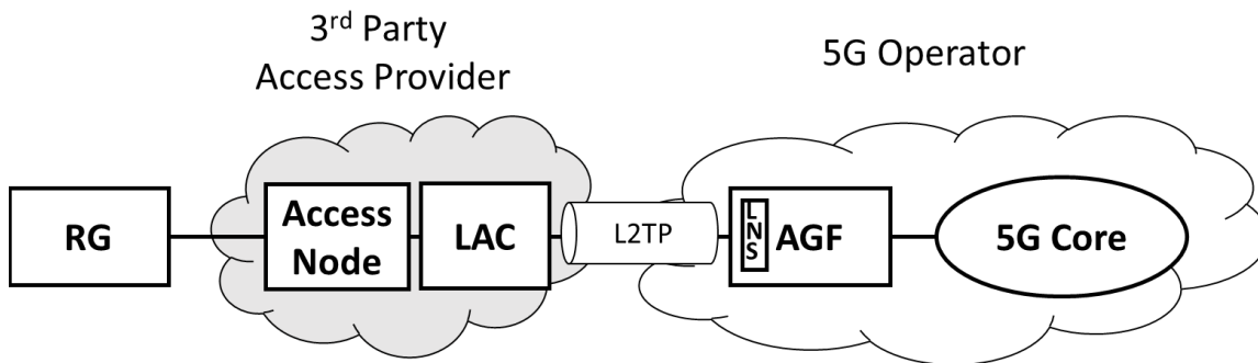
Figure 14: Access Wholesale based on L2TP.
