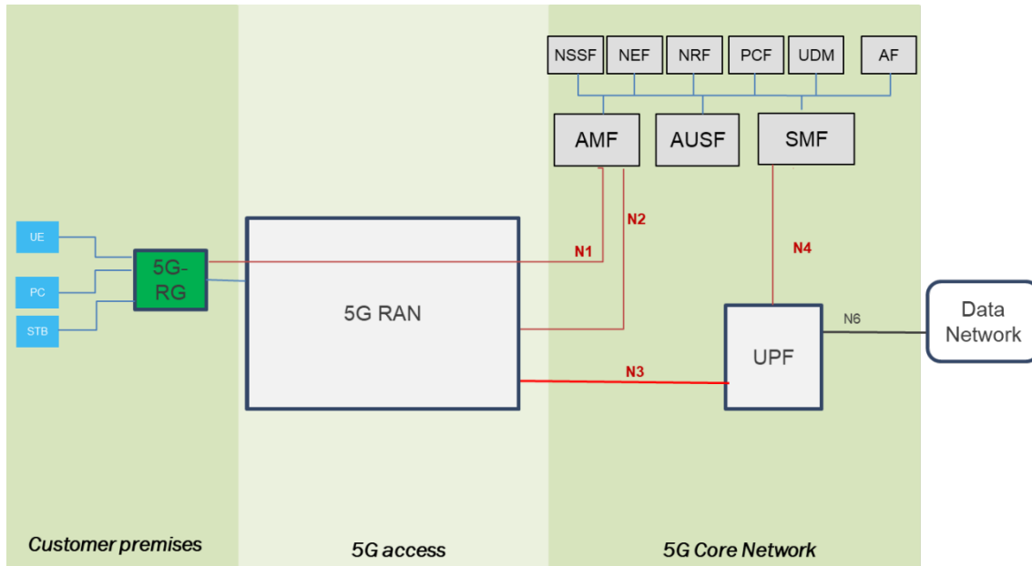
Figure 3: FWA offering fixed services and connecting to 5GC through RAN.
