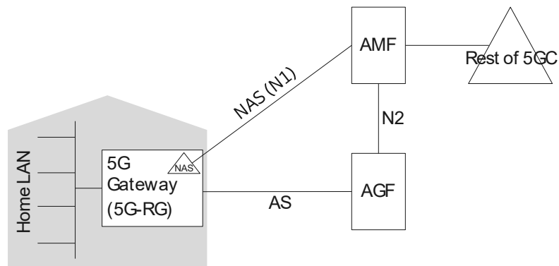
Figure 9: 5G-RG Control Connectivity.
