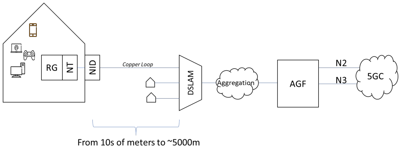
Figure 23: DSL access to 5GC Example.
