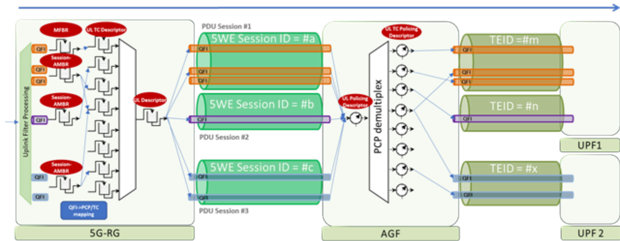
Figure 12: Example of upstream packet forwarding.
