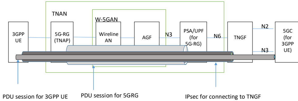
Figure 17: 5G UE behind a 5G-RG.
