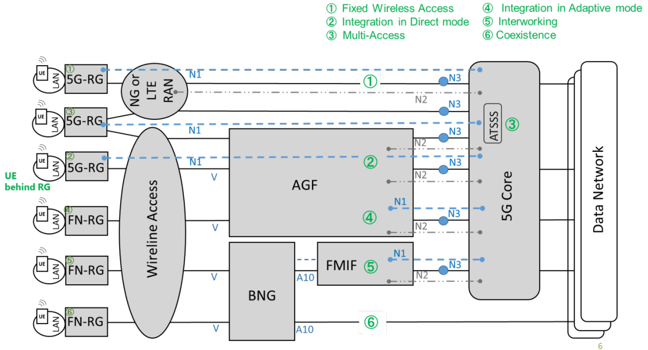
Figure 2: Different deployment scenarios for connecting RGs to the Data Network.
