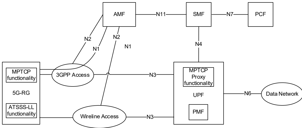
Figure 8: Architecture for ATSSS support.
