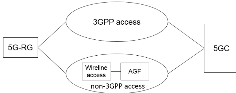
Figure 6: High level view of Hybrid Access for a 5G-RG.
