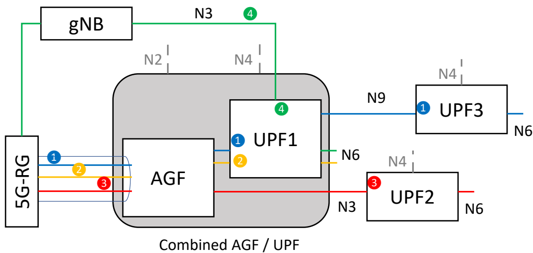
Figure 16: Example of combined AGF/UPF.
