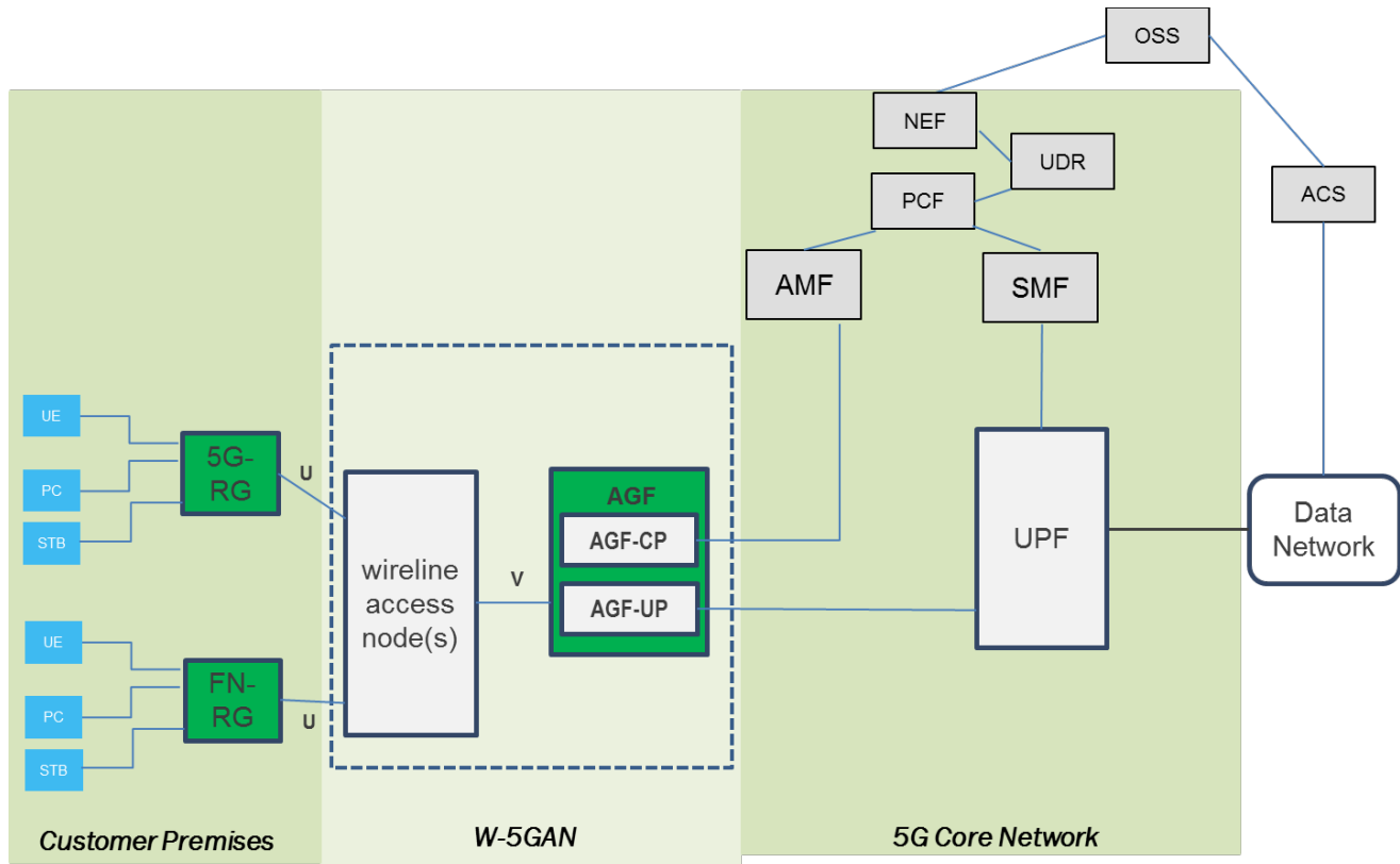
Figure 15: Interaction of ACS with PCF through the OSS.
