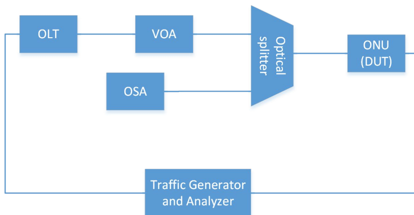
Figure 15: Test Setup Side Mode Suppression Ratio Parameter Tests
