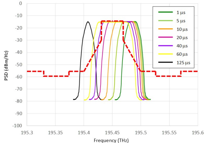
Figure 4 MSE and OOC Template Overlaid on Idealized Spectral Excursion Plot
