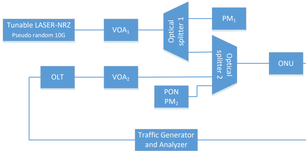
Figure 4: Test Setup for XG(S)-PON ONU filtering
