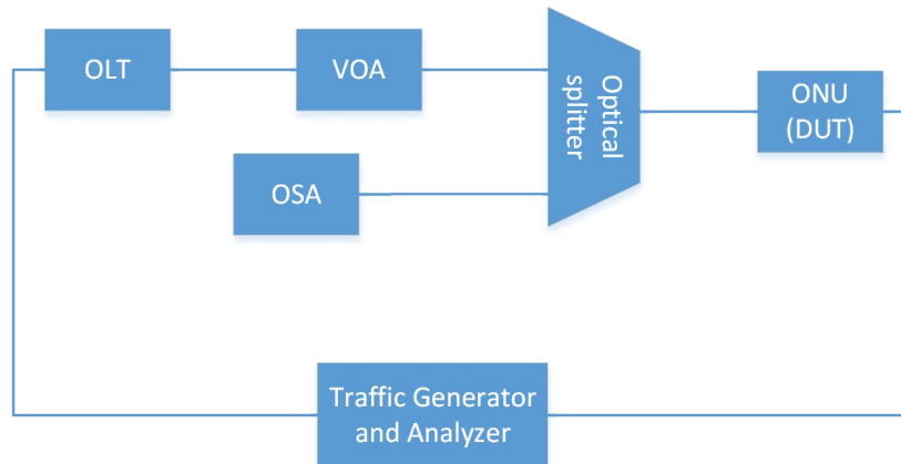
Figure 3: Test Setup Central ONU Wavelength Parameters Tests
