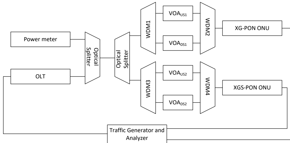
Figure 22: Test Setup for OLT Receive Sensitivity in dual rate operations
