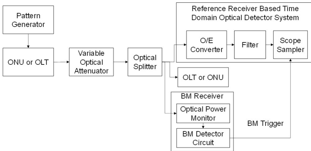
Figure 2 - Optical eye pattern, waveform, and extinction ratio measurement configuration
