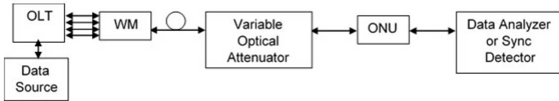
Figure 8 – Test Setup for ONU Receiver Tuning Time
