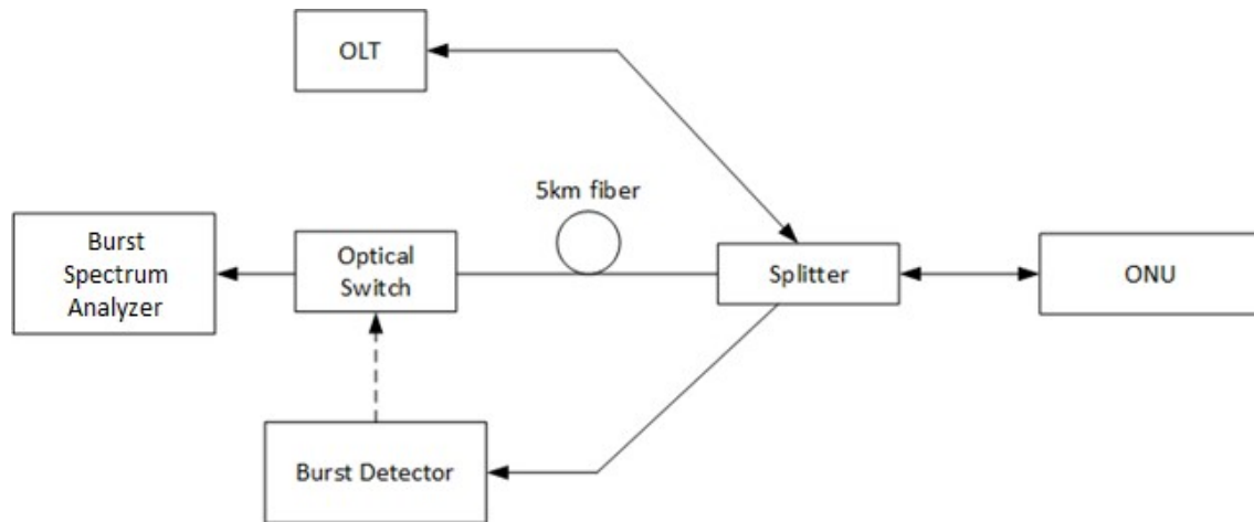
Figure 9 – Test Setup for Upstream Optical PSD when not Enabled
