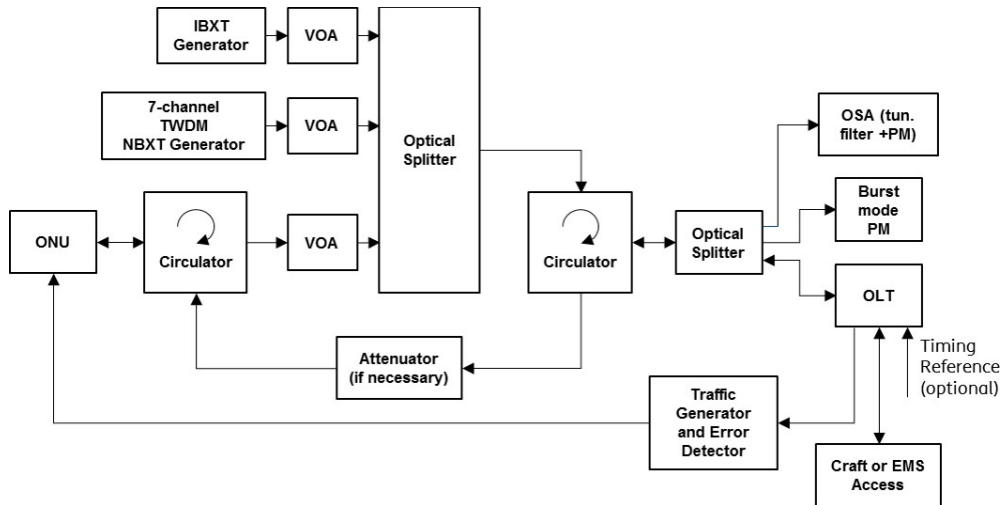
Figure 19– Test Setup for OLT Receive Sensitivity
