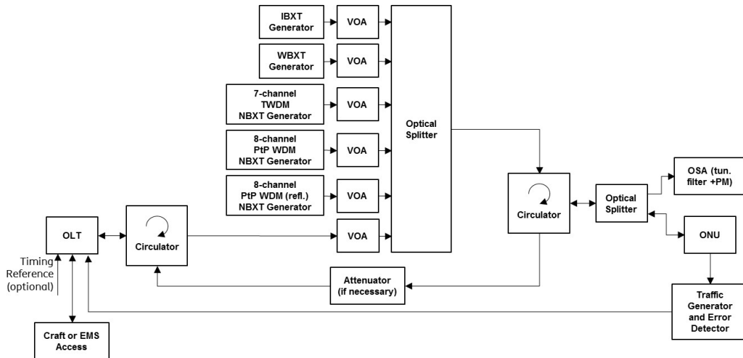
Figure 12.1 – Simplified Test Setup for ONU Receive Sensitivity
