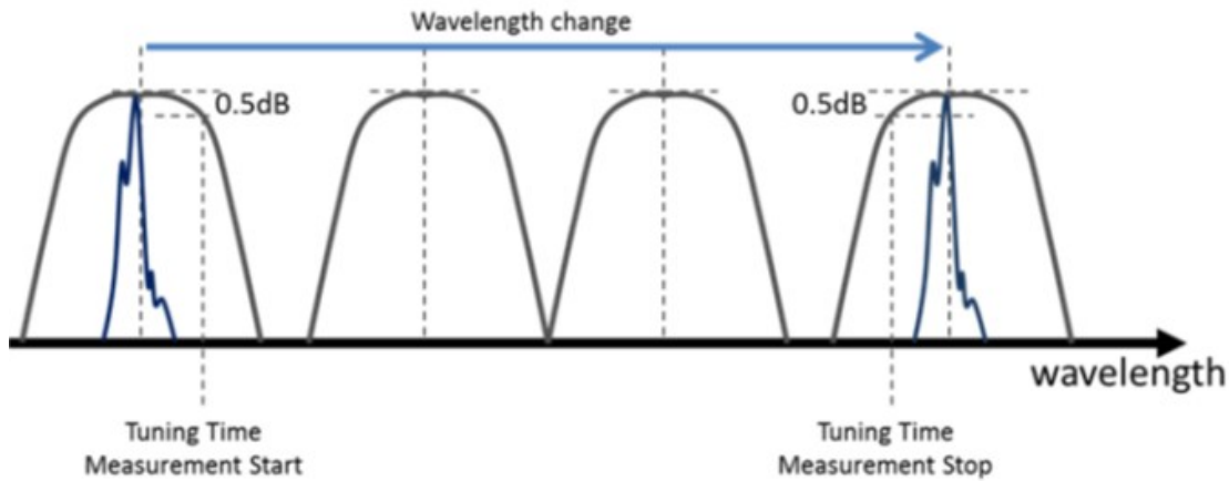
Figure 5 – Illustration of laser tuning across the operating band
