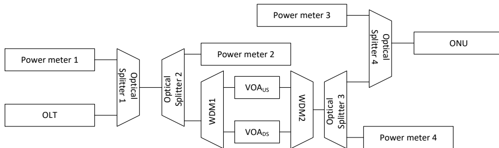
Figure 24: Test Setup for Optical supervision
