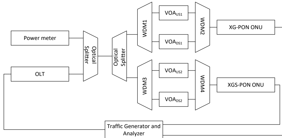
Figure 21: Test Setup for OLT Receive Overload in dual rate operations
