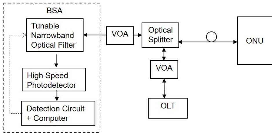
Figure 1 Test Setup for MSE, OOC and OOB (VOA = Variable Optical Attenuator)
