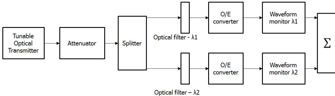
Figure 6 - Test Setup for Tuning Time of ONU Transmitter
