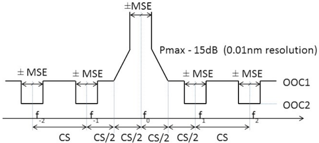
Figure 3 “OOC PDS Mask Definition” from G.989.2
