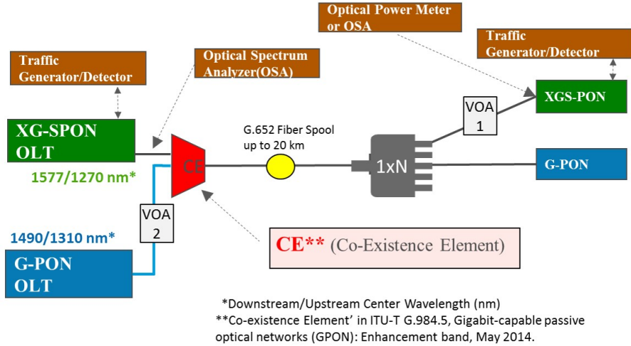
Figure 23 – Test Setup for XGS-PON ONU Coexistence with GPON
