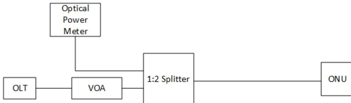
Figure 10 – Test Setup for ONU Transmit Power
