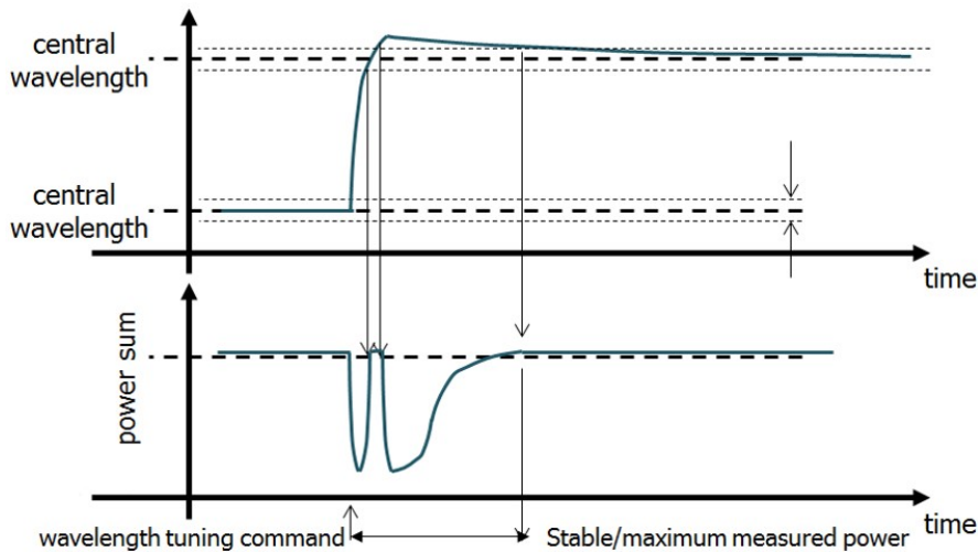
Figure 7 - Optical power vs. time from summation of waveform monitors
