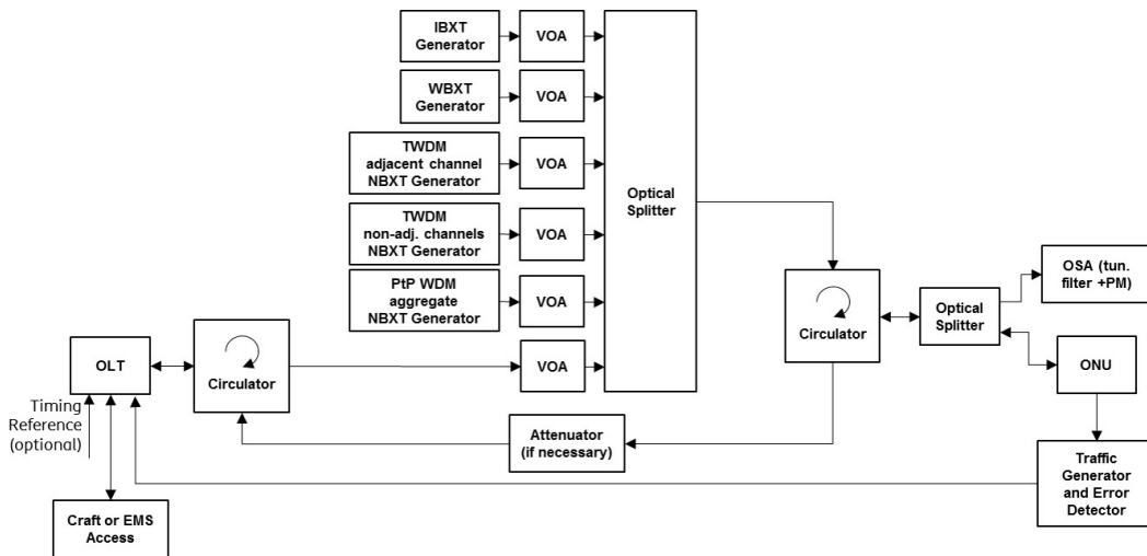
Figure 12.2– Simplified Test Setup for ONU Receive Sensitivity
