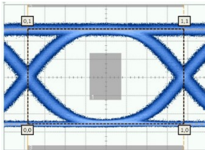
Figure 12 - Basic eye mask coordinate system
