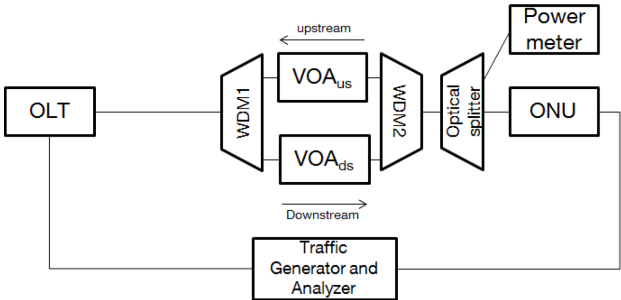
Figure 14: Test Setup for ONU Receive Overload
