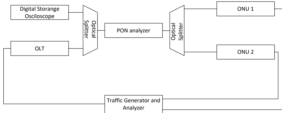
Figure 16:: Test Setup for Allocation of the physical layer overhead time and launched optical power without input to the transmitter
