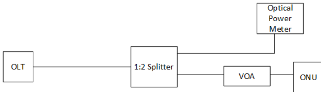
Figure 18 – Test Setup for OLT Transmit Power
