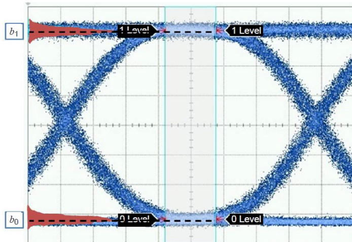
Figure 11 - Histograms centered in the central 20 % of the eye used to determine the mean logic one and 0 levels, b_1 and b_0
