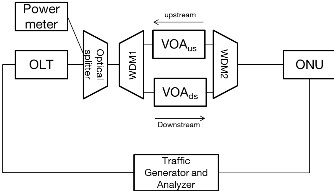
Figure 20: Test Setup for OLT Receive Overload
