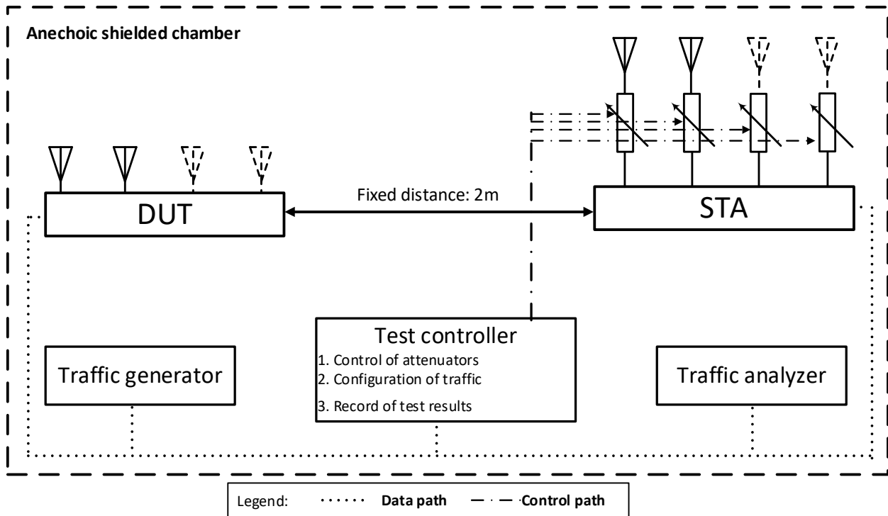
Figure 10: Test setup of Range Versus Rate Test
