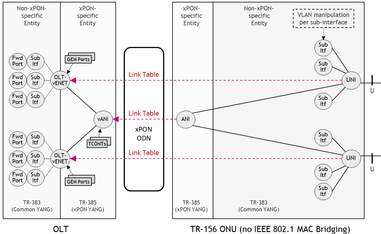
Figure 5-9/18 - Ethernet Service Model Example for TR-156 Application
