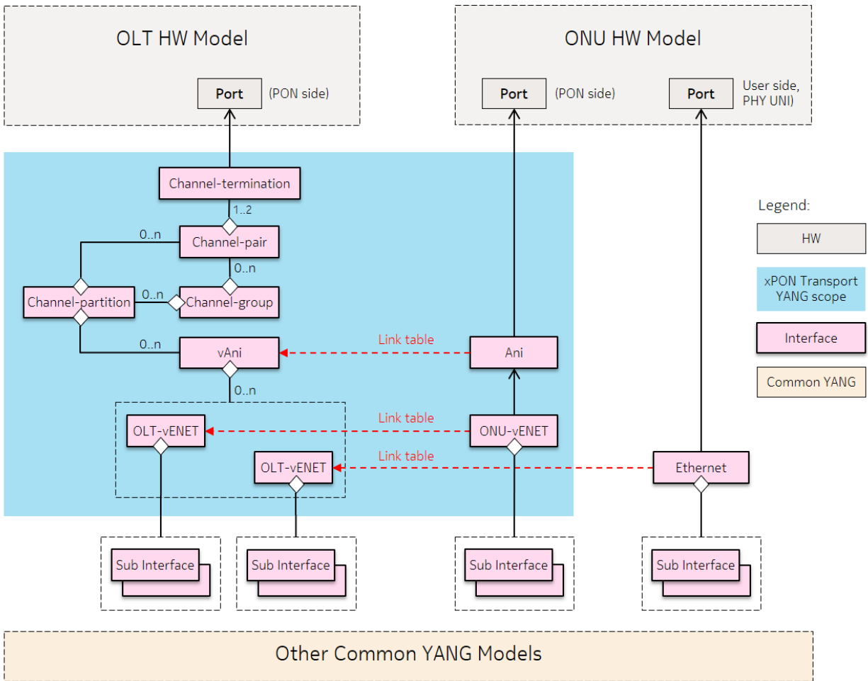
Figure 5-6/Figure 16 - Interfaces and Hardware Entities Relationships
