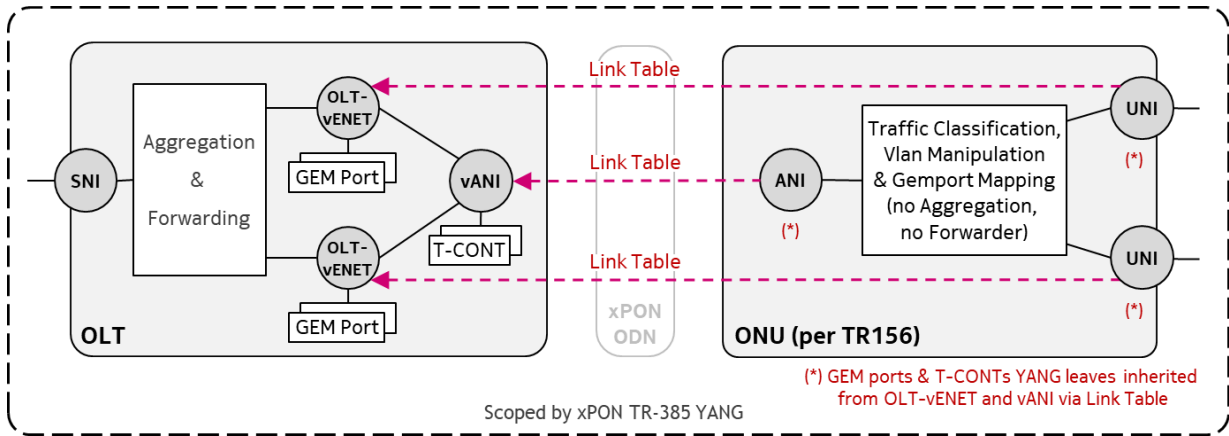
Figure 4-6/6 – TR-156 case with UNIs and ANI mirrored on the OLT
