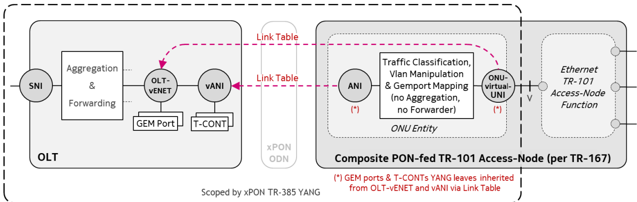
Figure 4-7/7 – TR-167 Case with ONU-virtual-UNI and ANI mirrored on the OLT
