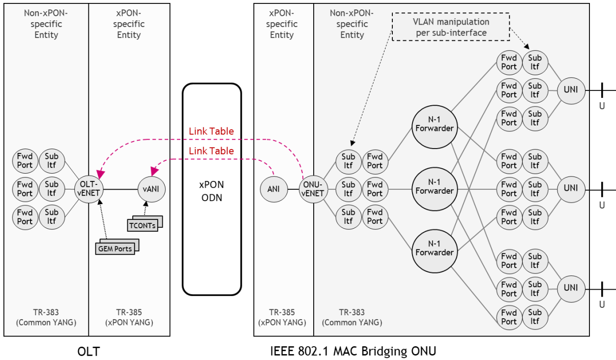
Figure 5-11/20 - Ethernet Service Model Example for IEEE 802.1 MAC Bridging ONU
