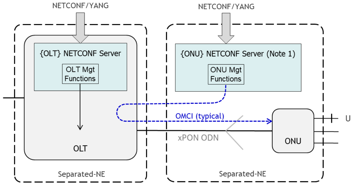
Figure 4-2/Figure 2 - {OLT} and {ONU}s Separated-NE mode
