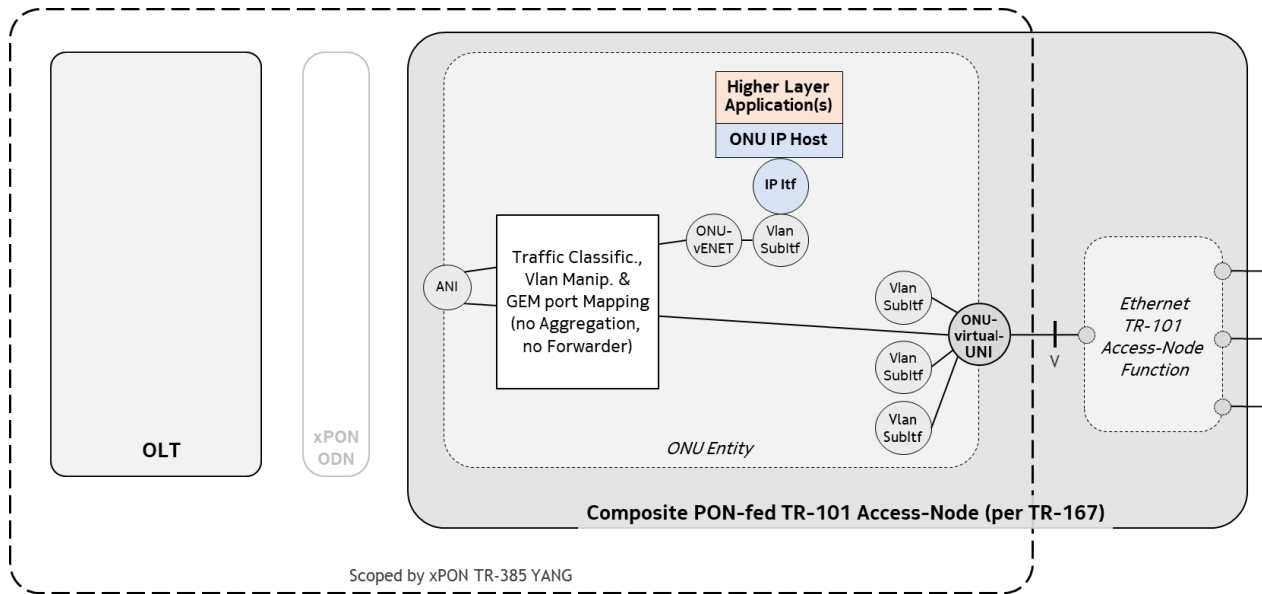
Figure 5-4/Figure 14 – GEM ports for a host function in a TR-167 ONU
