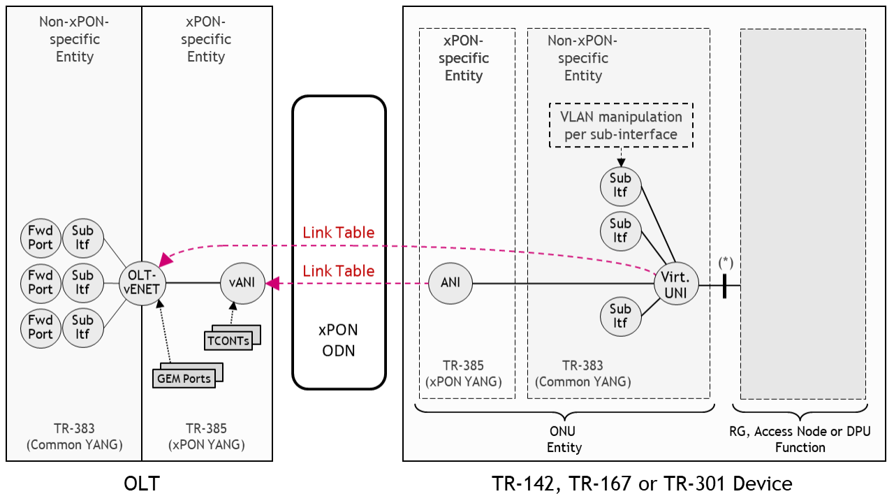
Figure 5-10/19 - Ethernet Service Model Example for TR-142, TR-167 and TR-301 Applications
