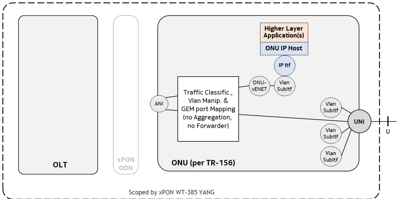
Figure 5-3/13 – GEM ports for a host function in a TR-156 ONU
