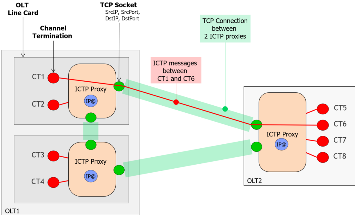
Figure 5-17/Figure 26 – An example of ICTP Interconnection Pattern
