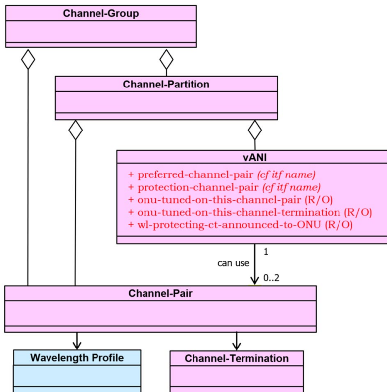
Figure 5-15/Figure 24 – Support for ONU WL Mobility
