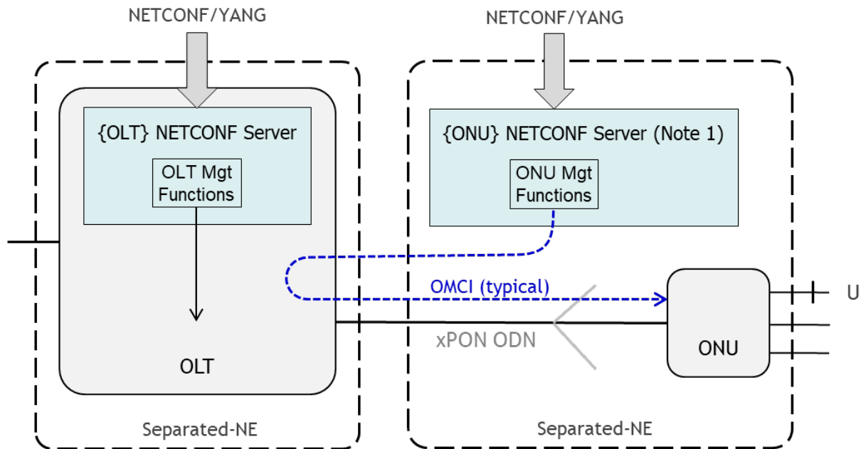
Figure 4-2/Figure 2 - {OLT} and {ONU}s Separated-NE mode
