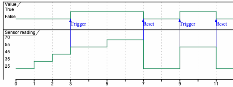
Figure 35: IoT threshold trigger sensitivity
