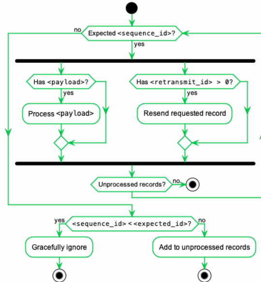
Figure 12: Processing of Received USP Records
