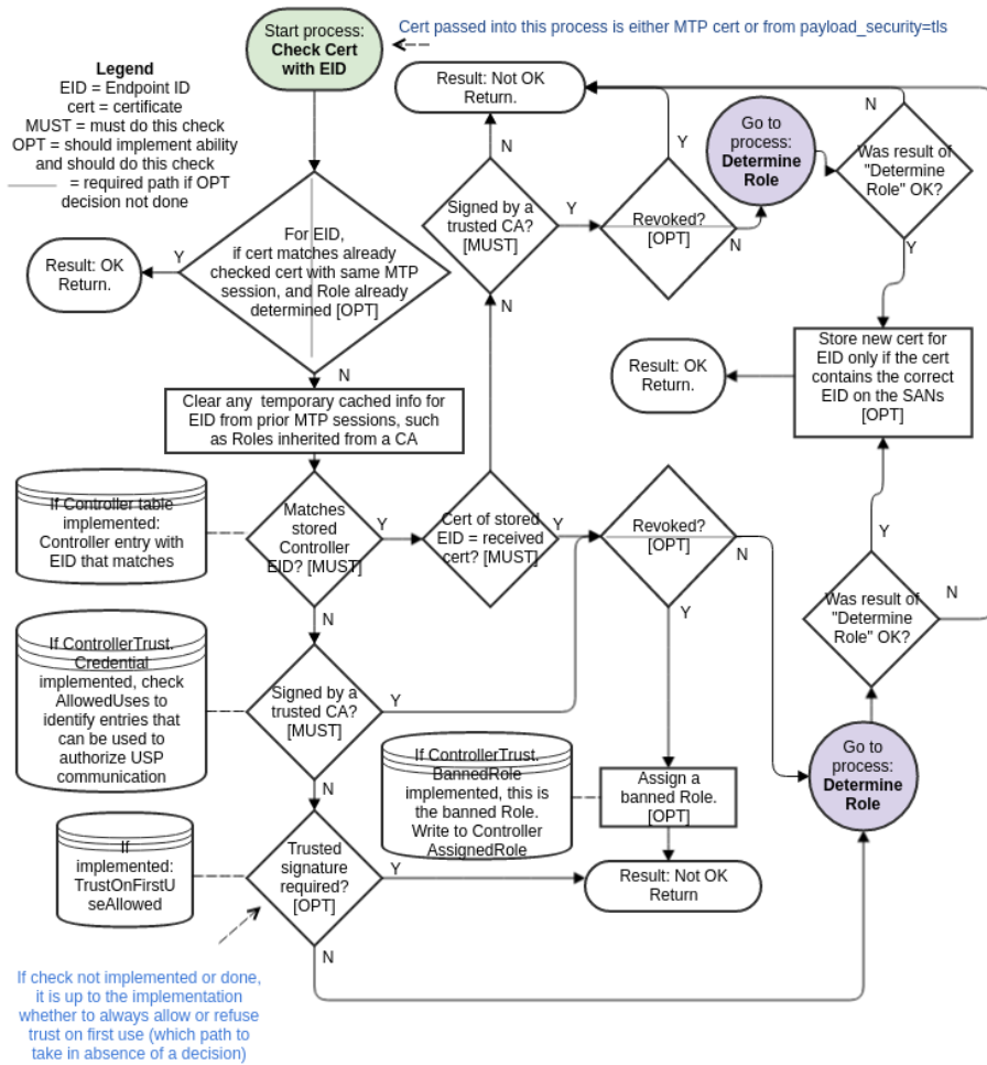
Figure 22: Checking a Certificate
