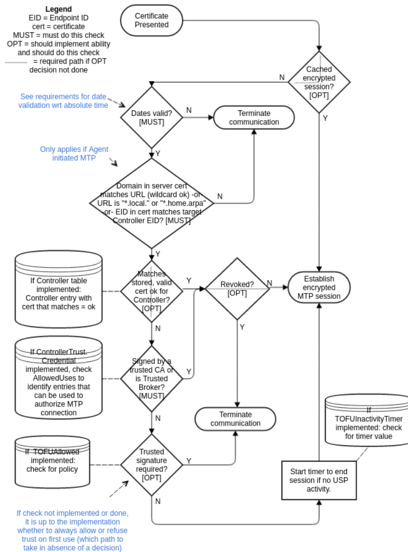
Figure 2: Receiving a X.509 Certificate
