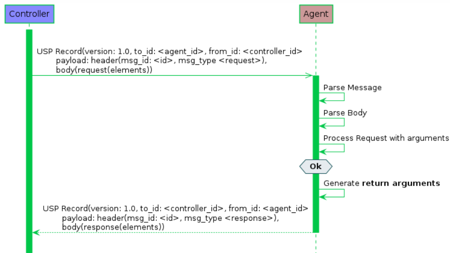
Figure 15: A successful request/response sequence
