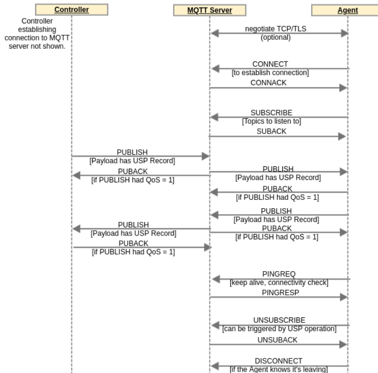
Figure 8: MQTT Packets
