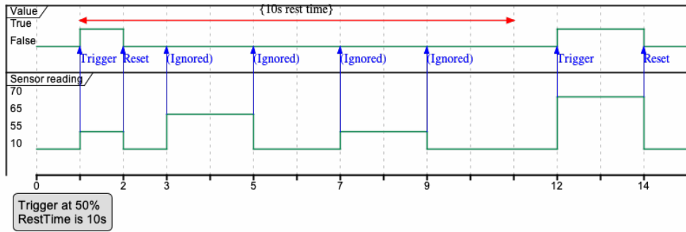
Figure 37: IoT threshold trigger rest time
