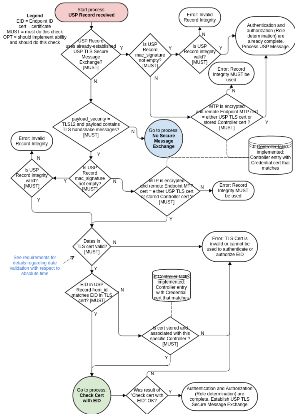
Figure 19: Receiving a USP Record
