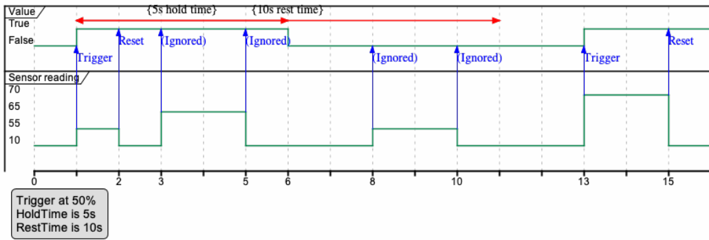
Figure 38: IoT threshold trigger minimum duration
