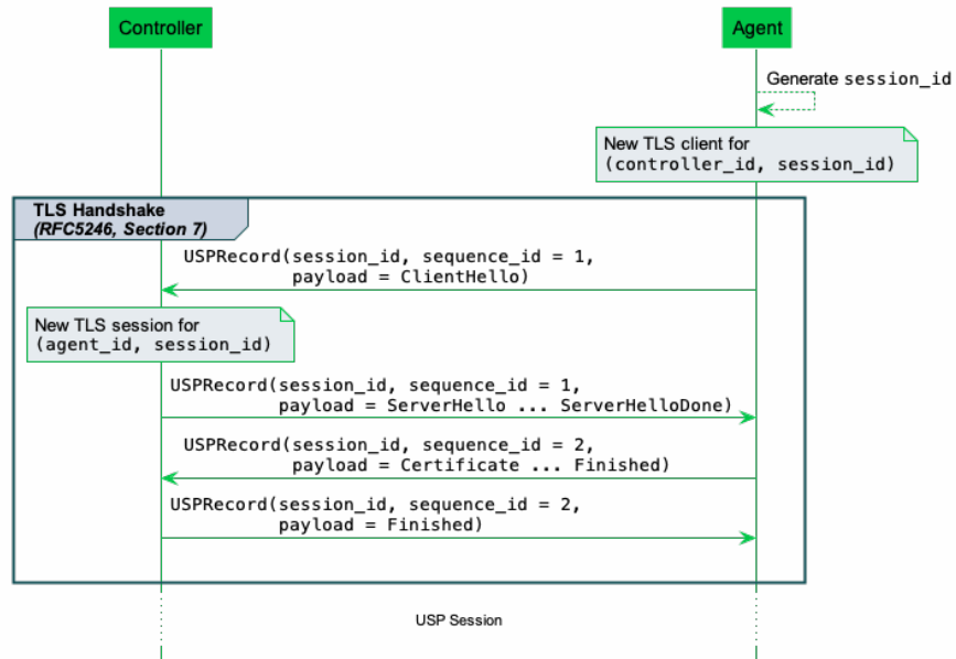
Figure 14: TLS Session Handshake
