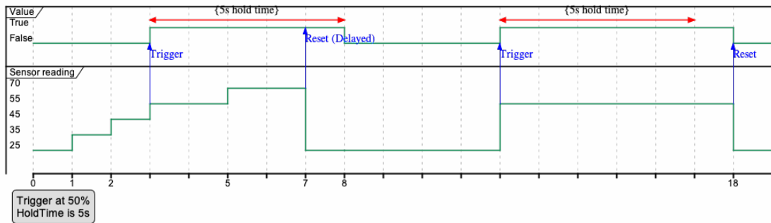
Figure 36: IoT threshold trigger hold time
