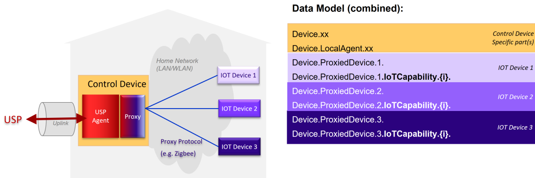
Figure 34: IoT proxied device model
