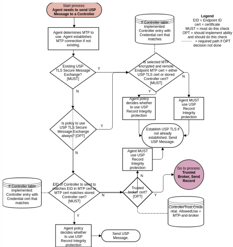
Figure 21: Sending a USP Record
