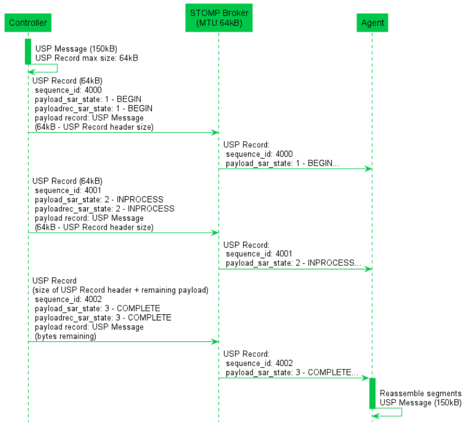
Figure 13: E2E Segmentation and Reassembly
