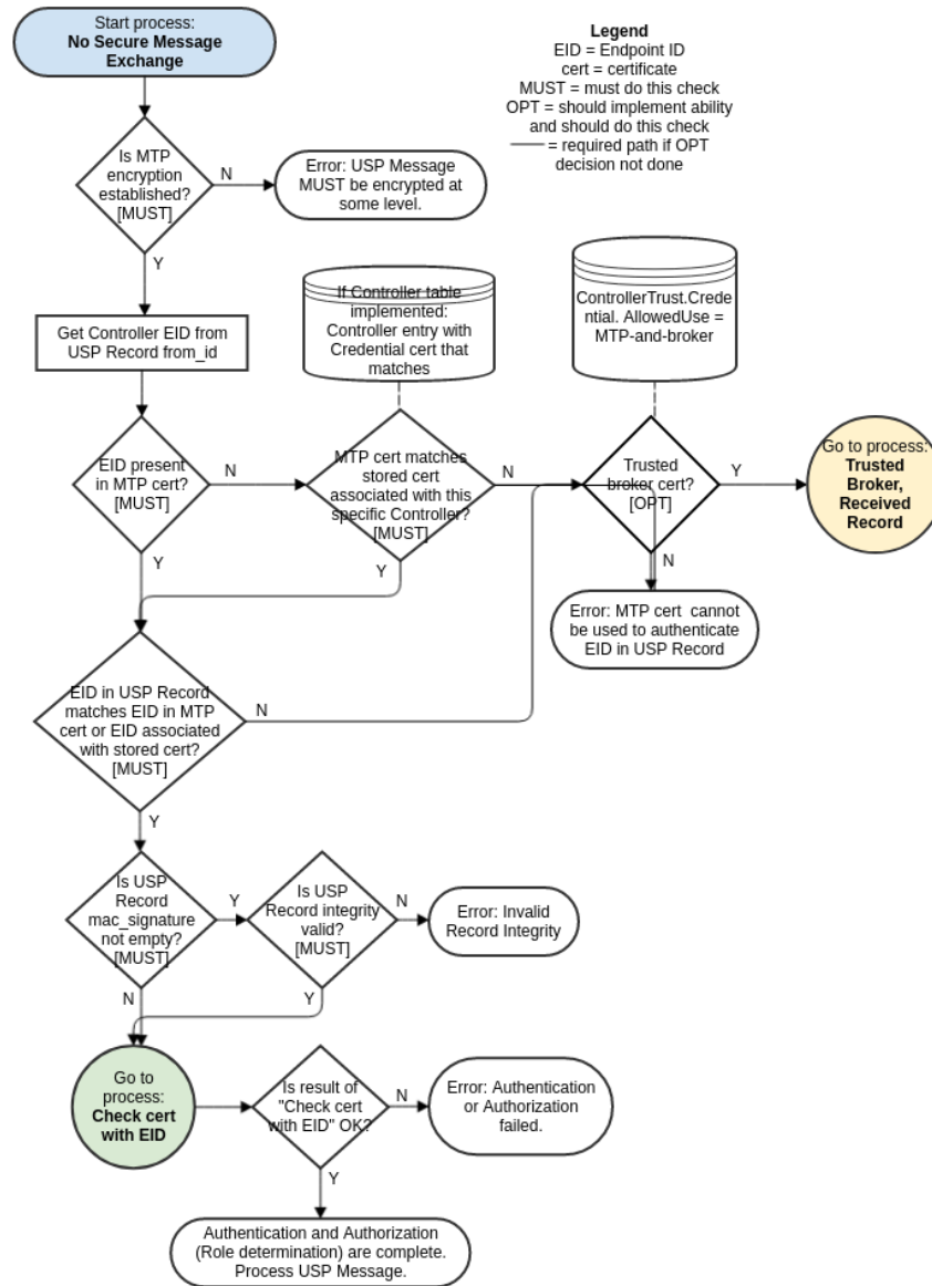
Figure 17: USP Record without USP Layer Secure Message Exchange
