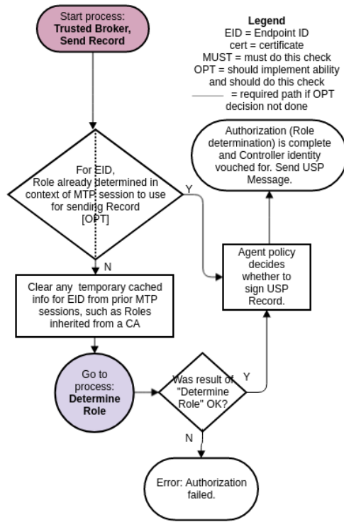
Figure 22: Trusted Broker Sending a Record
