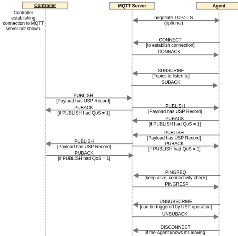
Figure 8: MQTT Packets
