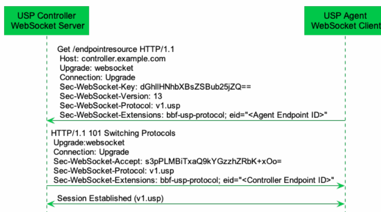
Figure 4: WebSocket Session Handshake
