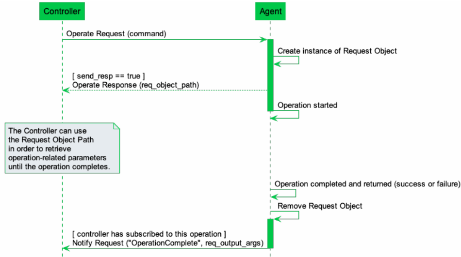
Figure 15: Operate Message Flow for Asynchronous Operations
