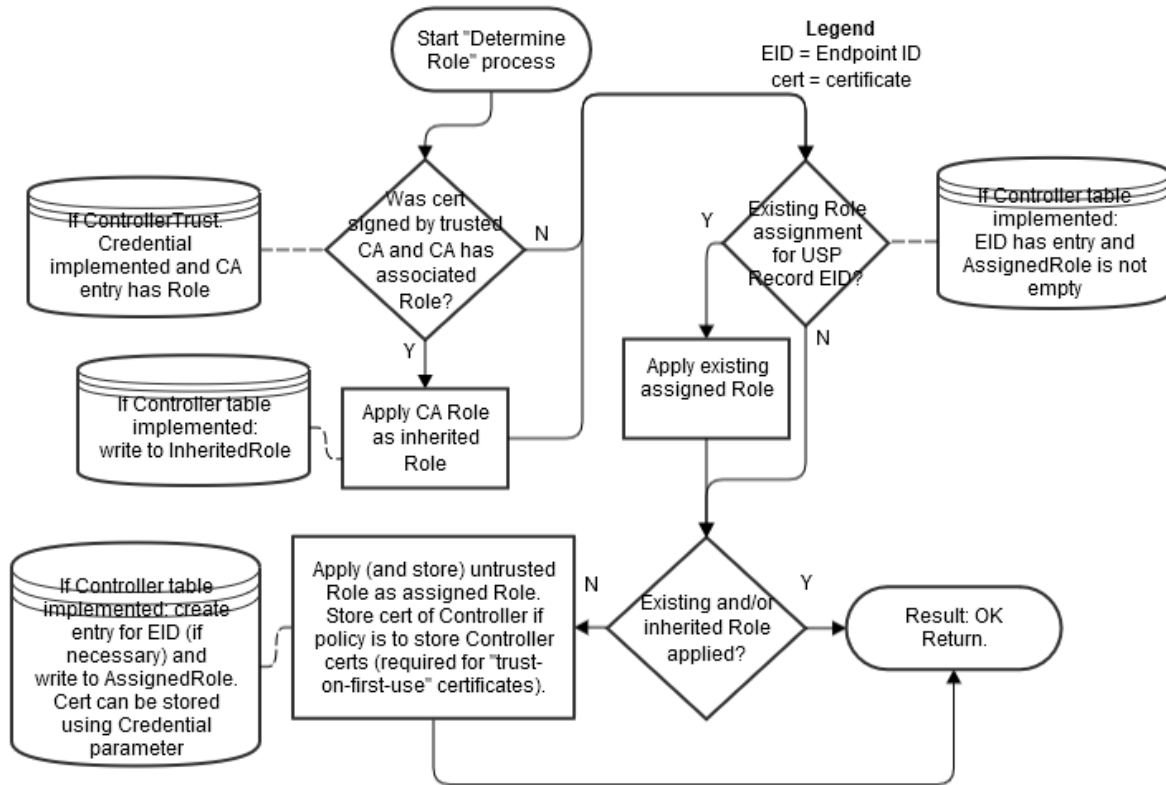
Figure SEC.5 – Determining the Role
