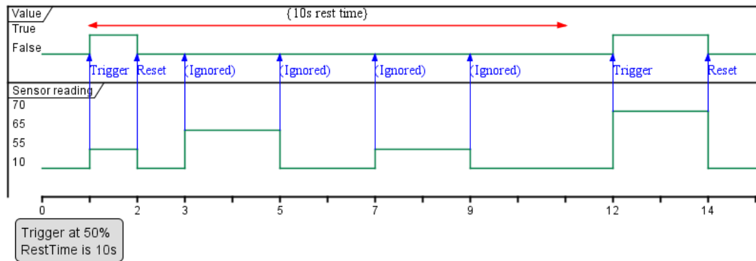
Figure IOT.6 - IoT threshold trigger rest time
