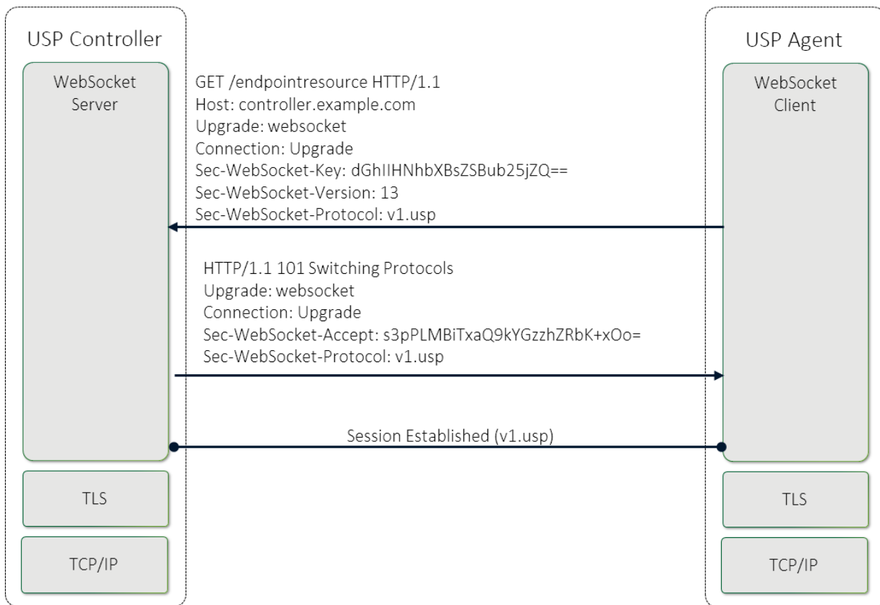
Figure WS.1 - WebSocket Session Handshake
