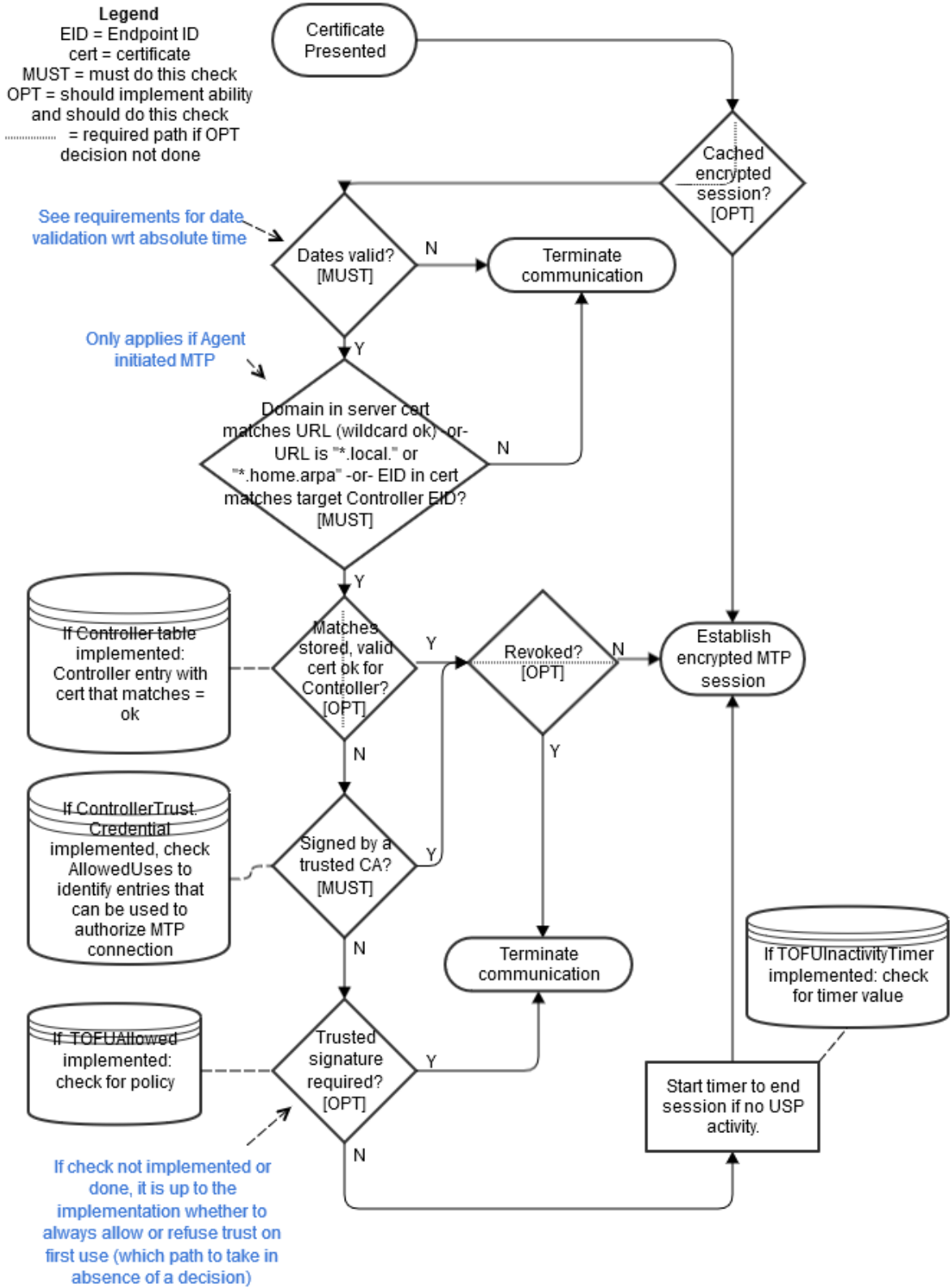
Figure MTP.1 – Receiving a X.509 Certificate
