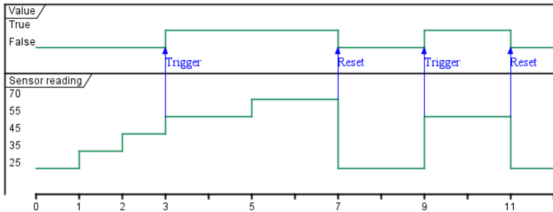
Figure IOT.4 - IoT threshold trigger sensitivity
