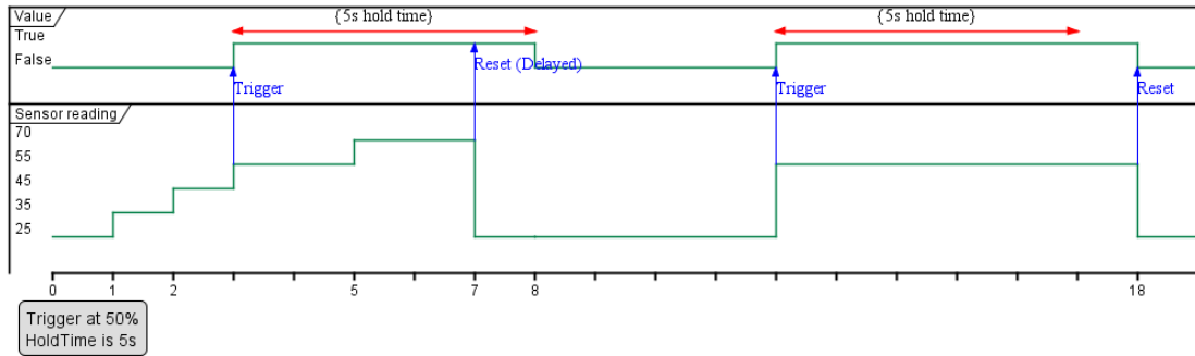
Figure IOT.5 - IoT threshold trigger hold time
