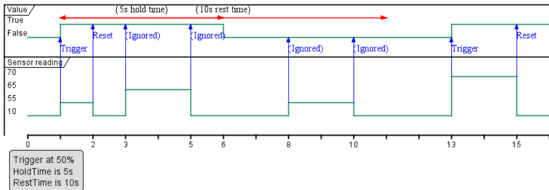
Figure IOT.7 - IoT threshold trigger minimum duration
