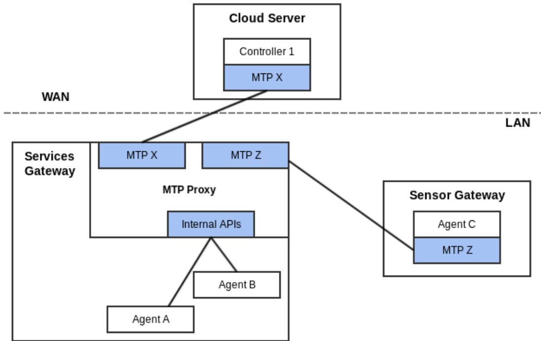
Figure PRX.1: Example of MTP Proxy in LAN with WAN Controller
