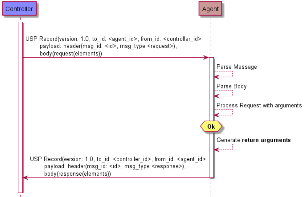
Figure MSG.1 - A successful request/response sequence
