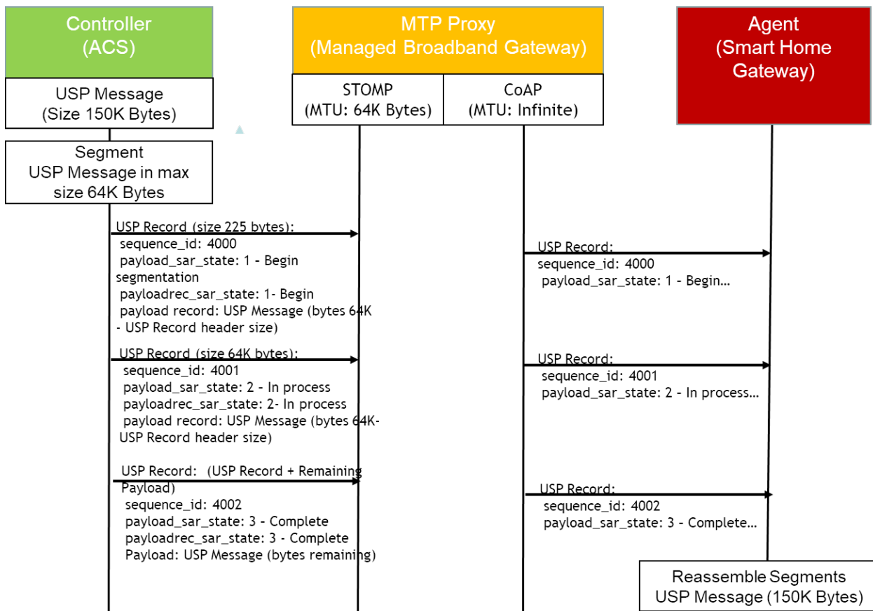
Figure E2E.3 – E2E Segmentation and Reassembly
