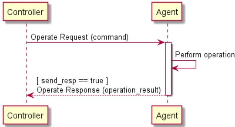
Figure OPR.1 - Operate Message Flow for Synchronous Operations
