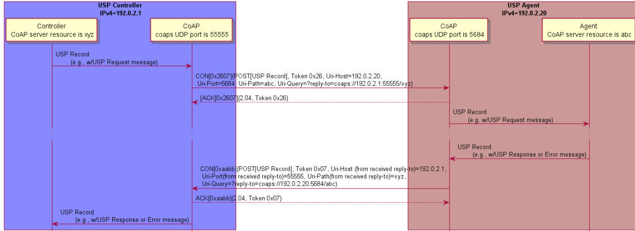
Figure COAP.1 - Example: USP Request/Response over the CoAP MTP
