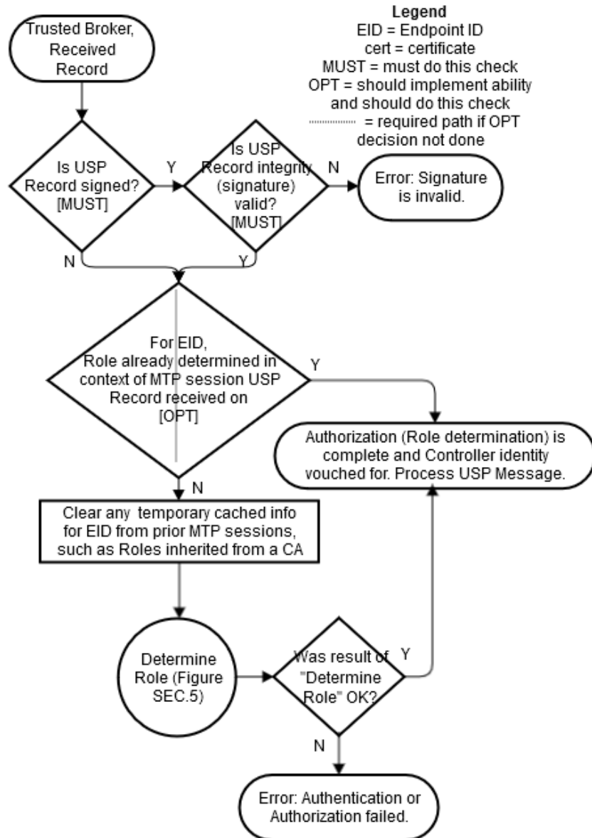
Figure SEC.6 - Trusted Broker with Received Record
