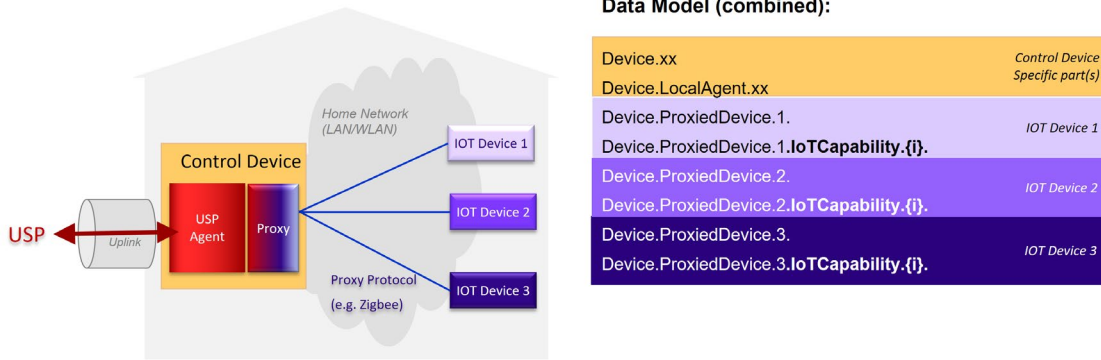
Figure IOT.3 - IoT proxied device model
