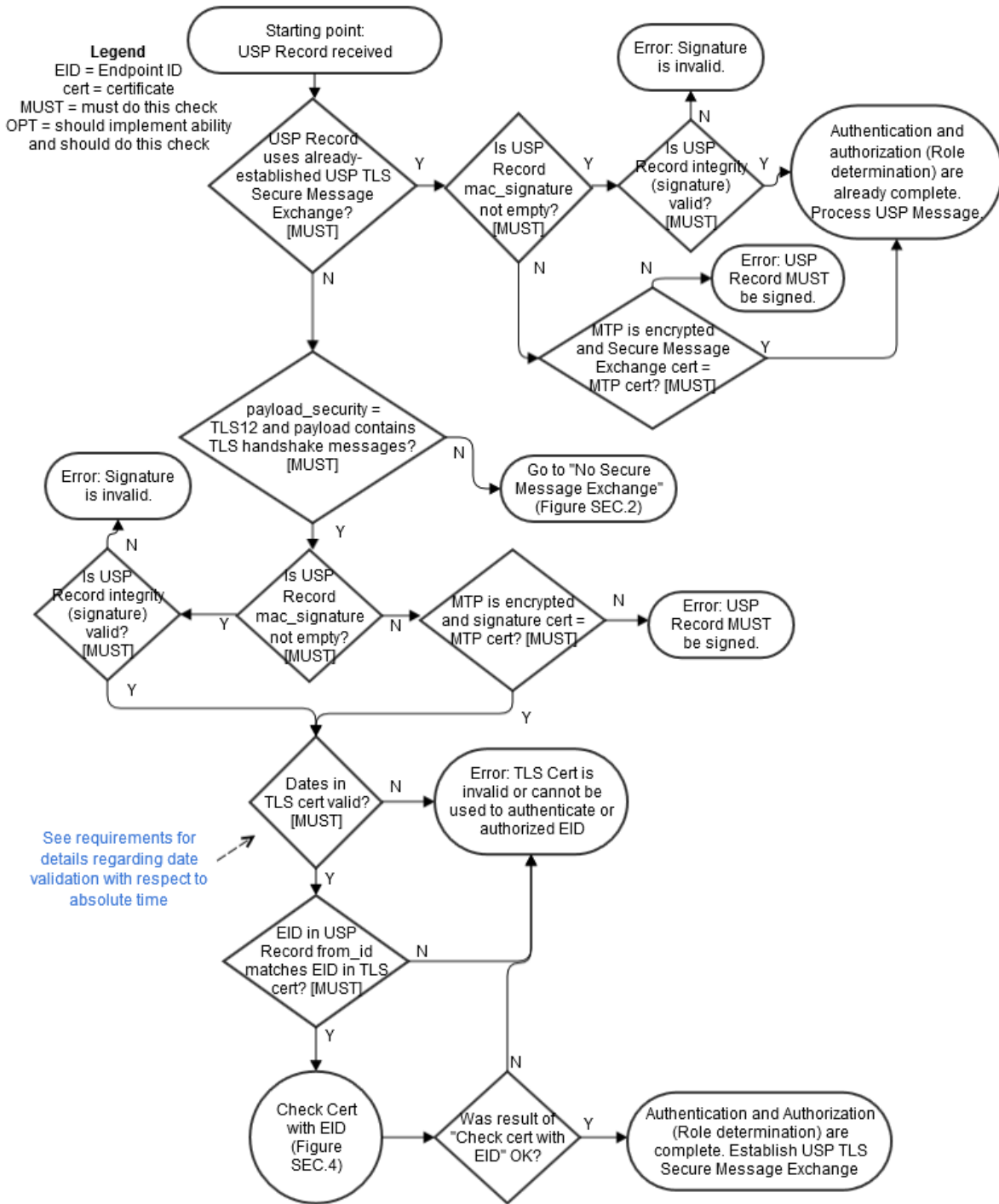
Figure SEC.1 – Receiving a USP Record
