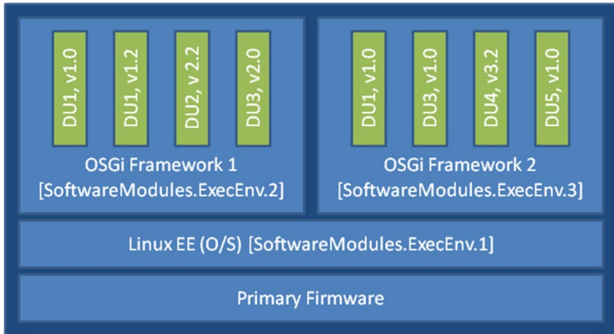
Figure SMM.3 – Possible Multi-Execution Environment Implementation
