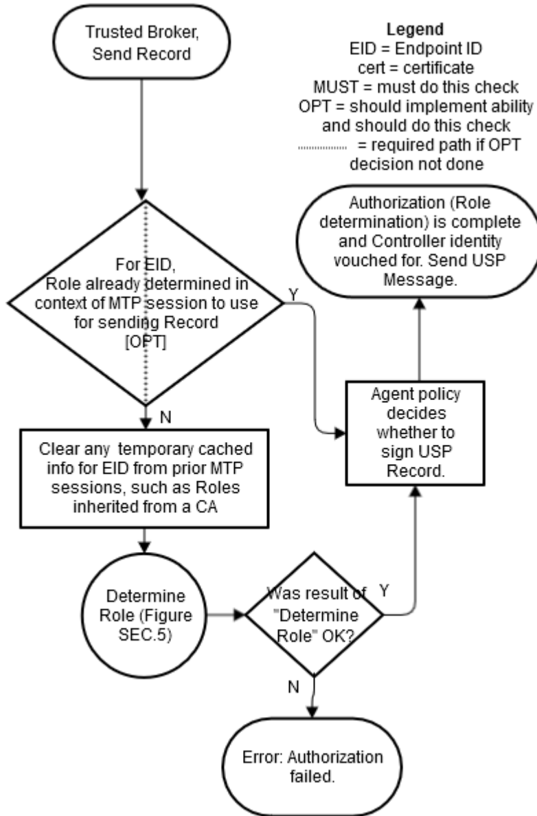
Figure SEC.7 - Trusted Broker Sending a Record
