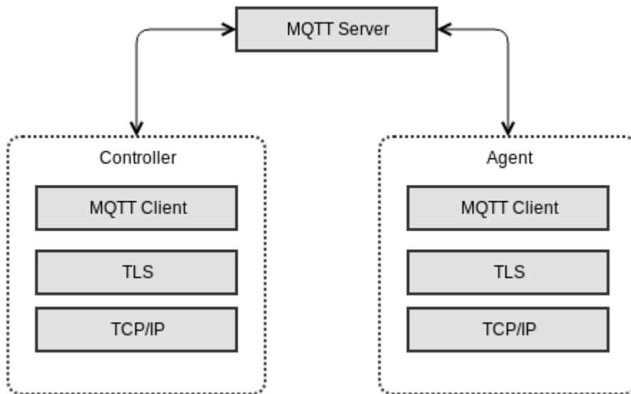
Figure MQTT.1 - USP over MQTT Architecture
