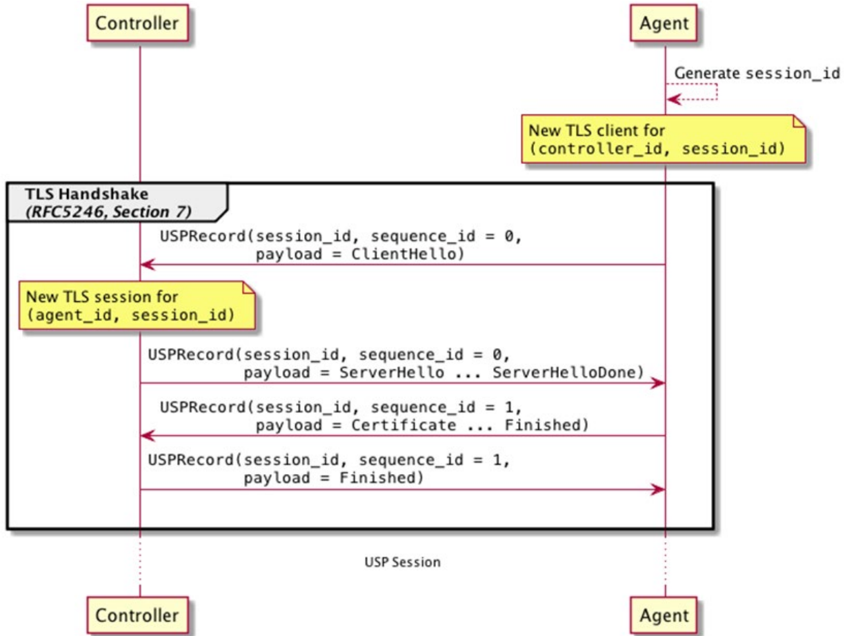
Figure E2E.4 – TLS session handshake
