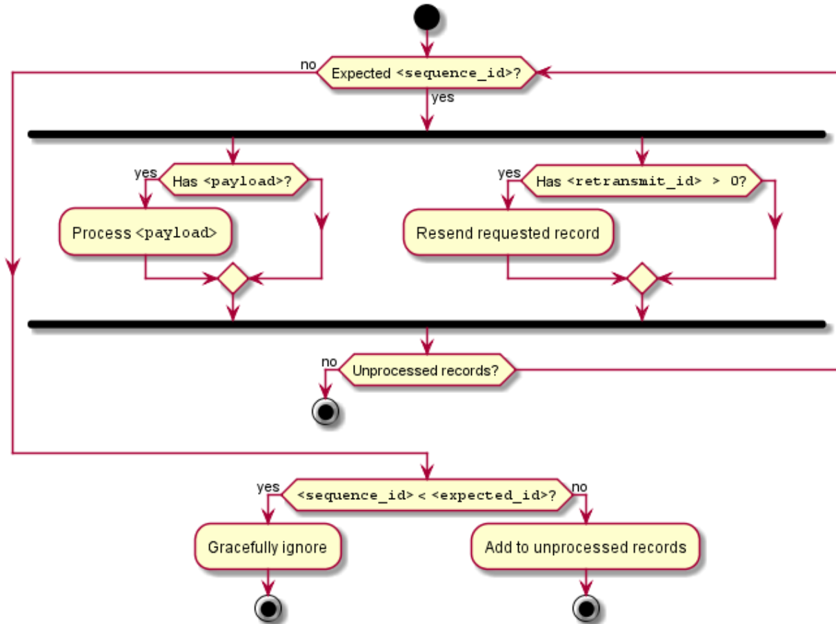
Figure E2E.1 – Processing of received USP Records
