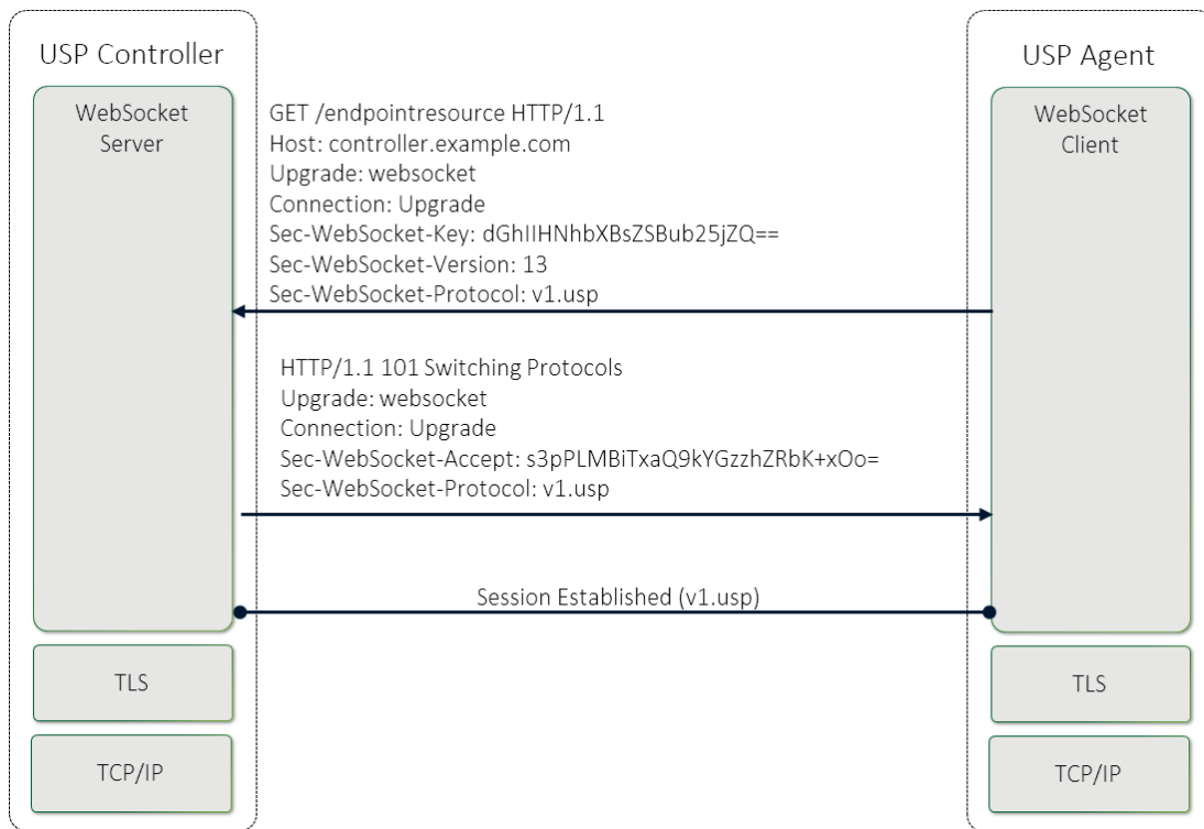
Figure 5 – WS.1 – WebSocket Session Handshake
