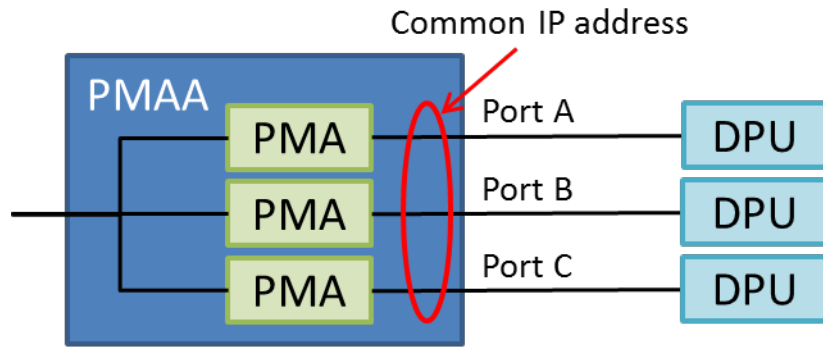
Figure 16-5 PMAs Sharing a Common Address
