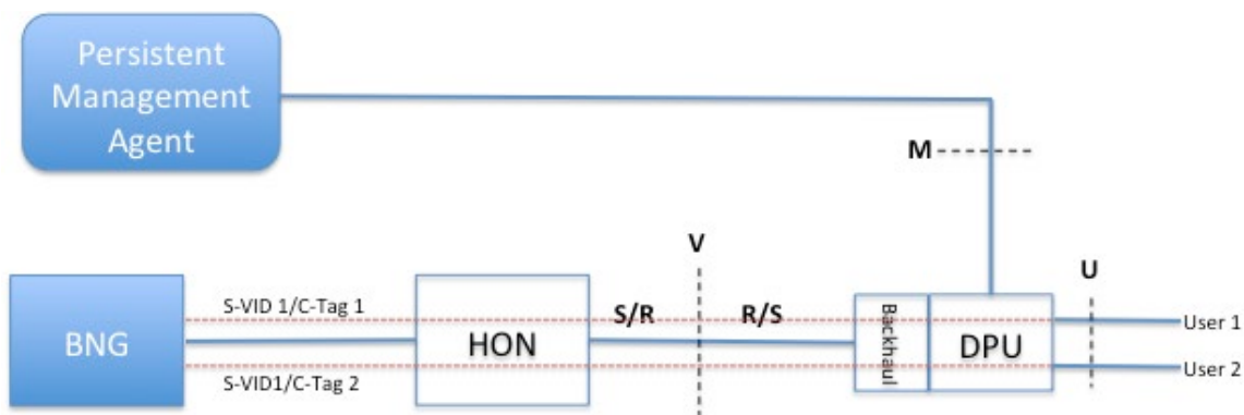
Figure 5-2 Deployment Model 1 (Pt-to-Pt Ethernet/TR-167 Backhaul)
