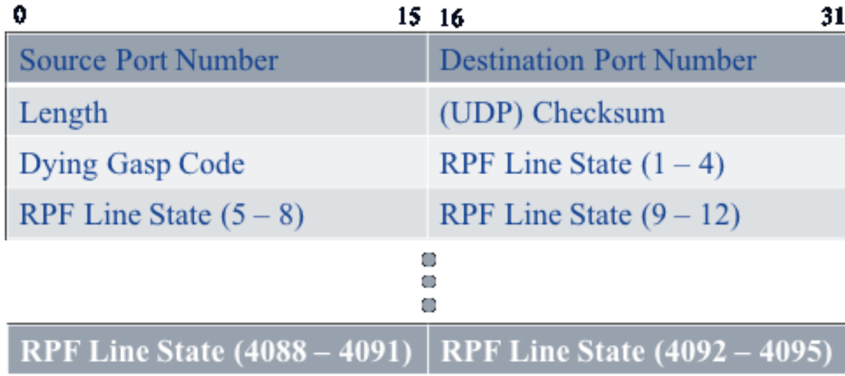
Figure 8-2 Dying Gasp Message
