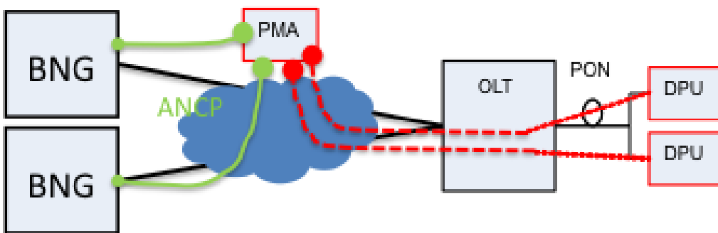
Figure 9-2 ANCP With The PMA External To The HON
