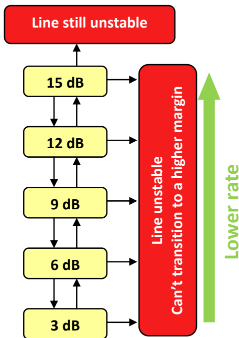
Figure 13: Example of target noise margin (TARSNRM) profiling schemes for AMA
