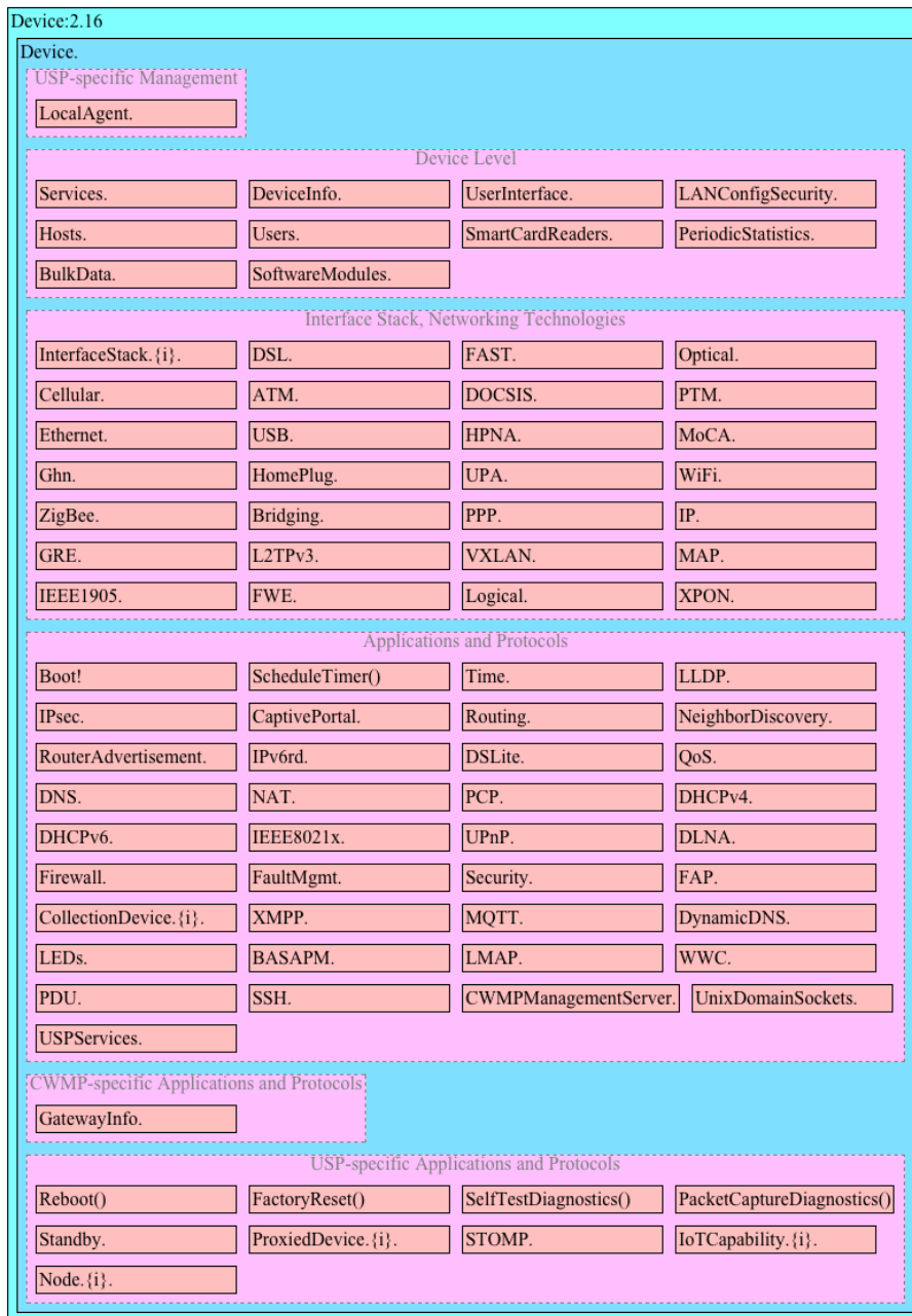
Figure 2: USP-specific Device:2 Data Model Structure – Overview
