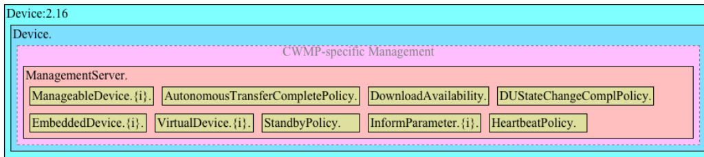
Figure 6: Device:2 Data Model Structure – CWMP Management
