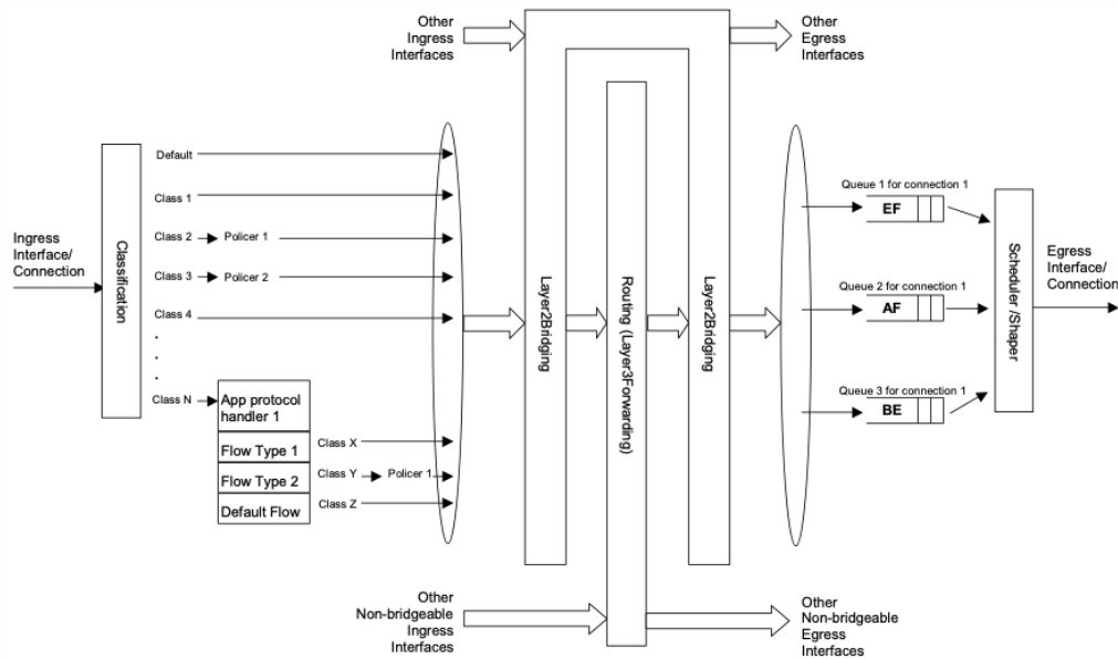
Figure 15: Queuing Model of a Device
