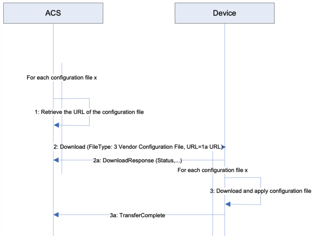
Figure 35: Device User Configuration Restore
