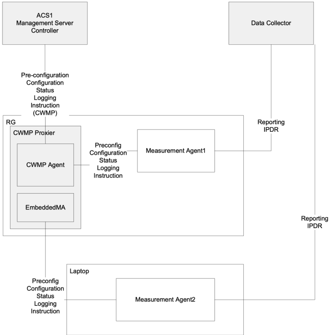
Figure 75: CWMP Proxy Device Deployment
