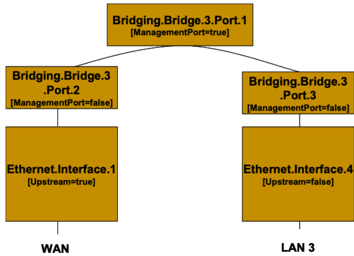
Figure 28: Bridge 3 model
