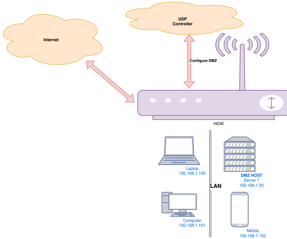
Figure 42: DMZ example
