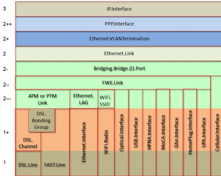
Figure 10: OSI Layers and Interface Objects
