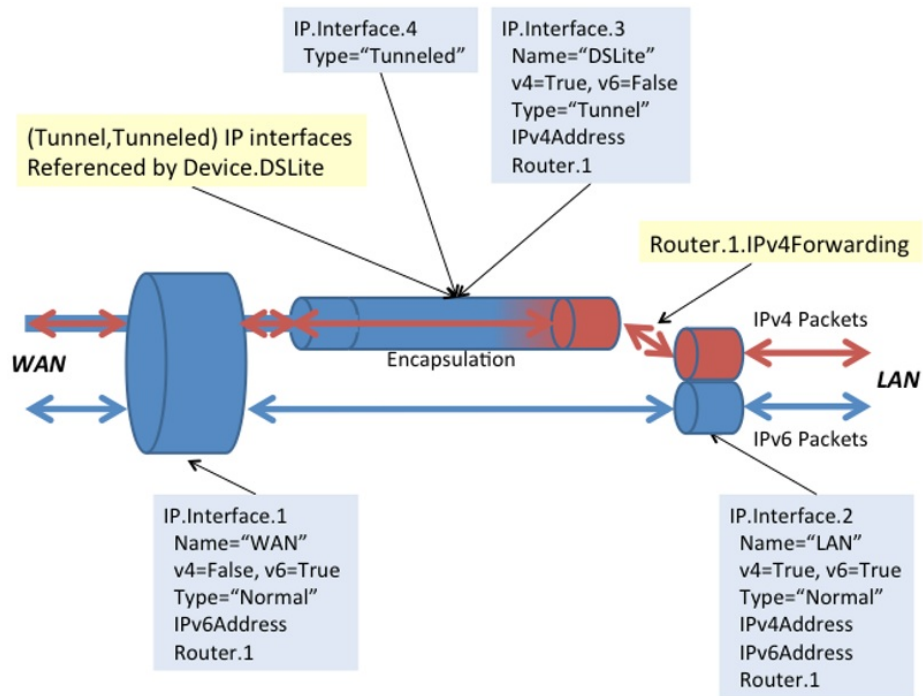
Figure 40: Sample DS-Lite Routing and Forwarding
