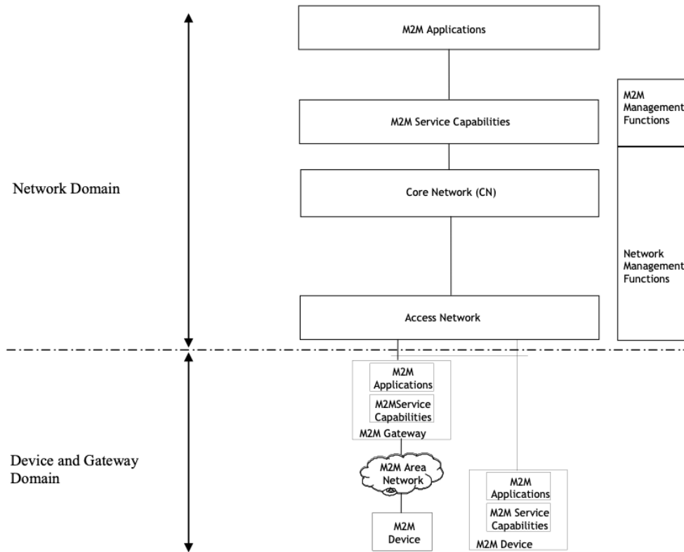
Figure 46: ETSI High Level Functional Architecture
