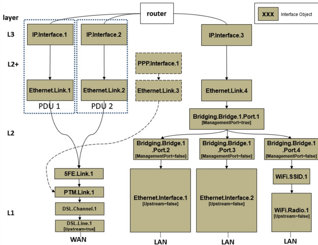
Figure 80: Fixed access only example
