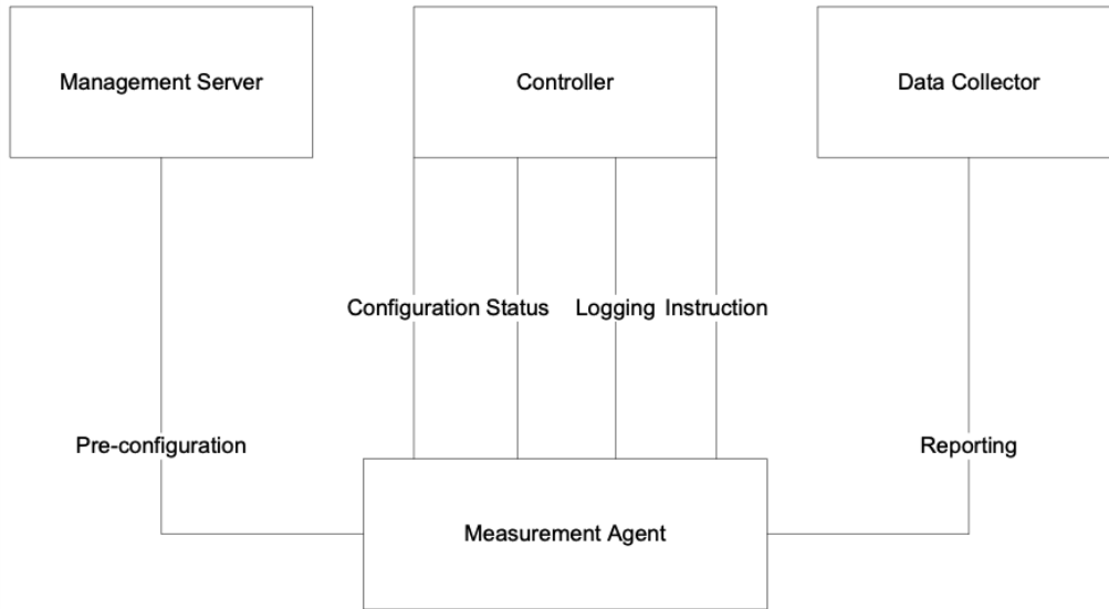
Figure 72: LMAP Framework
