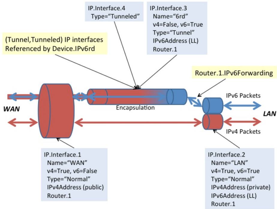
Figure 39: Sample 6rd Routing and Forwarding
