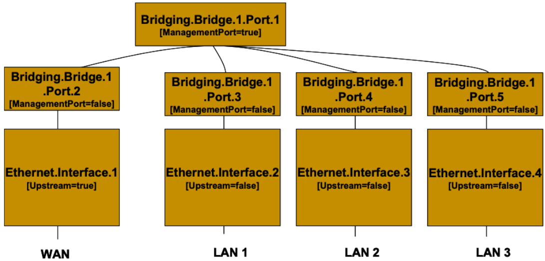
Figure 30: Bridge 1 model (additional Ethernet interfaces)
