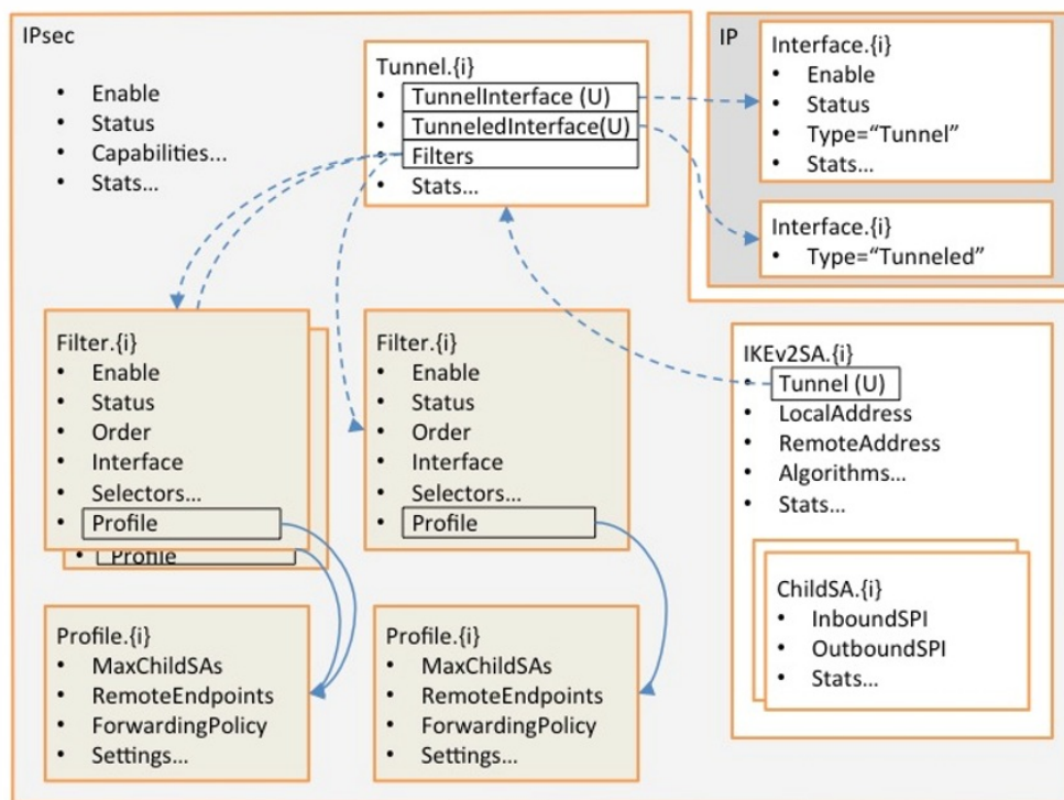
Figure 45: IPsec Data Model Objects
