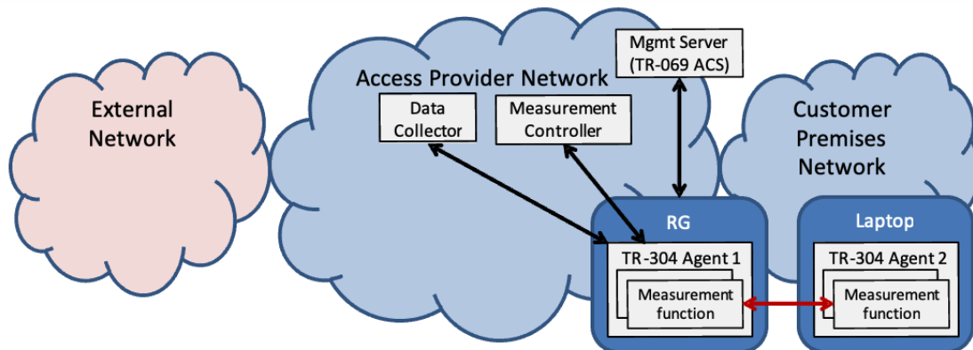
Figure 71: TR-304 Framework
