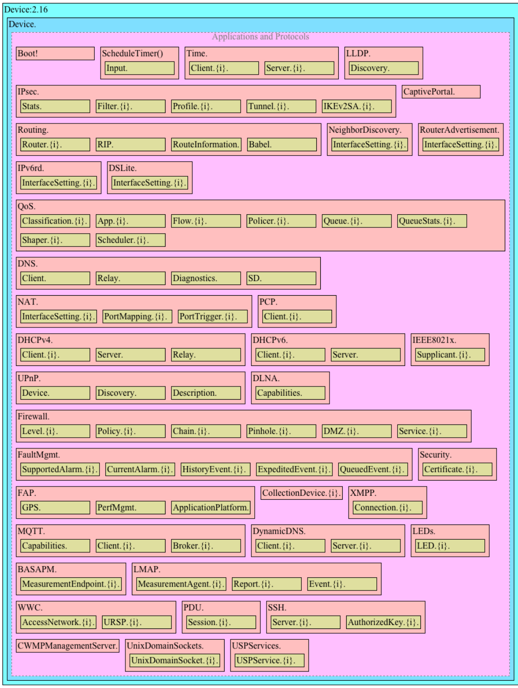
Figure 5: Device:2 Data Model Structure – Common Applications and Protocols
