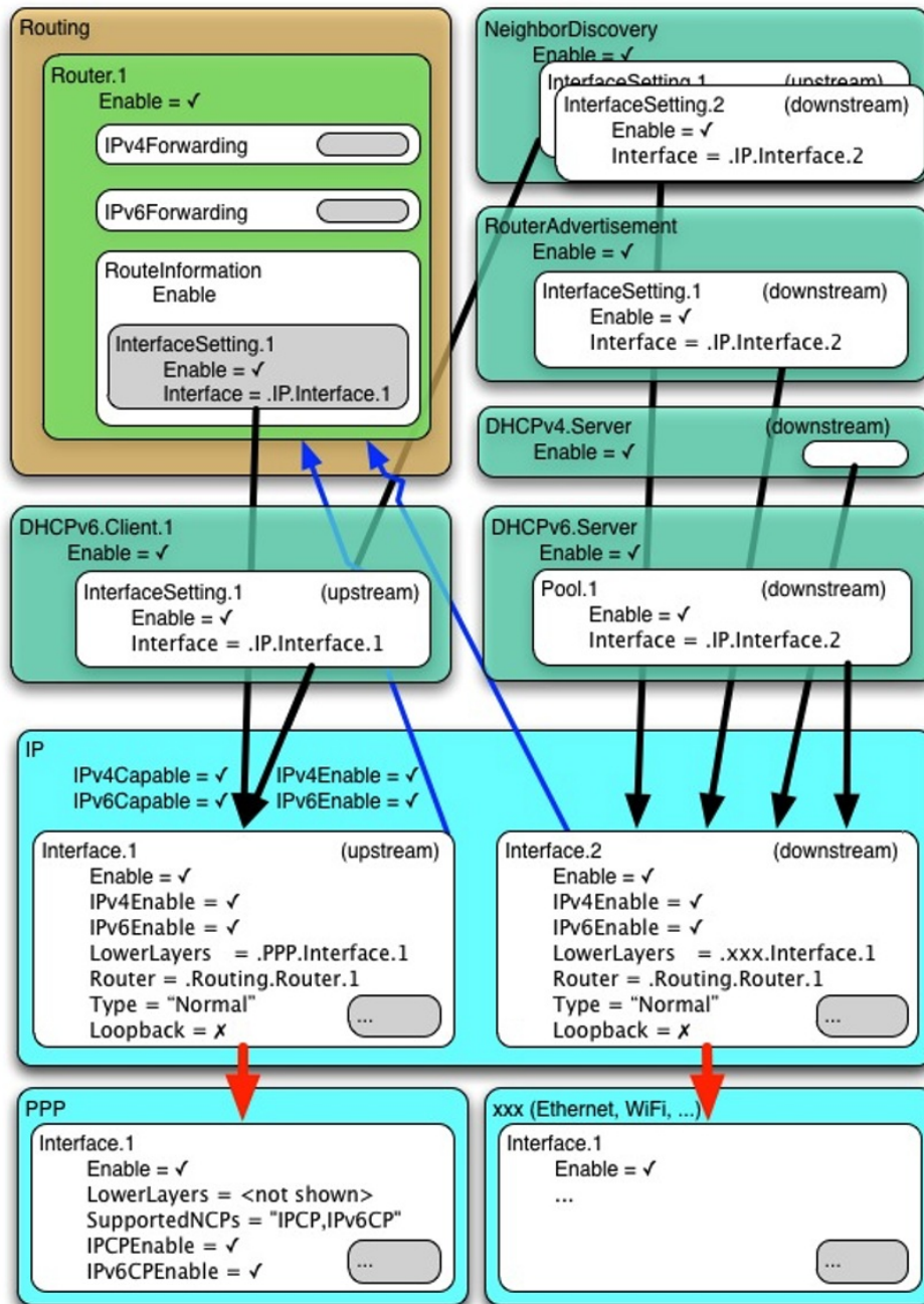
Figure 38: Example IPv6 RG Configuration
