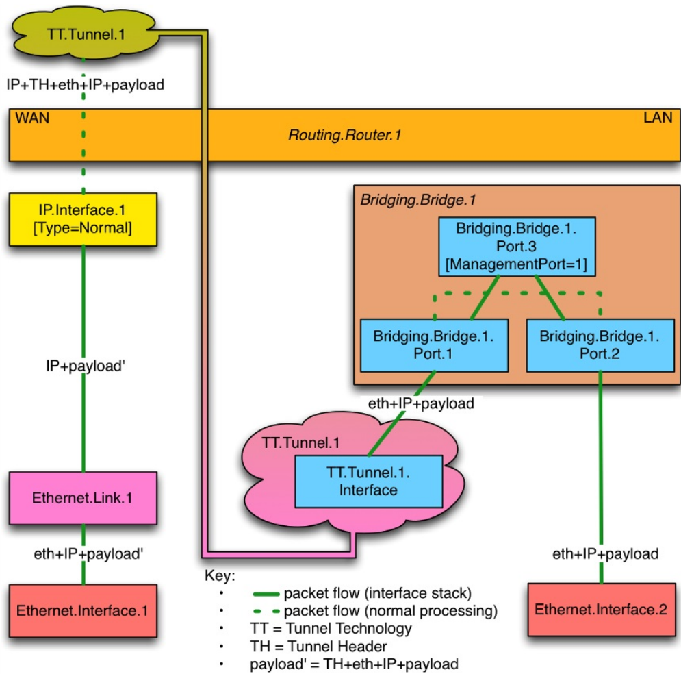
Figure 23: General Layer 2 Tunneling Interface Stack
