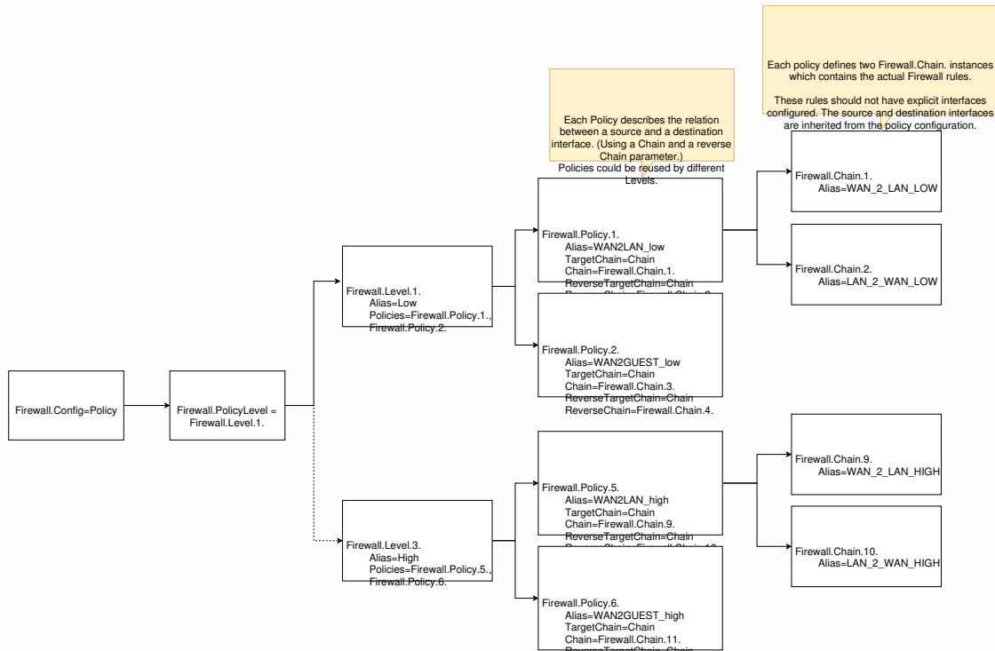
Figure 41: Policy configuration example
