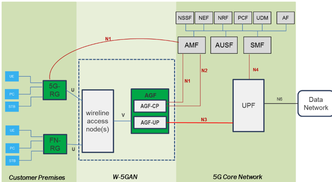
Figure 79: 5G Architecture
