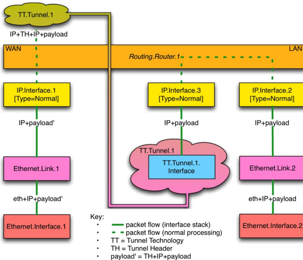
Figure 20: General Layer 3 Tunneling Interface Stack
