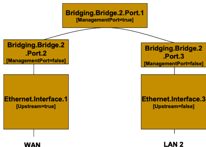
Figure 27: Bridge 2 model
