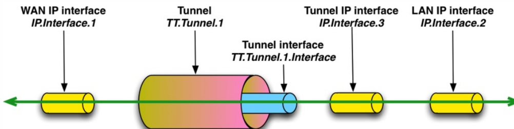
Figure 21: General Layer 3 Tunneling (from Tunneling Overview)
