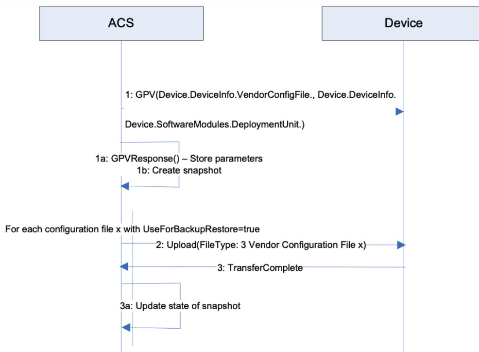
Figure 34: Device User Configuration Backup
