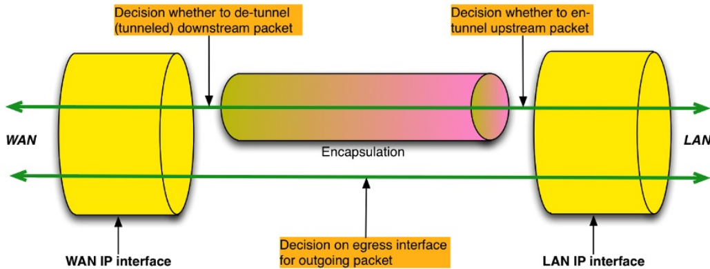
Figure 16: Tunneling Overview
