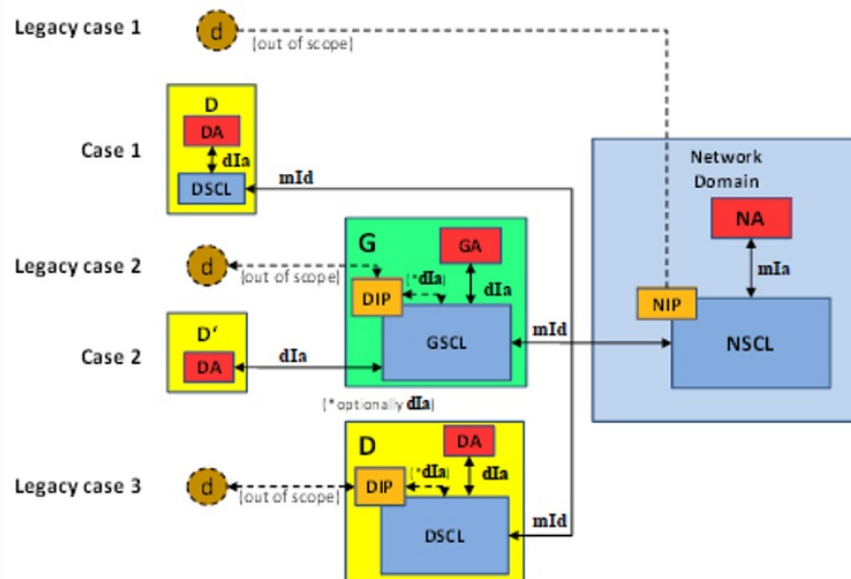
Figure 49: ETSI M2M Devices and Gateways
