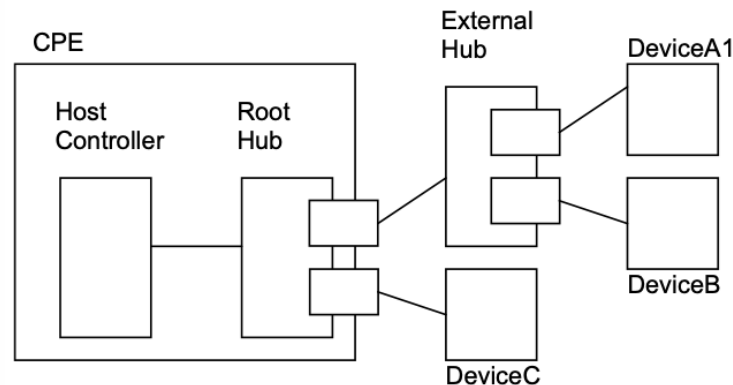
Figure 70: Example USB Host Connections
