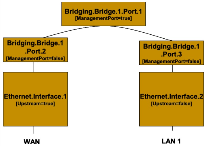
Figure 26: Bridge 1 model
