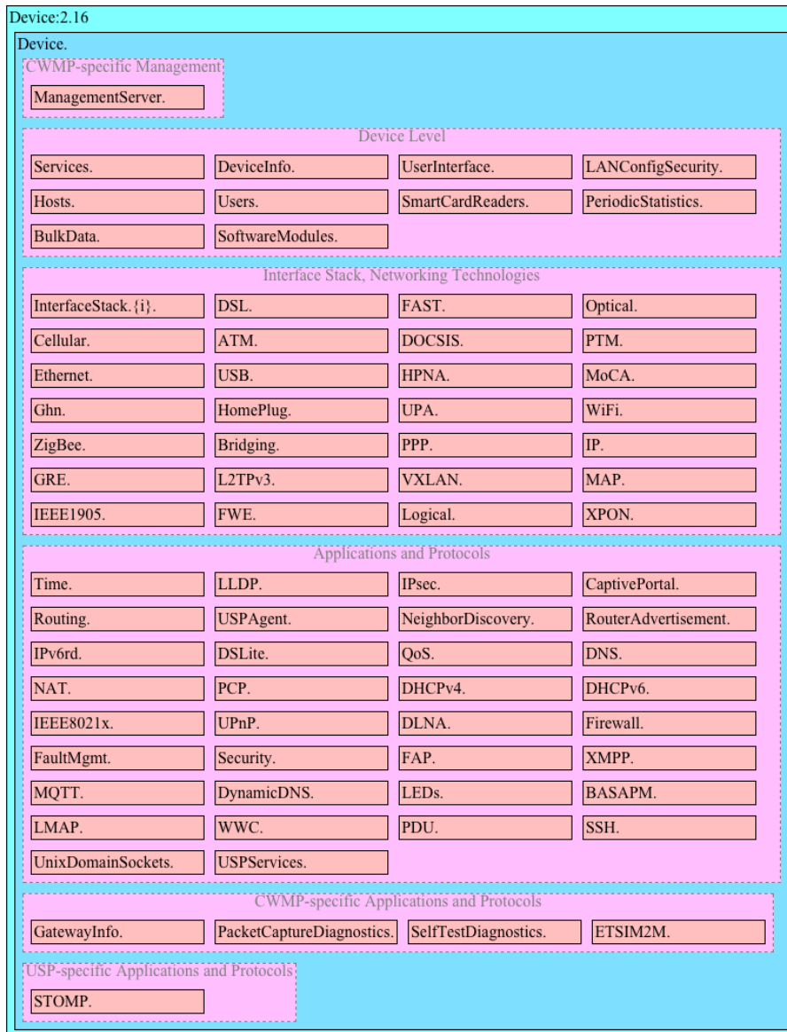
Figure 1: CWMP-specific Device:2 Data Model Structure – Overview
