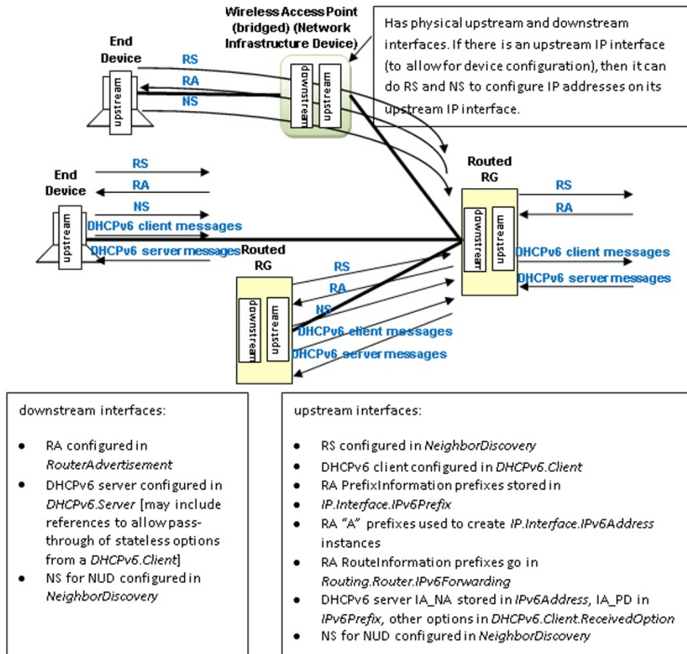
Figure 36: Relationship of Protocols to Data Model
