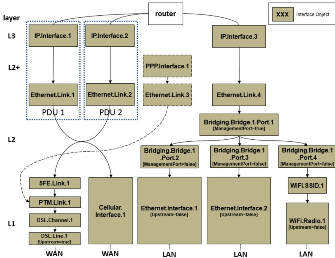
Figure 82: Hybrid access example
