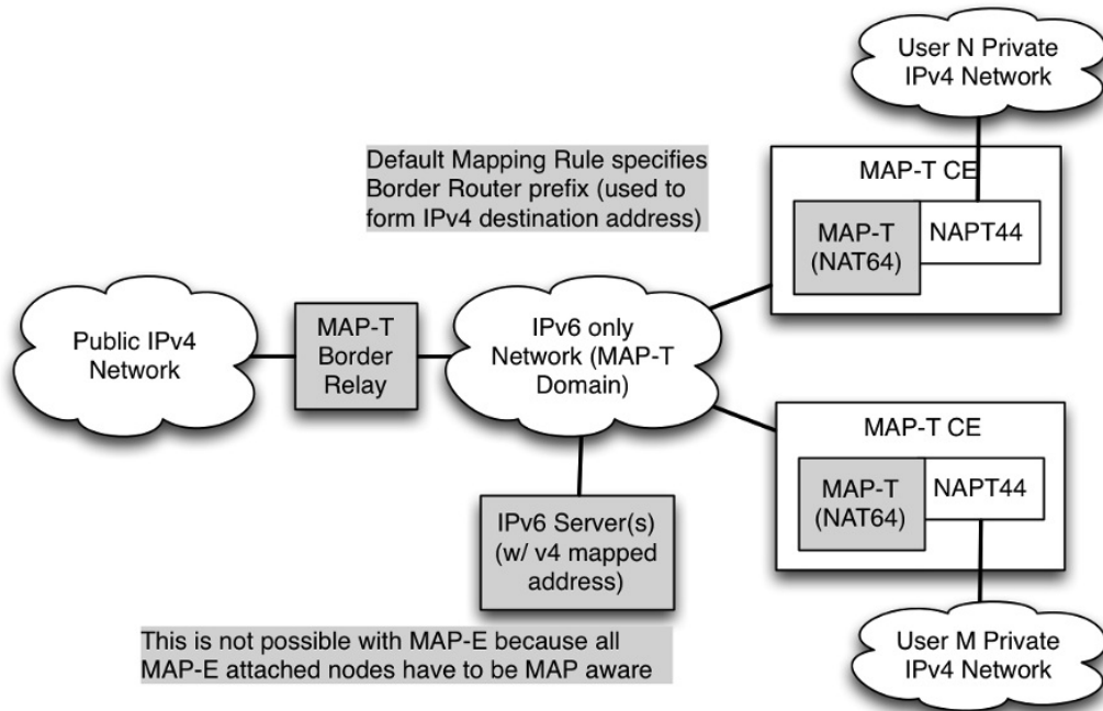
Figure 63: MAP-T Architecture
