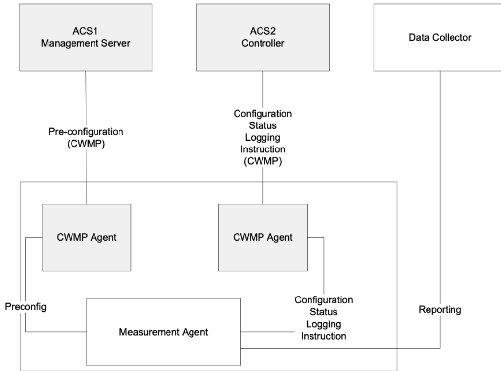
Figure 76: CWMP Multi-ACS Deployment
