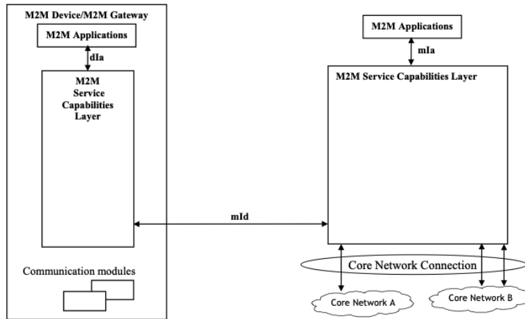
Figure 47: M2M SCL Functional Architecture Framework
