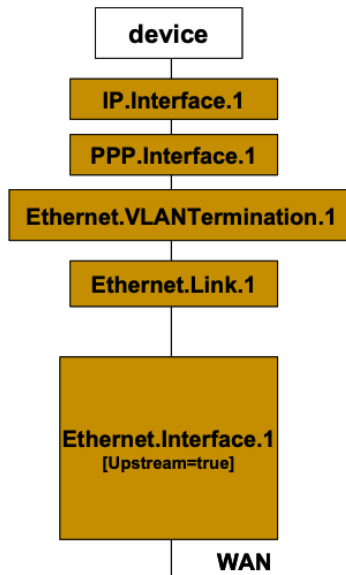
Figure 29: VLAN Termination model
