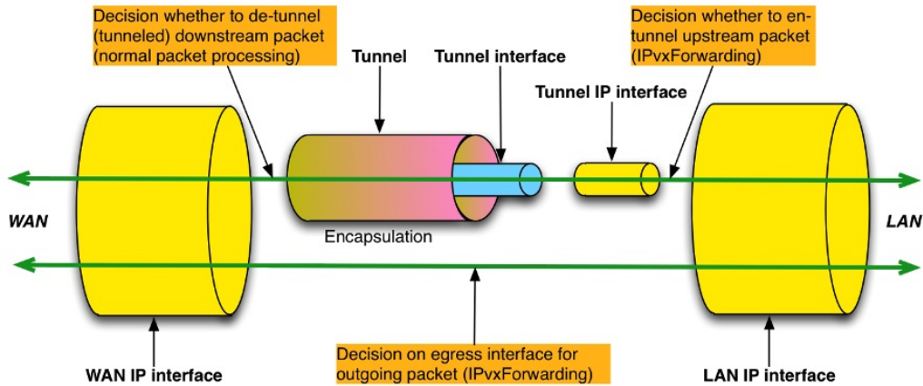
Figure 17: Tunneling Overview (Showing Forwarding Decisions)
