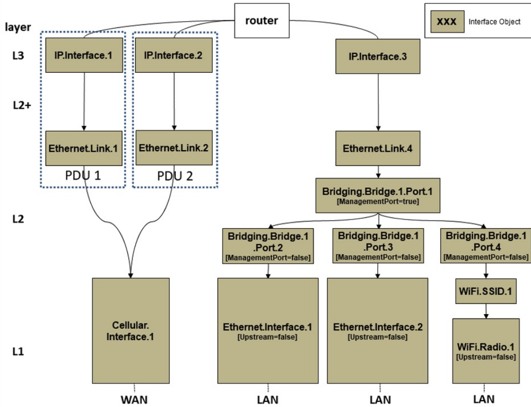
Figure 81: Cellular access only example
