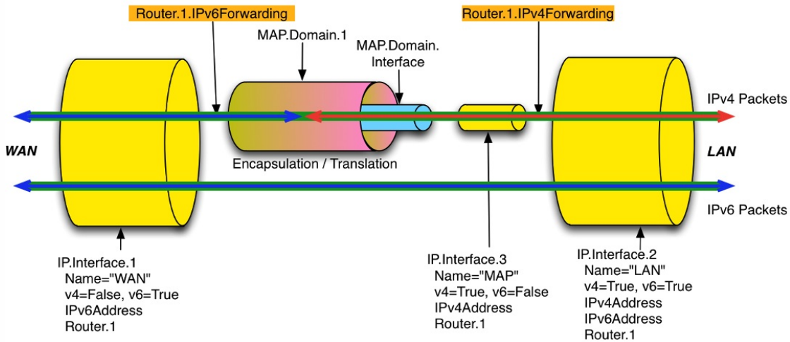
Figure 64: Sample MAP Routing and Forwarding
