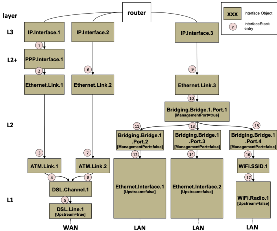
Figure 14: Simple Router Example (Interfaces Visualized)
