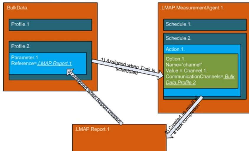
Figure 77: Integration of Bulk Data Profiles with LMAP
