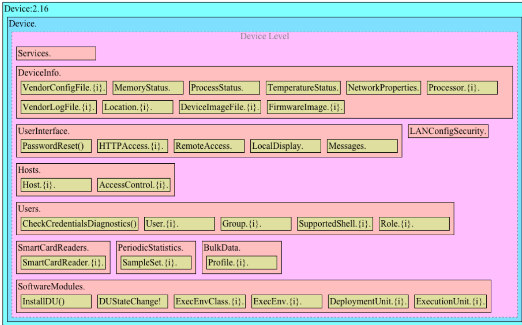
Figure 3: Device:2 Data Model Structure – Device Level
