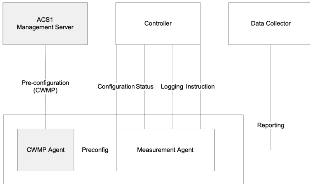
Figure 73: CWMP for Pre-configuration
