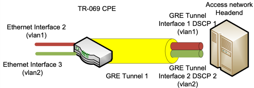
Figure 59: VLAN Traffic over GRE
