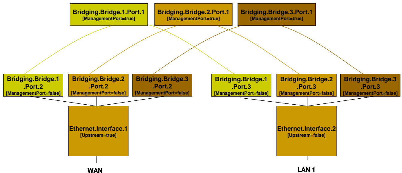
Figure 27 – Bridge 1,2,3 model
