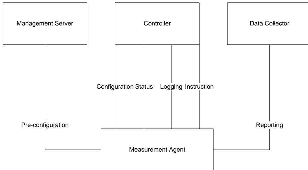
Figure 62 – LMAP Framework
