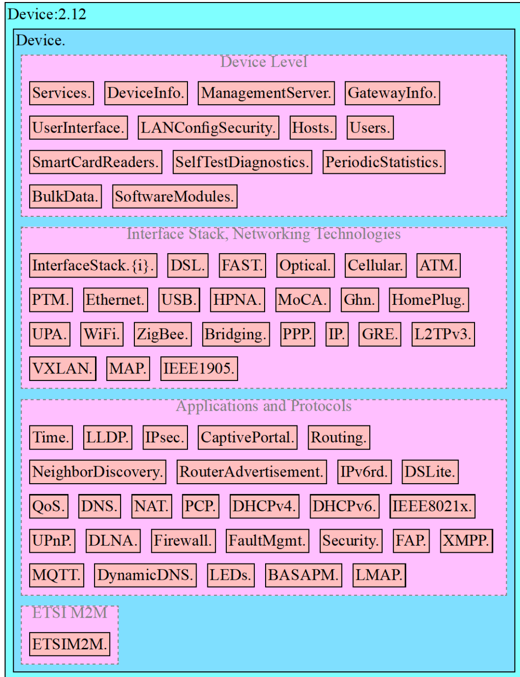
Figure 1 – Device:2 Data Model Structure – Overview
