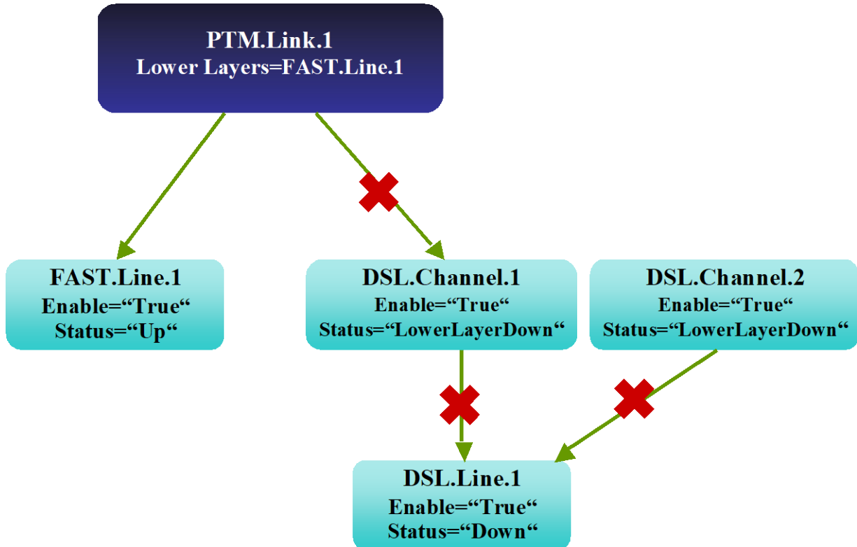
Figure 57 – PTM Link for FAST mode Line
