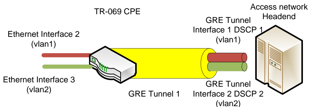
Figure 49 – VLAN Traffic over GRE
