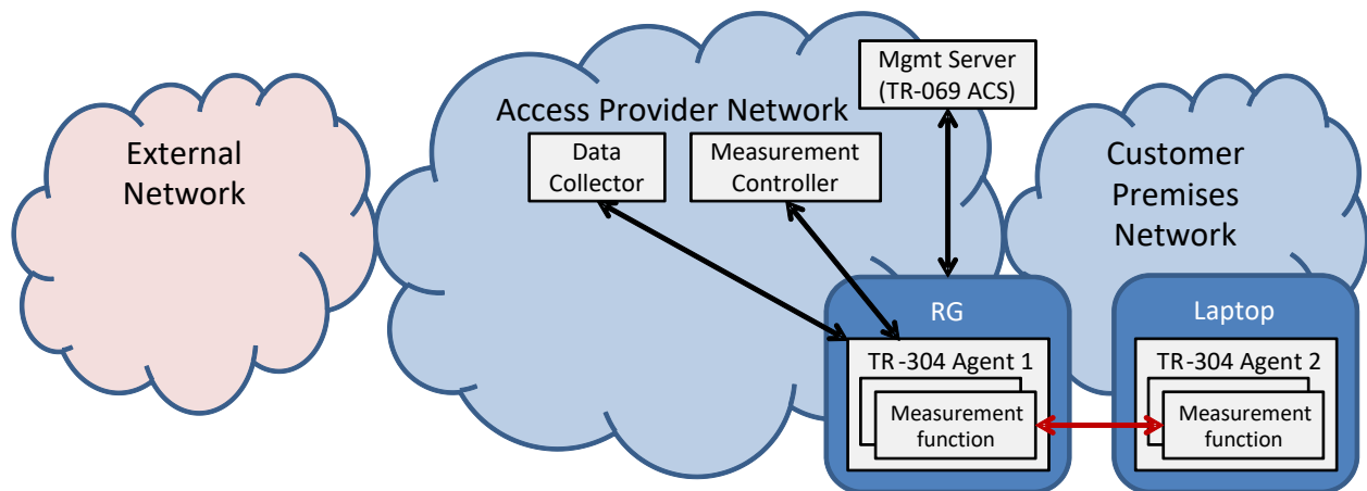
Figure 61 – TR-304 Framework
