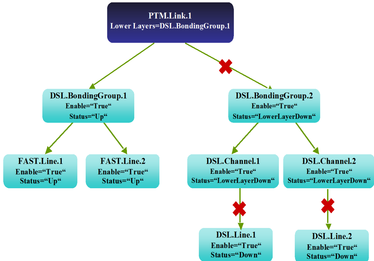
Figure 58 – PTM Link Bonding Groups for FAST mode Lines
