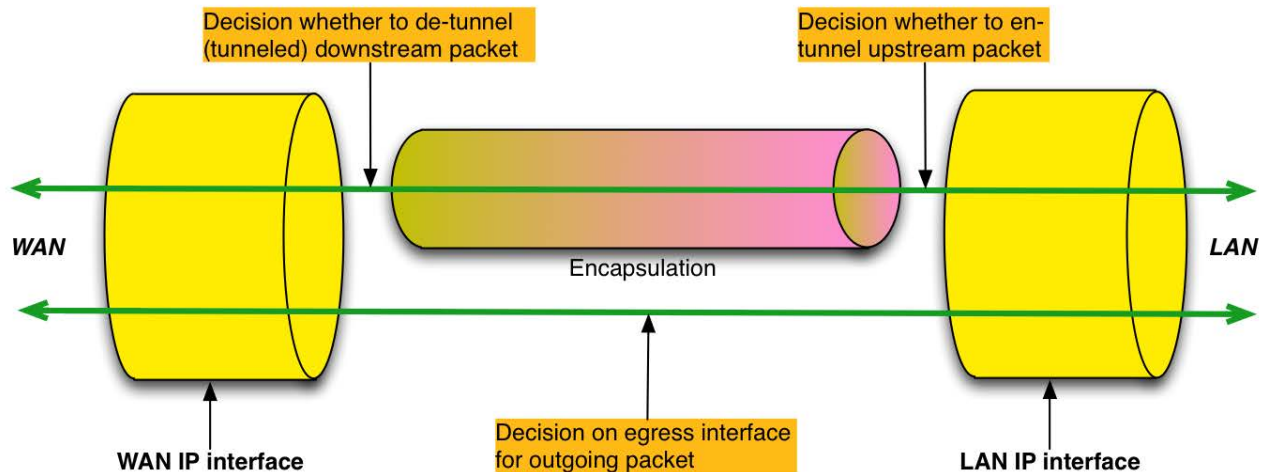
Figure 11 – Tunneling Overview
