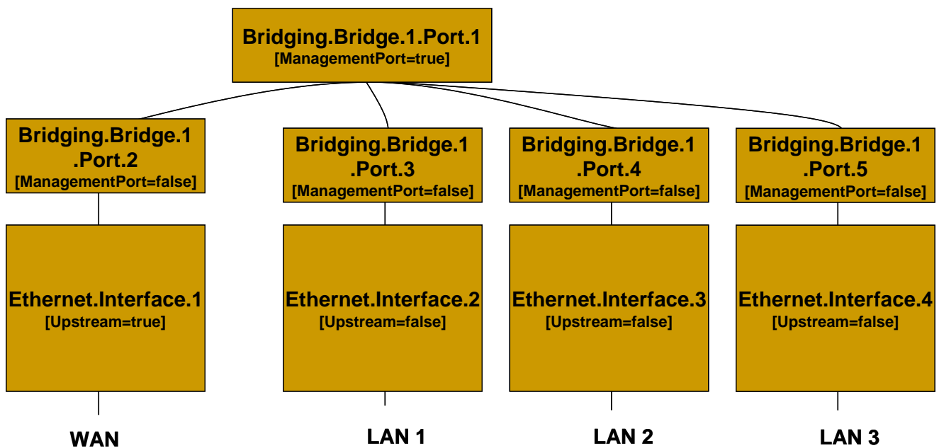
Figure 25 – Bridge 1 model
