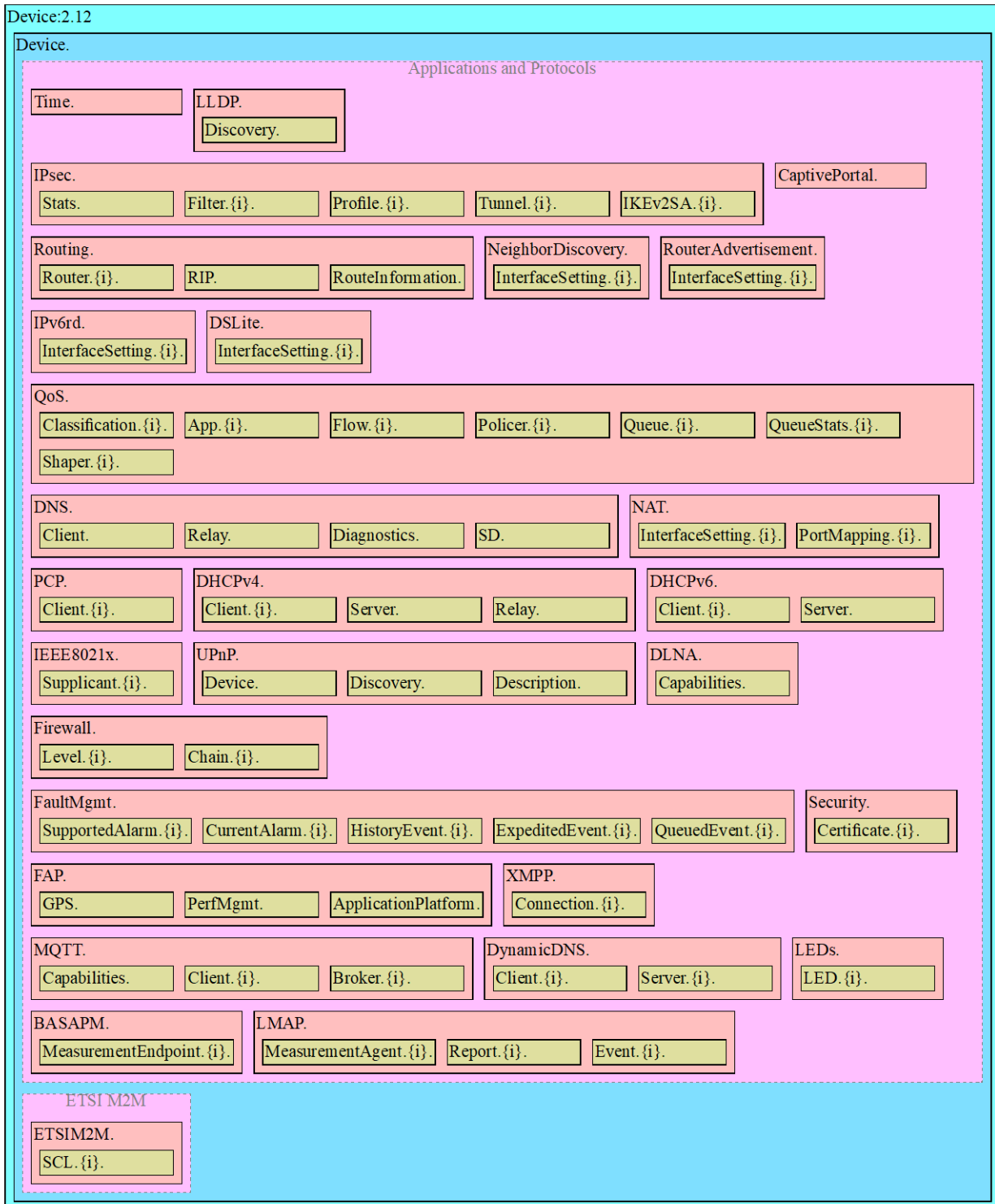
Figure 4 – Device:2 Data Model Structure – Applications and Protocols
