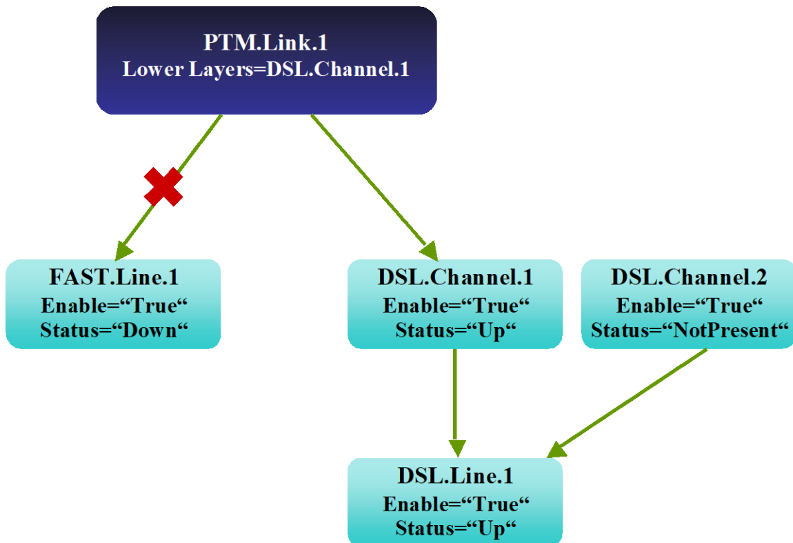
Figure 56 – PTM Link for DSL mode Line
