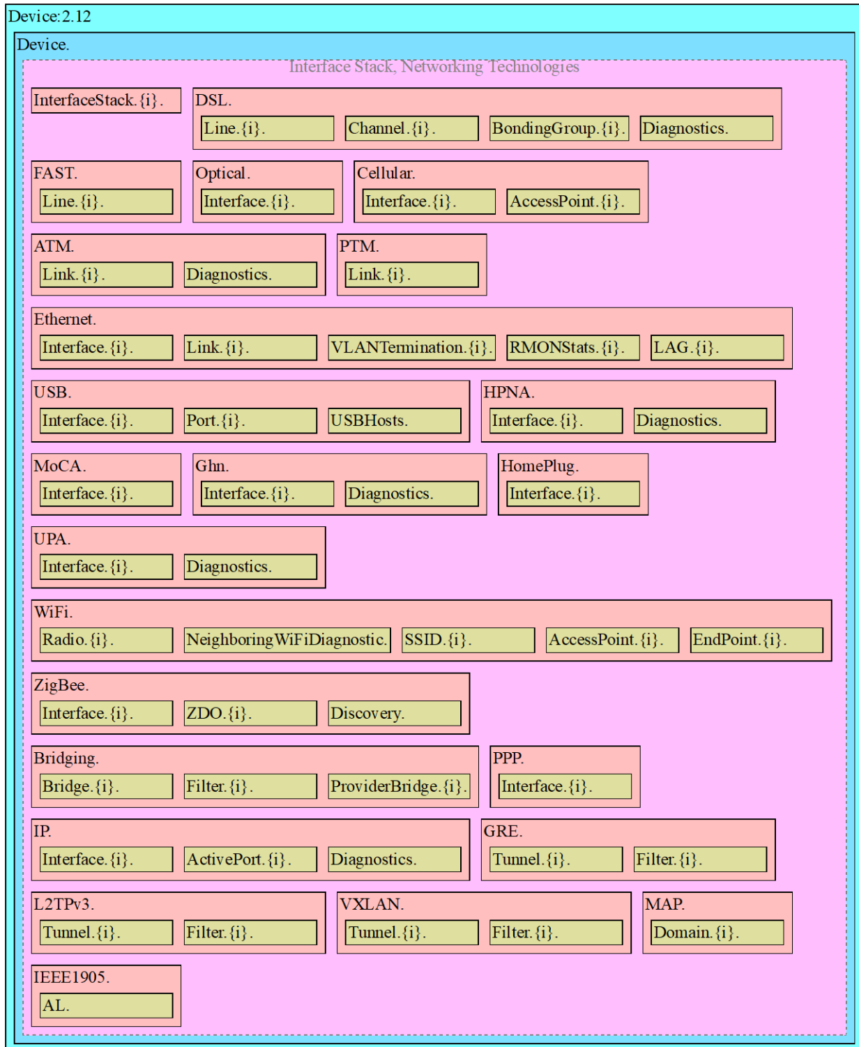
Figure 3 – Device:2 Data Model Structure – Interface Stack and Networking Technologies
