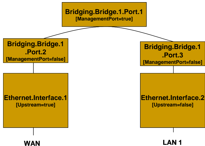
Figure 21 – Bridge 1 model
