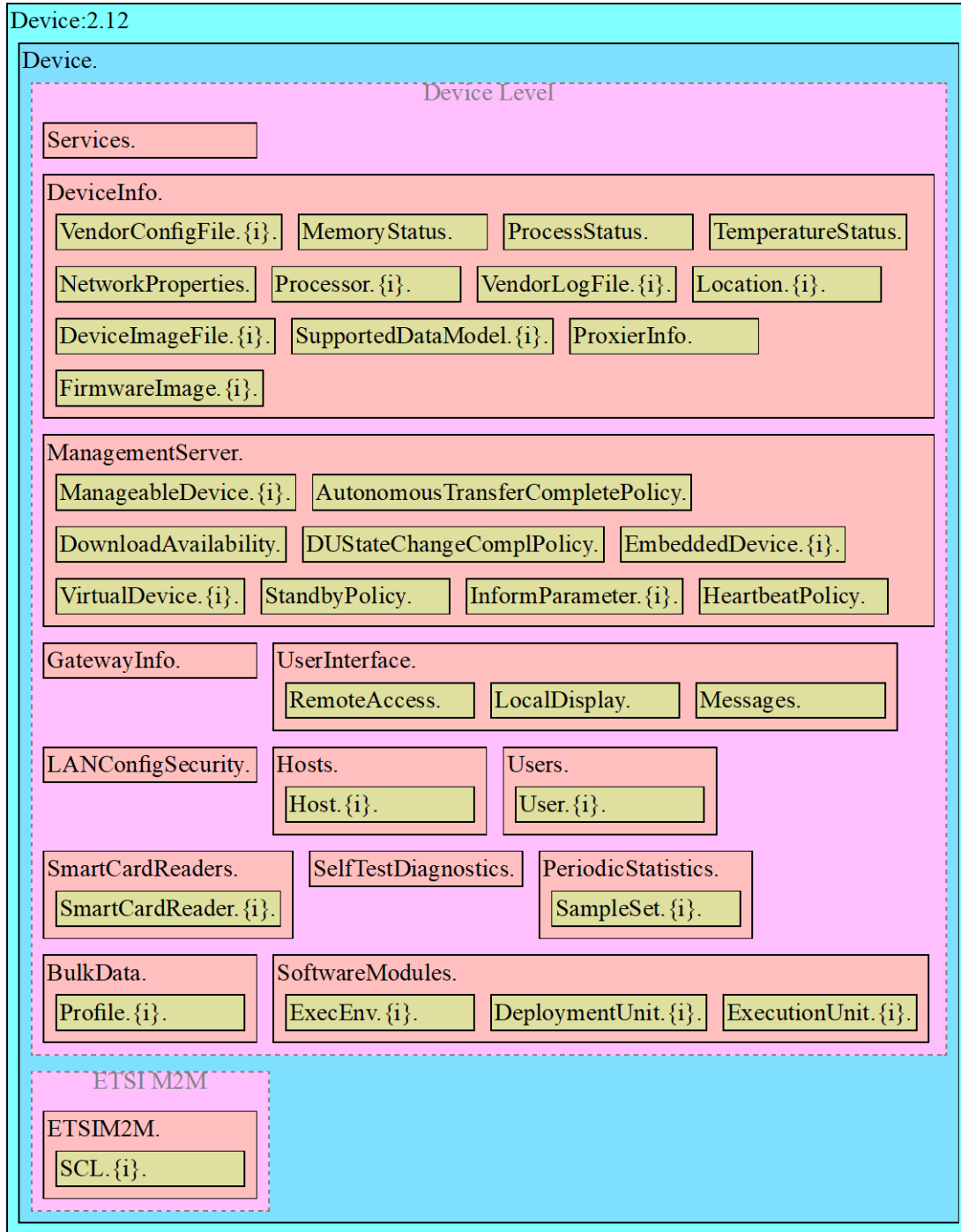
Figure 2 – Device:2 Data Model Structure – Device Level
