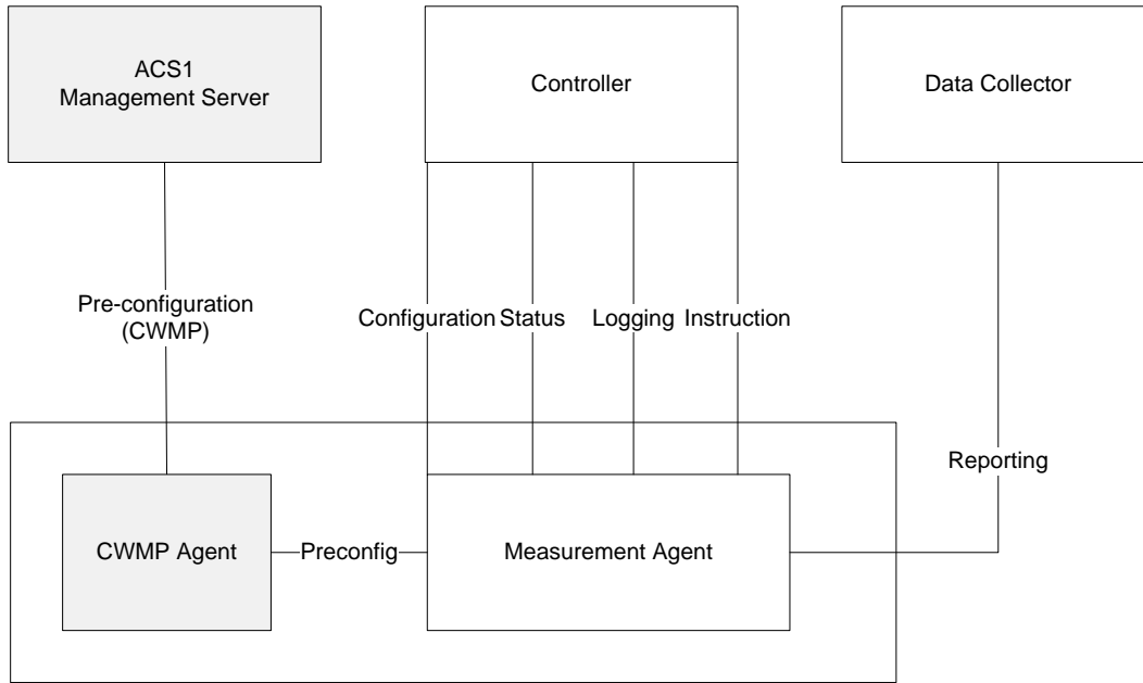
Figure 63 – CWMP for Pre-configuration
