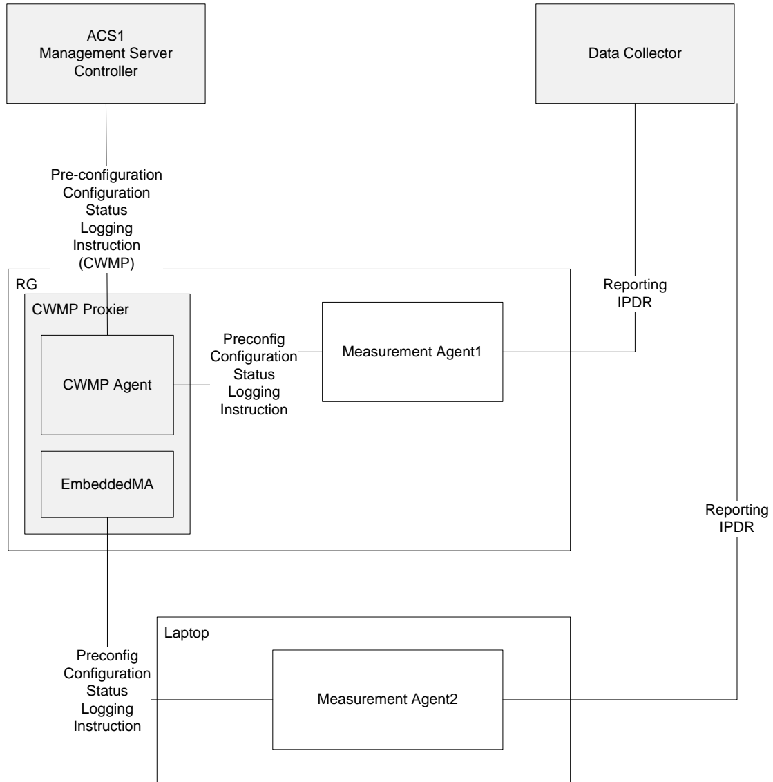
Figure 65 – CWMP Proxy Device Deployment
