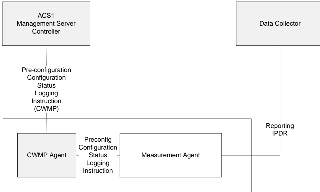
Figure 64 – CWMP for Control and Pre-configuration, IPDR for Reporting
