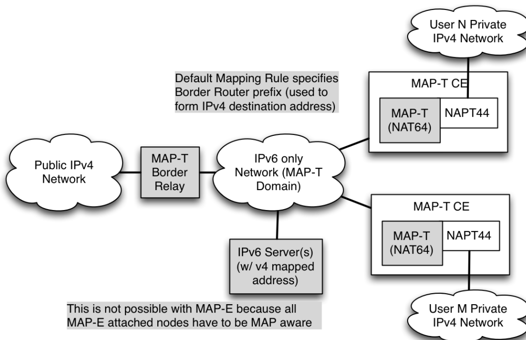
Figure 53 – MAP-T Architecture
