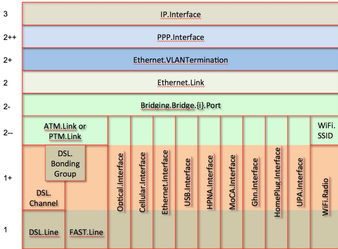
Figure 5 – OSI Layers and Interface Objects 2 3
