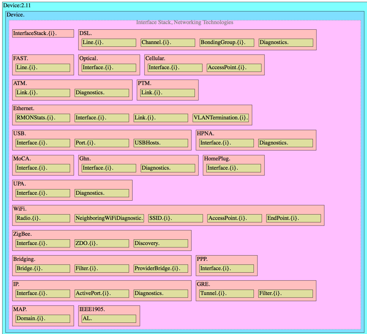
Figure 3 – Device:2 Data Model Structure – Interface Stack and Networking Technologies
