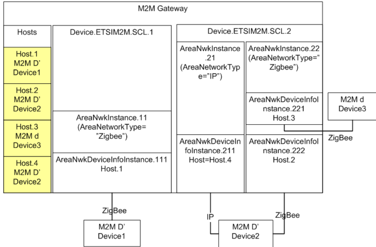
Figure 40 - Example M2M Network
