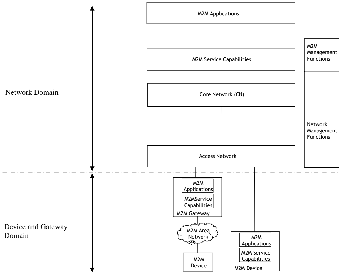
Figure 36 – ETSI High Level Functional Architecture
