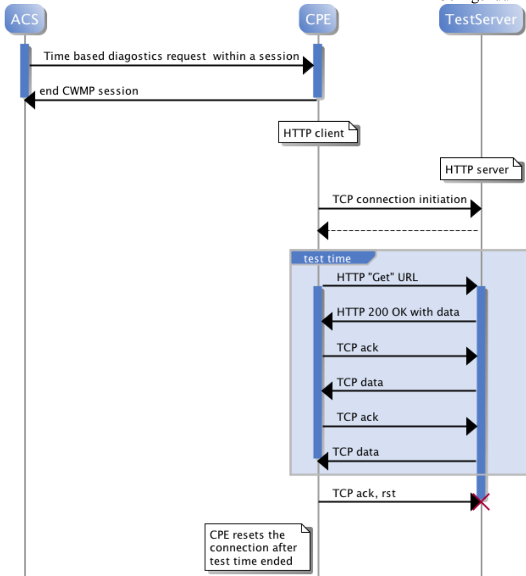
Figure 8 CPE Time-based throughput diagnostics using HTTP/FTP transport.
