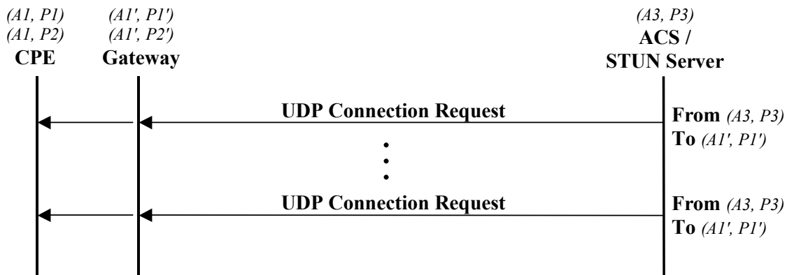
Figure 15 – UDP Connection Request
