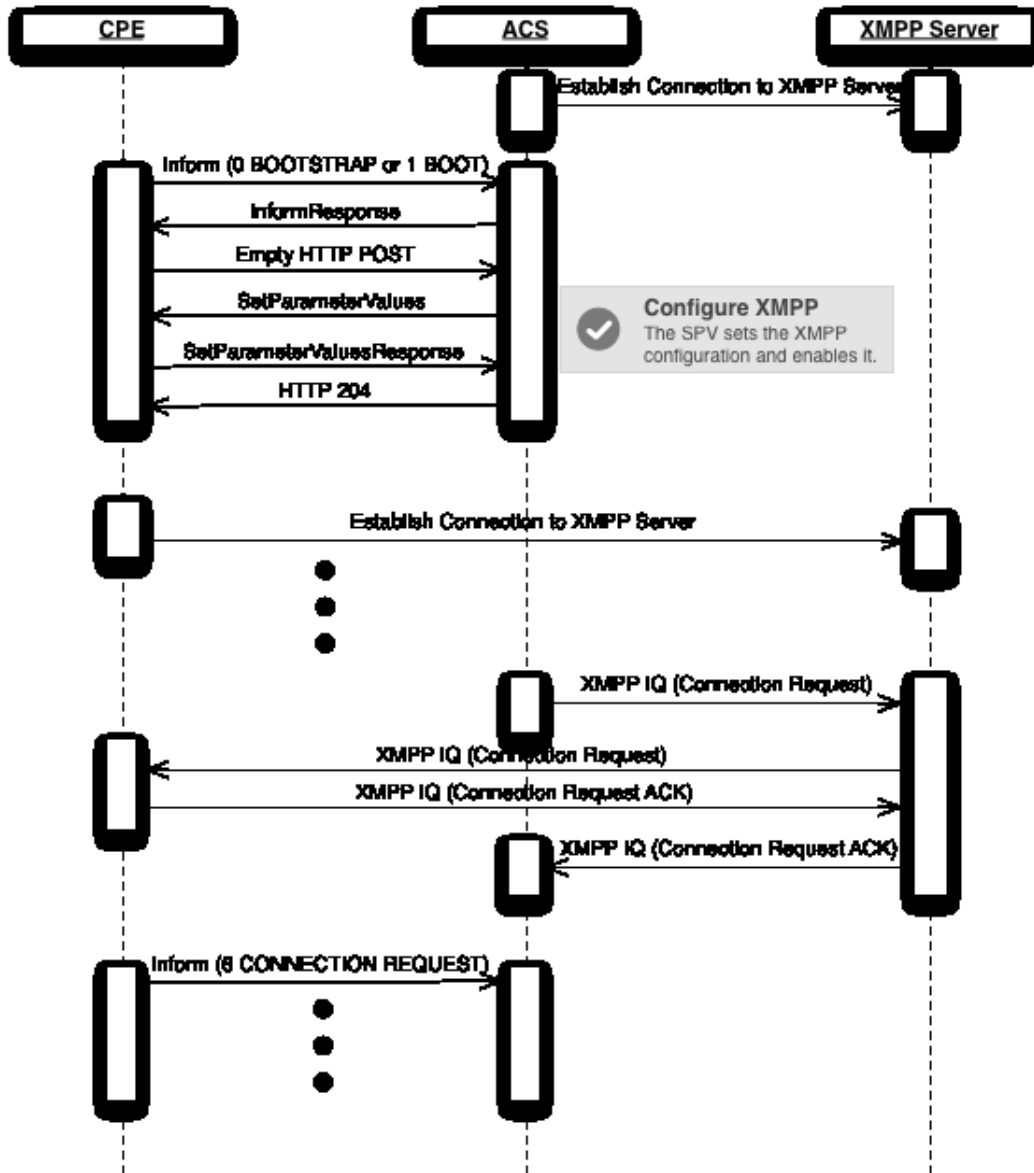
Figure 18 – XMPP Connection Request Message Sequence
