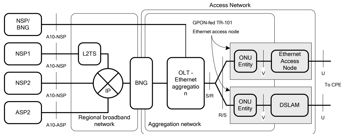
Figure 1 – Network architecture for Ethernet-based G-PON aggregation (TR-167 issue 2 [21])
