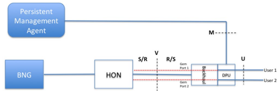
Figure 5-3 Deployment Model 2 (TR-156 Backhaul)
