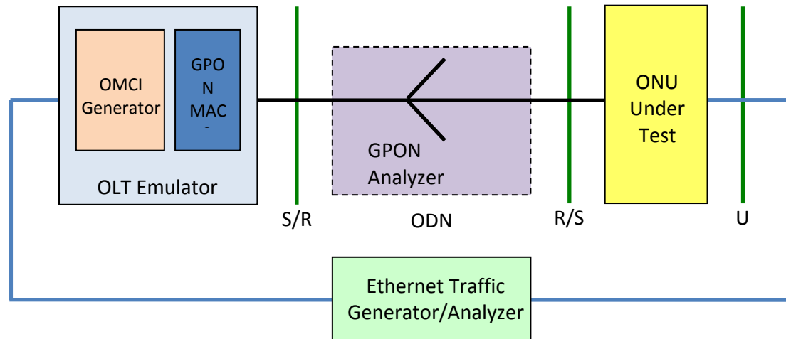
Figure 1 - Basic test setup for ONU conformance testing
