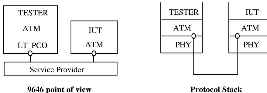
Figure 1. Test Configuration for an End System
