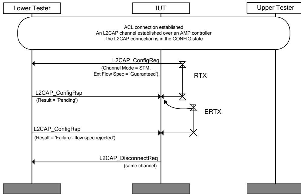
Figure 4.128: L2CAP/LSC/BV-12-C [Remote Failed on Guaranteed, AMP Channel]
