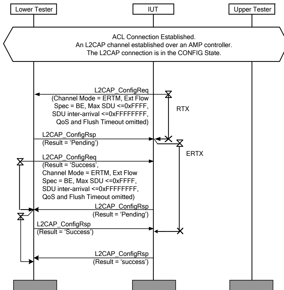
Figure 4.123: L2CAP/LSC/BV-07-C [Normal Lock Step Configuration Process for Best Effort, AMP Channel]
