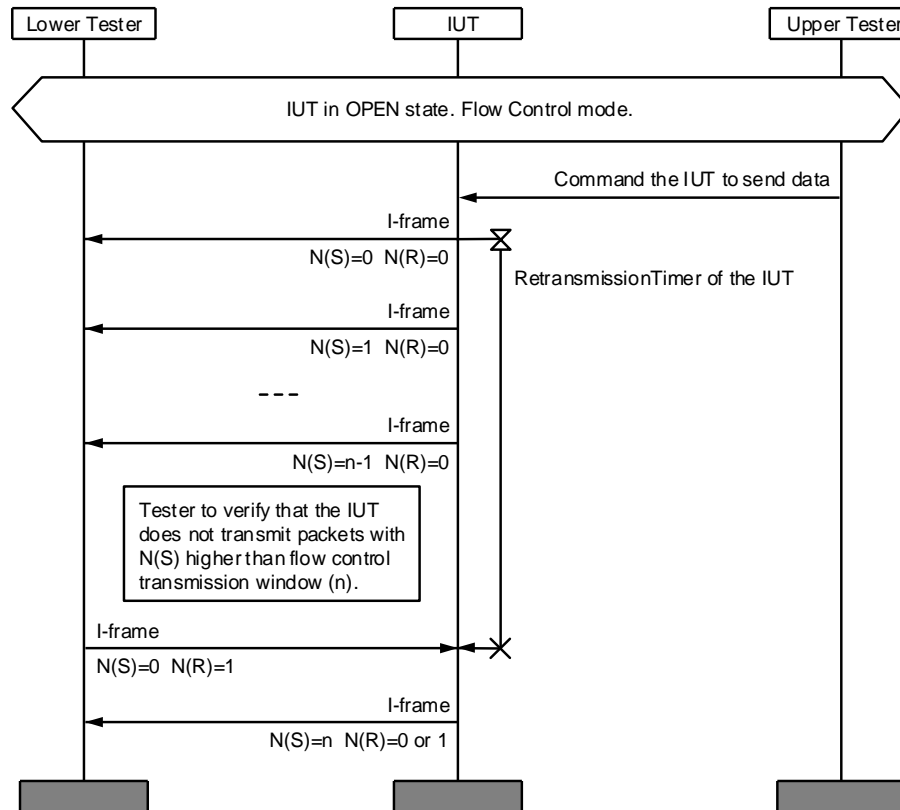
Figure 4.40: L2CAP/COS/FLC/BV-03-C [Resume Flow on I-frame Ack]
