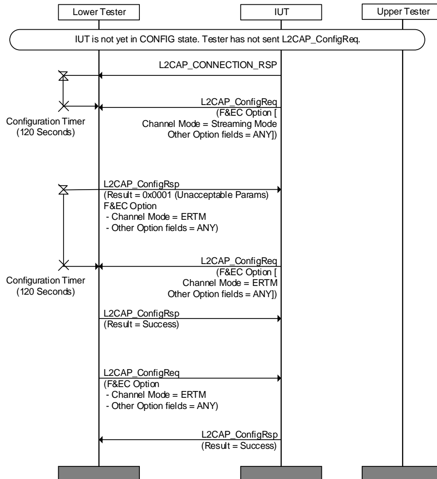
Figure 4.67: L2CAP/CMC/BV-14-C [Failed Configuration of Streaming Mode when use of the mode is optional and ERTM is proposed by the Lower Tester]
