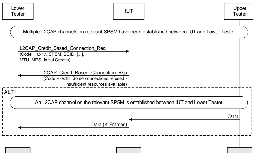
Figure 4.202: L2CAP Credit Based Connection Response – refused due to insufficient resources
