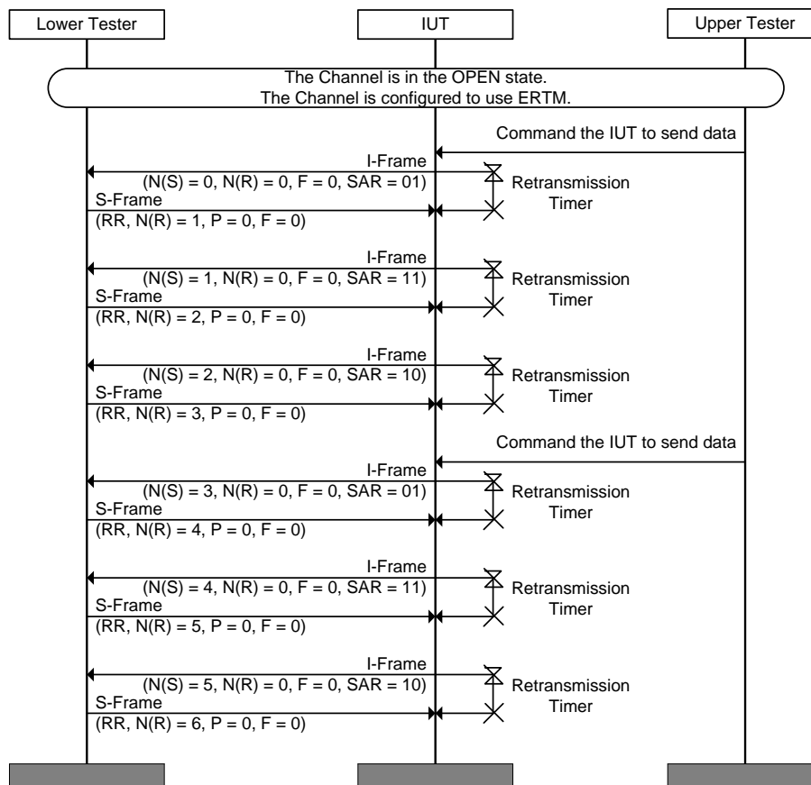
Figure 4.176: L2CAP/ECF/BV-08-C [Transmit I-Frames using Extended Control Field and SAR]
