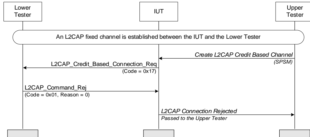
Figure 4.192: L2CAP Credit Based Connection Request – Legacy Peer
