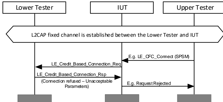
Figure 4.233: L2CAP/LE/CFC/BV-21-C [LE Credit Based Connection Request - refused due to Unacceptable Parameters - Initiator]
