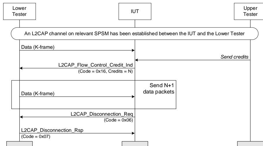
Figure 4.199: Credit Exchange – No Credits
