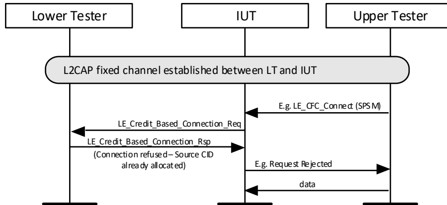
Figure 4.231: L2CAP/LE/CFC/BV-19-C [LE Credit Based Connection Request - refused due to source CID already allocated - Initiator]
