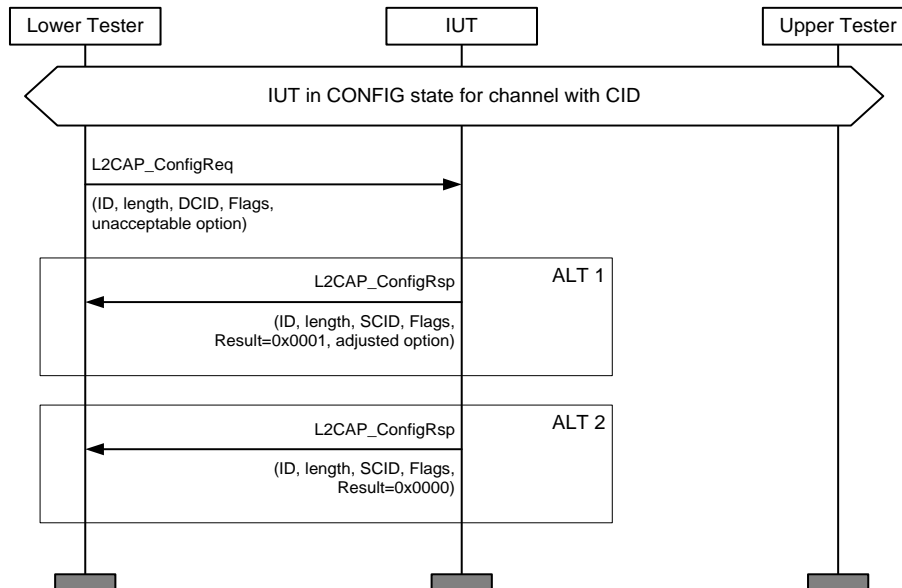
Figure 4.20: L2CAP/COS/CFD/BV-11-C [Negotiation of Unsupported Parameter]
