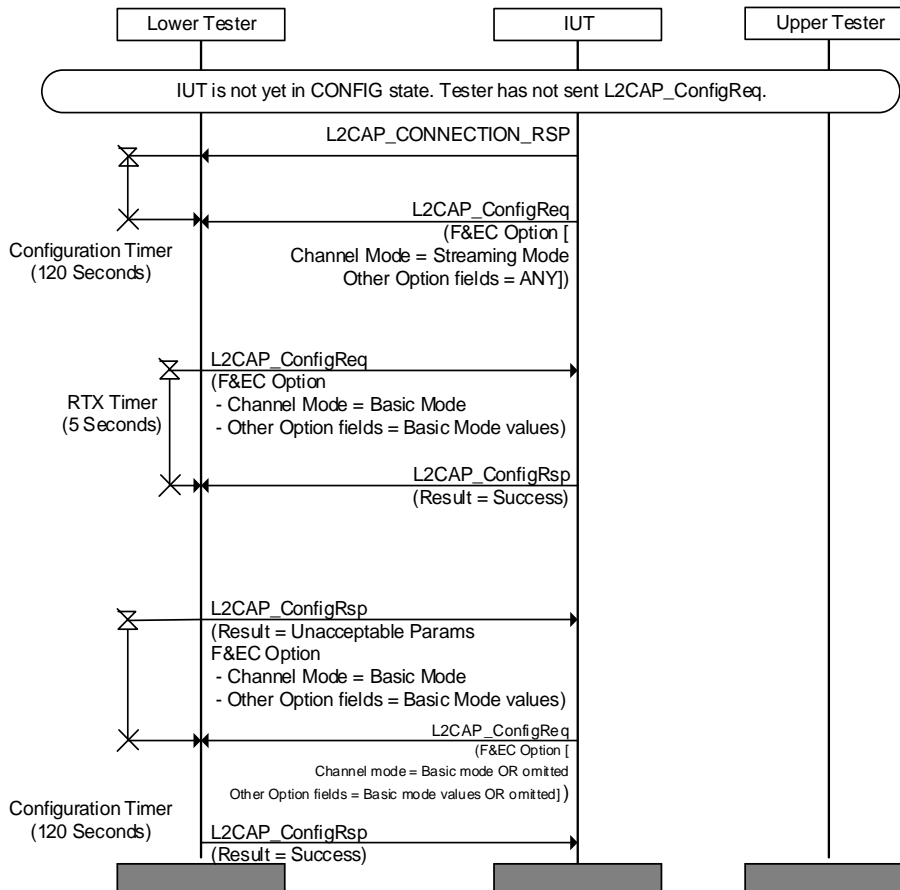
Figure 4.55: L2CAP/CMC/BV-08-C [Configuration Mode Mismatch when use of Streaming Mode is Optional]
