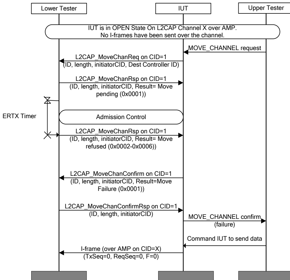
Figure 4.157: L2CAP/MCH/BV-25-C [Move Channel Request for AMP to BR/EDR (STM Source) – AMP Fail]
