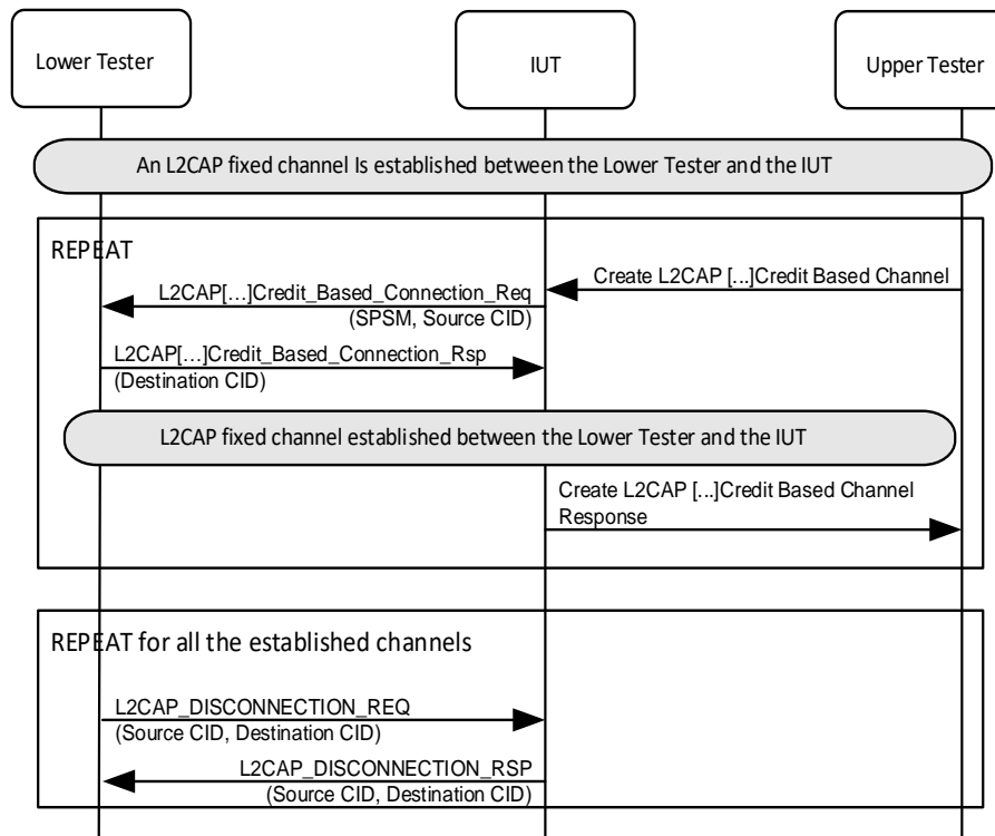
Figure 4.234: Credit Based Connection Request Dynamically Allocated Source CID
