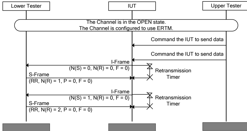
Figure 4.83: L2CAP/ERM/BV-05-C [Resume Transmitting I-Frames when an S-Frame [RR] is Received]
