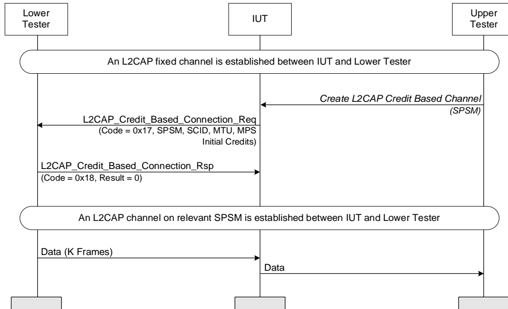
Figure 4.193: L2CAP Credit Based Connection Request on Supported PSM
