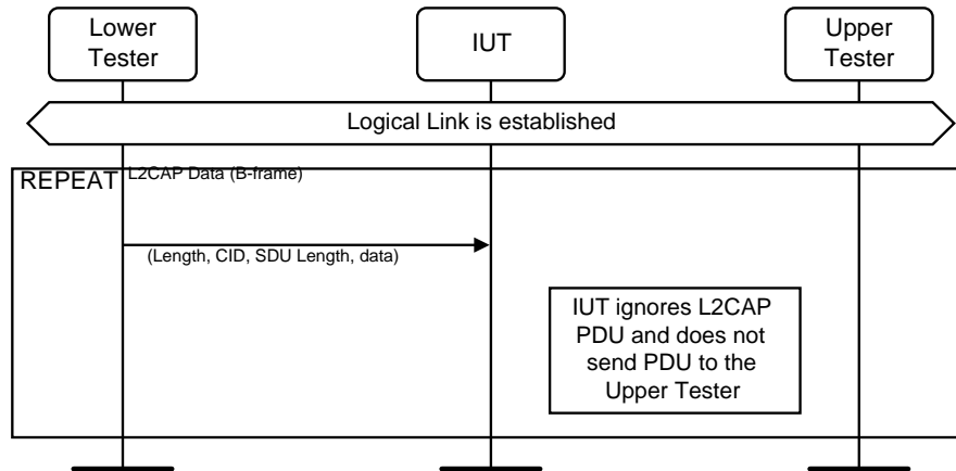
Figure 4.190: Ignore Unsupported CIDs
