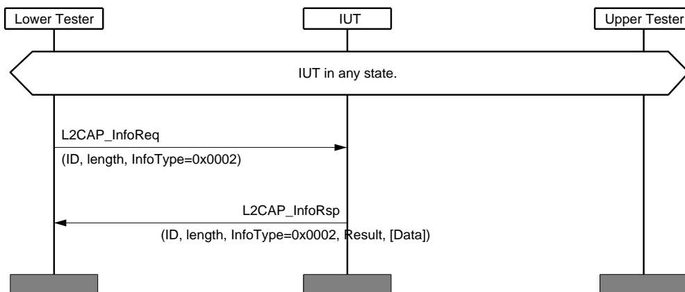
Figure 4.25: L2CAP/COS/IE/BV-02-C [Respond with 1.2 Features]
