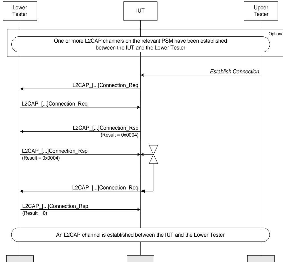
Figure 4.250: Back-off on Connection Request Collision
