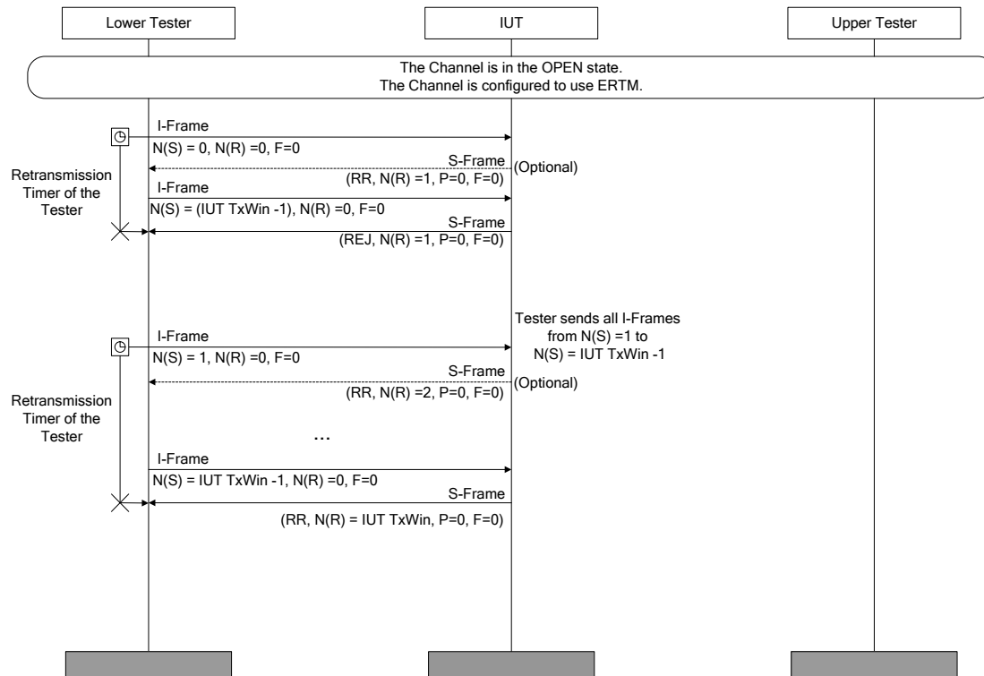
Figure 4.94: L2CAP/ERM/BV-16-C [Send S-Frame [REJ]]
