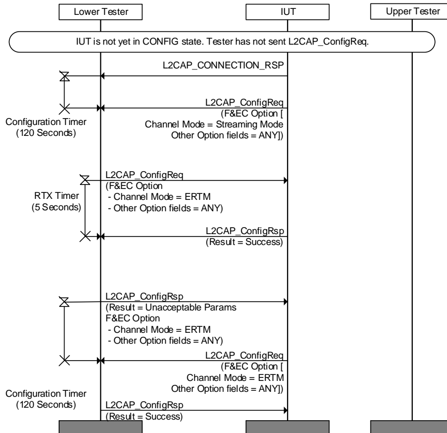
Figure 4.68: L2CAP/CMC/BV-15-C [Configuration Mode Mismatch when use of Streaming Mode is Optional and ERTM is proposed by the Lower Tester]
