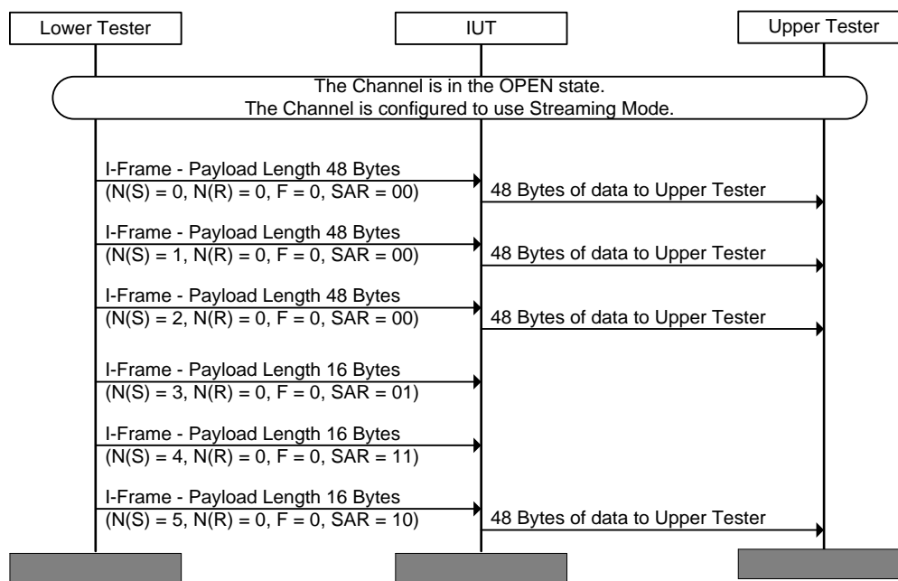
Figure 4.107: L2CAP/STM/BV-02-C [Streaming Mode Sink]
