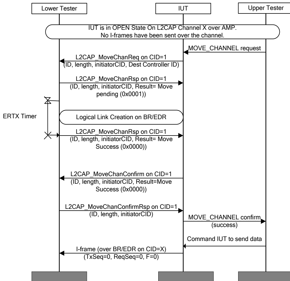
Figure 4.153: L2CAP/MCH/BV-21-C [Move Channel Request for AMP to BR/EDR (STM Source) – Success]
