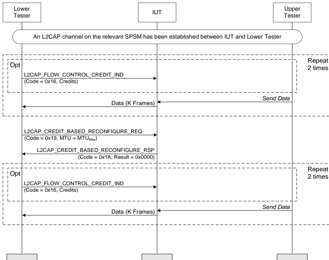
Figure 4.208: Renegotiate MTU – Responder
