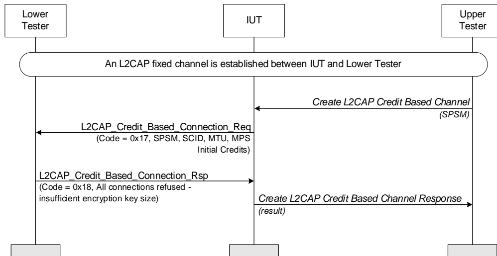
Figure 4.201: Security – Insufficient Encryption Key Size – Initiator
