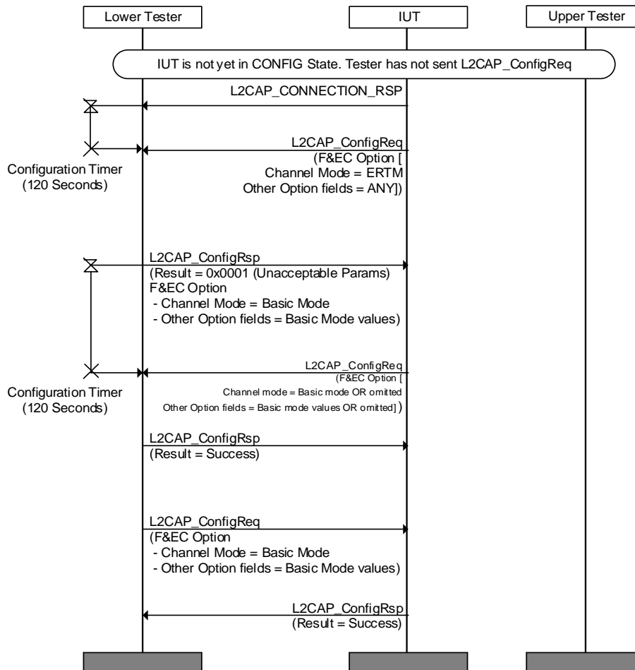
Figure 4.50: L2CAP/CMC/BV-03-C [Failed Configuration of Enhanced Retransmission Mode when use of the Mode is Optional]
