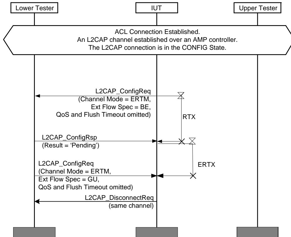
Figure 4.126: L2CAP/LSC/BV-10-I [Mismatched Service Type, Best Effort, AMP Channel]
