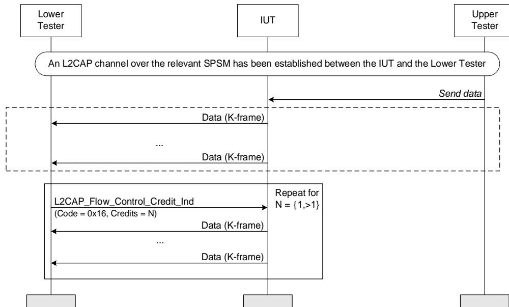
Figure 4.196: Credit Exchange – Receiving Incremental Credits
