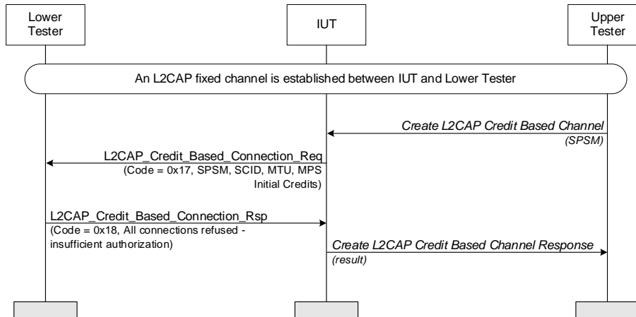
Figure 4.238: Security – Insufficient Authorization – Initiator
