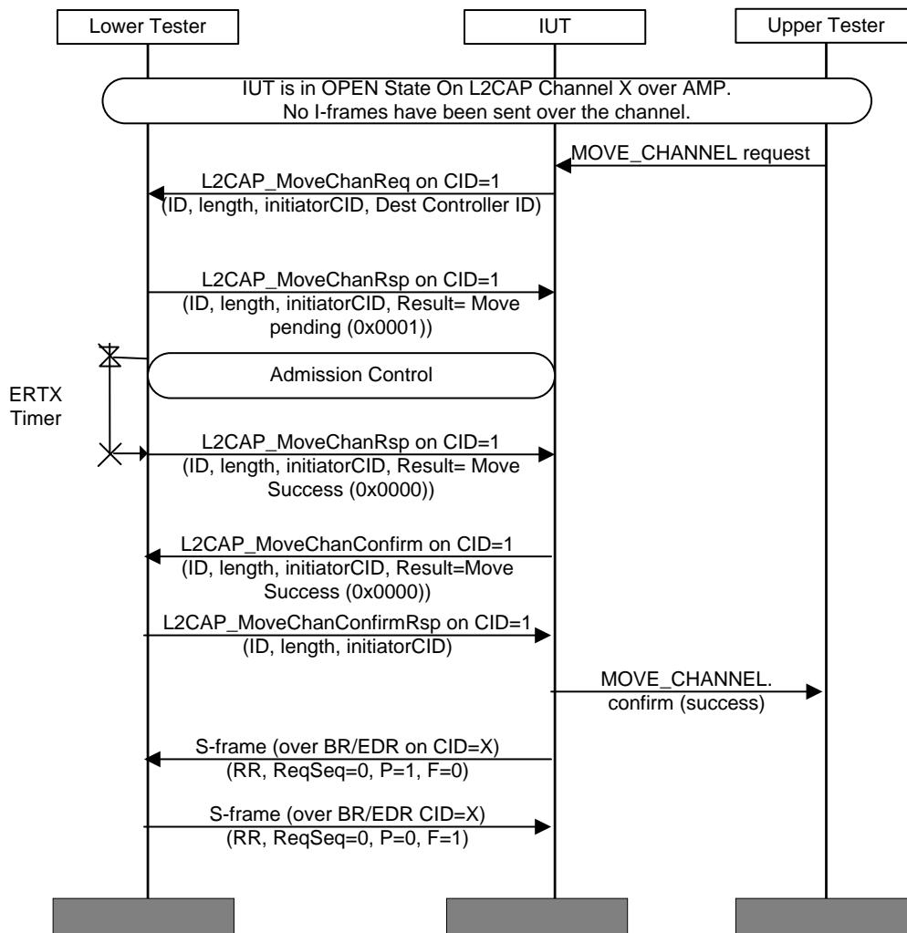
Figure 4.136: L2CAP/MCH/BV-04-C [Move ERTM Channel Request for AMP to BR/EDR – Success]
