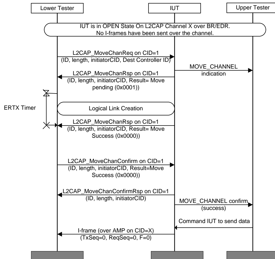
Figure 4.159: L2CAP/MCH/BV-27-C [Move Channel Response for BR/EDR to AMP (STM Source) – Success]
