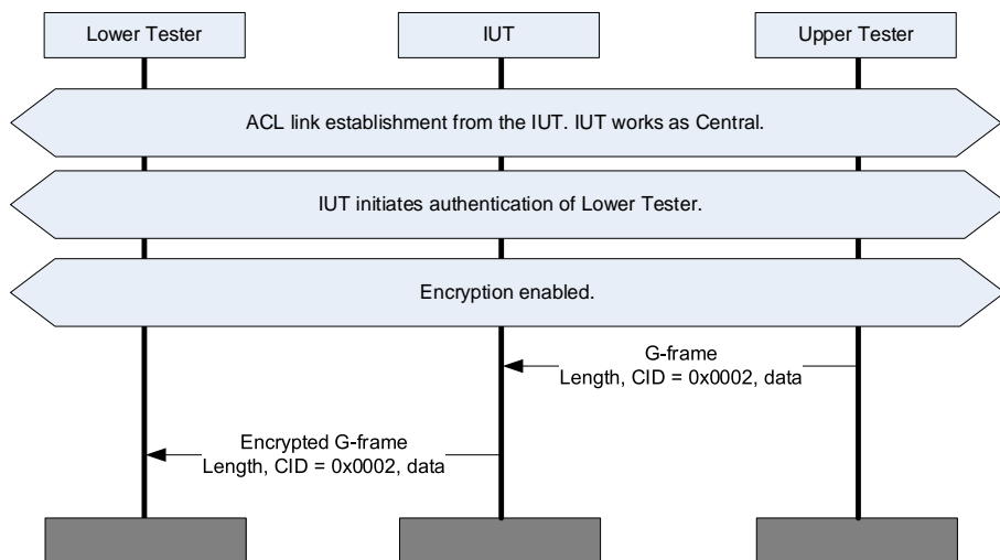
Figure 4.189: L2CAP/CLS/UCD/BV-03-C [Encrypted Data Transmission over Unicast Connectionless Channel]
