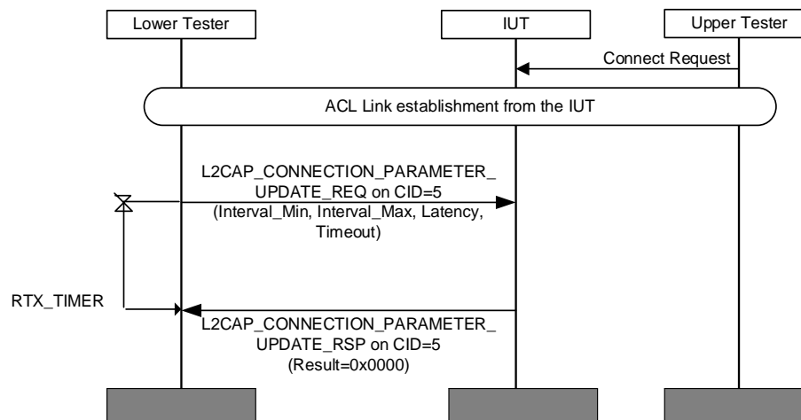
Figure 4.181: L2CAP/LE/CPU/BV-02-C [Accept Connection Parameter Update Request]
