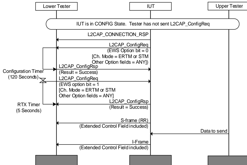
Figure 4.115: L2CAP/EWC/BV-02-C [Lower Tester Requests Extended Window Size]
