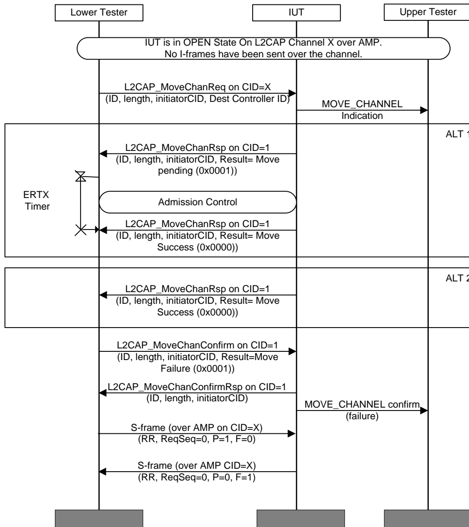
Figure 4.141: L2CAP/MCH/BV-09-C [Move ERTM Channel Response for AMP to BR/EDR – Failure]
