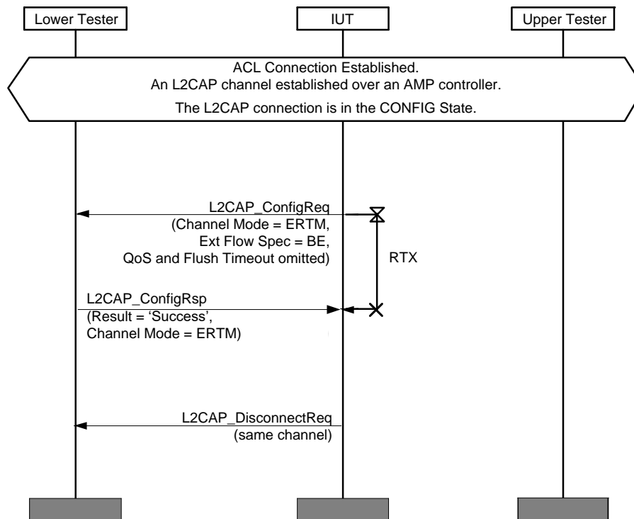
Figure 4.125: L2CAP/LSC/BV-09-C [Premature Success in Configuration Response, AMP Channel]
