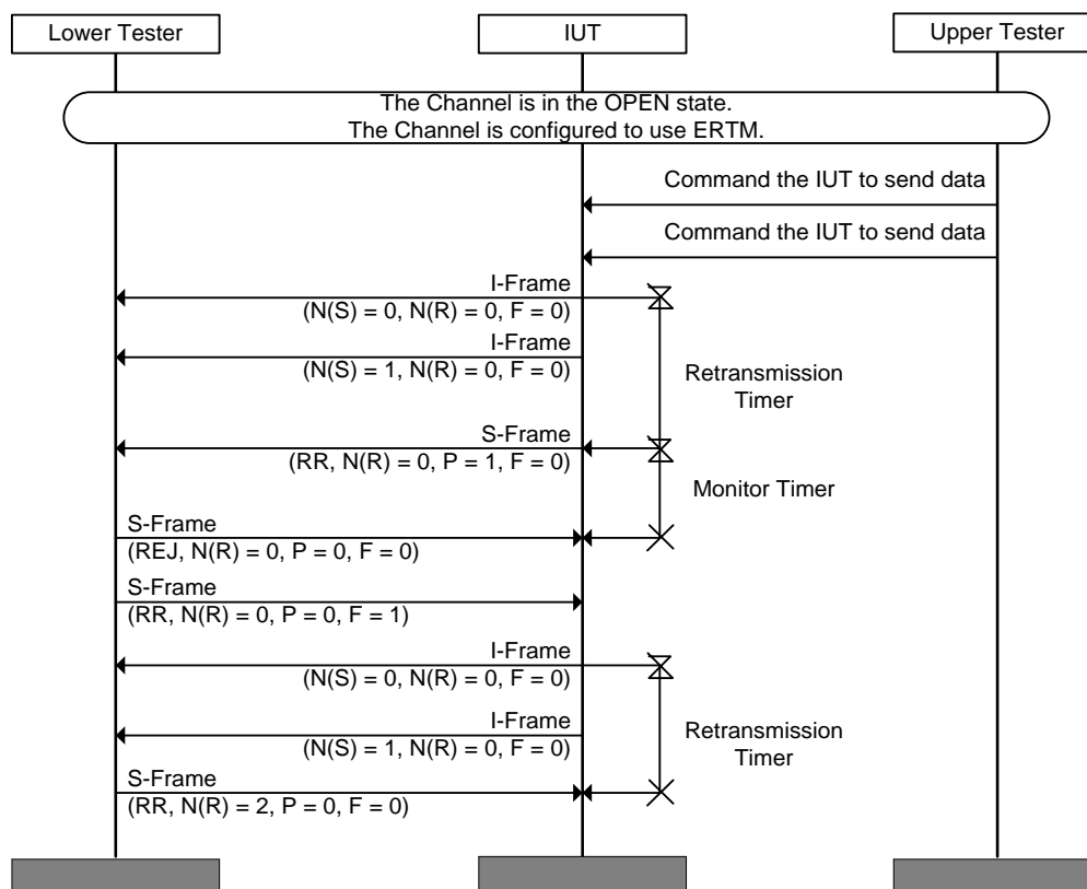
Figure 4.104: L2CAP/ERM/BI-04-C [Handle Receipt of S-Frame [REJ] and S-Frame [RR, F=1] that Both Require Retransmission of the Same I-Frames]
