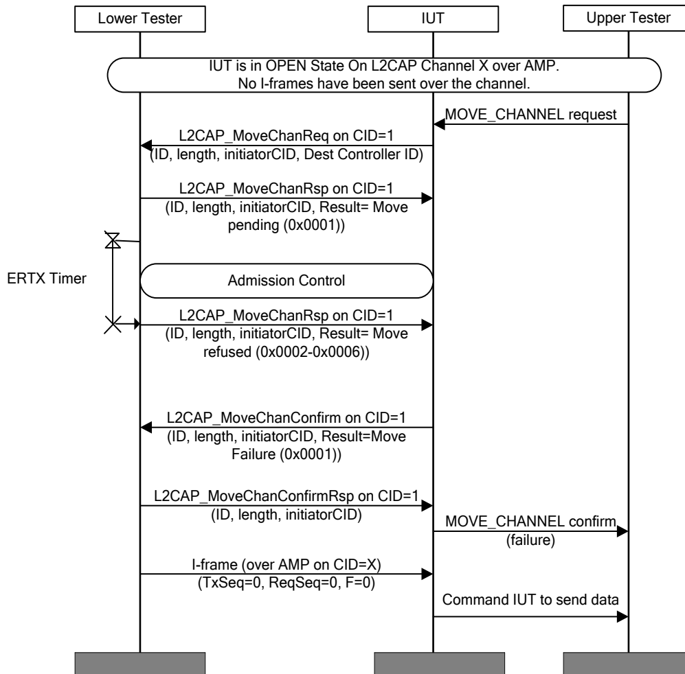
Figure 4.158: L2CAP/MCH/BV-26-C [Move Channel Request for AMP to BR/EDR (STM Sink) – AMP Failed]
