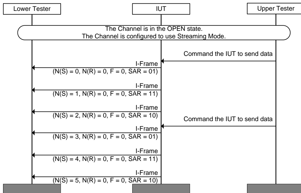
Figure 4.108: L2CAP/STM/BV-03-C [Streaming Mode Source using SAR]
