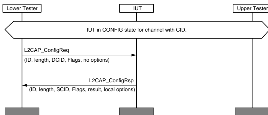
Figure 4.16: L2CAP/COS/CFD/BV-03-C [Send Requested Options]
