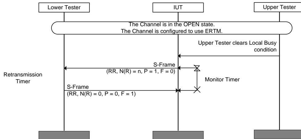
Figure 4.99: L2CAP/ERM/BV-22-C [Exit Local Busy Condition]
