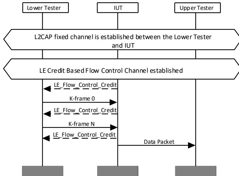
Figure 4.30: L2CAP/COS/CFC/BV-03-C [Reassembling]
