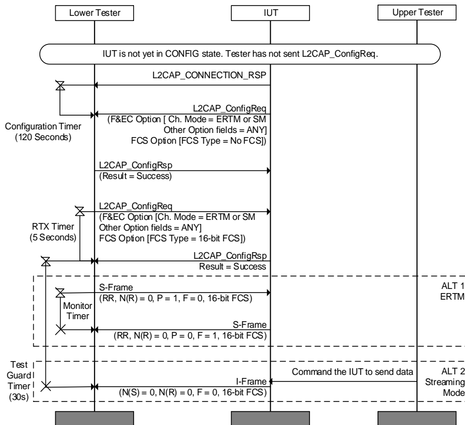
Figure 4.70: L2CAP/FOC/BV-02-C [Lower Tester Explicitly Requests FCS should be Used]
