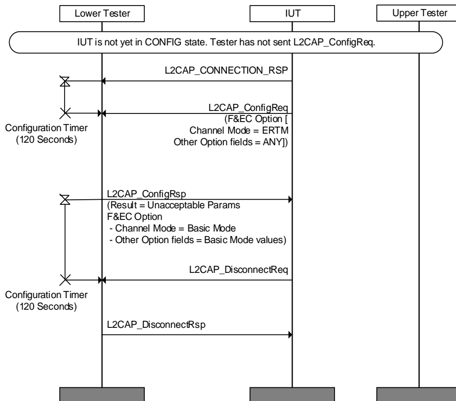
Figure 4.57: L2CAP/CMC/BI-01-C [Failed Configuration of Enhanced Retransmission Mode when use of the Mode is Mandatory]
