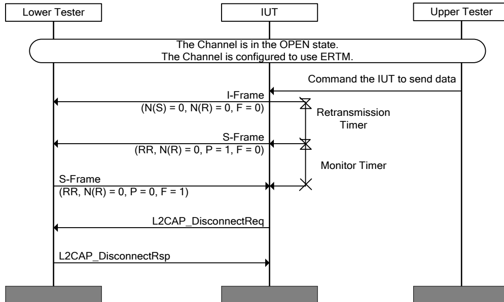
Figure 4.90: L2CAP/ERM/BV-12-C [I-Frame Transmissions Exceed MaxTransmit]
