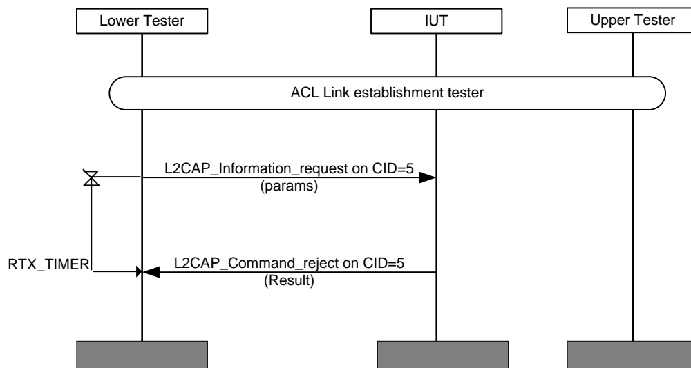
Figure 4.184: L2CAP/LE/REJ/BI-01-C [Reject Unknown Command in LE Signaling Channel]
