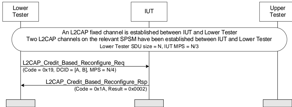
Figure 4.212: Renegotiate MPS – MPS value is decreased
