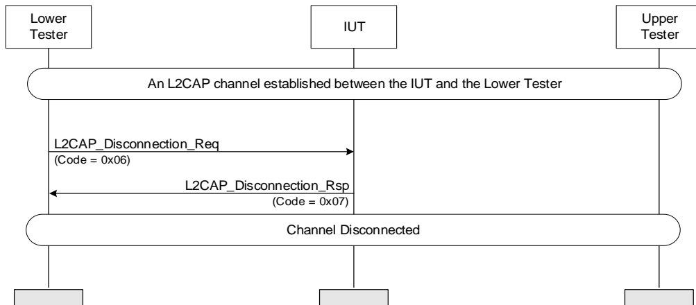
Figure 4.236: Disconnect Response
