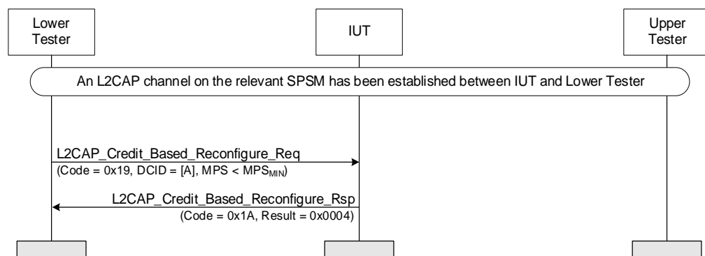
Figure 4.216: Reconfigure – other unacceptable parameters
