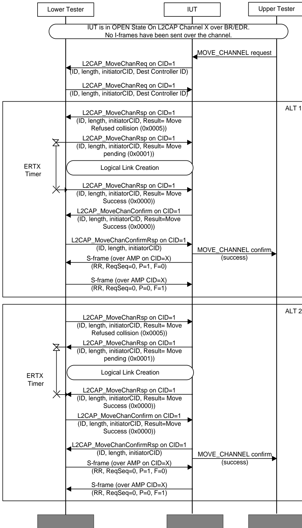
Figure 4.146: L2CAP/MCH/BV-14-C [Move Collision – ERTM]
