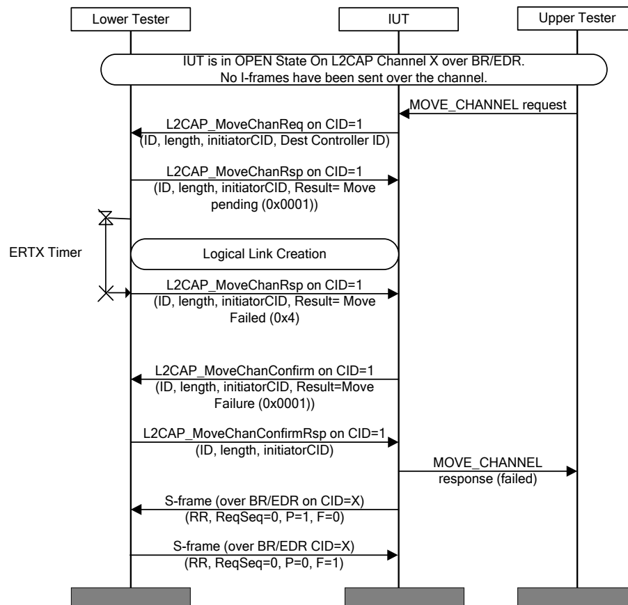
Figure 4.135: L2CAP/MCH/BV-03-C [Move ERTM Channel Request for BR/EDR to AMP – AMP Fail]
