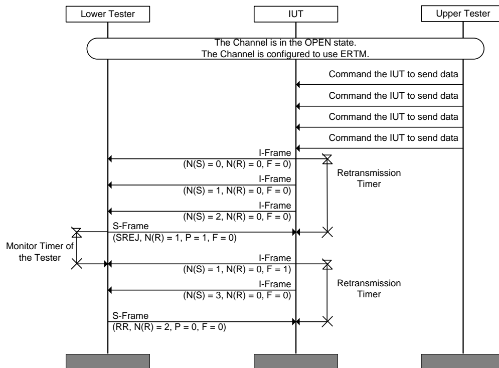
Figure 4.174: L2CAP/ECF/BV-06-C [Respond to S-Frame [SREJ] with Extended Control Field and POLL bit Set]
