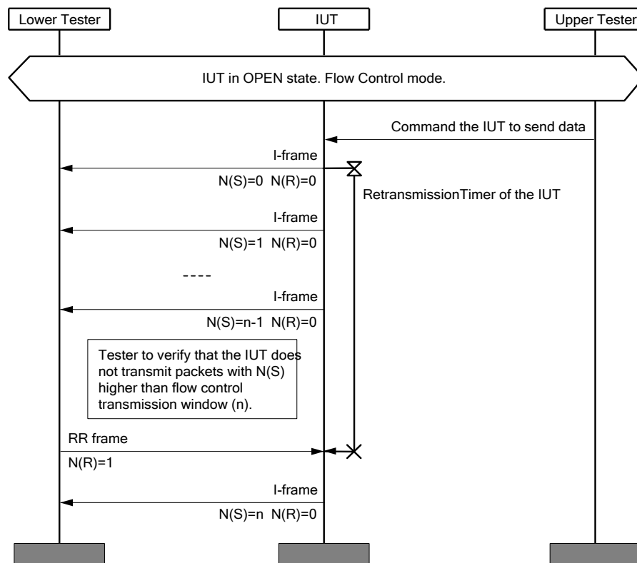
Figure 4.39: L2CAP/COS/FLC/BV-02-C [Resume Flow on RR Frame Ack]
