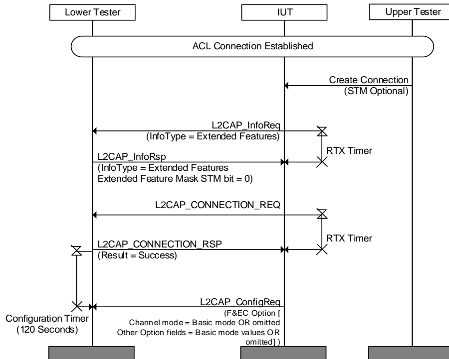
Figure 4.64: L2CAP/CMC/BV-11-C [Streaming Mode not supported by Lower Tester for Optional Streaming Mode Channel]
