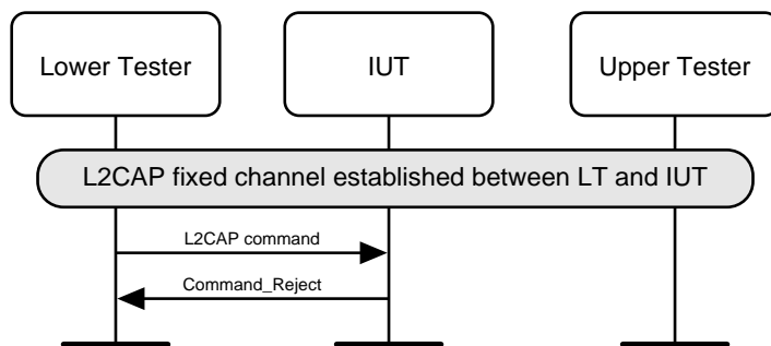
Figure 4.185: L2CAP/LE/REJ/BI-02-C [Command Reject – Reserved PDU Codes]
