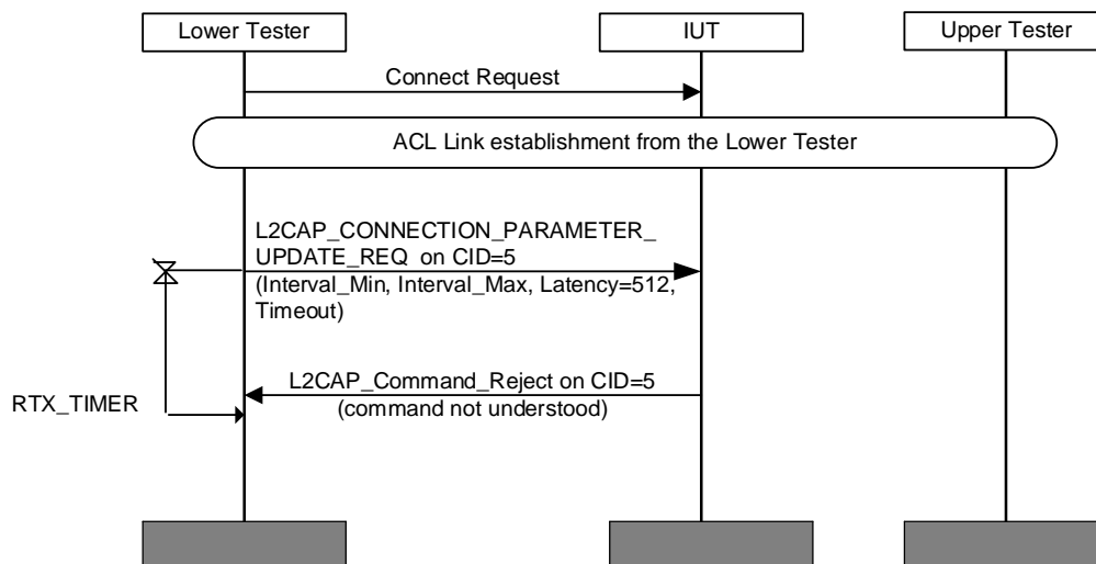
Figure 4.183: L2CAP/LE/CPU/BI-02-C [Reject Connection Parameter Update Request]
