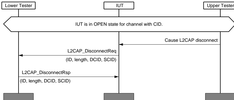
Figure 4.3: L2CAP/COS/CED/BV-04-C [Disconnect]
