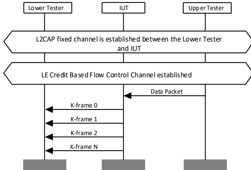
Figure 4.28: L2CAP/COS/CFC/BV-01-C [Segmentation]
