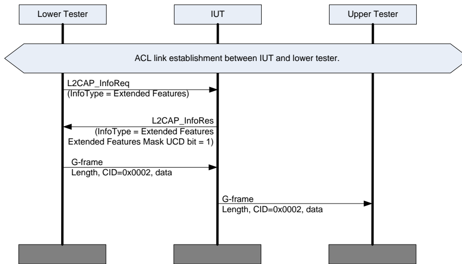
Figure 4.187: L2CAP/CLS/UCD/BV-01-C [Data Reception over Unicast Connectionless Channel]
