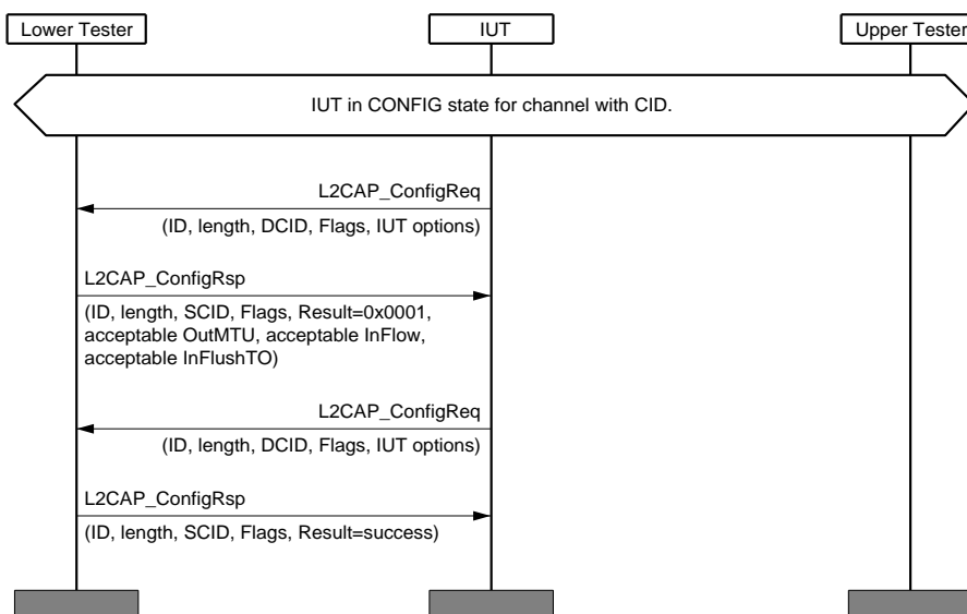
Figure 4.15: L2CAP/COS/CFD/BV-02-C [Negotiation with Reject]
