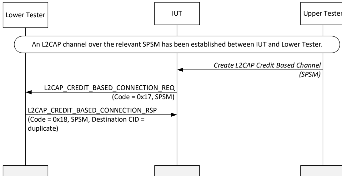
Figure 4.217: L2CAP Credit Based Connection Response – Duplicate DCID
