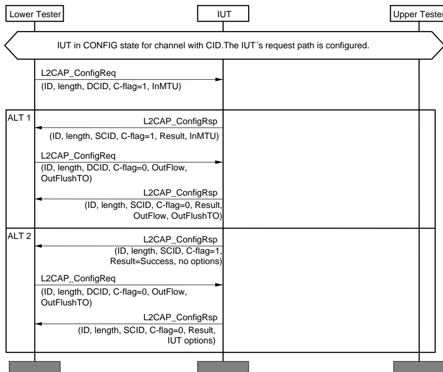
Figure 4.14: L2CAP/COS/CFD/BV-01-C [Continuation Flag]
