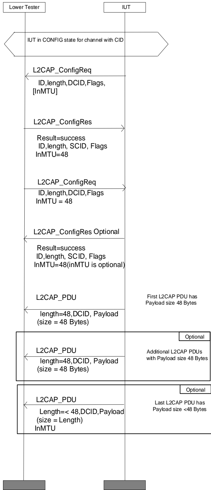
Figure 4.18: L2CAP/COS/CFD/BV-09-C [Mandatory 48 Byte MTU]
