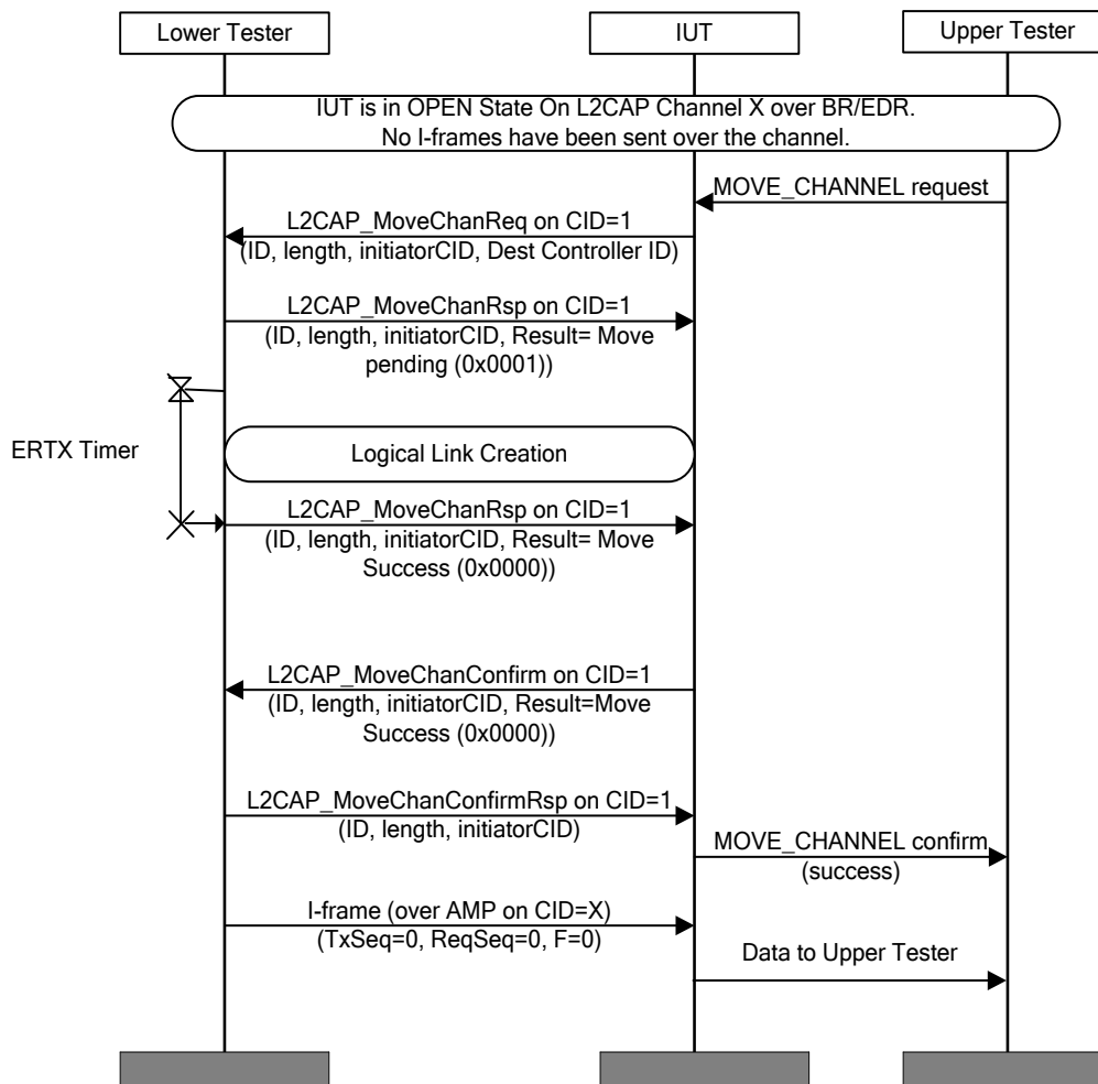
Figure 4.148: L2CAP/MCH/BV-16-C [Move Channel Request for BR/EDR to AMP (STM Sink) – Success]
