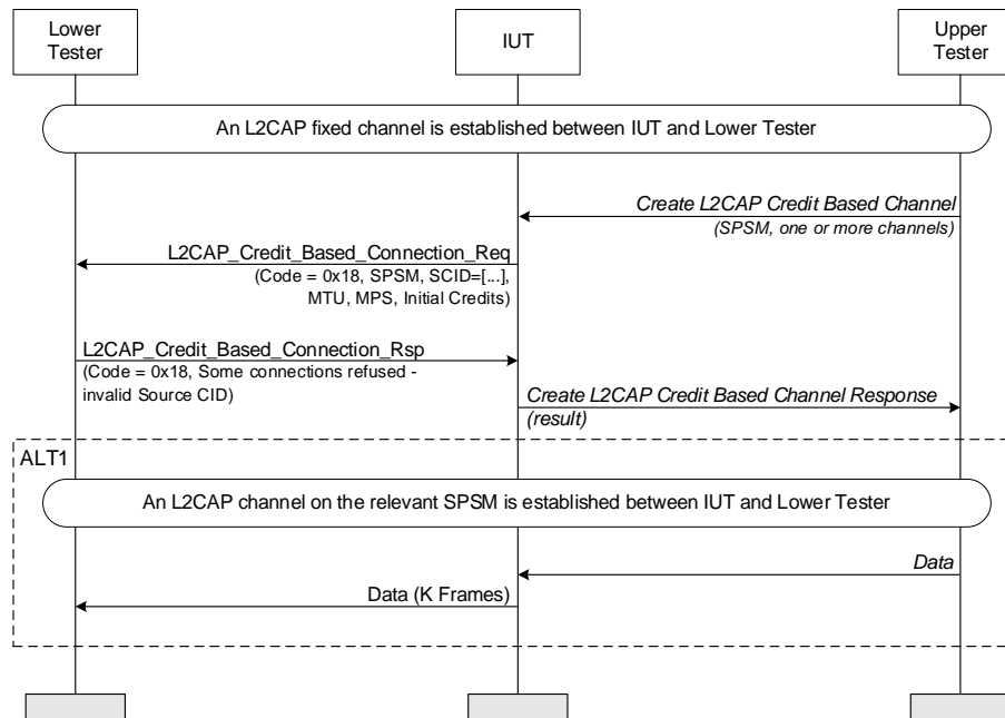
Figure 4.203: L2CAP Credit Based Connection Request – refused due to Invalid Source CID
