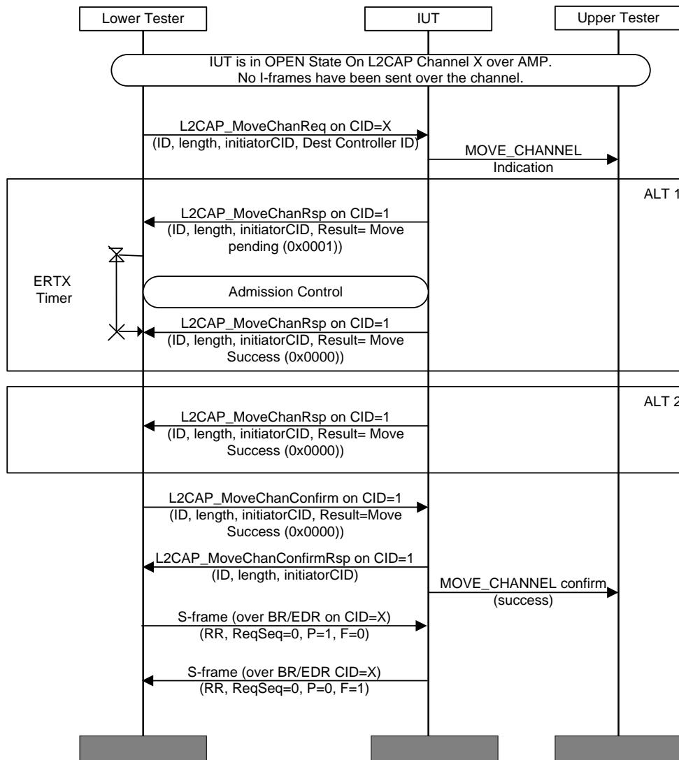
Figure 4.140: L2CAP/MCH/BV-08-C [Move ERTM Channel Response for AMP to BR/EDR – Success]
