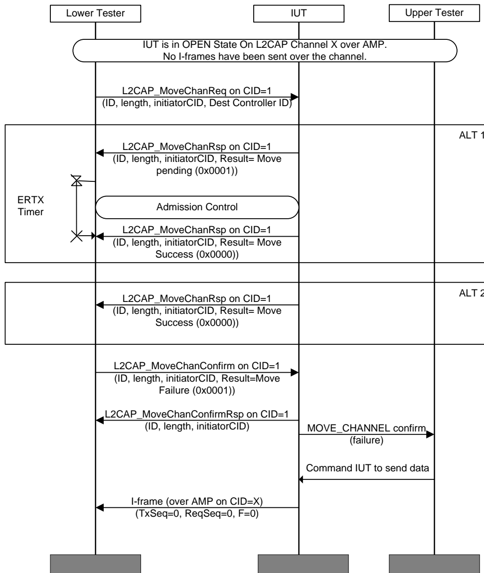
Figure 4.165: L2CAP/MCH/BV-33-C [Move Channel Response for AMP to BR/EDR (STM Source) – Failed]
