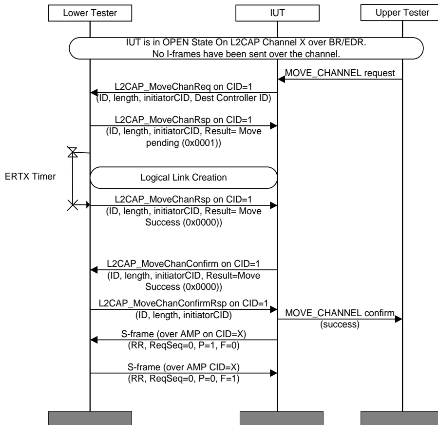
Figure 4.133: L2CAP/MCH/BV-01-C [Move ERTM Channel Request for BR/EDR to AMP – Success]
