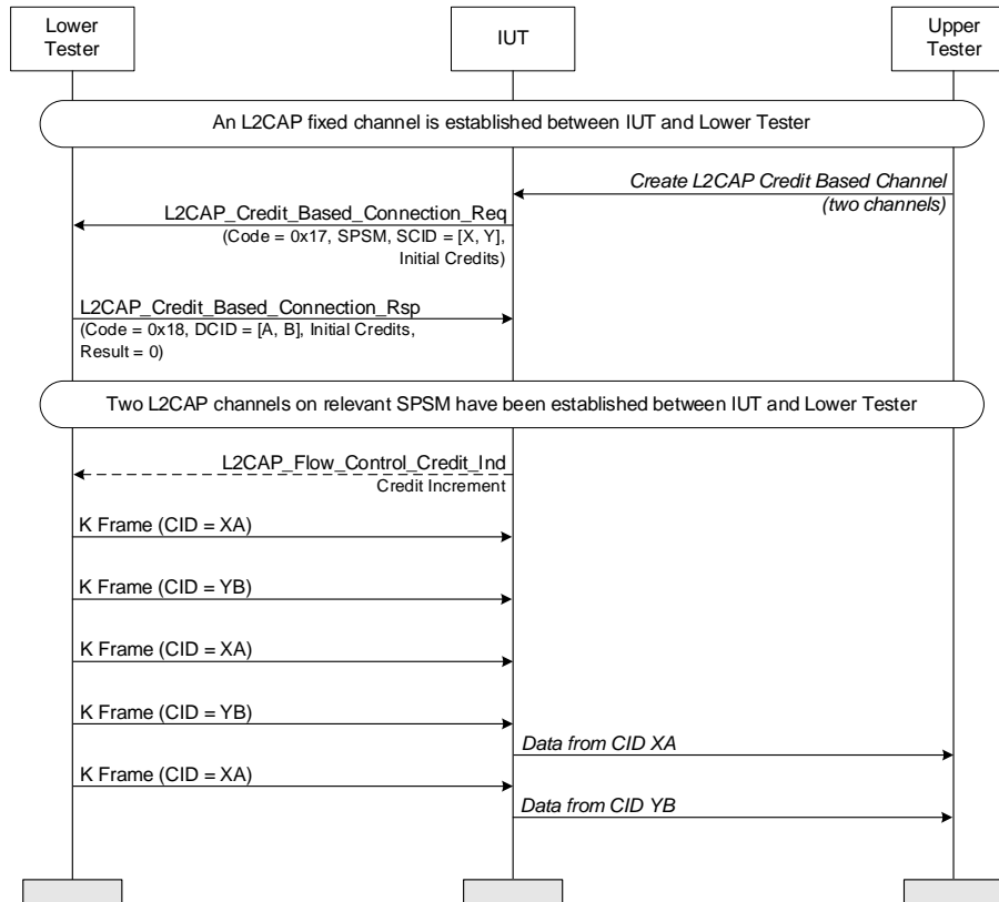
Figure 4.37: Multiple Channels with Interleaved Data Streams
