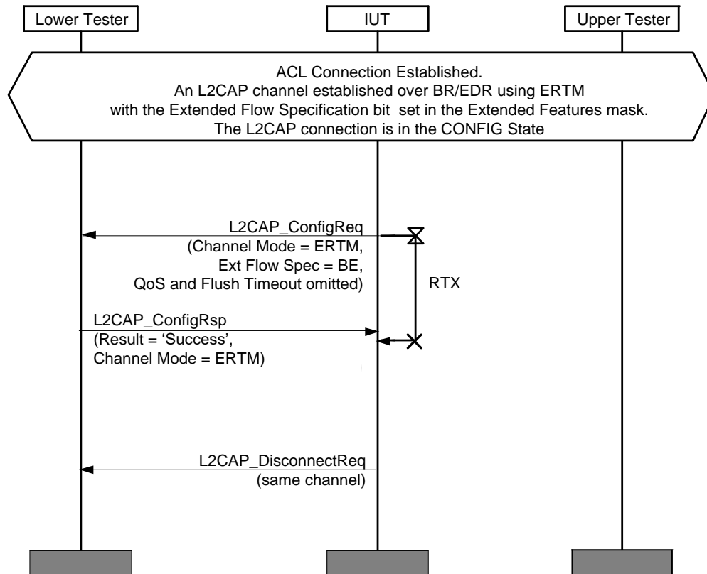
Figure 4.117: L2CAP/LSC/BV-01-C [Normal Lock Step Configuration Process for Best Effort, BR/EDR ERTM Channel]
