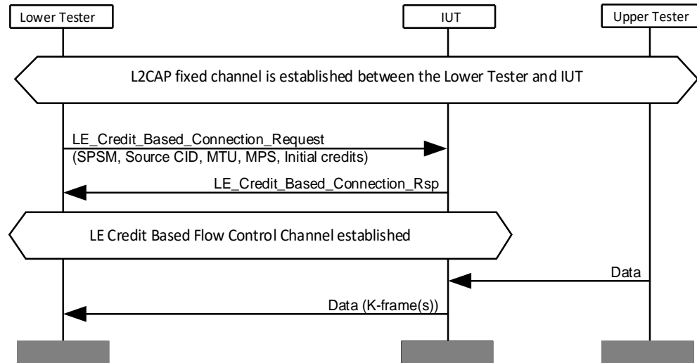
Figure 4.221: L2CAP/LE/CFC/BV-03-C [LE Credit Based Connection Response on Supported SPSM]
