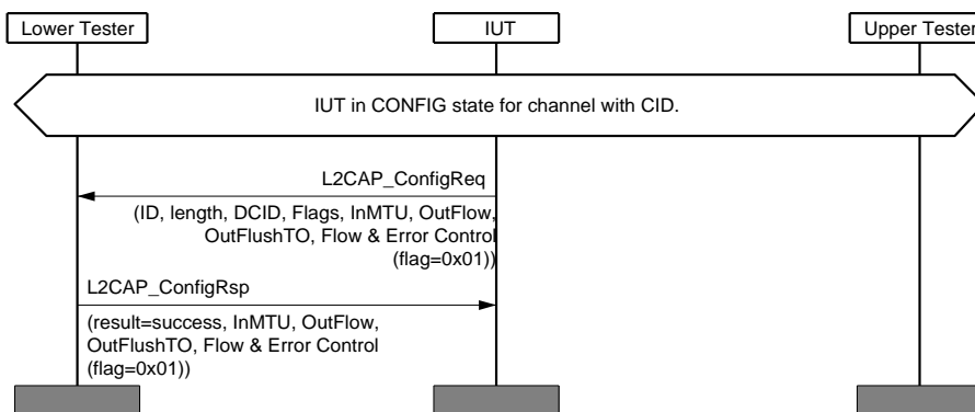
Figure 4.19: L2CAP/COS/CFD/BV-10-C [Retransmission Mode Negotiation]
