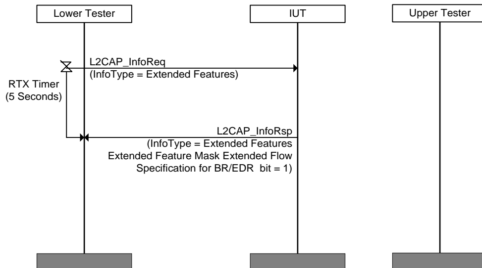
Figure 4.109: L2CAP/EXF/BV-04-C [Extended Features Information Response for Extended Flow Specification for BR/EDR]
