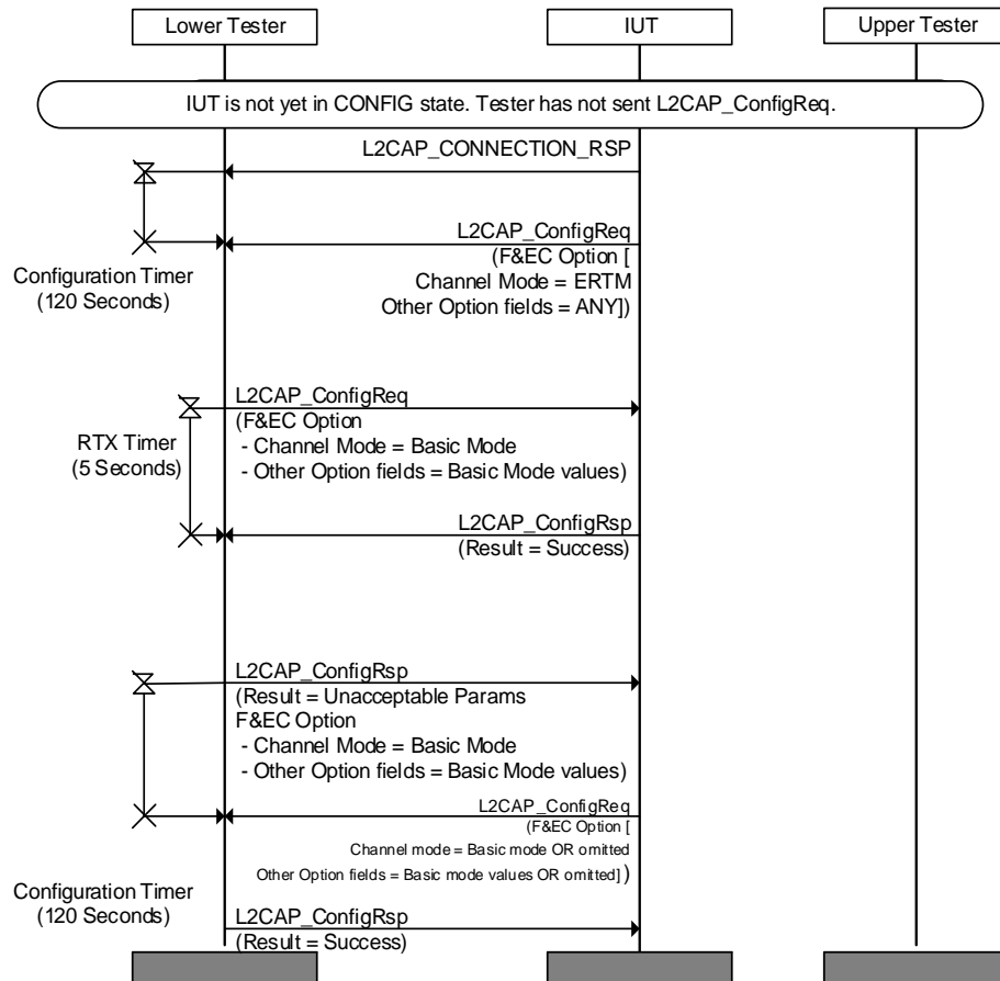
Figure 4.54: L2CAP/CMC/BV-07-C [Configuration Mode mismatch when use of Enhanced Retransmission Mode is Optional]
