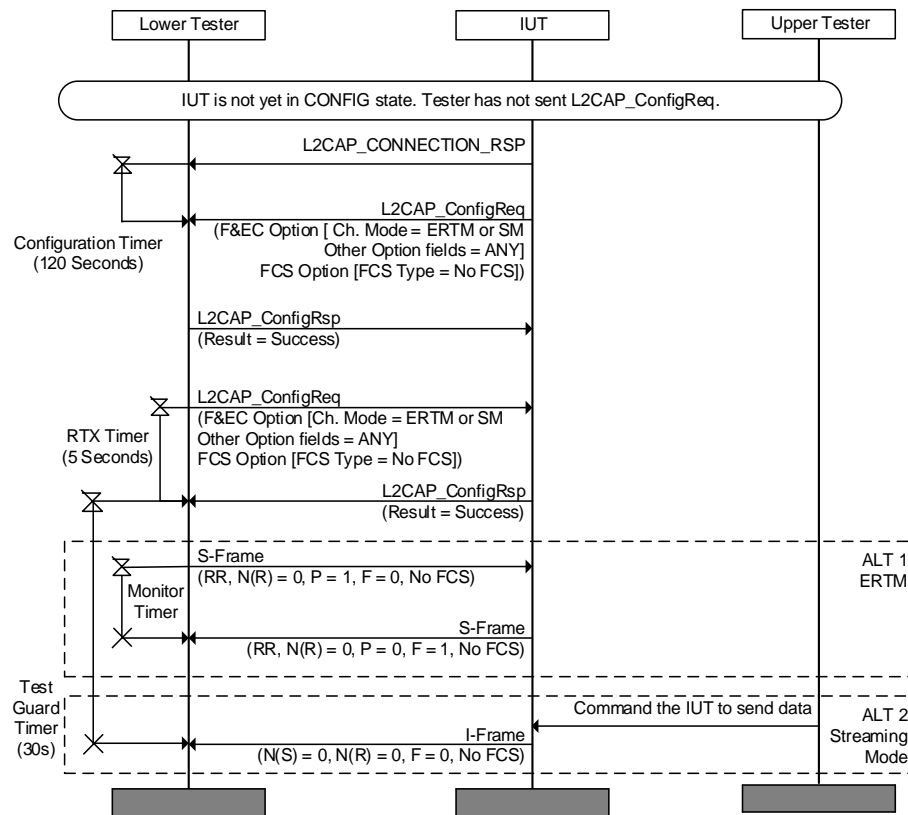
Figure 4.69: L2CAP/FOC/BV-01-C [IUT Initiated Configuration of the FCS Option]
