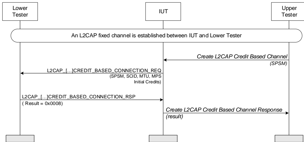
Figure 4.244: Security – Insufficient Encryption – Initiator
