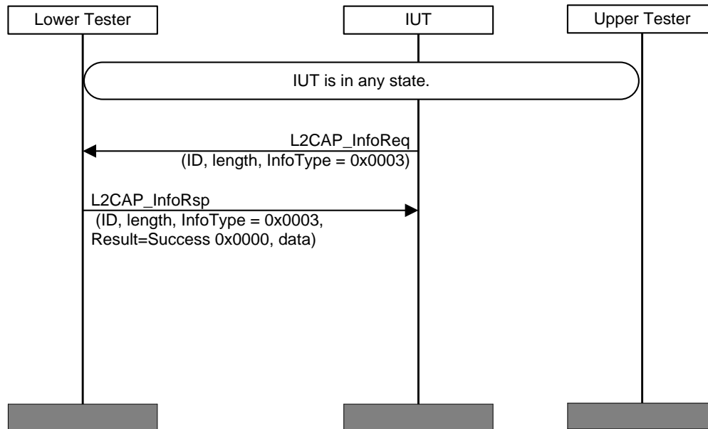
Figure 4.112: L2CAP/FIX/BV-01-C [Fixed Channels Supported Information Request]
