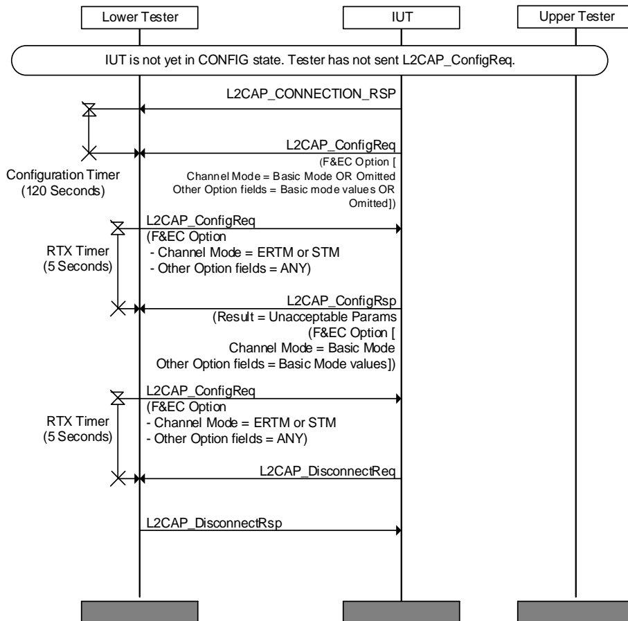
Figure 4.61: L2CAP/CMC/BI-05-C [Failed Configuration to Basic Mode by the IUT]
