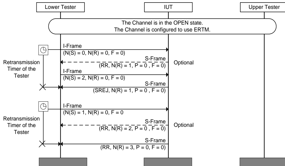
Figure 4.95: L2CAP/ERM/BV-17-C [Send S-Frame [SREJ]]
