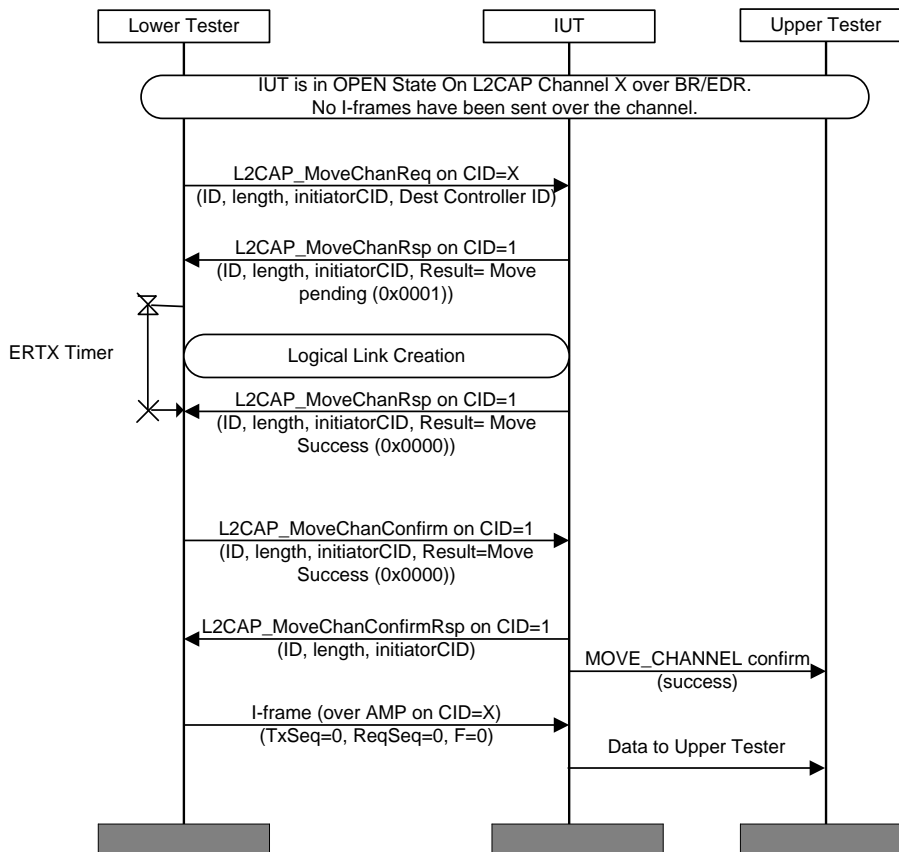
Figure 4.160: L2CAP/MCH/BV-28-C [Move Channel Response for BR/EDR to AMP (STM Sink) – Success]
