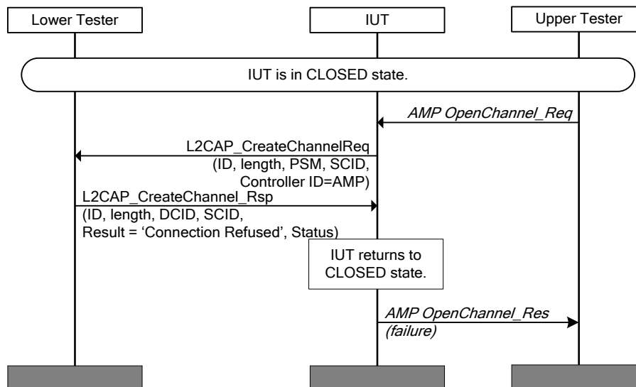
Figure 4.130: L2CAP/CCH/BV-02-C [Create Channel Request for an AMP Physical Link – Refused]
