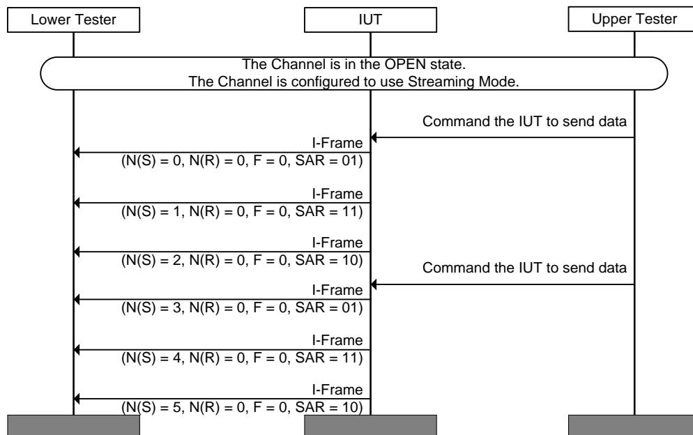
Figure 4.179: L2CAP/STM/BV-03-C [Streaming Mode Source using Extended Control Field and SAR]
