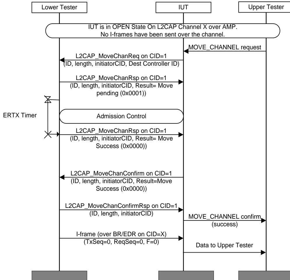
Figure 4.154: L2CAP/MCH/BV-22-C [Move Channel Request for AMP to BR/EDR (STM Sink) – Success]
