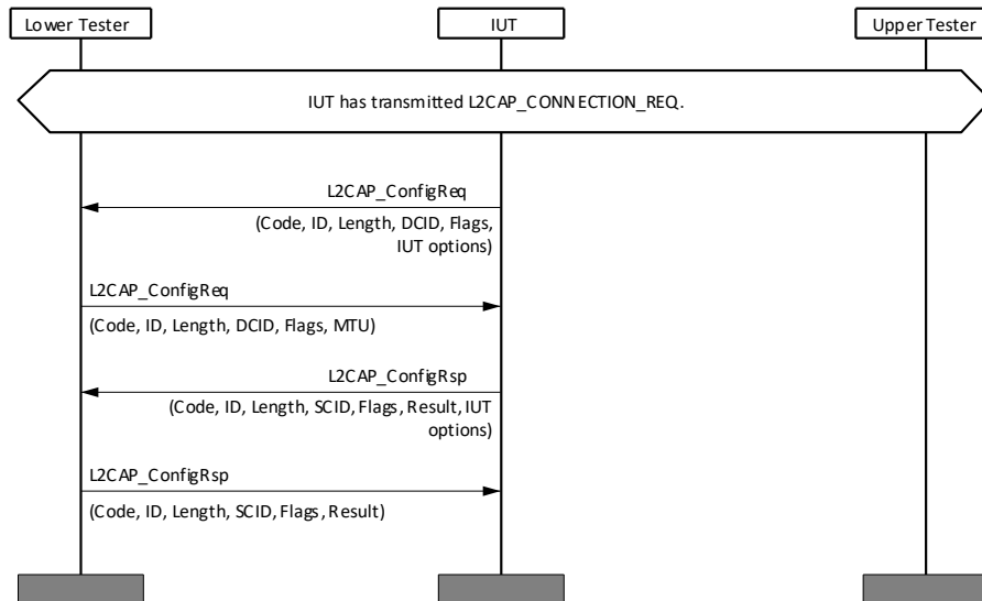
Figure 4.17: L2CAP/COS/CFD/BV-08-C [Non-blocking Config Response]
