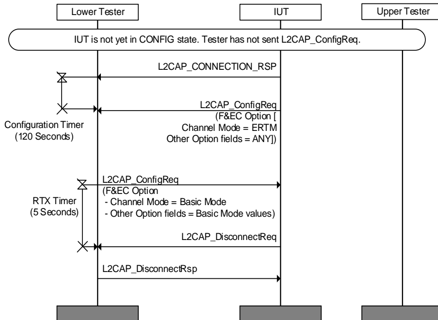
Figure 4.58: L2CAP/CMC/BI-02-C [Configuration Mode mismatch when use of Enhanced Retransmission Mode is Mandatory]
