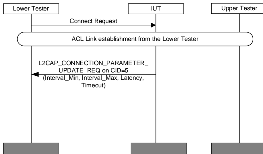
Figure 4.180: L2CAP/LE/CPU/BV-01-C [Send Connection Parameter Update Request]
