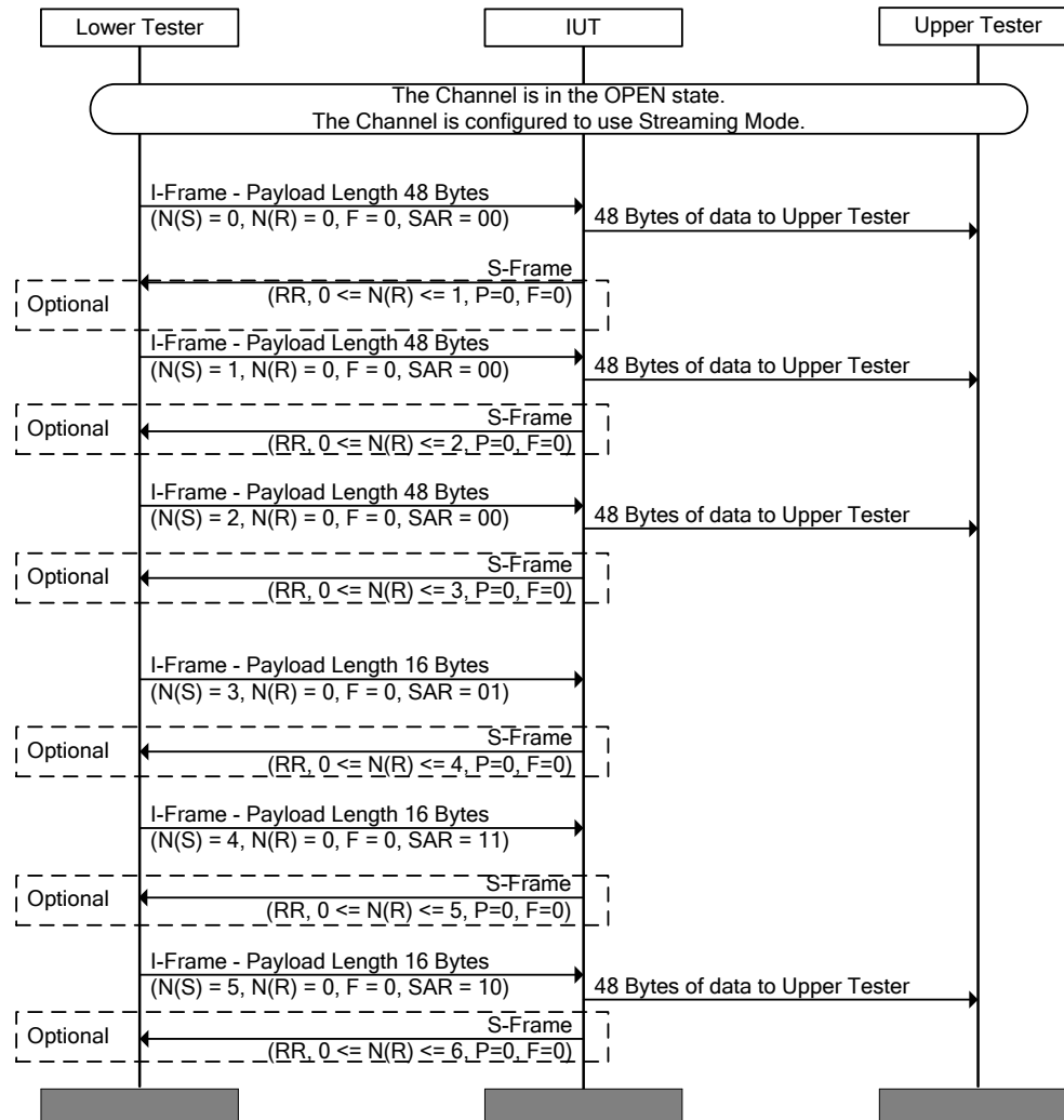
Figure 4.169: L2CAP/ECF/BV-01-C [Receive I-Frames with Extended Control Field]
