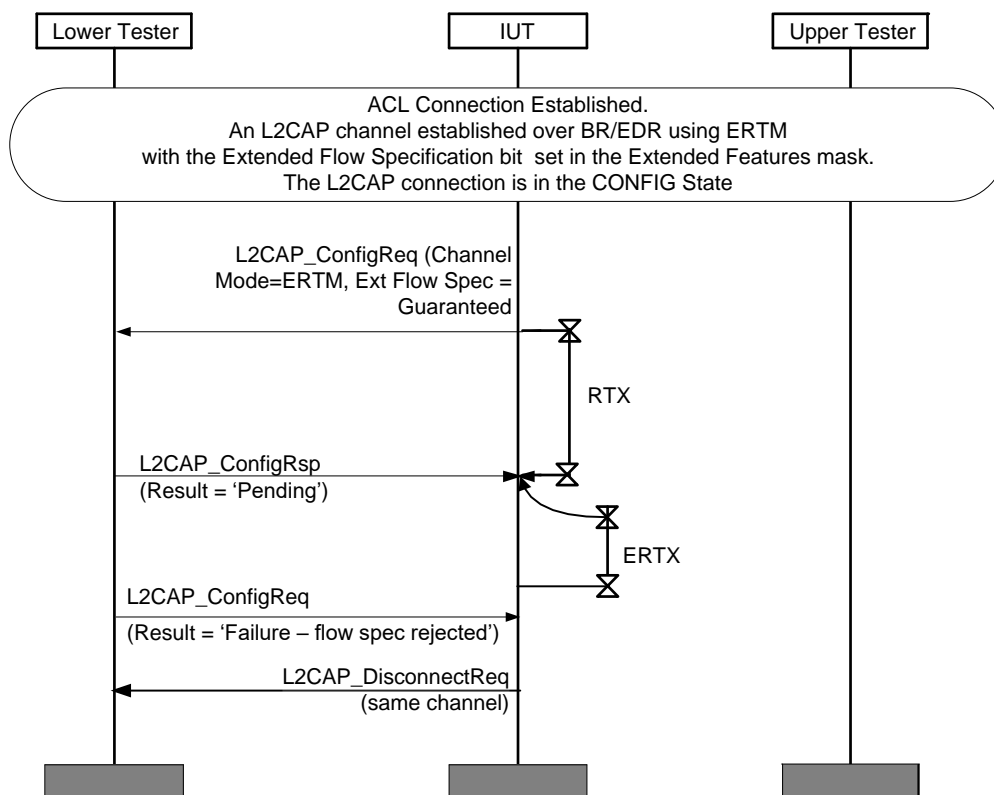
Figure 4.121: L2CAP/LSC/BI-05-C [Mismatched Service Type, Guaranteed, BR/EDR ERTM Channel]
