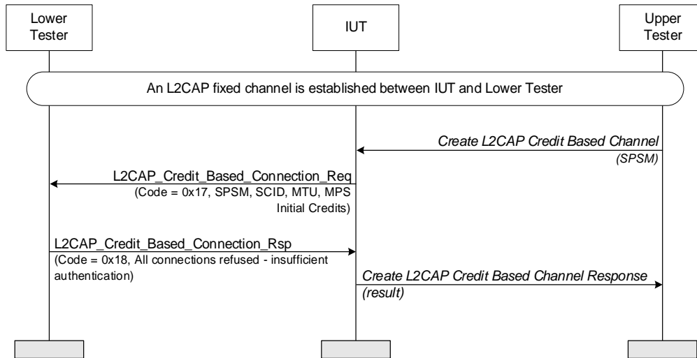
Figure 4.237: Security – Insufficient Authentication – Initiator
