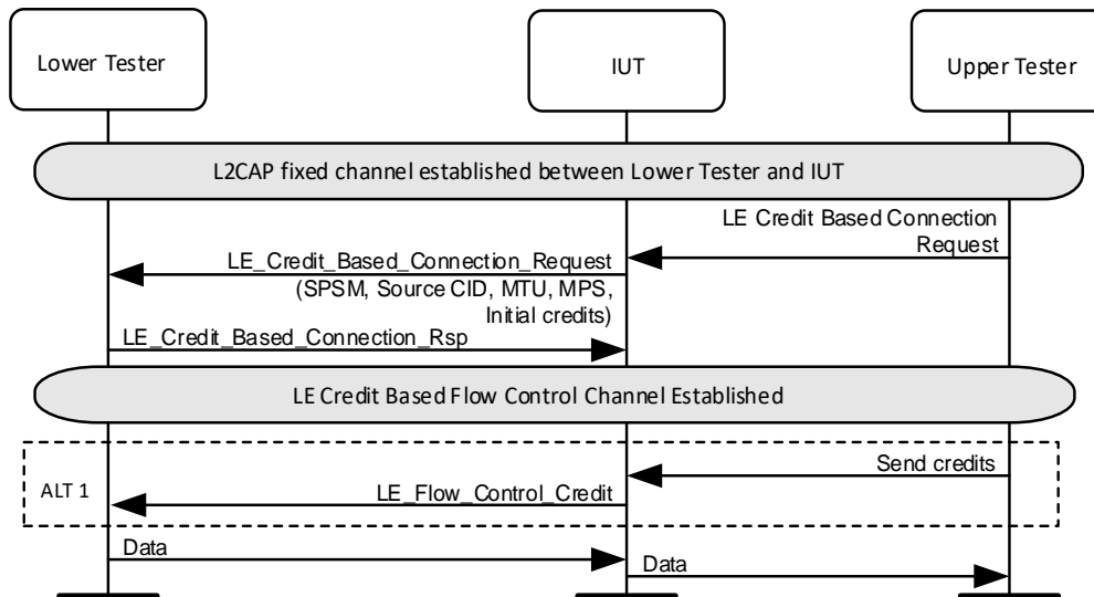
Figure 4.220: L2CAP/LE/CFC/BV-02-C [LE Credit Based Connection Request on Supported SPSM]
