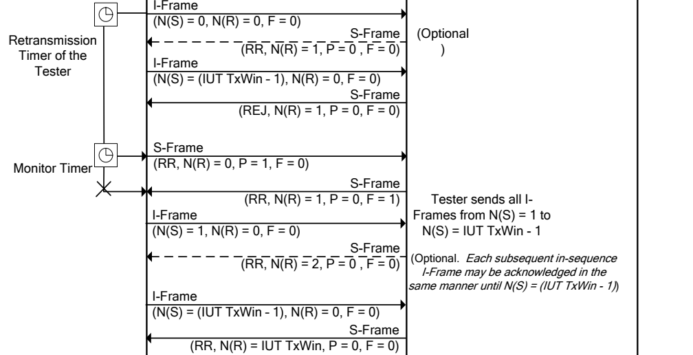
Figure 4.101: L2CAP/ERM/BI-01-C [S-Frame [REJ] Lost or Corrupted]
