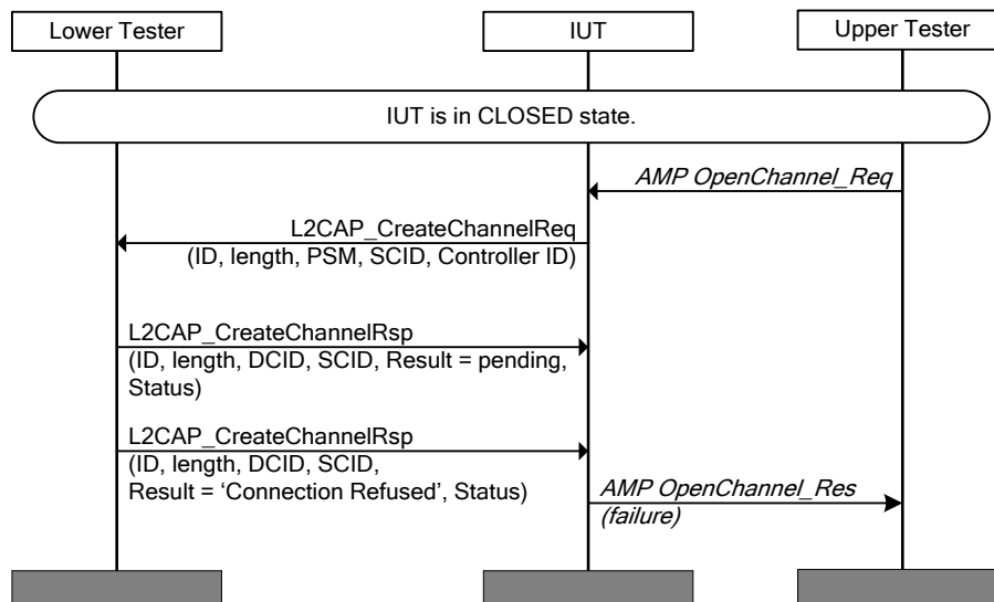
Figure 4.131: L2CAP/CCH/BV-03-C [Create Channel Request for an AMP Physical Link – Failed]
