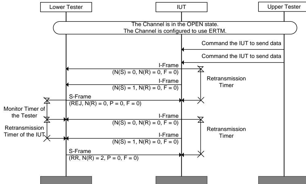
Figure 4.173: L2CAP/ECF/BV-05-C [Respond to S-Frame [REJ] with Extended Control Field]
