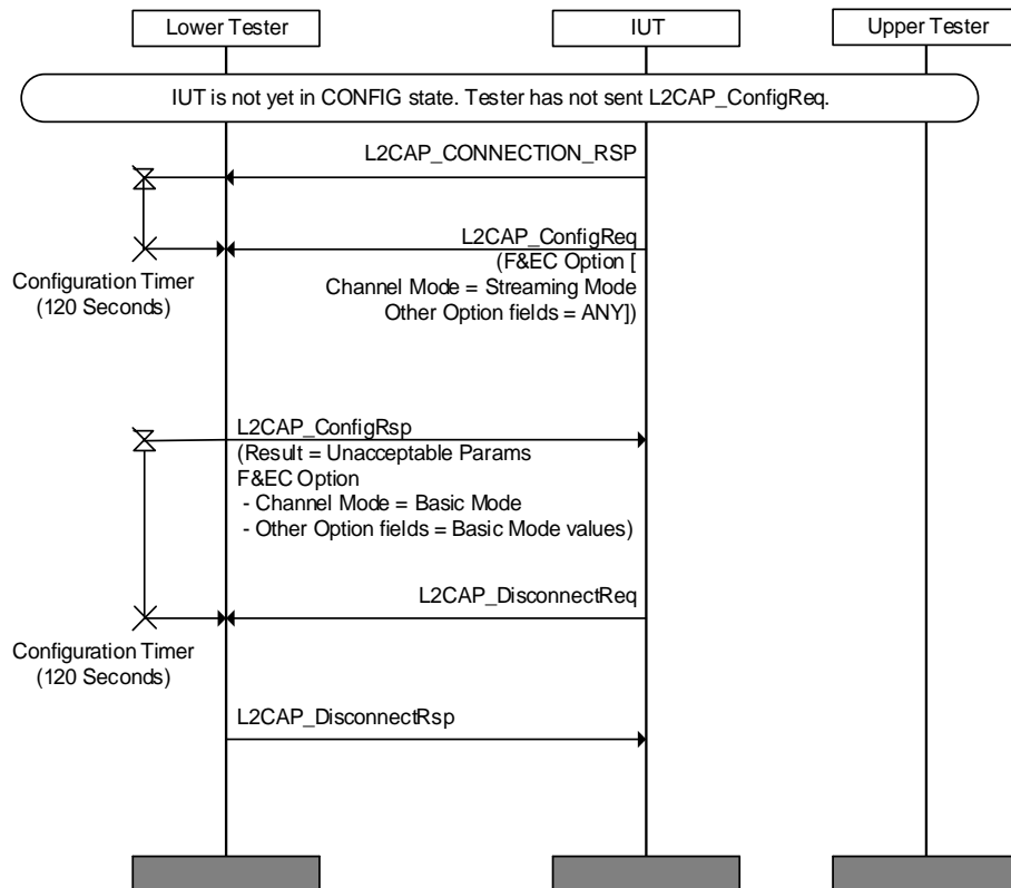
Figure 4.59: L2CAP/CMC/BI-03-C [Failed Configuration of Streaming Mode when use of the Mode is Mandatory]
