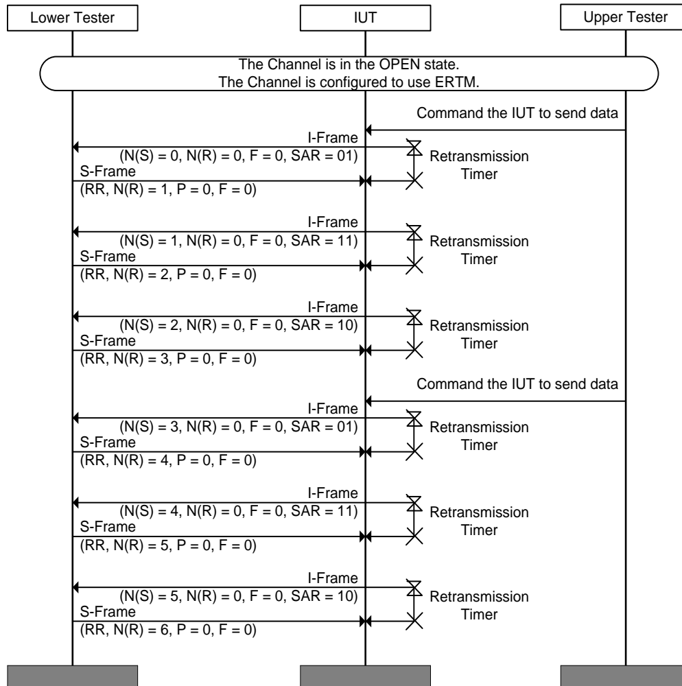
Figure 4.100: L2CAP/ERM/BV-23-C [Transmit I-Frames using SAR]
