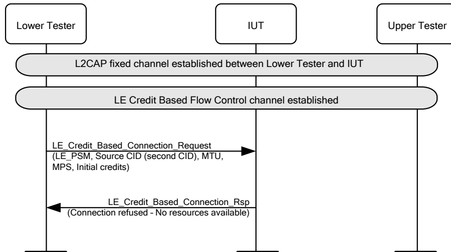
Figure 4.229: L2CAP/LE/CFC/BV-17-C [LE Credit Based Connection Response - refused due to insufficient resources - Responder]
