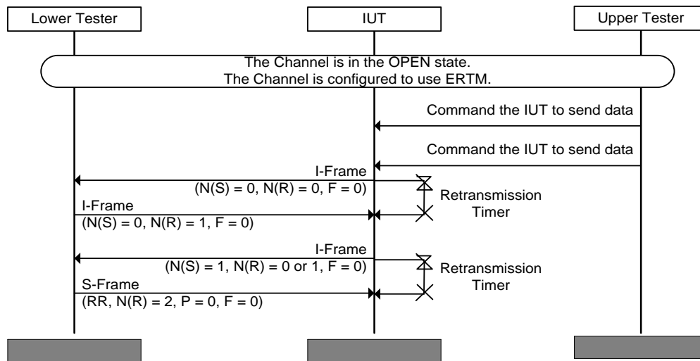
Figure 4.84: L2CAP/ERM/BV-06-C [Resume Transmitting I-Frames when an I-Frame is Received]
