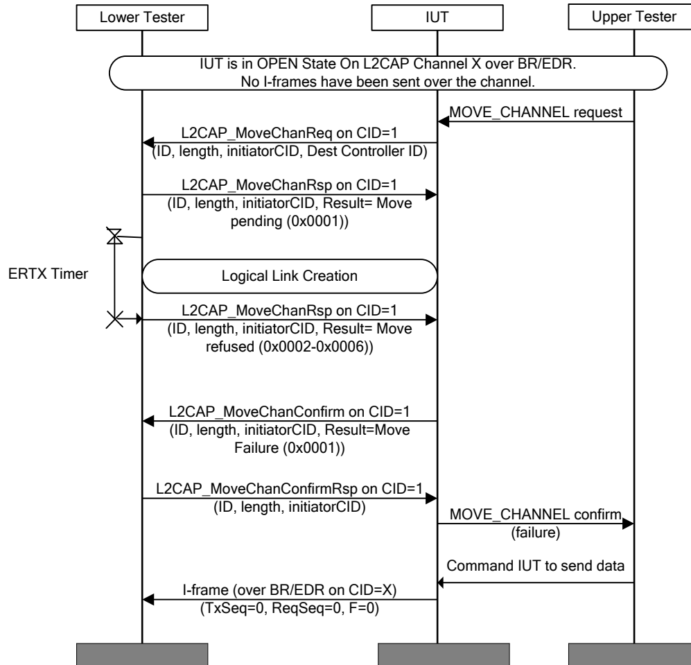
Figure 4.151: L2CAP/MCH/BV-19-C [Move Channel Request for BR/EDR to AMP (STM Source) – AMP Fail]
