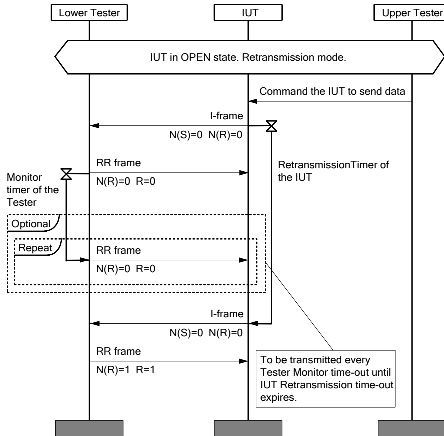
Figure 4.43: L2CAP/COS/RTX/BV-02-C [Retransmission with R=0 in RR frame]
