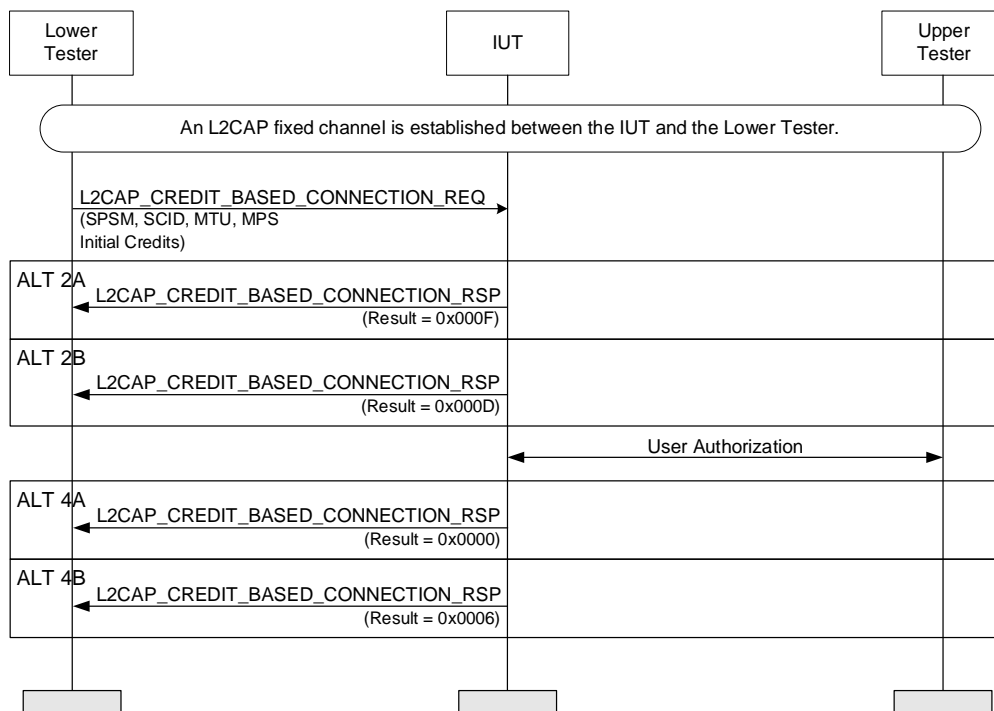
Figure 4.249: L2CAP/ECFC/BV-44-C [Security – Insufficient Authorization – Responder, LE]
