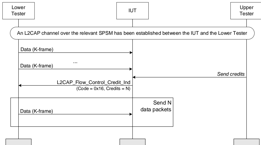
Figure 4.197: Credit Exchange – Sending Credits
