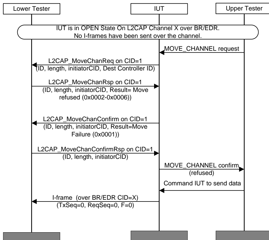
Figure 4.149: L2CAP/MCH/BV-17-C [Move Channel Request for BR/EDR to AMP (STM Source) – Refused]
