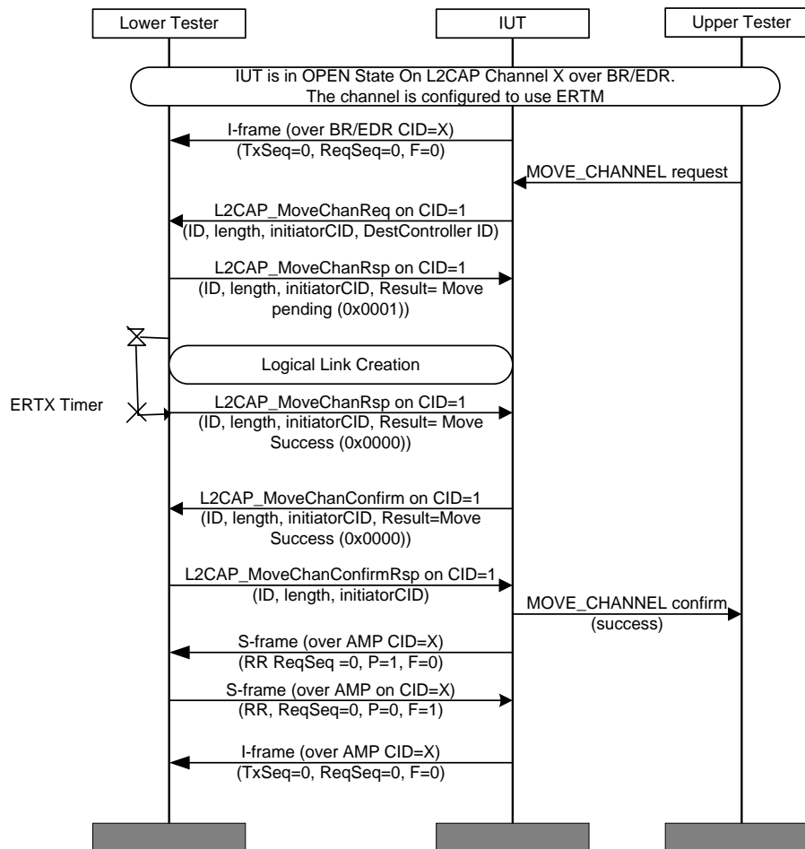
Figure 4.143: L2CAP/MCH/BV-11-C [Data Transfer while Moving ERTM Channel from BR/EDR to AMP – Unacknowledged Data]
