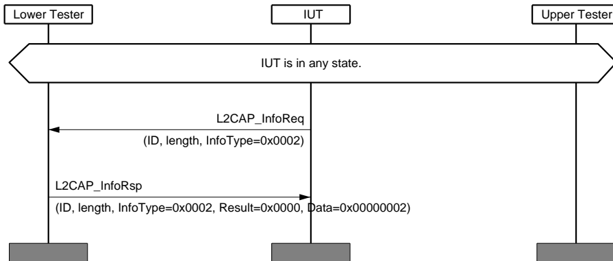
Figure 4.24: L2CAP/COS/IE/BV-01-C [Query for 1.2 Features]
