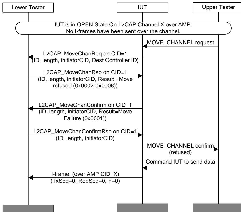
Figure 4.155: L2CAP/MCH/BV-23-C [Move Channel Request for AMP to BR/EDR (STM Source) – Refused]
