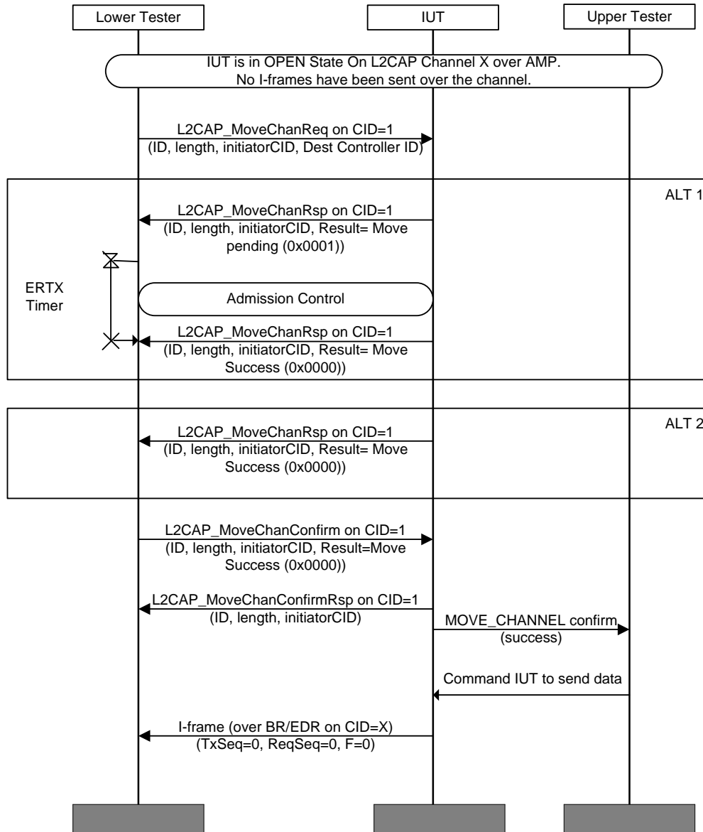
Figure 4.161: L2CAP/MCH/BV-29-C [Move Channel Response for AMP to BR/EDR (STM Source) – Success]
