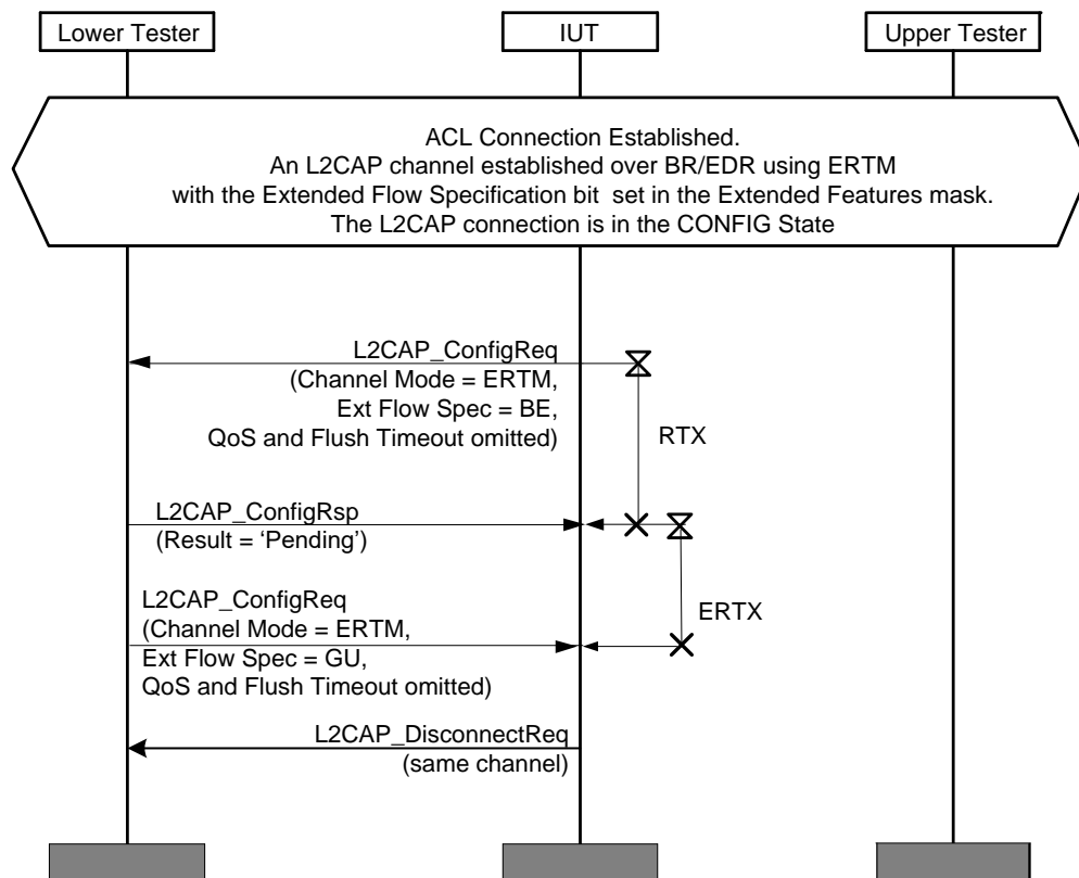
Figure 4.120: L2CAP/LSC/BI-04-C [Mismatched Service Type, Best Effort, BR/EDR ERTM Channel]
