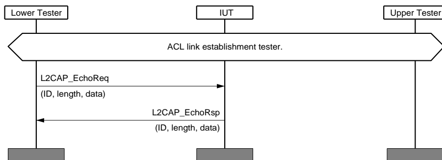
Figure 4.26: L2CAP/COS/ECH/BV-01-C [Respond to Echo Request]
