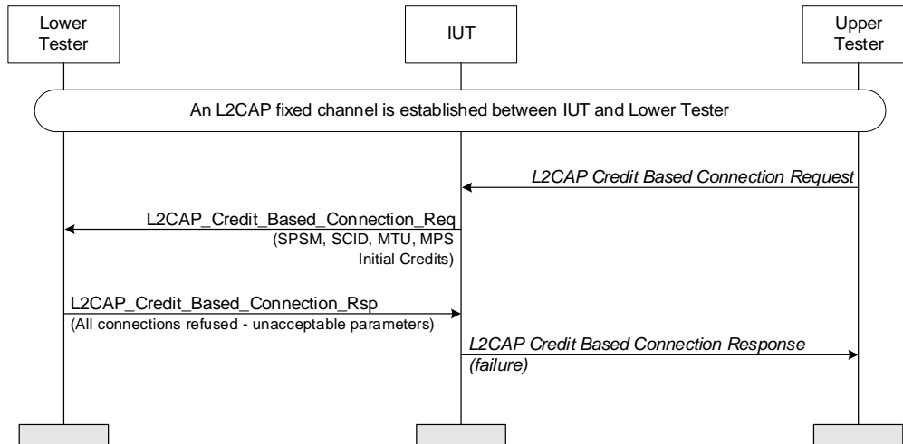
Figure 4.206: L2CAP Credit Based Connection Request – refused due to Unacceptable Parameters
