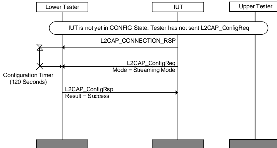
Figure 4.51: L2CAP/CMC/BV-04-C [IUT Initiated Configuration of Streaming Mode]
