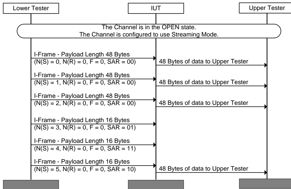
Figure 4.178: L2CAP/STM/BV-02-C [Streaming Mode Sink with Extended Control Field]
