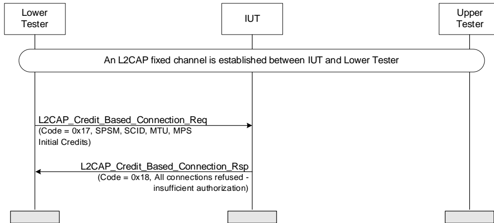
Figure 4.239: Security – Insufficient Authorization – Responder
