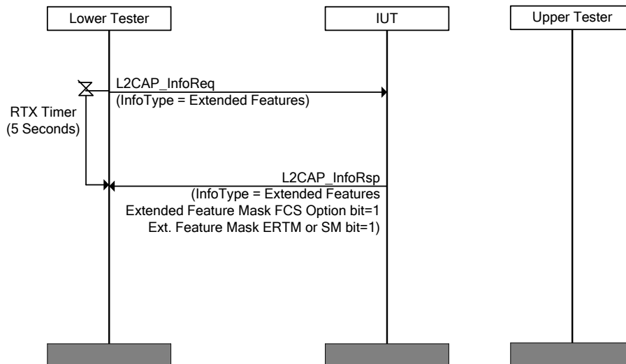
Figure 4.47: L2CAP/EXF/BV-03-C [Extended Features Information Response for FCS Option]
