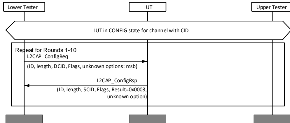
Figure 4.23: L2CAP/COS/CFD/BV-14-C [Unknown Mandatory Options Request]
