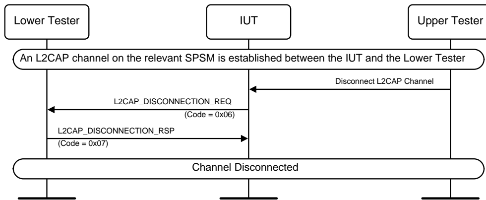
Figure 4.235: Disconnection Request
