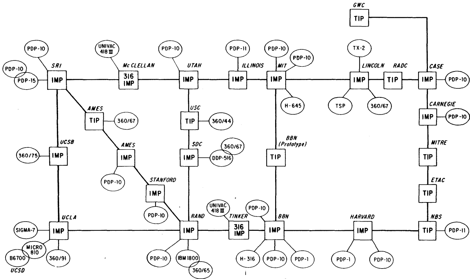
ARPA NETWORK, LOGICAL MAP, MARCH 1972
