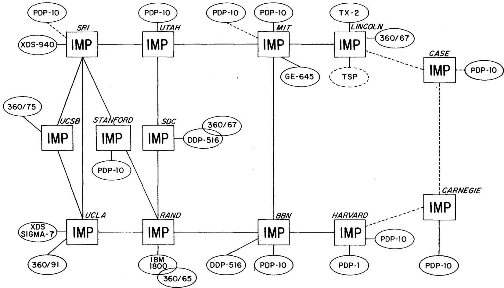
ARPA NET, DECEMBER 1970
