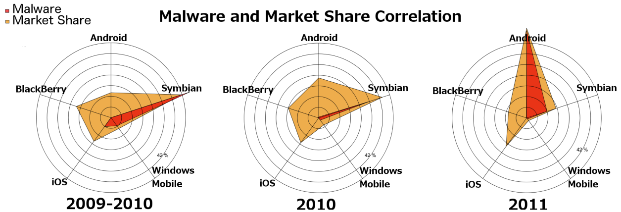
Fig. 2. Correlation between the number of malware cases and platform market share during a) 2009-2010 [41], b) 2010 [2], and c) 2011 [2].
