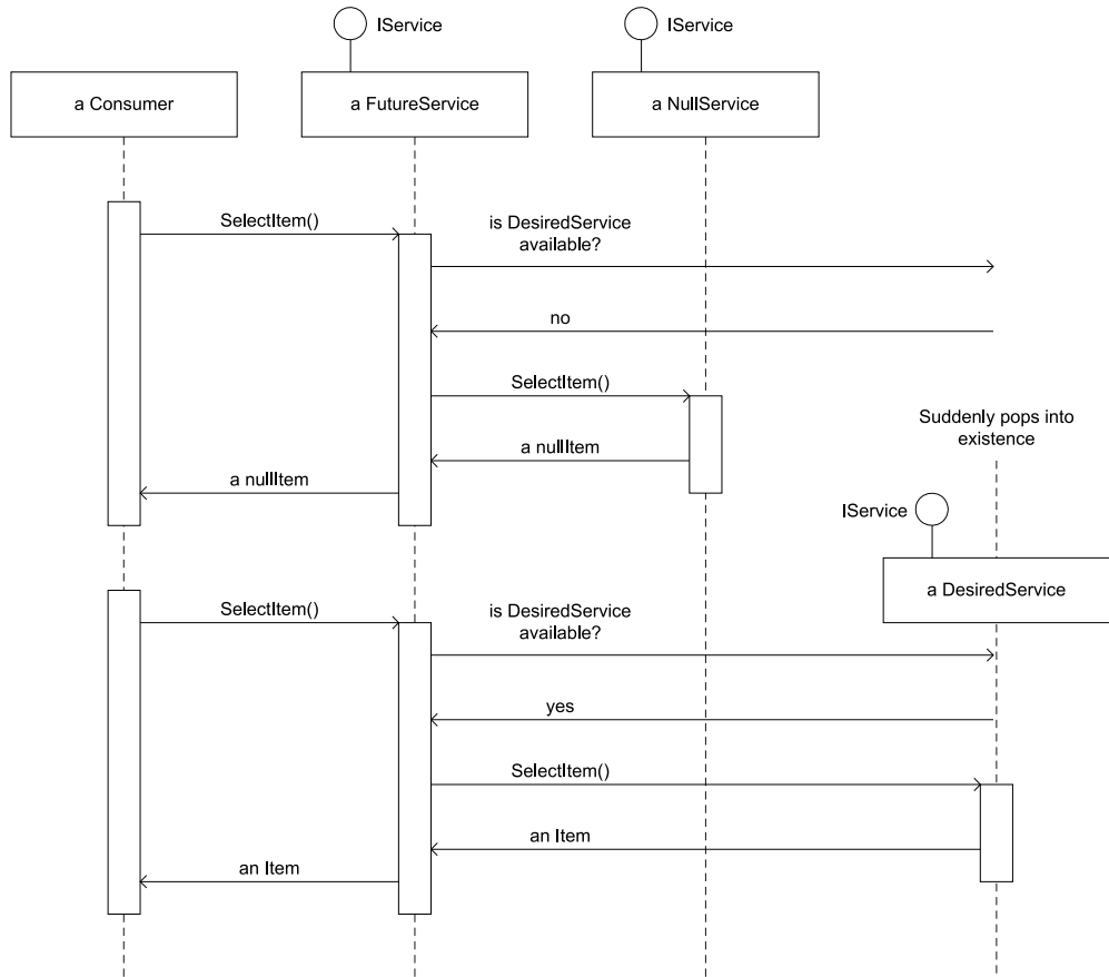
Figure 8.14 A consumer requires an instance of IService , but DesiredService may not yet be available. In this case, we can encapsulate a NullService as a stand-in to be used while we wait for Godot. FutureService is a state machine that polls to see if DesiredService has become available. As long as it isn't, the FutureService Decorator has no choice but to use the fallback implementation provided by NullService . When DesiredService finally becomes available, all future requests are directed to it.
