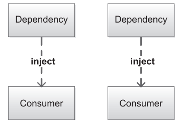
Figure 1.14 Each consumer sharing the same type of DEPENDENCY is injected with its own private instance.
