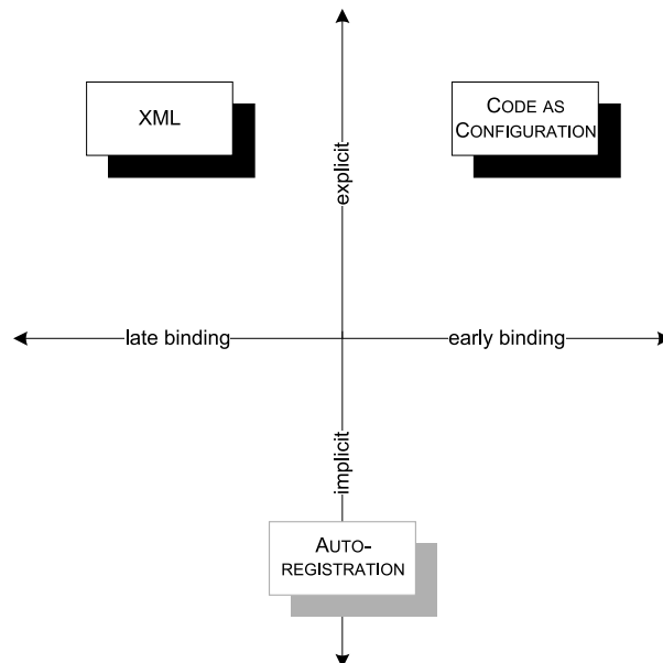
Figure 14.3 Conceptually different configuration options. CODE AS CONFIGURATION is strongly typed and tends to be explicit. XML , on the other hand, is late bound, but still explicit. AUTO-REGISTRATION instead relies on conventions that can be both strongly typed and more loosely defined, but Unity has no built-in support for that.
