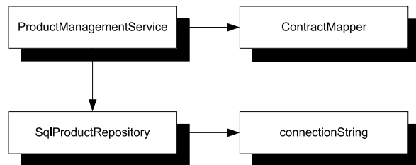
Figure 8.5 Object graph as created by CommerceServiceContainer . Each ProductManagementService instance created contains its own ContractMapper and its own SqlProductRepository , which in turn contains its own connection string. The DEPENDENCIES on the right are immutable.
