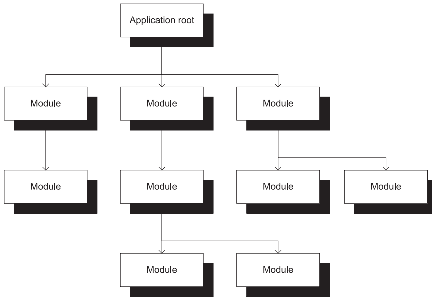
Figure 3.7 The entry point of an application is the root of a modular application. Either directly or indirectly, the root consumes the other modules. A COMPOSITION ROOT should be placed in the application’s root—as close to the entry point as possible.
