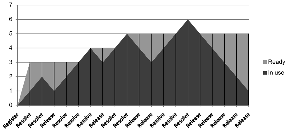
Figure 10.4 Size progression of a pool with an initial size of 3 and maximum size of 5. Even though the initial size of the pool is 3, the pool stays empty until the first instance is resolved. At that point, all 3 instances for the initial size are created and one is immediately put to use. When an instance is released, it's returned to the pool. The pool increases in size if more instances than the minimum size are necessary. Notice that it's possible to exceed the maximum size, but that the surplus instances aren't recycled when released.
