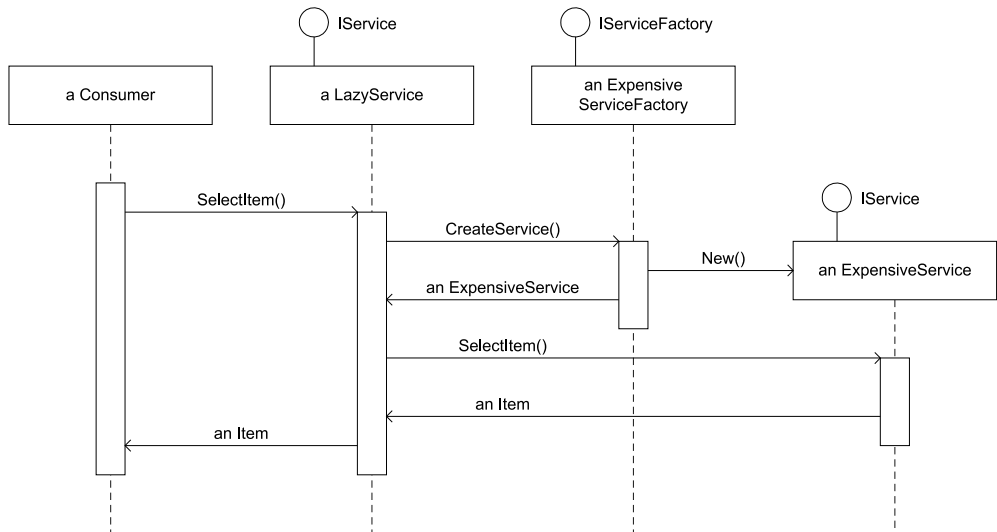
Figure 8.13 A consumer requires an IService DEPENDENCY , but if it only uses this DEPENDENCY in a small fraction of the time, it can live for a long time before requiring the services of IService . When it finally invokes IService.SelectItem() , LazyService uses its injected IServiceFactory to create an instance of another IService . It isn't until this point that the ExpensiveService instance is created. After ExpensiveService is created, all subsequent calls can be delegated to it.
