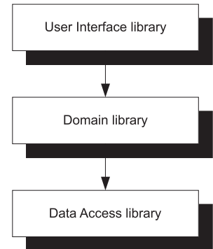
Figure 2.13 Dependency graph of the hypothetical situation where the dependency of the User Interface on the Data Access library has been severed.
