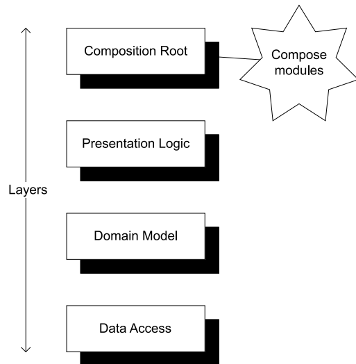
Figure 7.2 The COMPOSITION ROOT composes all the independent modules of the application. In contrast to mise en place , this doesn't happen as late as possible, but happens in a place where the integration of the different modules is required.
