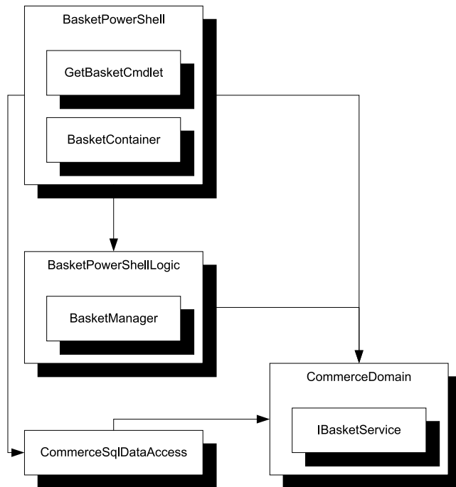
Figure 7.18 The BasketPowerShell library only contains the infrastructure necessary to make PowerShell happy—it's a HUMBLE OBJECT. As soon as the static BasketContainer has resolved a BasketManager , all further implementation happens in different assemblies. The BasketManager class has no access to the internal BasketContainer but consumes an IBasketService from the Domain Model. As usual, arrows denote references. Not all involved classes are shown.
