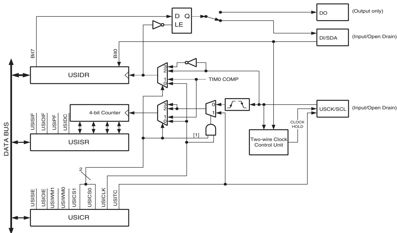
Figure 1-3. Universal Serial Interface, Block Diagram
