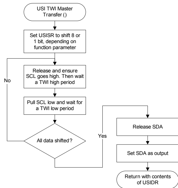
Figure 2-2. Flowchart of the general transfer function. The function is used by the USI_TWI_Start_Transceiver_With_Data function in Figure 2-1
