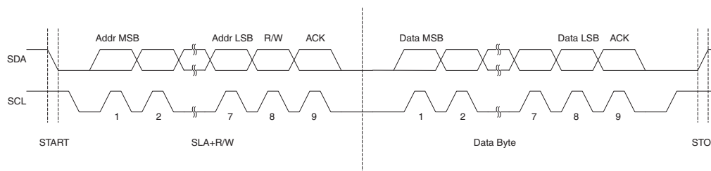
Figure 1-2. TWI Address and Data Packet Format
