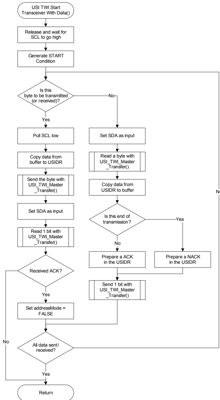
Figure 2-1. Flowchart of the transceiver function. A flowchart of the sub function USI_TWI_Master_Transfer is found in Figure 2-2
