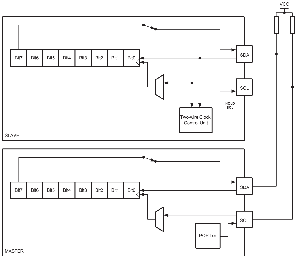
Figure 1-4. Two-wire Mode Operation, Simplified Diagram
