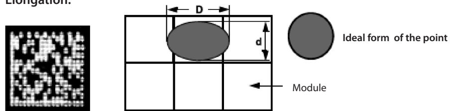
Figure 3.6.2-4 Elongation
