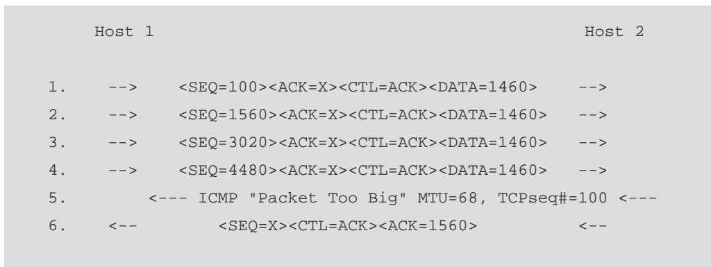
Figure 23: Active connection being attacked after discovery of PMTU
