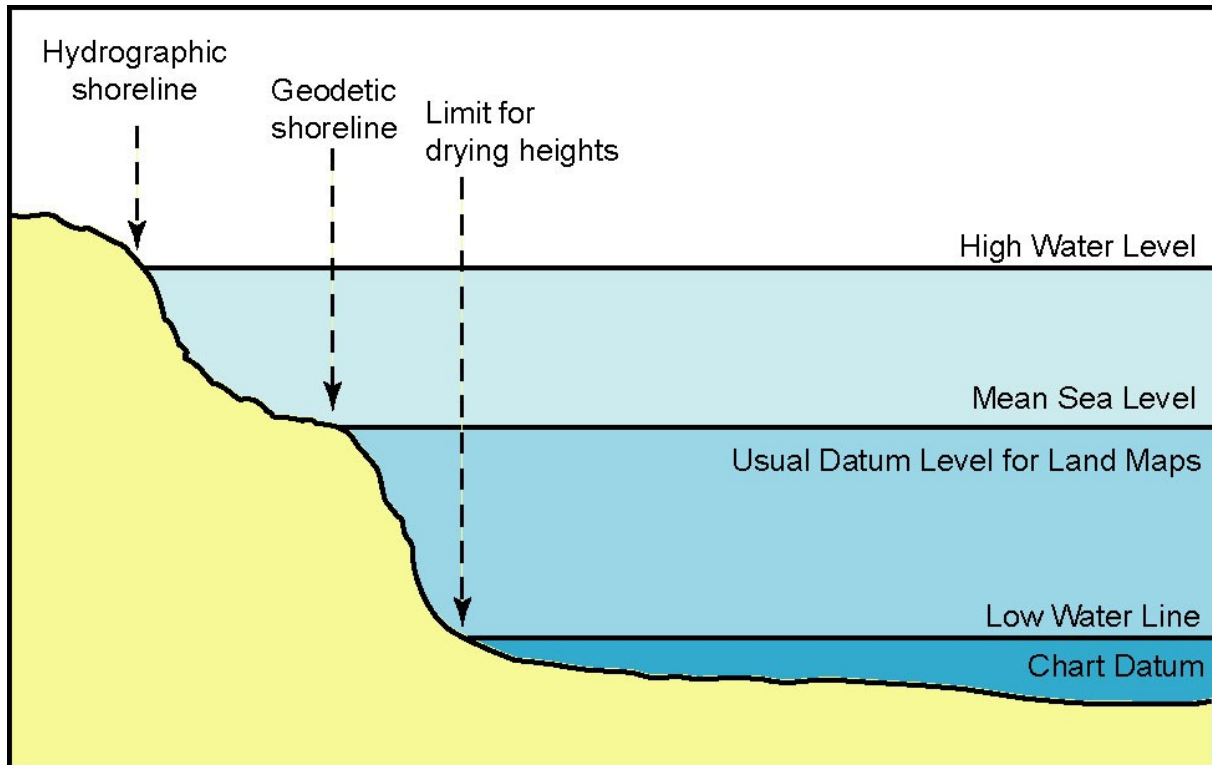
Figure 2.9 - Vertical Datums
