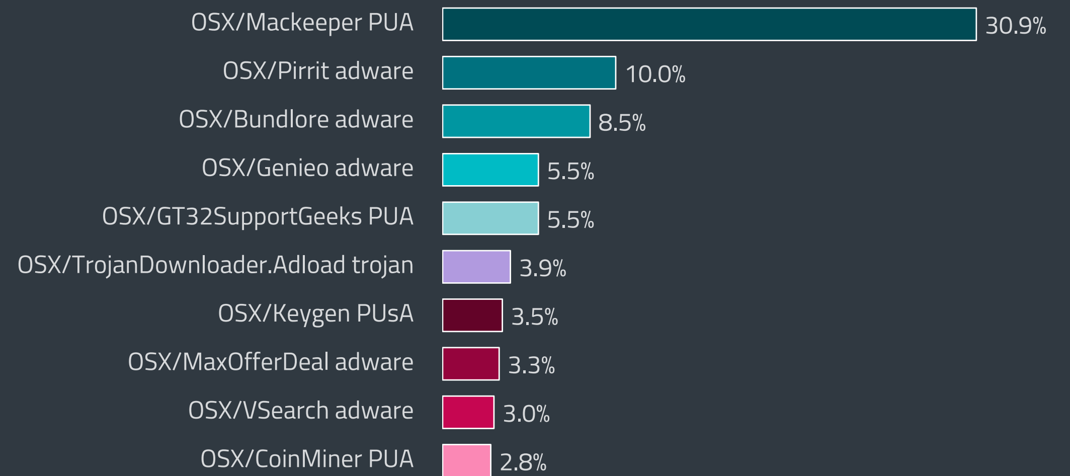
Top 10 macOS detections in T1 2022
