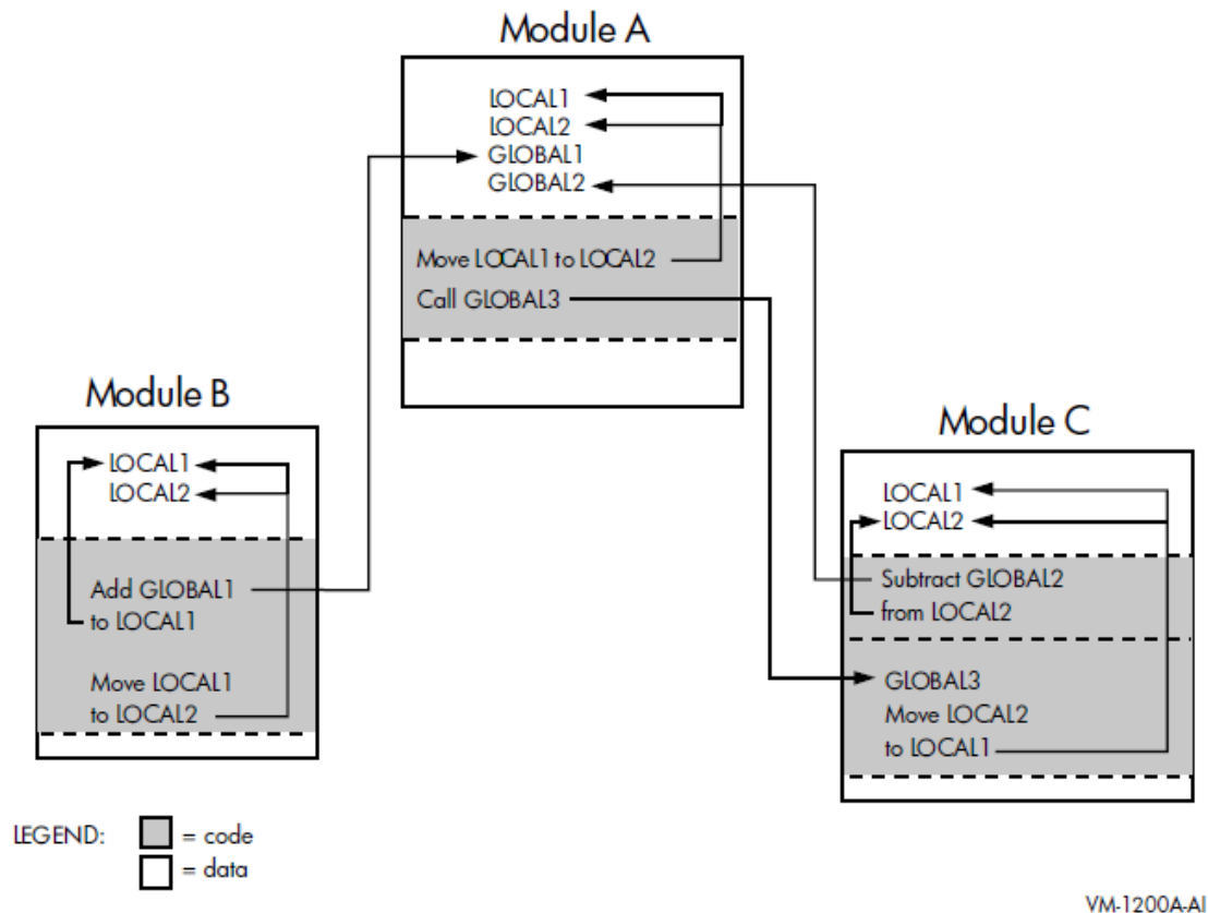
Figure 2.3. Symbol Resolution
