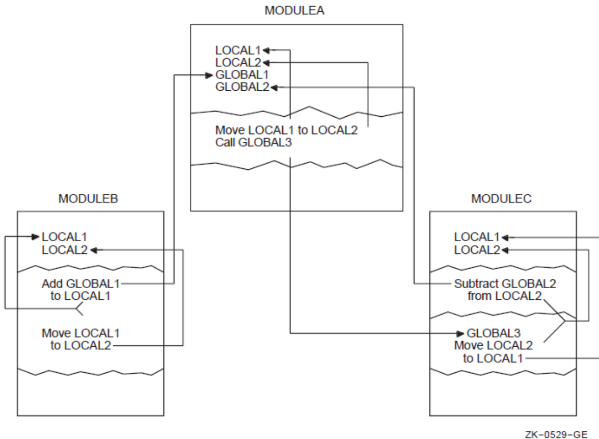
Figure 6.2. Symbol Resolution
