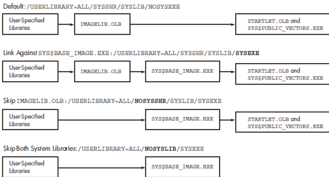
Figure 2.5. Linker Processing of Default Libraries and SYS$BASE_IMAGE.EXE
