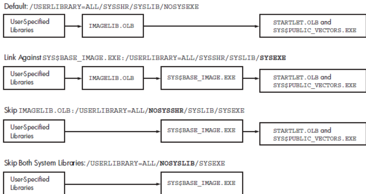
Figure 6.4. Linker Processing of Default Libraries and SYSS$BASE_IMAGE.EXE
