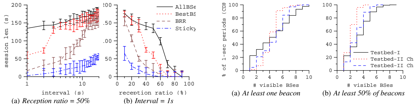
Figure 4: The median session length in VanLAN as a function of the time interval (a) and the minimum reception ratio (b) used to define adequate connectivity. The left graph has logarithmic x -axis. Error bars represent 95% confidence intervals.
